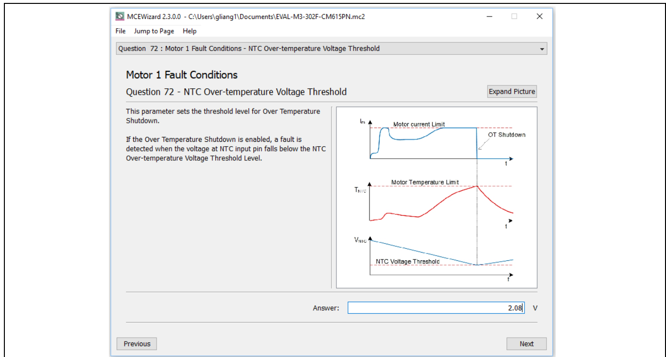
Figure 25 External temperature-sensing input configuration in MCEWizard
