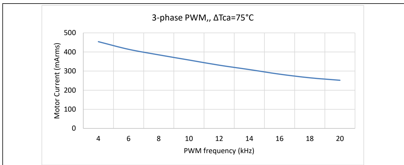
Figure 14 Thermal Characterization of IMI111T-026H, 3-phase PWM, \Delta T_{ca} = 75^\circ\text{C} , FR4 PCB with 1 oz copper
