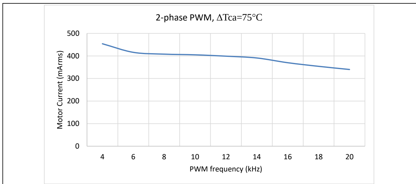
Figure 13 Thermal Characterization of IMI111T-026H, 2-phase PWM, \Delta T_{ca} = 75^\circ\text{C} , FR4 PCB with 1 oz copper
