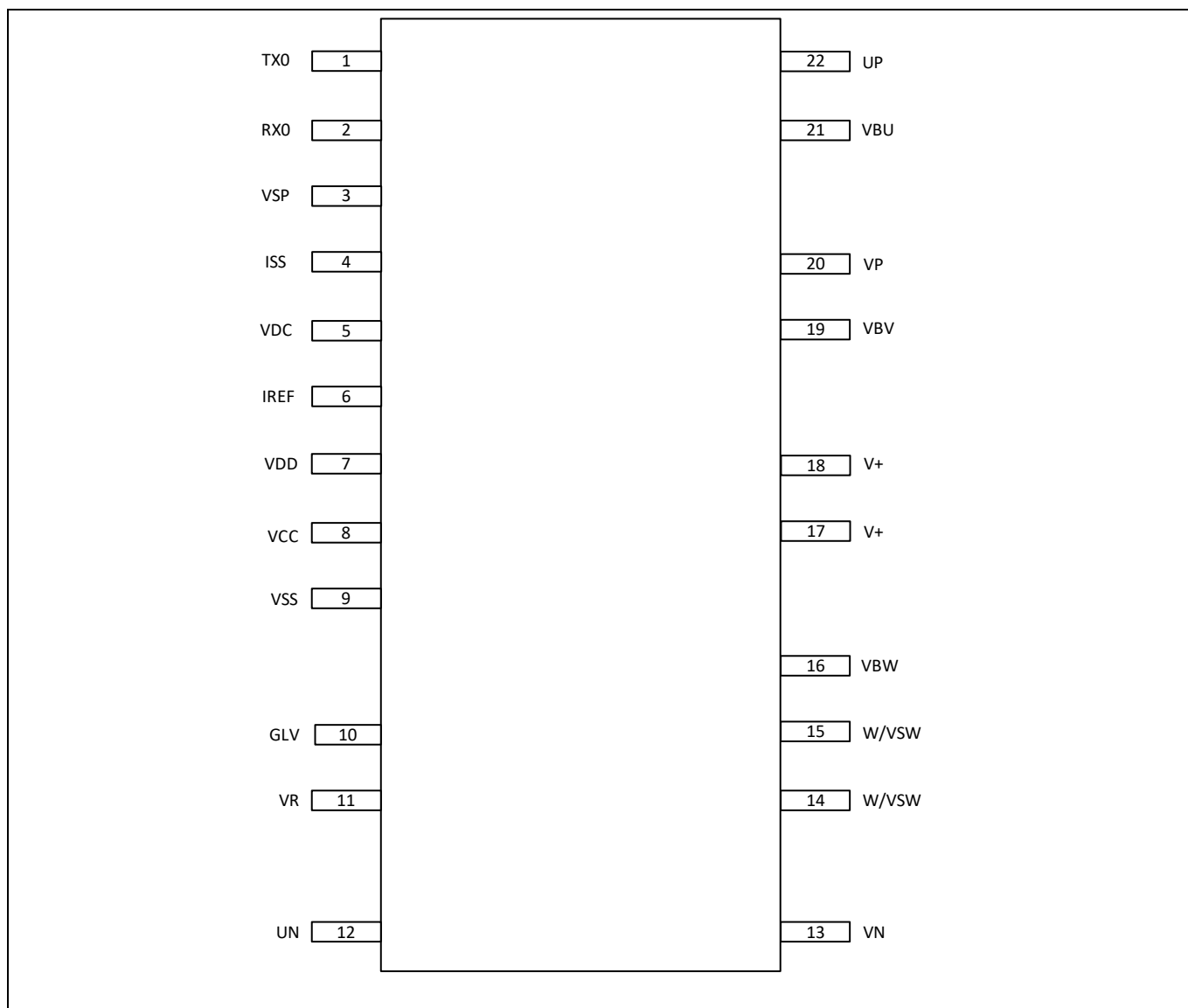
Figure 3 IMI111T pinout
