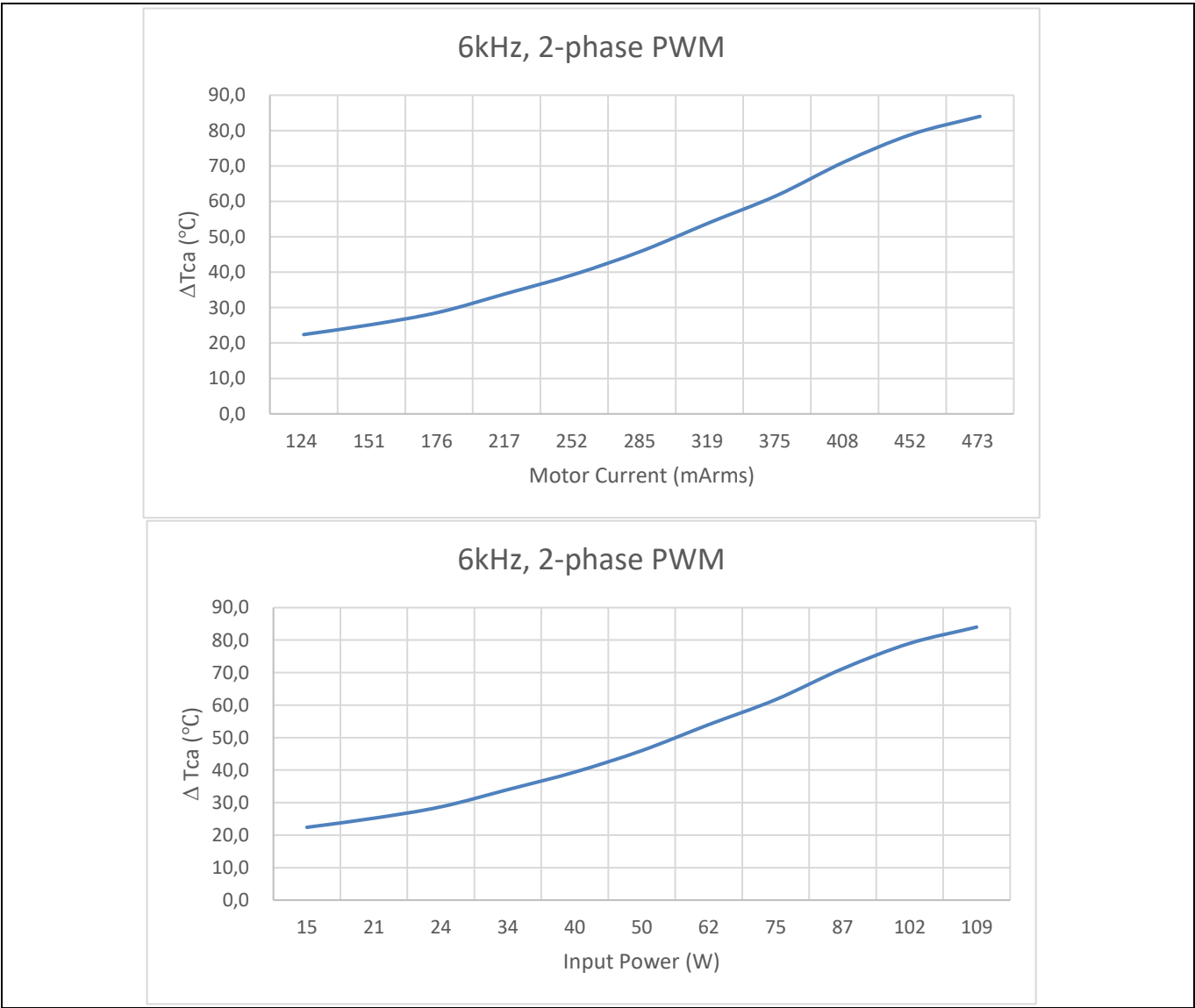
Figure 11 Thermal Characterization of IMI111T-026H, 2-phase PWM, 6 kHz, FR4 PCB with 1 oz copper
