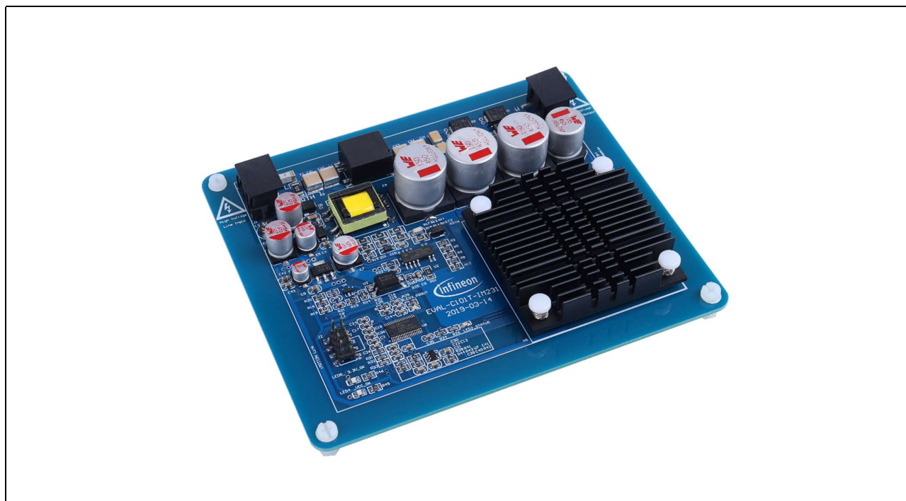
Figure 1 Evaluation board of the EVAL-C101T-IM231
