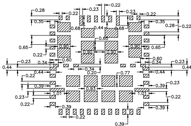
Figure A.2.3(a) 7x7 stencil design
