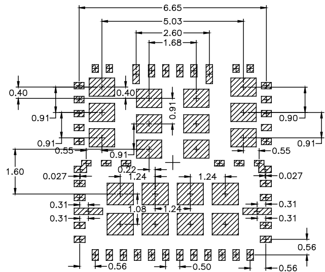
Figure A.2.3(b) 7x7 stencil design
