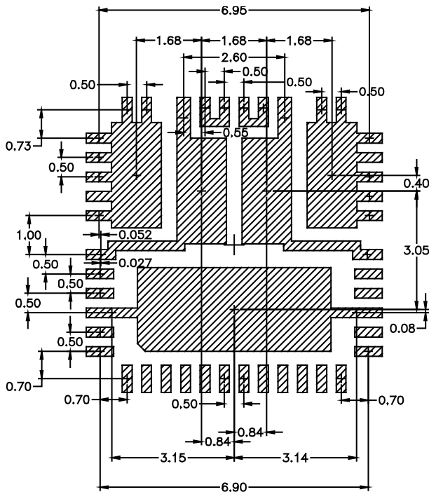
Figure A.2.2(c) 7x7 substrate/PCB layout
