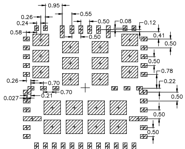
Figure A.2.3(c) 7x7 stencil design
