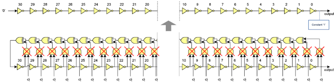
Figure 11-13. FIRO31 “stopped”
