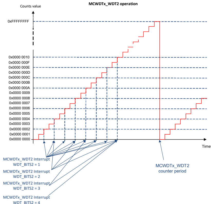
Figure 23-5. MCWDTx_WDT2 Operation
