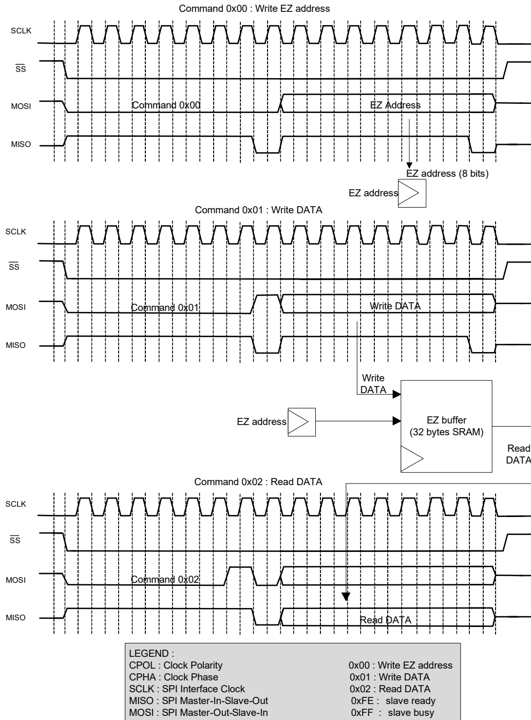
Figure 26-9. EZSPI Example
