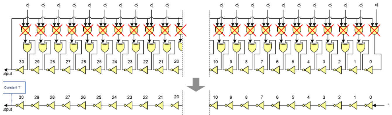
Figure 11-10. GARO31 “stopped”
