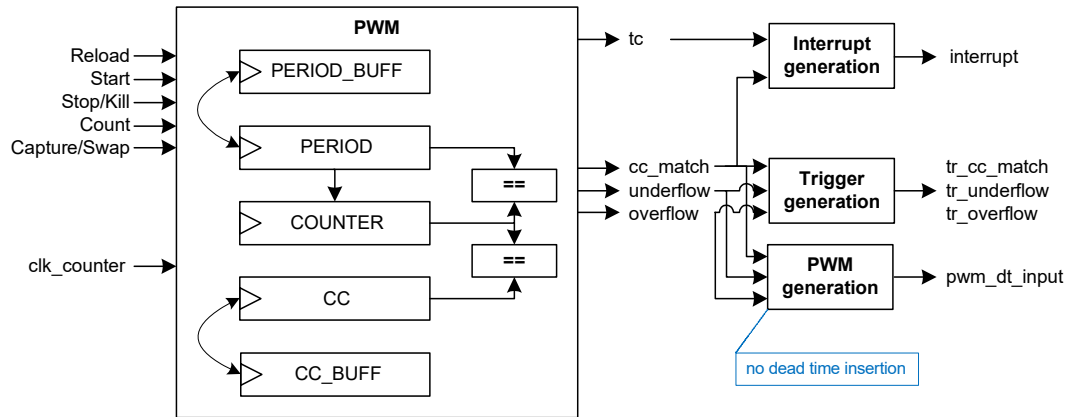
Figure 28-23. PWM Mode Functionality
