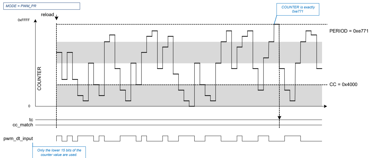
Figure 28-42. PWM_PR Output
