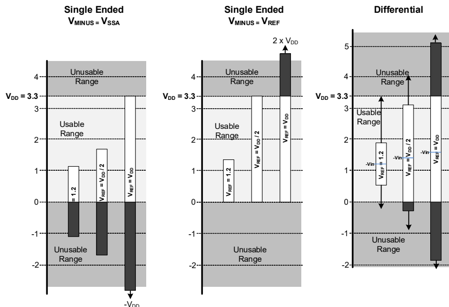
Figure 39-2. Input Range
