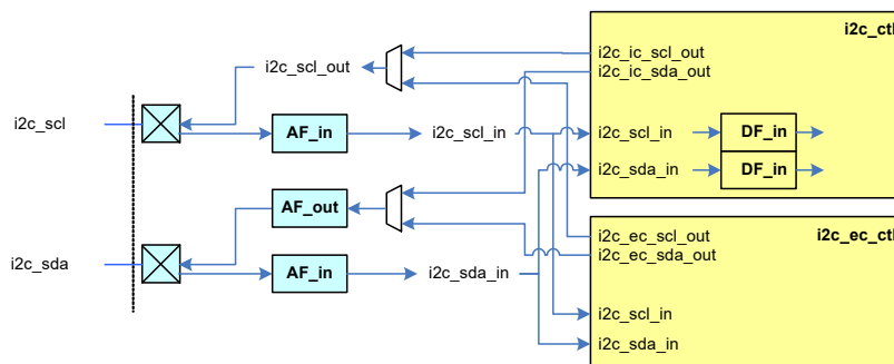
Figure 26-42. I 2 C Glitch Filtering Connection
