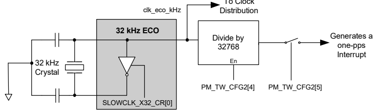
Figure 14-7. RTC Implementation
