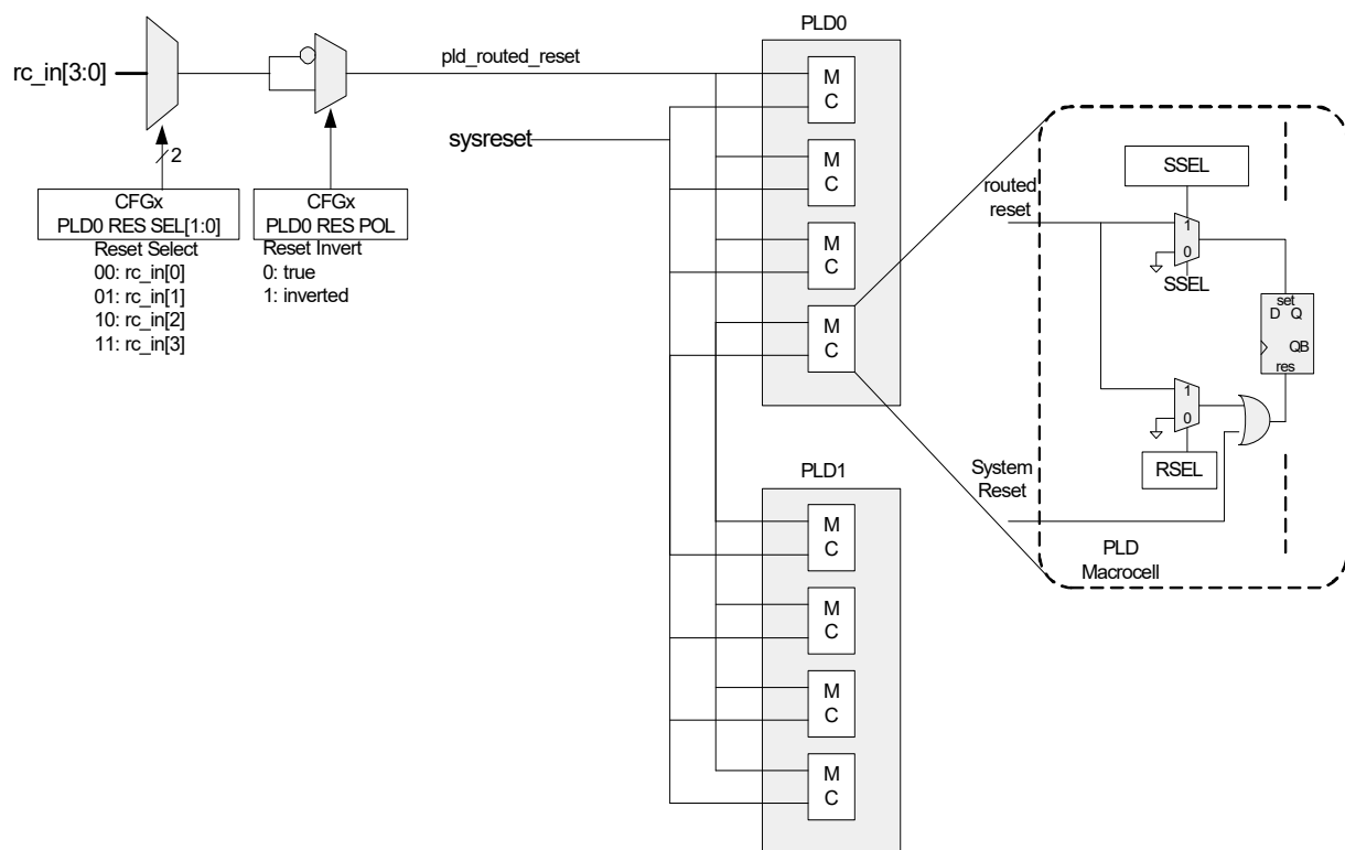
Figure 21-40. PLD Reset Structure
