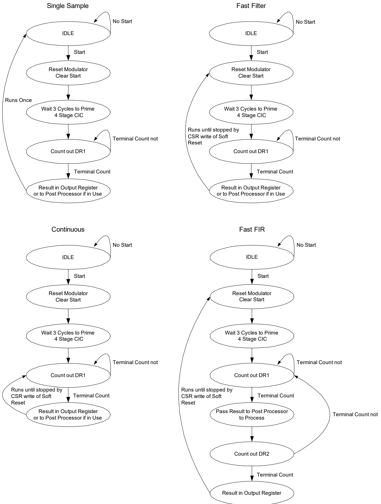
Figure 37-10. Decimator Modes
