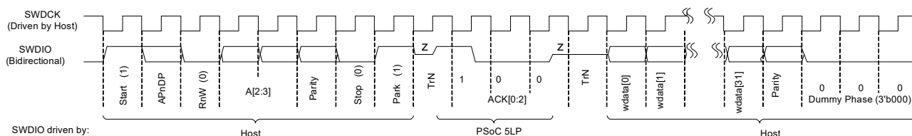
Figure 39-5. SWD 'Write Packet' Timing Diagram
