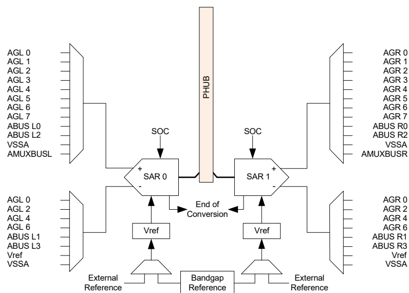
Figure 38-1. SAR ADC Block Diagram
