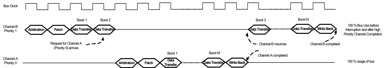
Figure 6-6. Priority 0 and Priority 1
