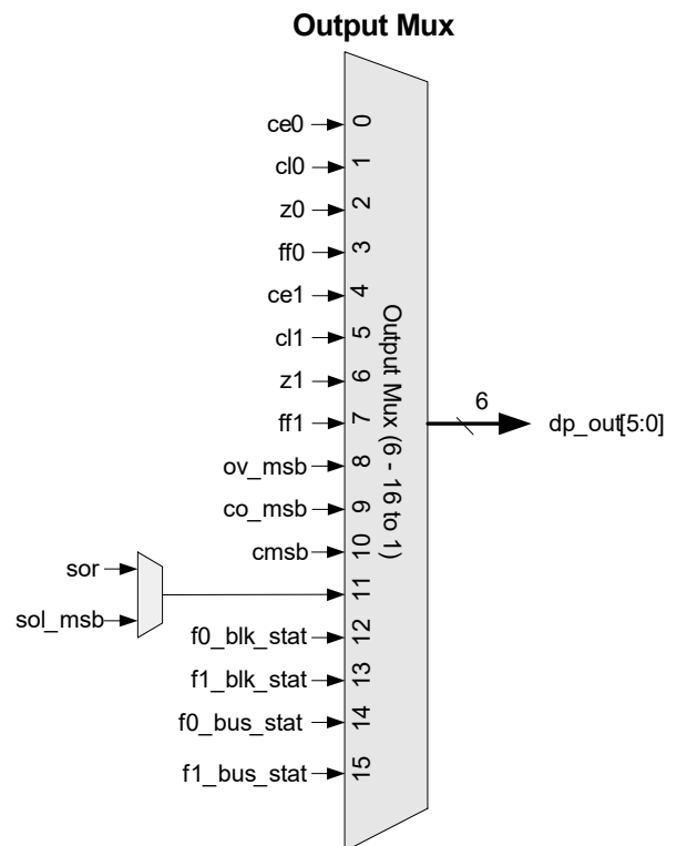
Figure 21-22. Output Mux Connections
