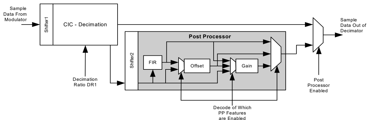
Figure 37-9. Decimator
