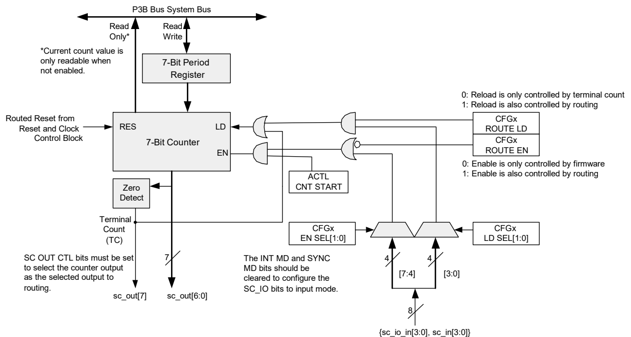
Figure 21-36. Counter Mode
