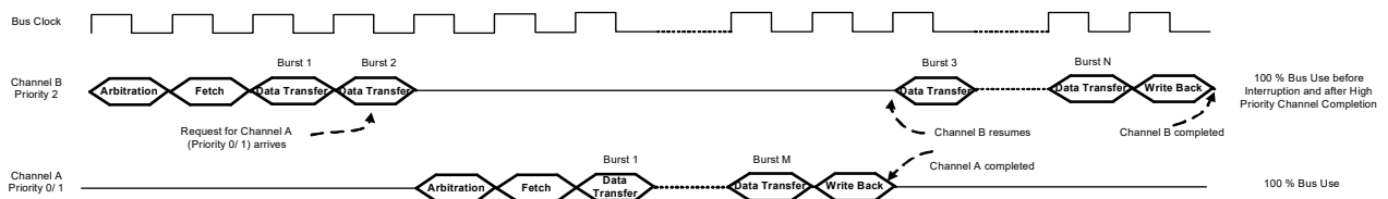
Figure 6-7. Priority 0/1 and Other Low Priority
