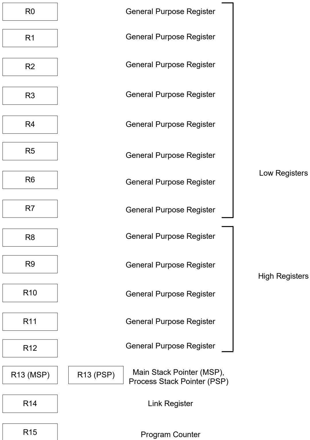
Figure 4-2. Cortex-M3 Registers
