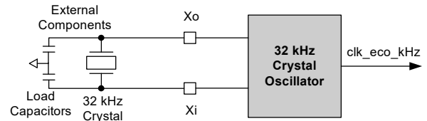
Figure 14-6. kHzECO Block Diagram
