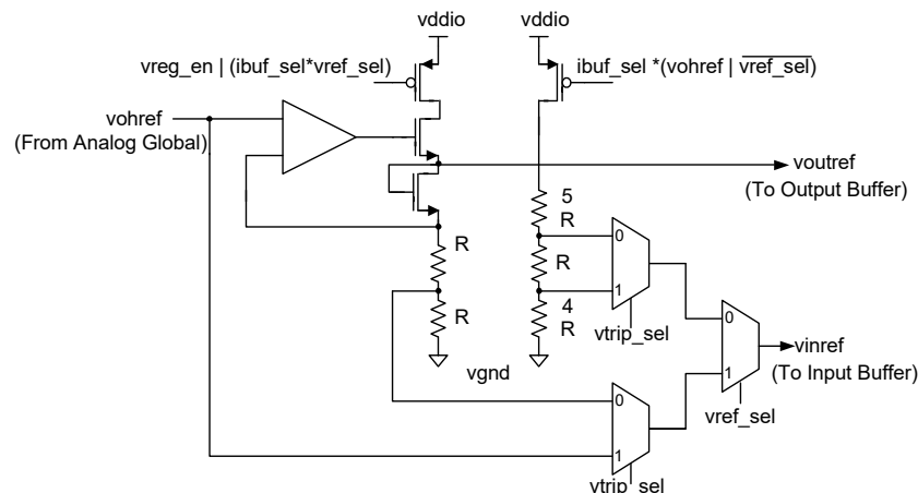
Figure 19-10. SIO Reference Voltage
