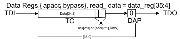
Figure 39-10. TC in APACC while DAP in BYPASS
