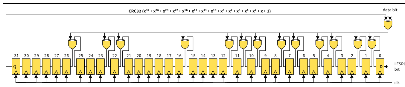
Figure 11-7. CRC32 functionality
