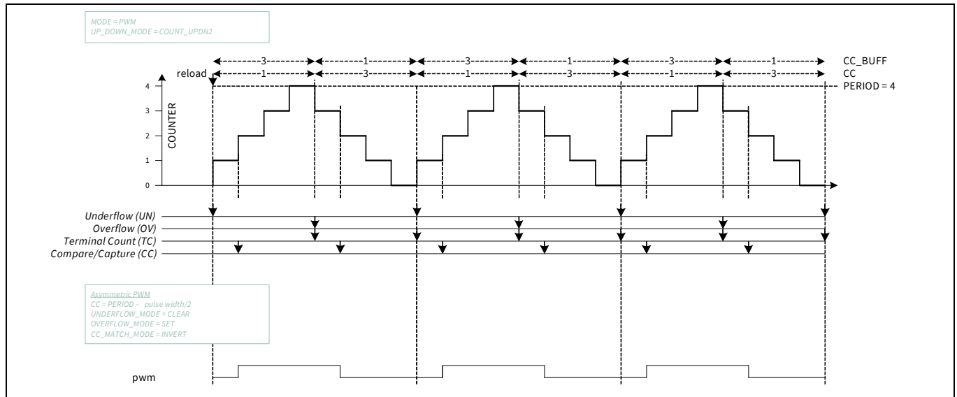
Figure 28-36. Asymmetric PWM
