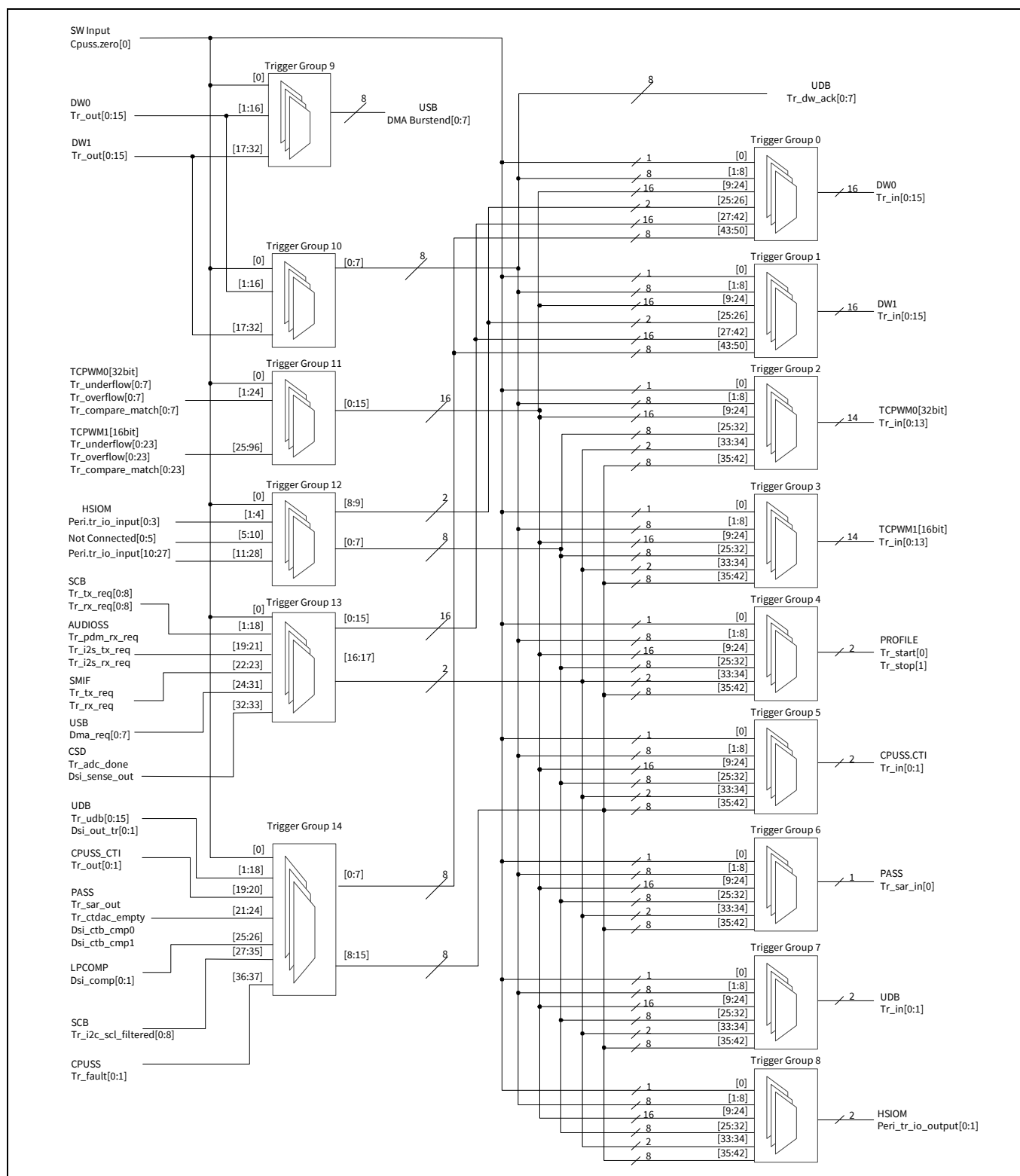
Figure 24-4. PSoC™ 6 MCU trigger multiplexer block architecture
