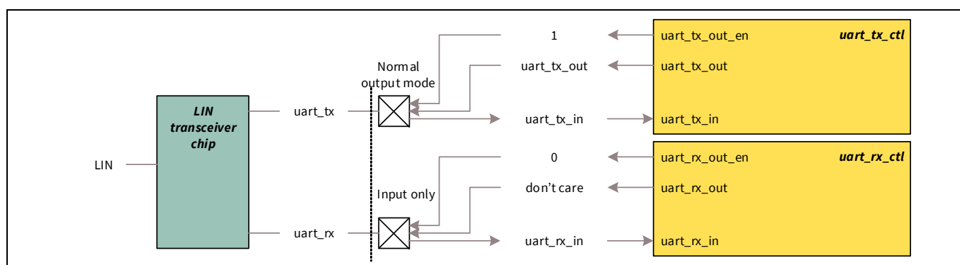
Figure 26-34. LIN mode I/O pad connections
