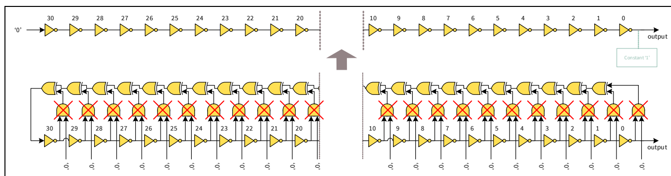
Figure 11-17. FIRO31 "stopped"
