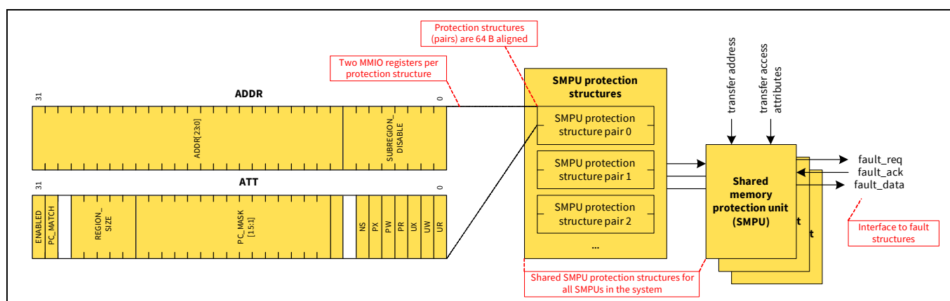
Figure 9-4. SMPU functionality
