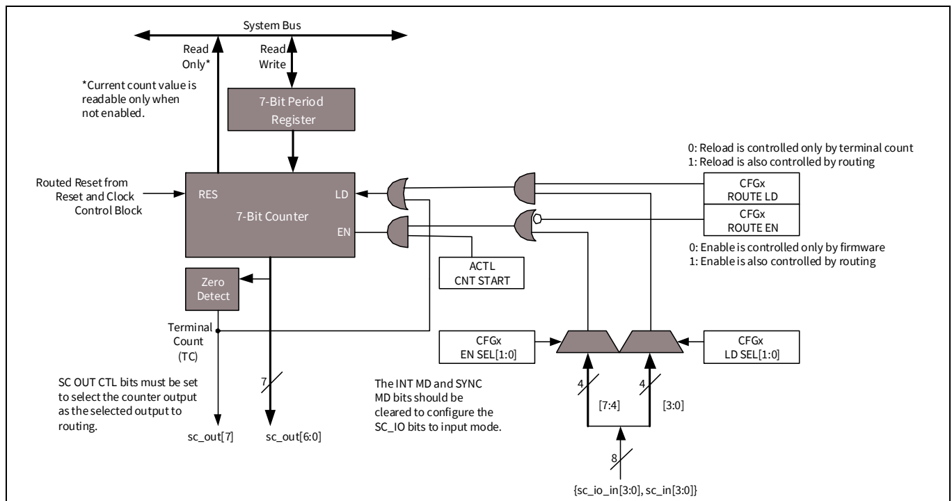
Figure 34-37. Counter mode
