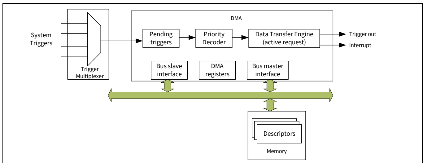
Figure 10-1. DMA controller
