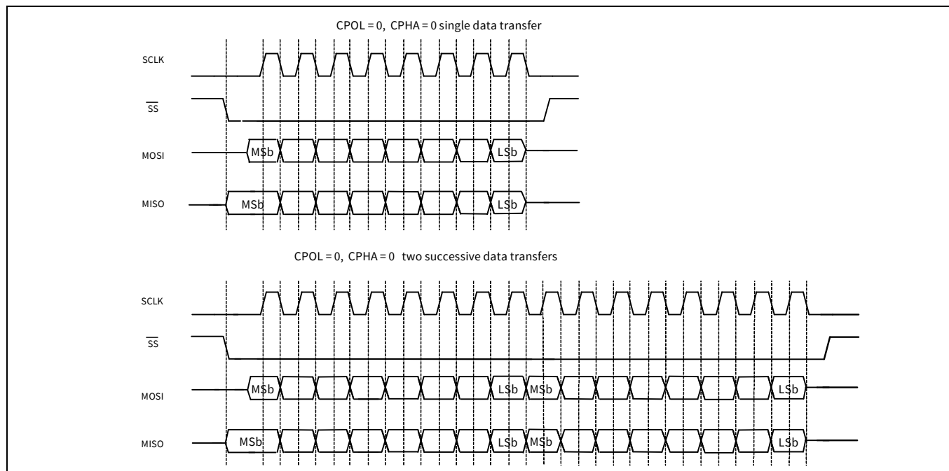
Figure 26-3. SPI Motorola data transfer example
