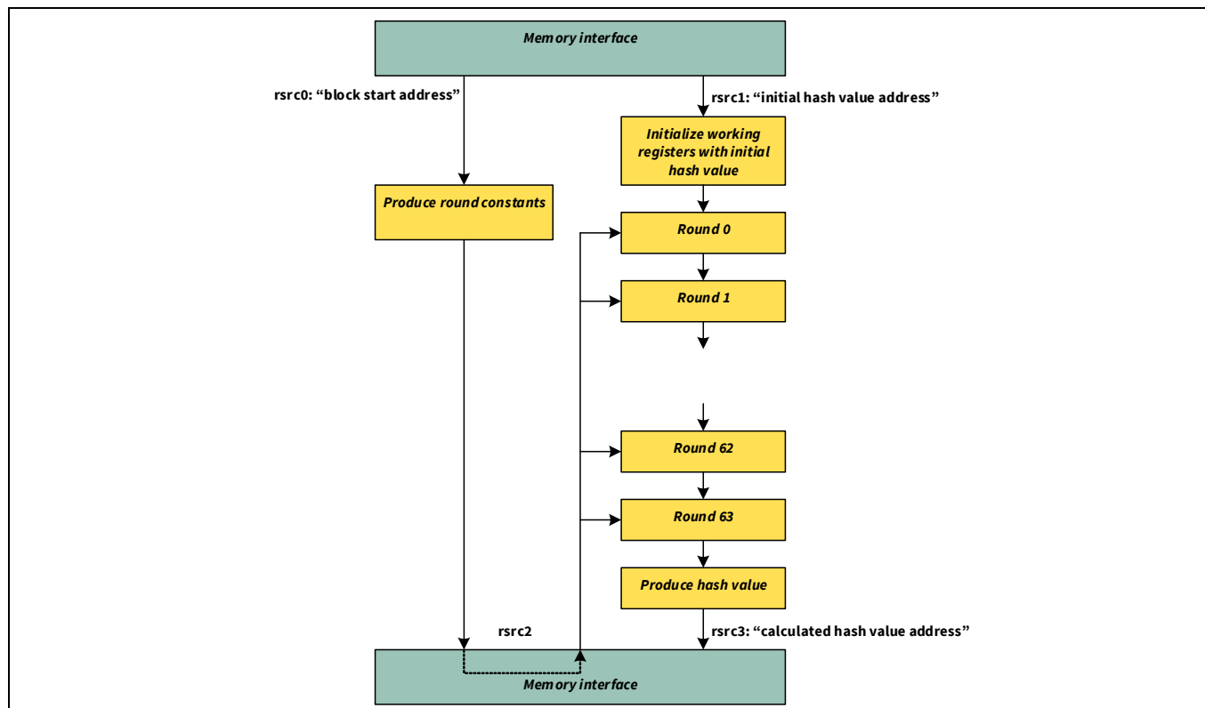
Figure 11-5. SHA functionality
