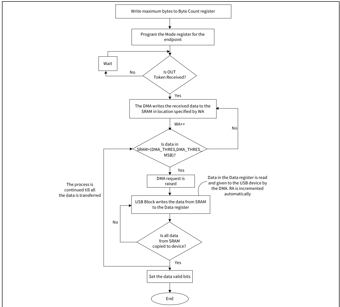
Figure 31-8. OUT Transaction using automatic DMA mode
