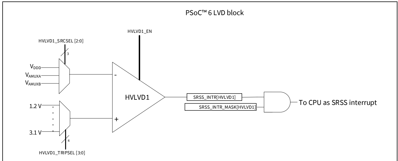
Figure 17-2. PSoC™ 6 MCU LVD block
