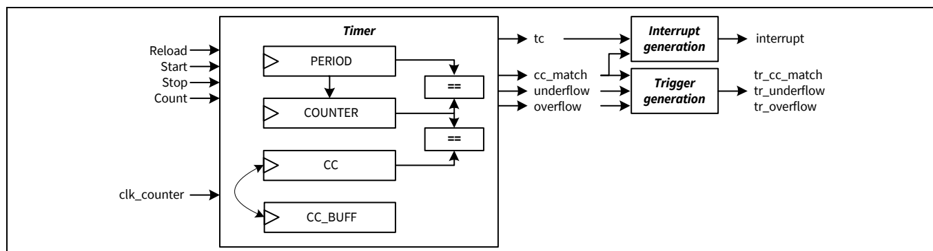
Figure 28-6. Timer functionality
