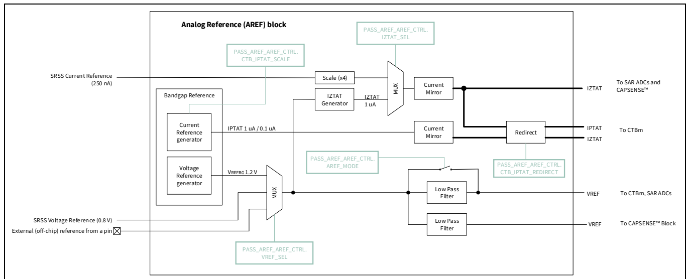
Figure 35-1. AREF block diagram
