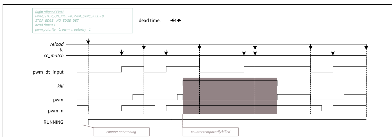
Figure 28-40. Dead time and kill
