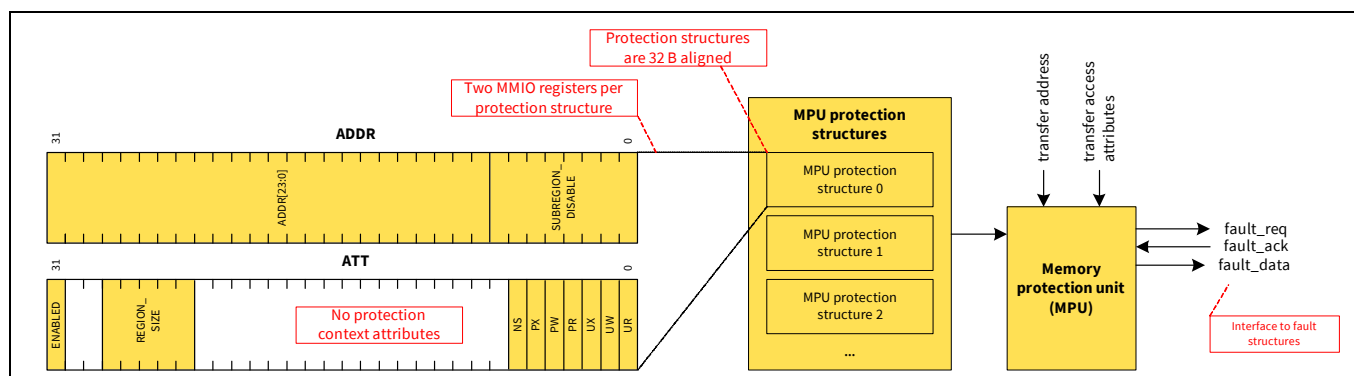
Figure 9-3. MPU functionality
