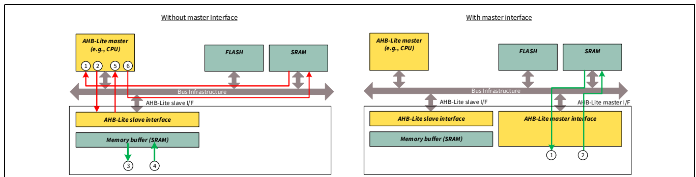
Figure 11-3. AHB-Lite interface
