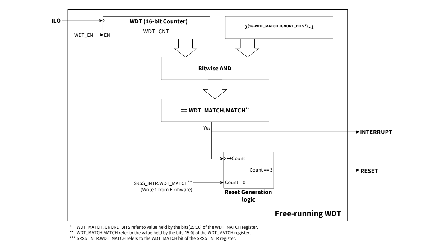
Figure 23-2. Free-running WDT functional diagram
