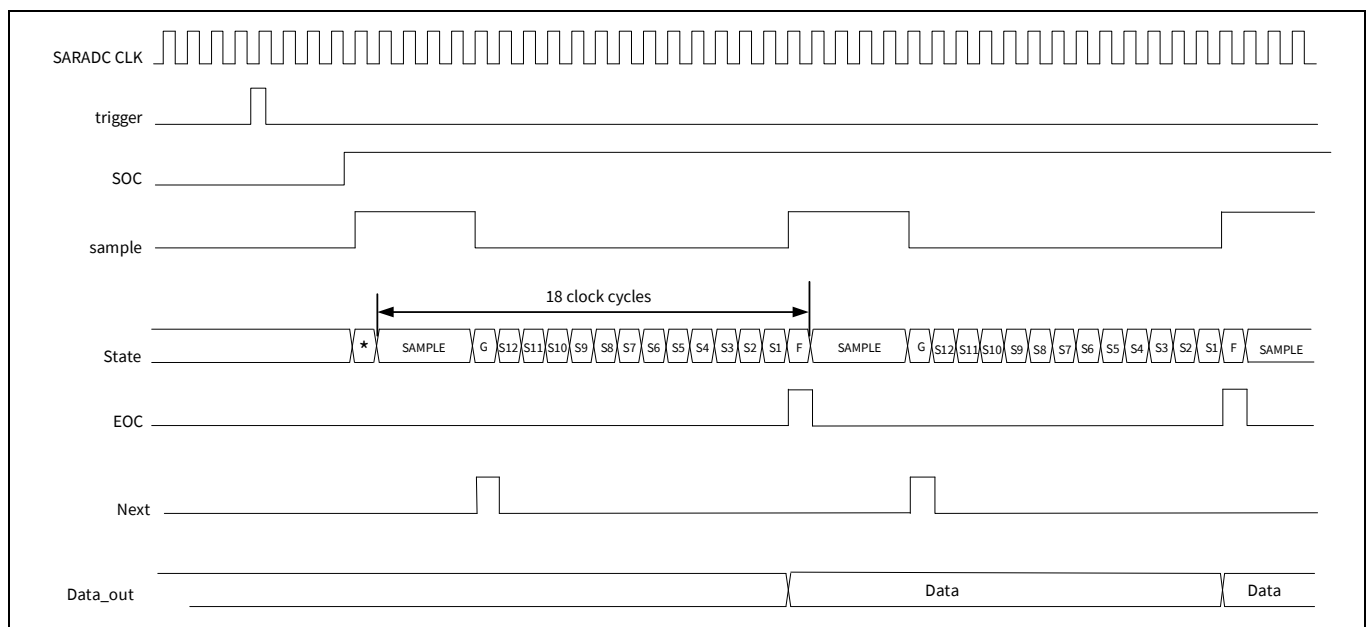
Figure 39-4. SAR ADC timing
