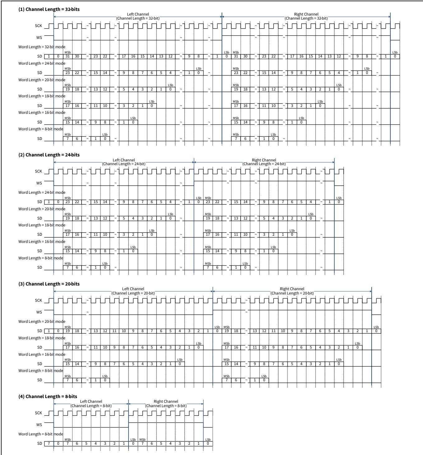
Figure 29-2. Standard I²S format (word length and channel length combination timing diagrams)
