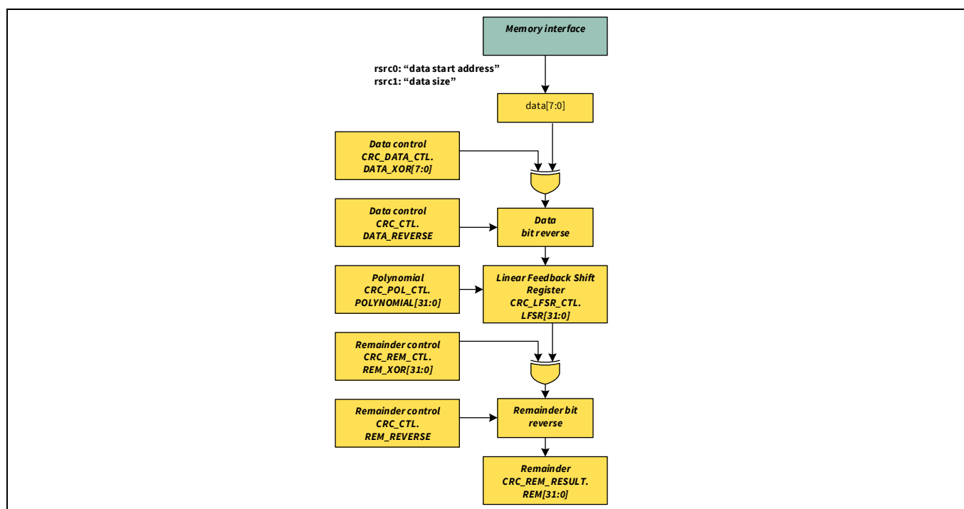
Figure 11-6. CRC functionality
