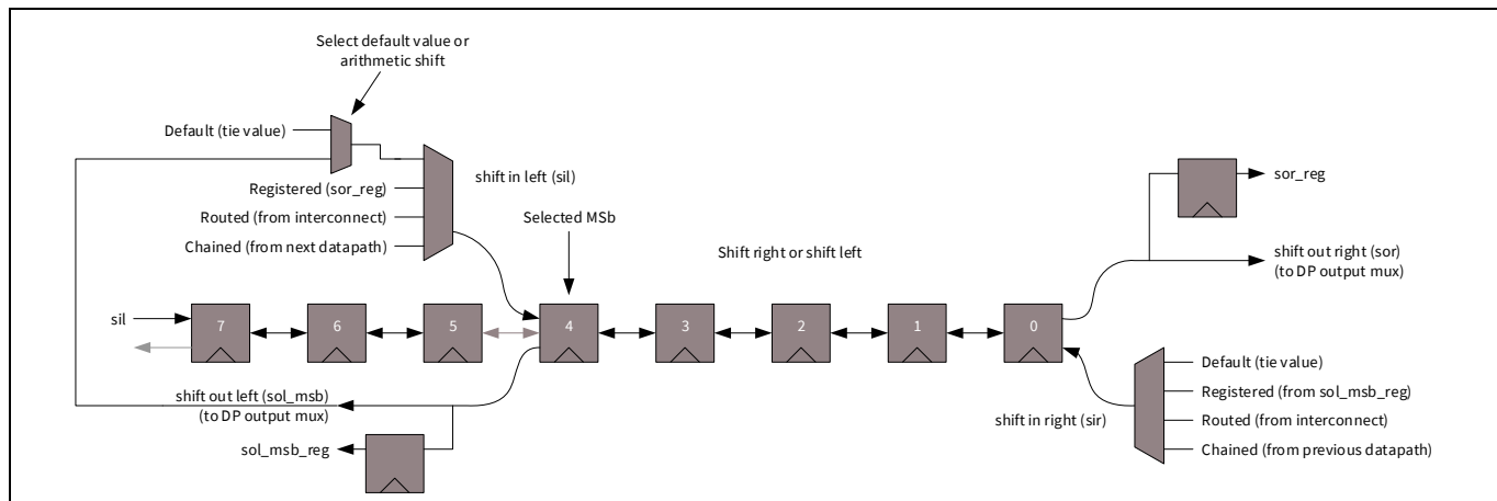
Figure 34-16. Shift operation
