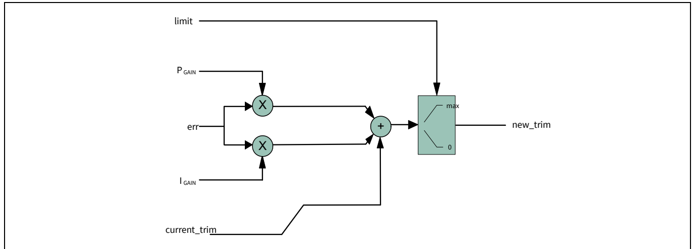
Figure 20-3. FLL error correction diagram
