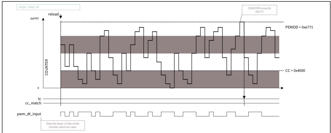
Figure 28-42. PWM_PR output
