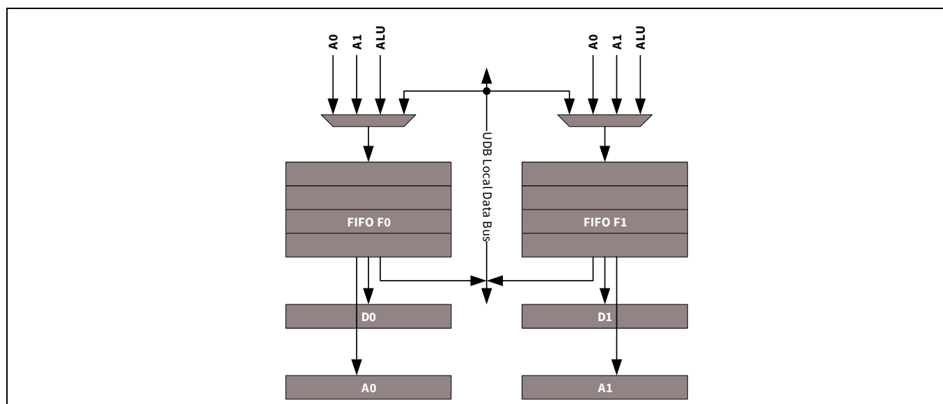
Figure 34-8. FIFO sources and sinks
