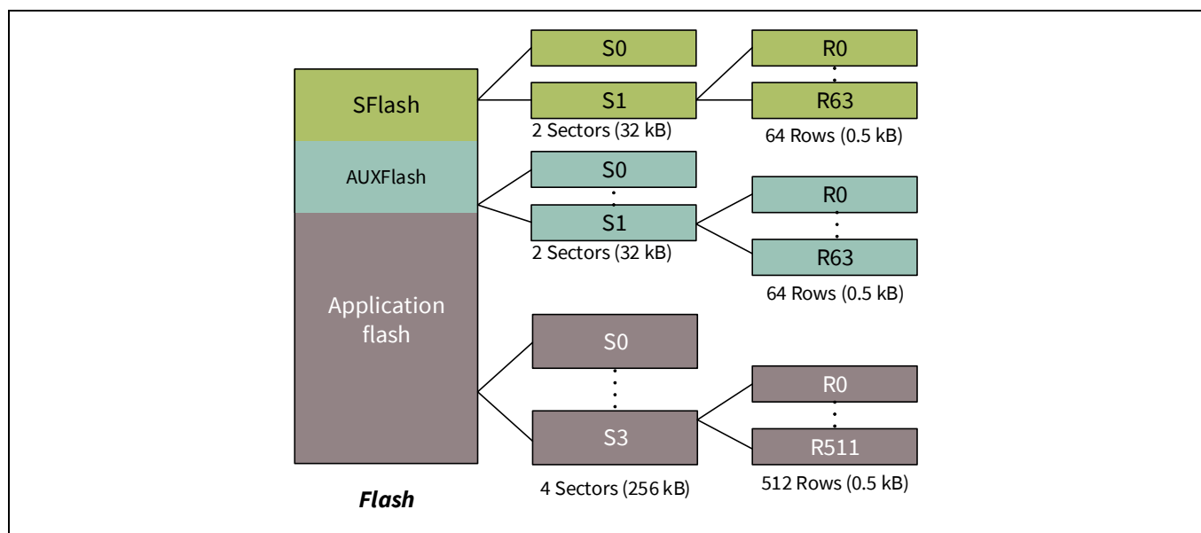
Figure 13-2. Flash geometry organization
