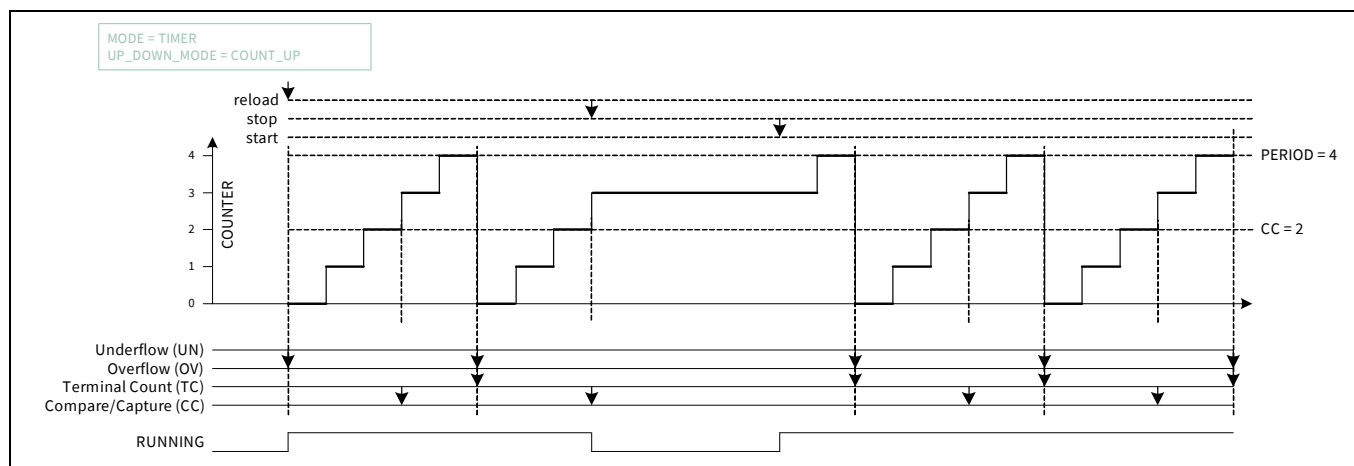
Figure 28-10. Counter start/stopped/continued
