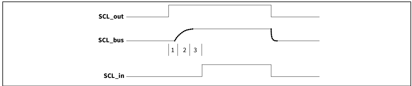
Figure 26-43. I²C SCL turnaround path
