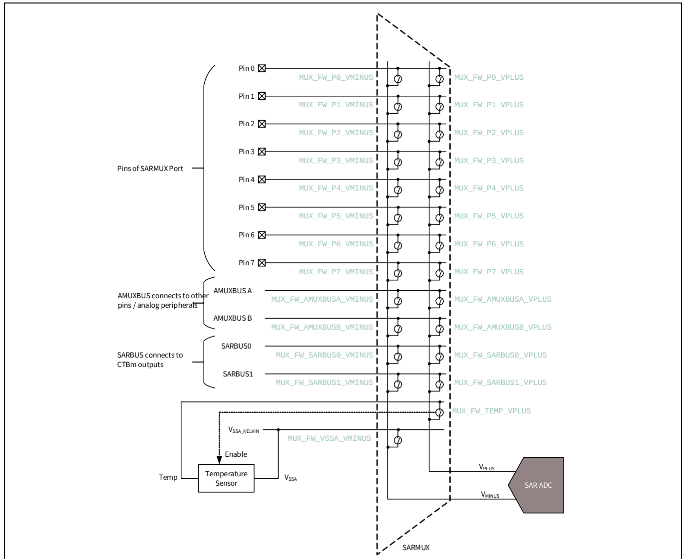
Figure 39-5. SARMUX switches
