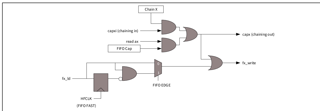
Figure 34-12. Software capture configuration
