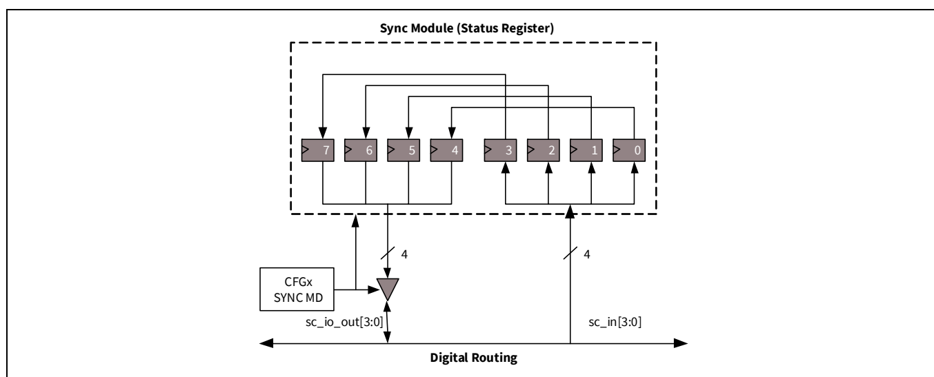
Figure 34-38. Sync mode
