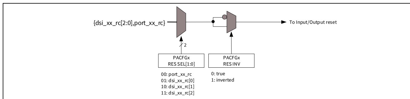
Figure 34-54. PA reset multiplexer detail
