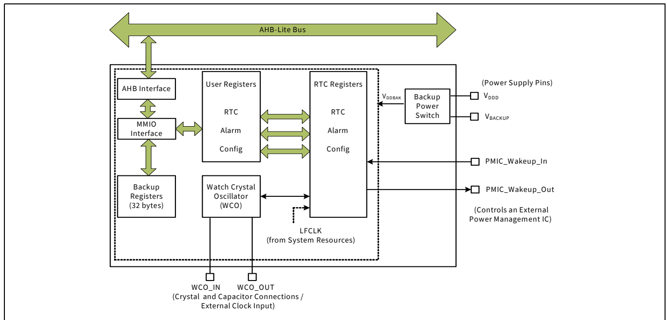
Figure 19-1. Block diagram
