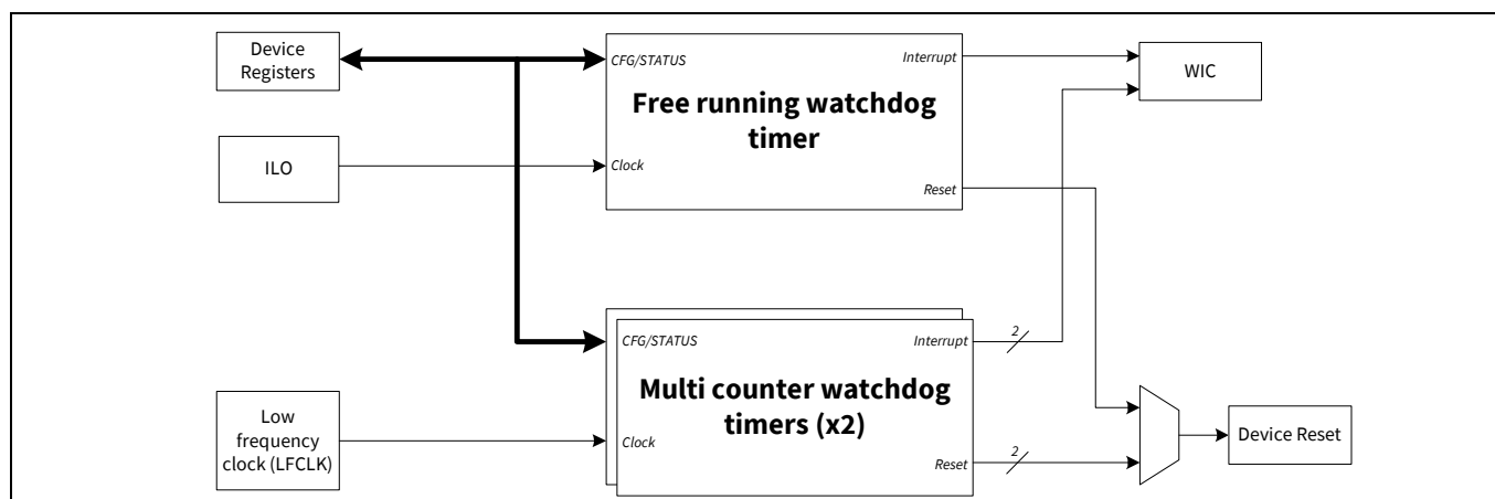
Figure 23-1. Watchdog timer block diagram
