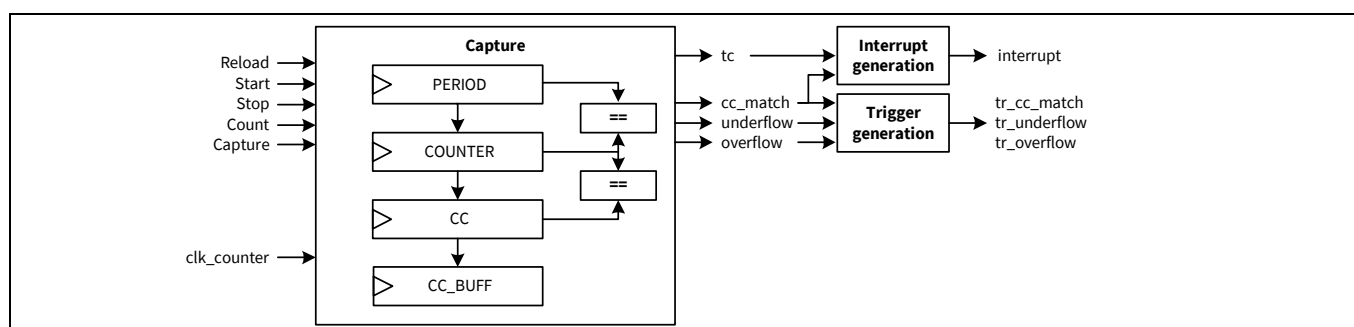
Figure 28-16. Capture functionality
