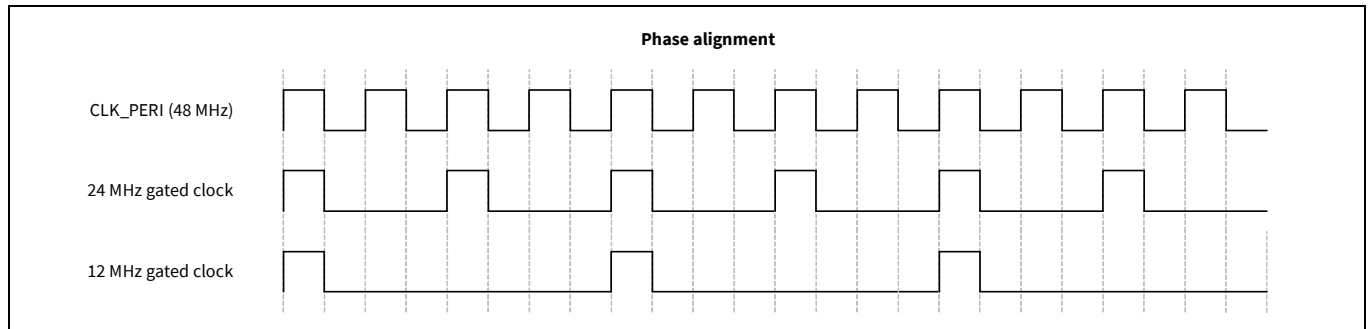
Figure 20-6. Phase-aligned clock dividers
