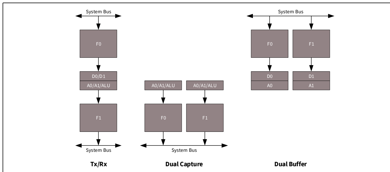
Figure 34-7. FIFO configurations
