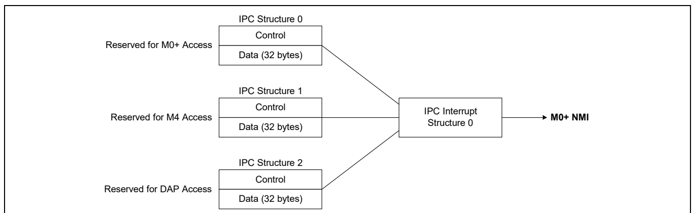
Figure 13-3. System call interface using IPC
