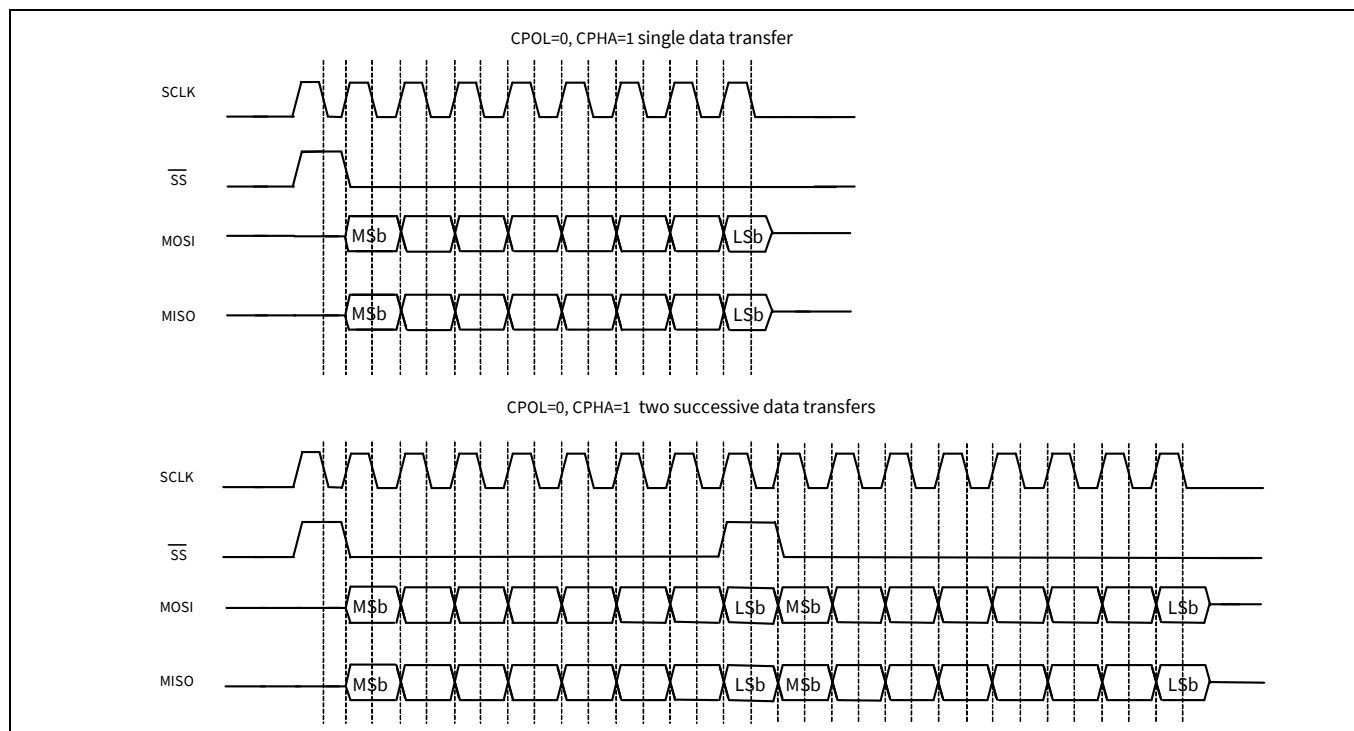
Figure 26-5. SPI TI data transfer example
