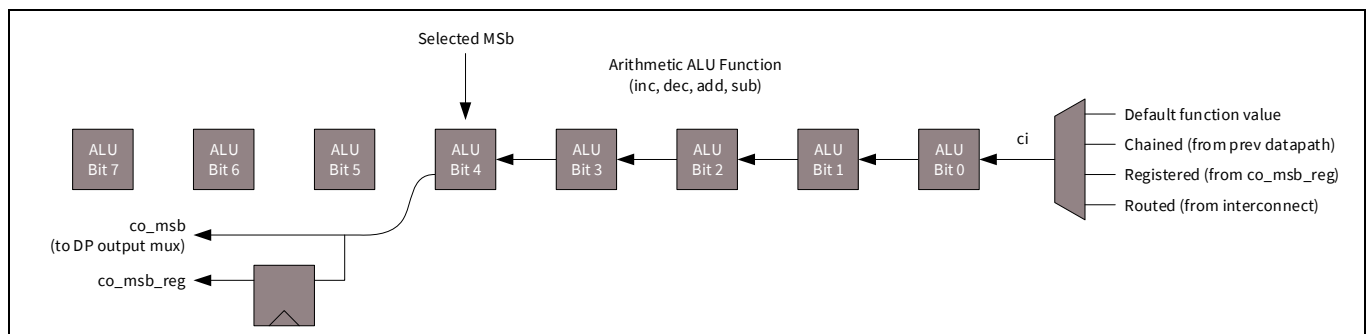
Figure 34-15. Carry operation
