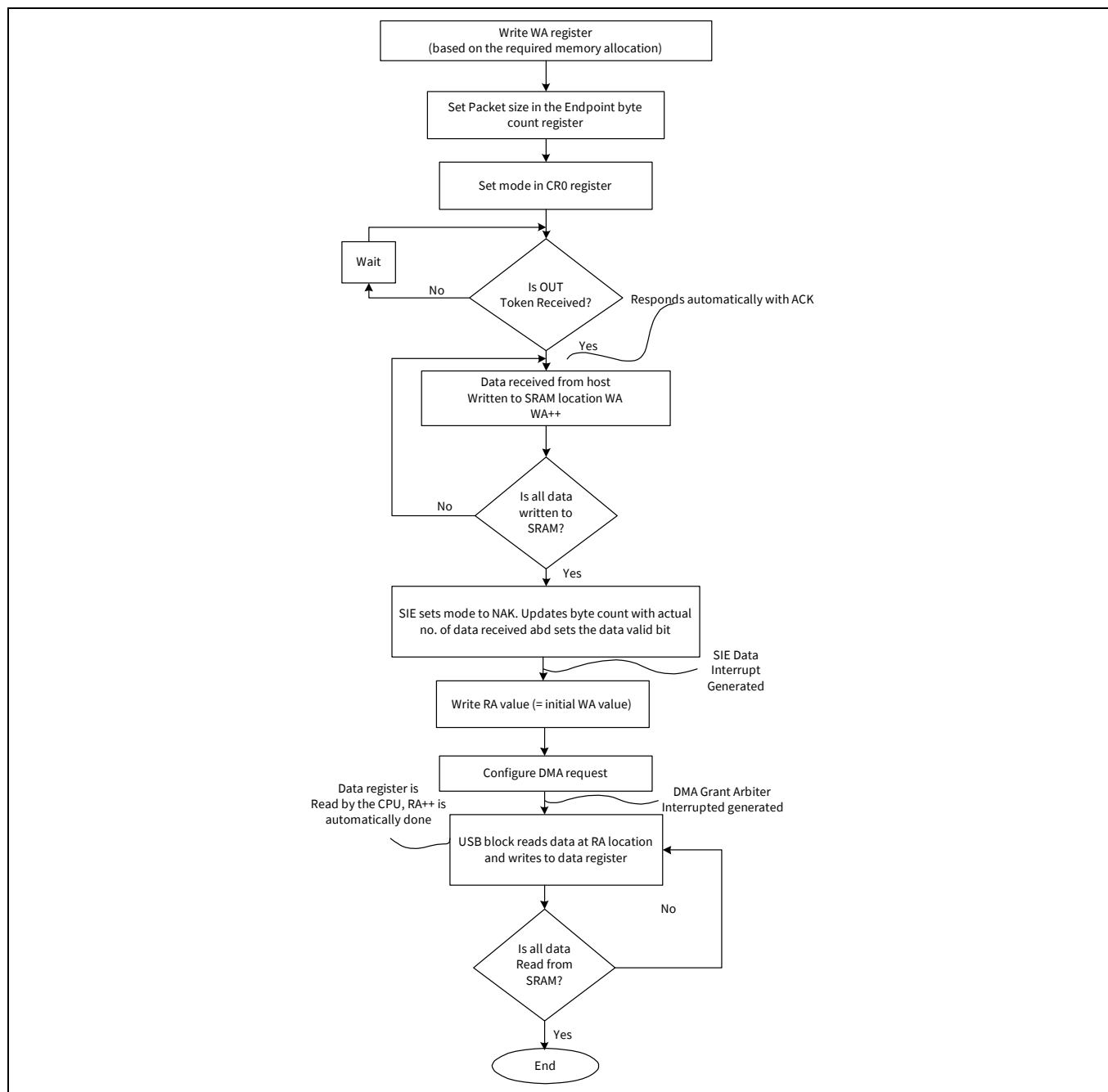
Figure 31-6. Manual DMA OUT transaction
