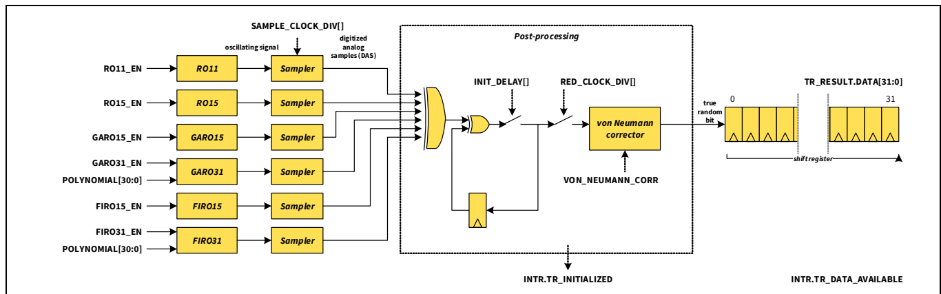
Figure 11-10. TRNG overview
