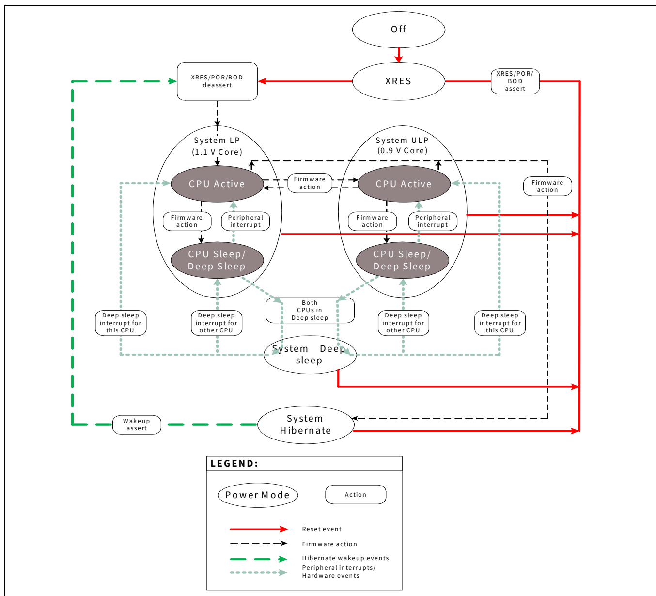
Figure 18-1. Power mode transitions in PSoC™ 6 MCU
