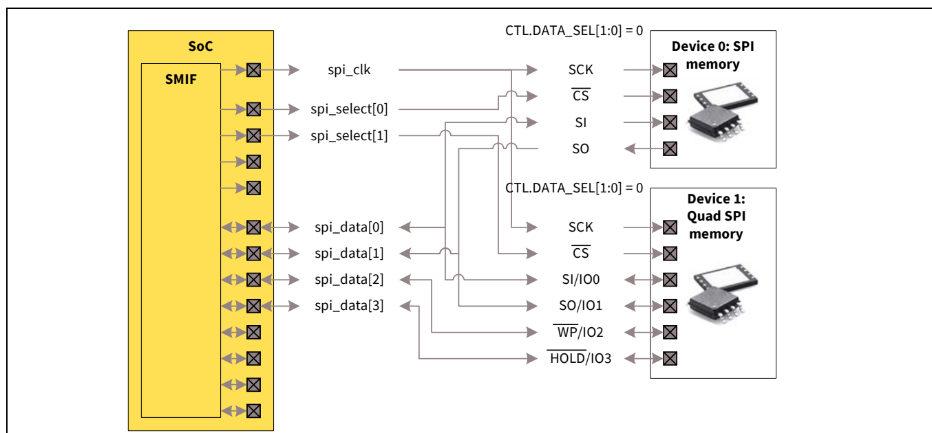
Figure 27-10. Single SPI memory device 0 and Quad SPI memory device 1 - Shared data signal
