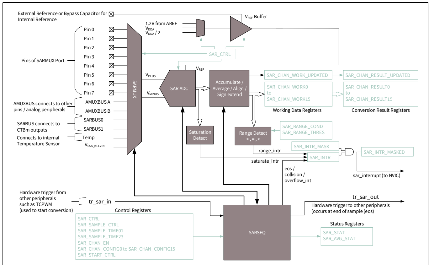
Figure 39-1. Block diagram
