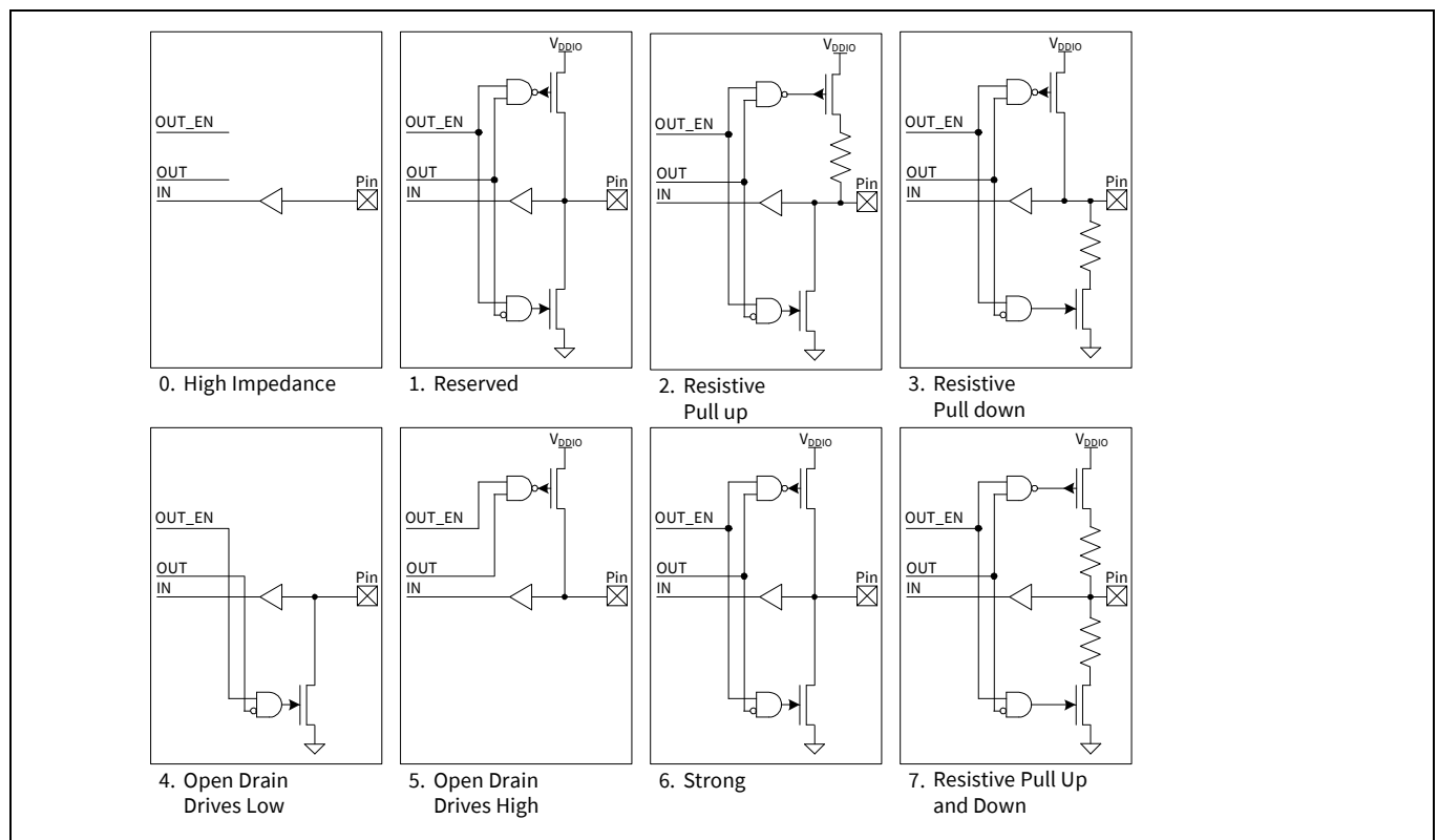
Figure 22-3. CPU and DSI/UDB I/O drive mode block diagram
