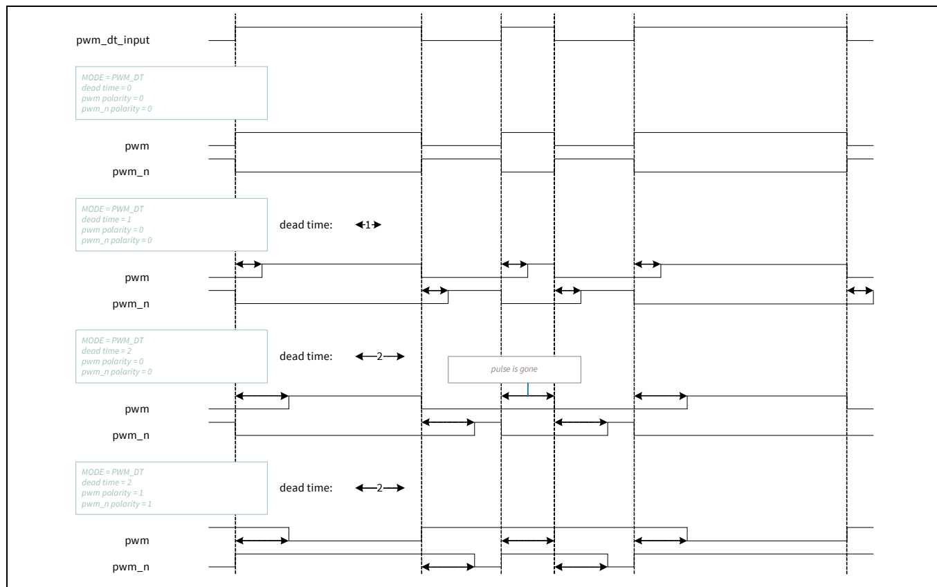
Figure 28-39. Dead-time timing
