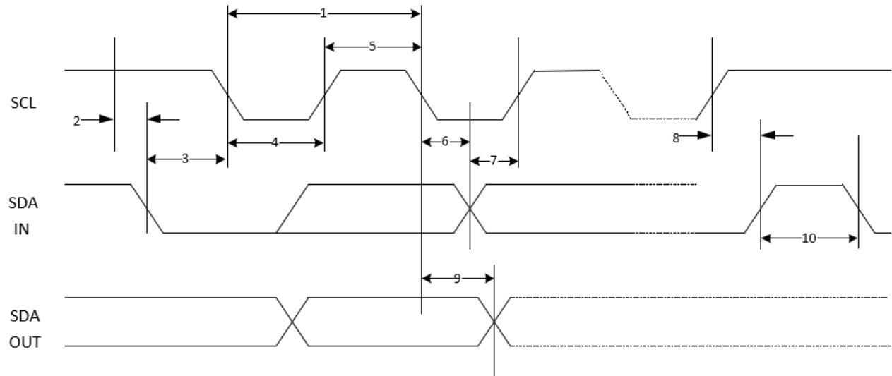
Figure 16. I 2 C Interface Timing Diagram
