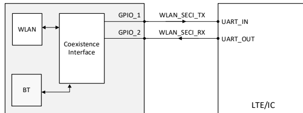
Figure 27. 2-Wire Coexistence Interface to an External IC
