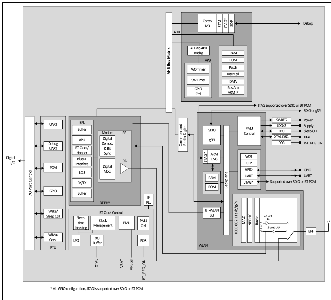
Figure 2. CYW43438 Block Diagram
