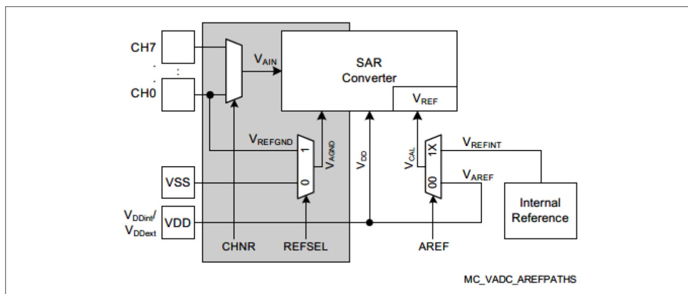
Figure 11 ADC Voltage Supply
