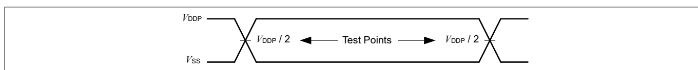
Figure 17 Testing Waveform, Output Delay
