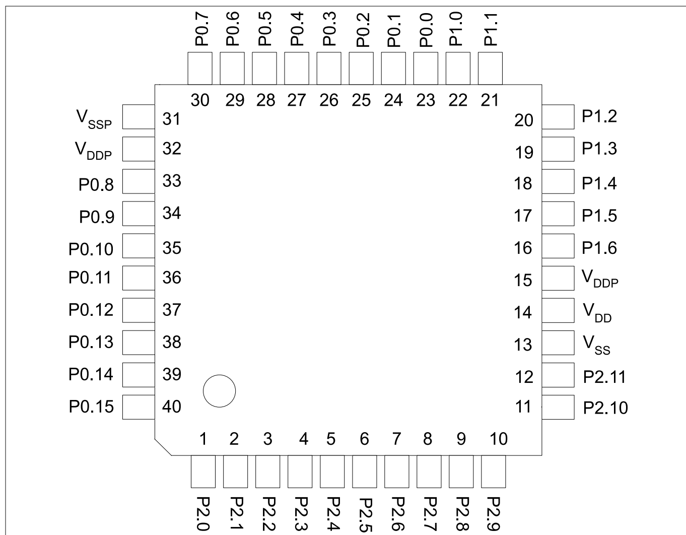
Figure 8 XMC1200 PG-VQFN-40 Pin Configuration (top view)
