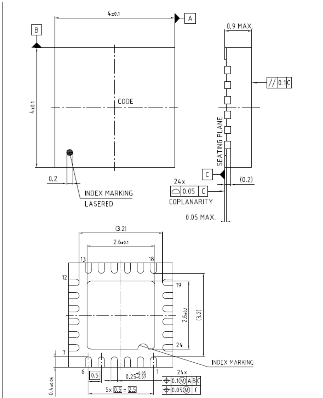
Figure 29 PG-VQFN-24-19
