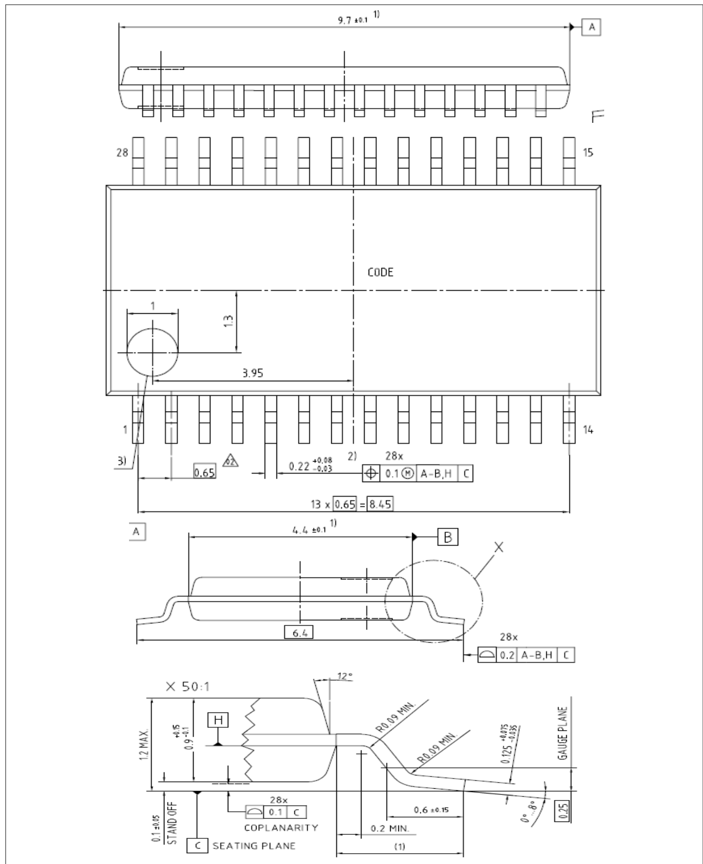
Figure 27 PG-TSSOP-28-16
