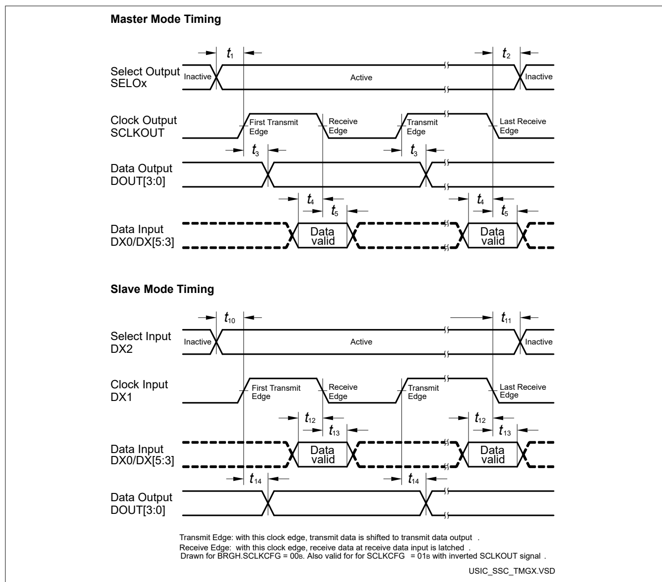
Figure 22 USIC - SSC Master/Slave Mode Timing
