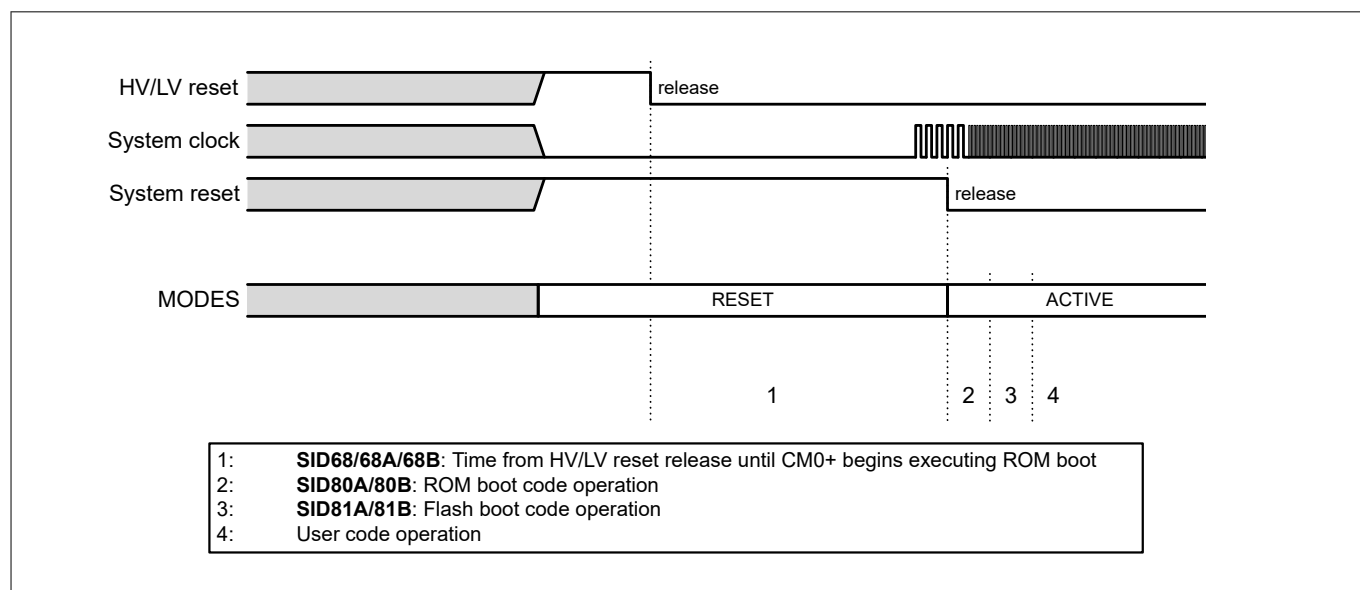
Figure 11 Reset sequence
