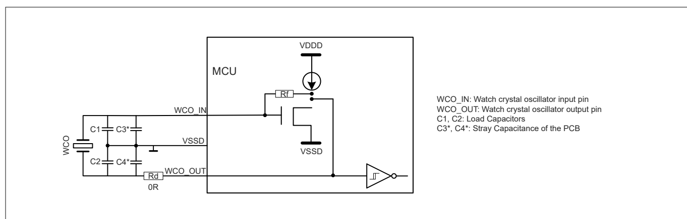
Figure 31 WCO connection scheme
