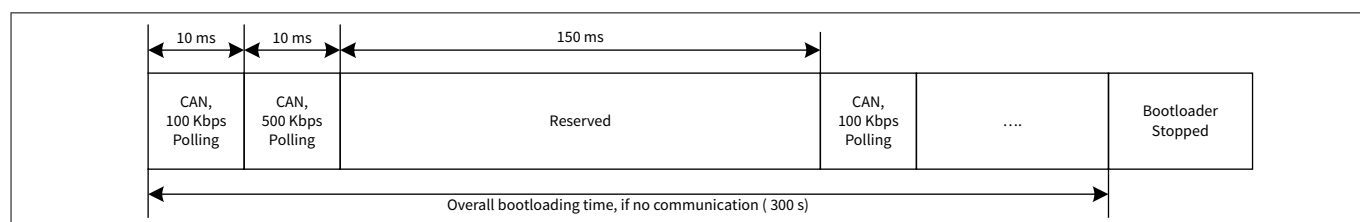
Figure 36 Bootloading sequence
