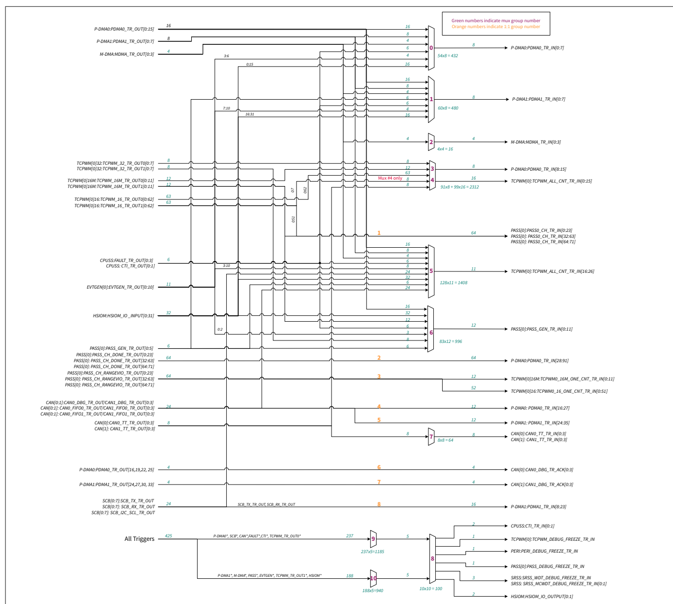
Figure 8 Trigger multiplexer
