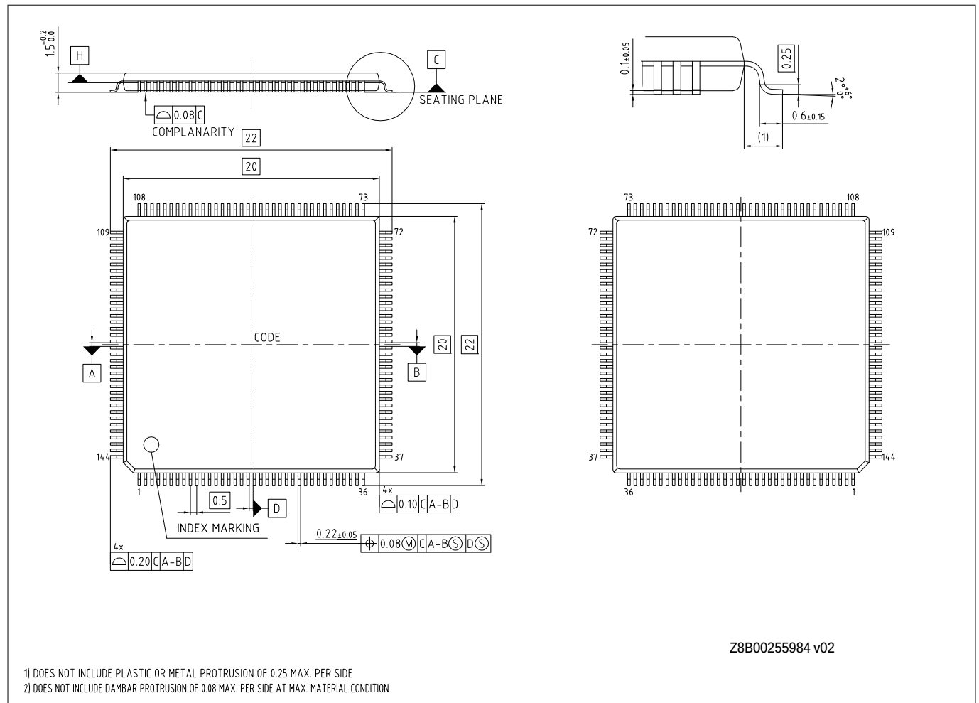
Figure 34 144-pin LQFP (20.0 × 20.0 × 1.7 mm) LQS144 (PG-LQFP-144)
