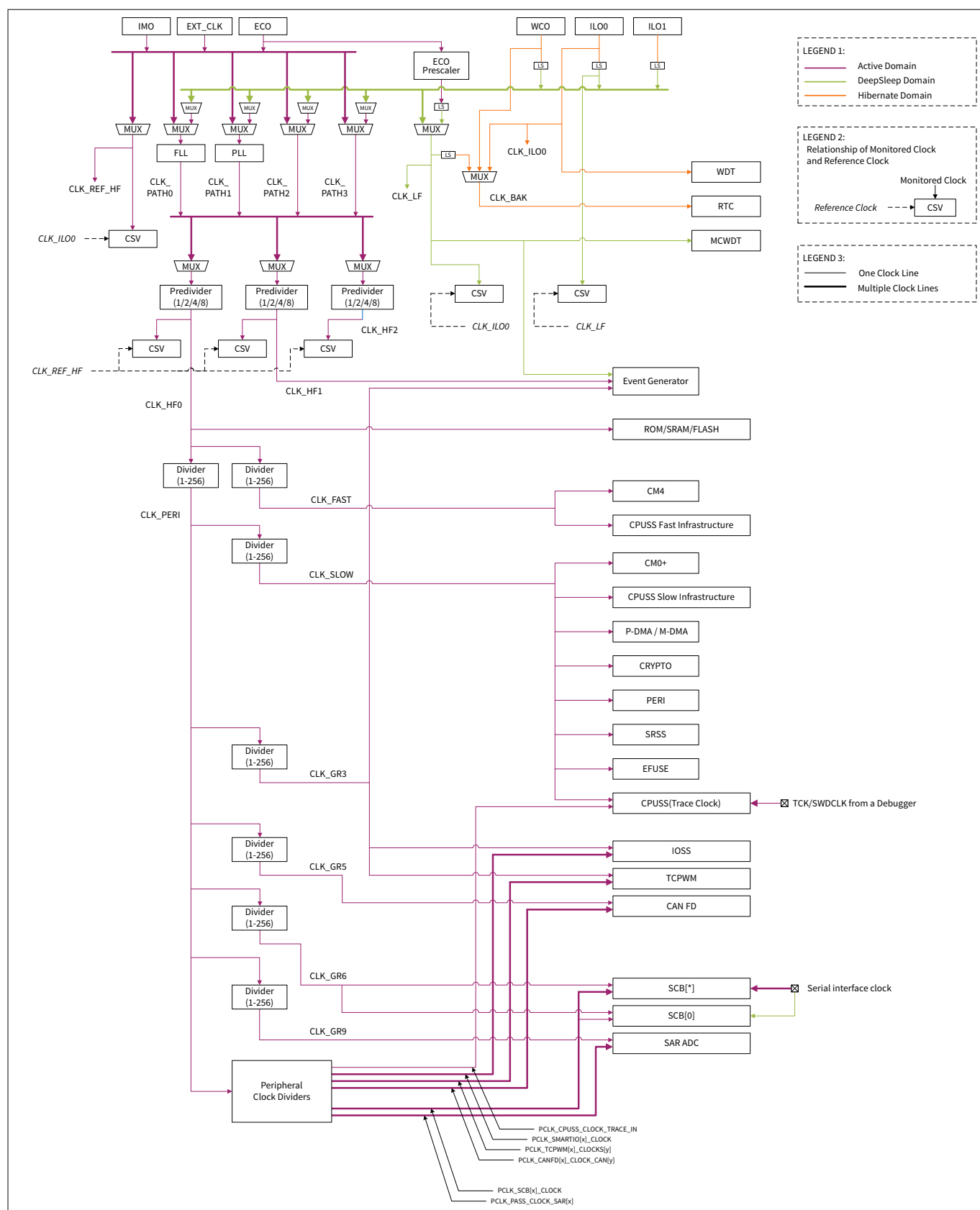
Figure 3 XMC5300 clock diagram
