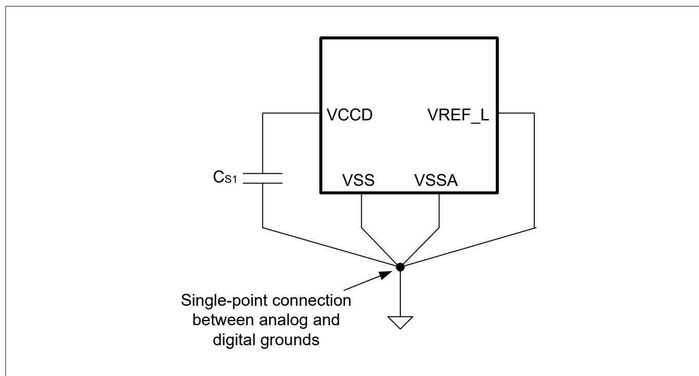
Figure 10 Smoothing capacitor
