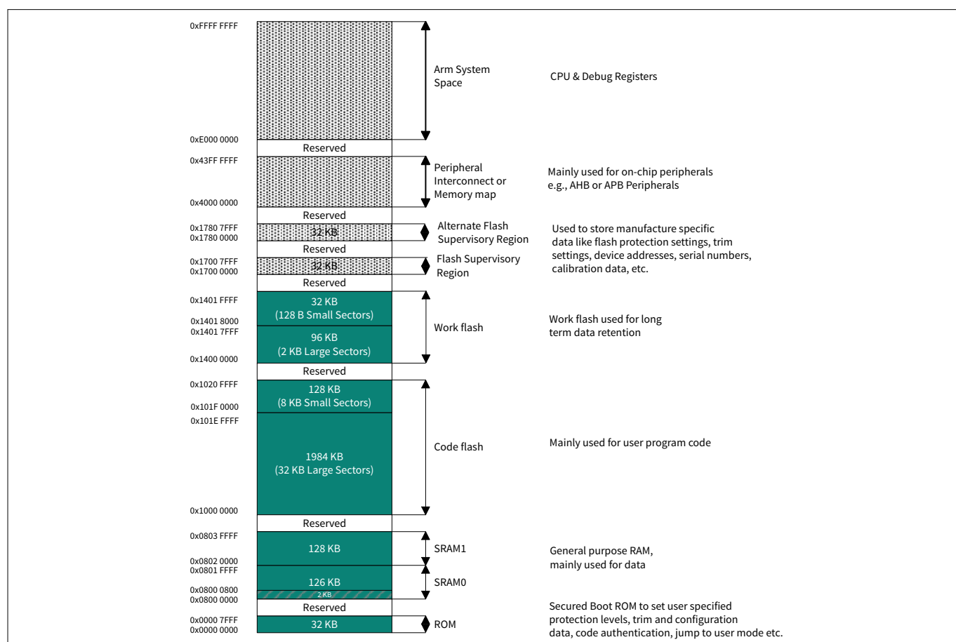
Figure 2 XMC5300 address map
