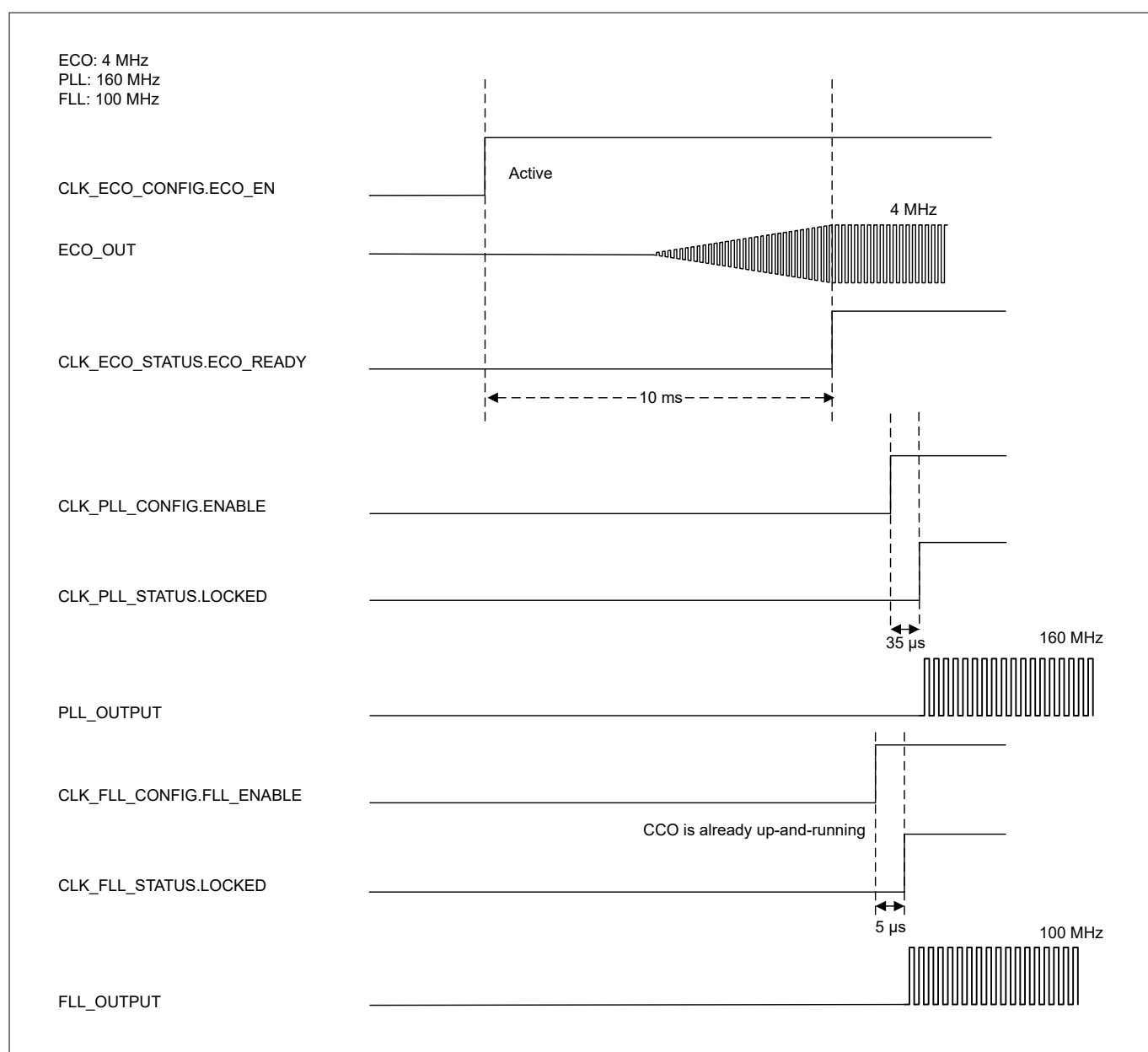
Figure 32 ECO to PLL or FLL diagram
