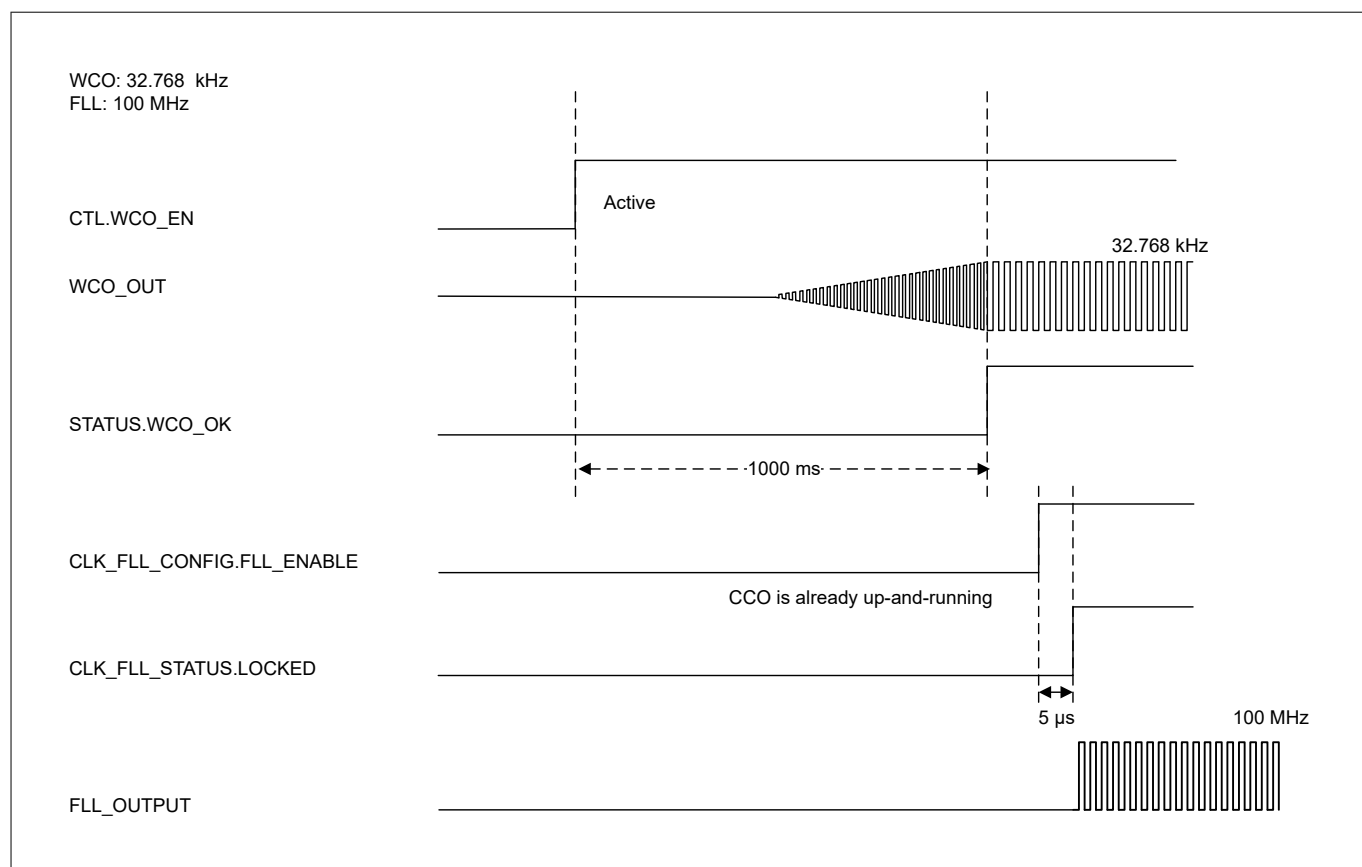
Figure 33 WCO to FLL diagram
