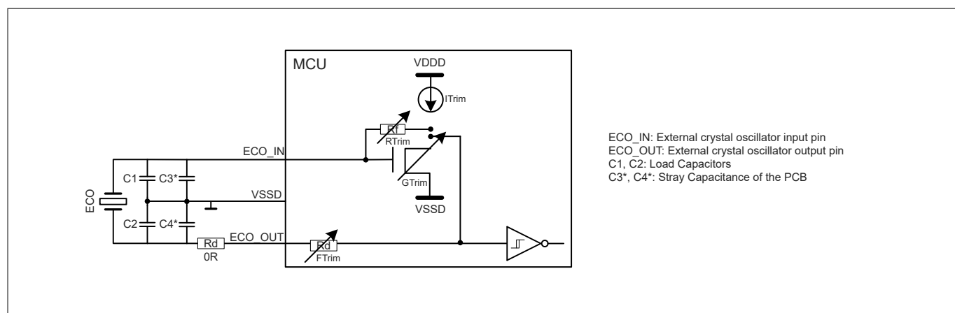
Figure 30 ECO connection scheme
