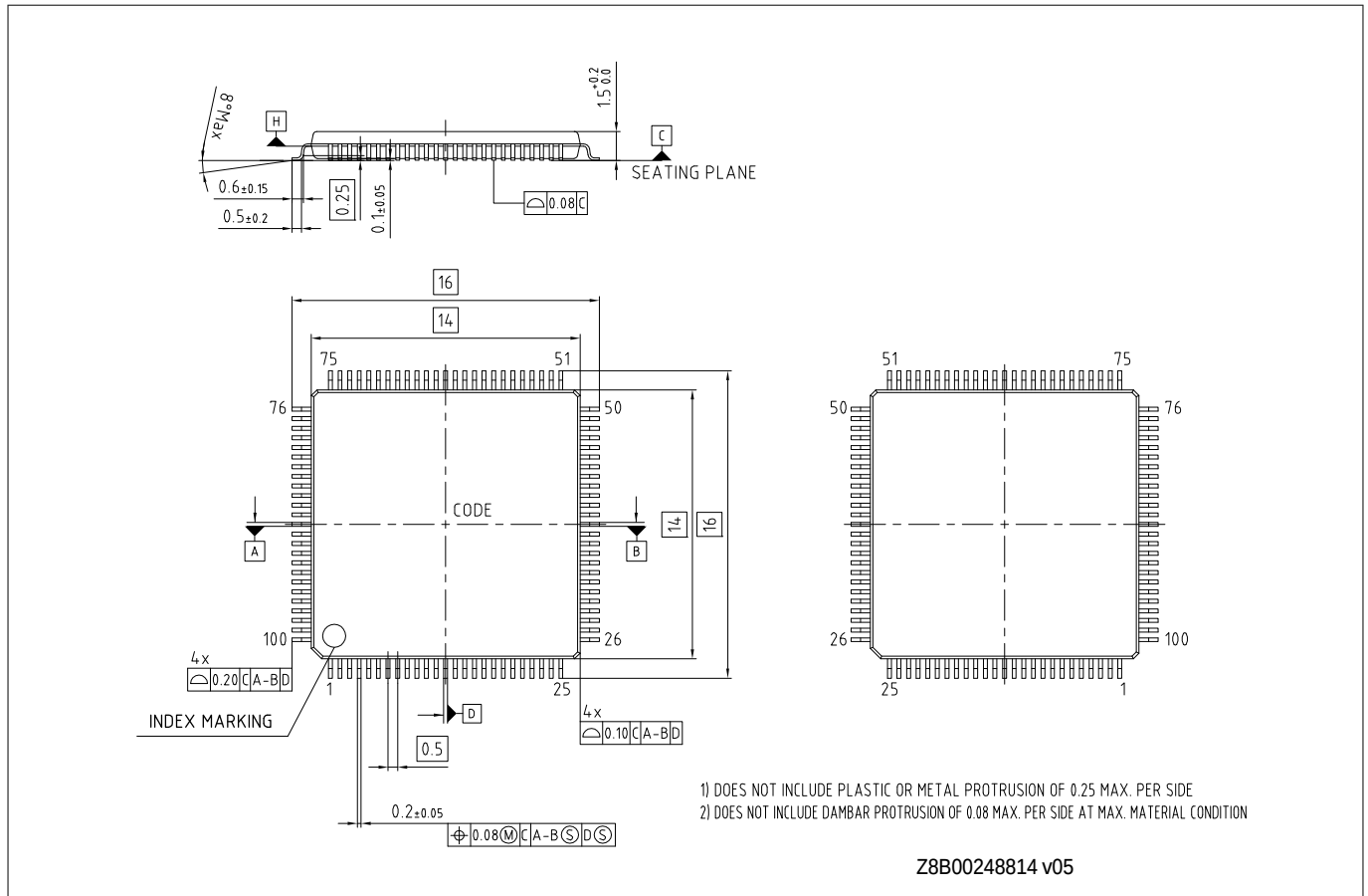
Figure 35 100-pin LQFP (14.0 × 14.0 × 1.7 mm) LQI100 (PG-LQFP-100)
