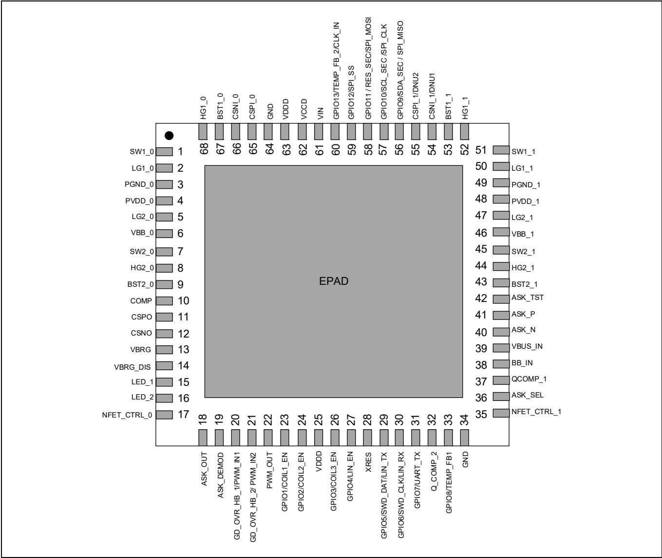
Figure 3 WLC1515-68LDXS pinout
