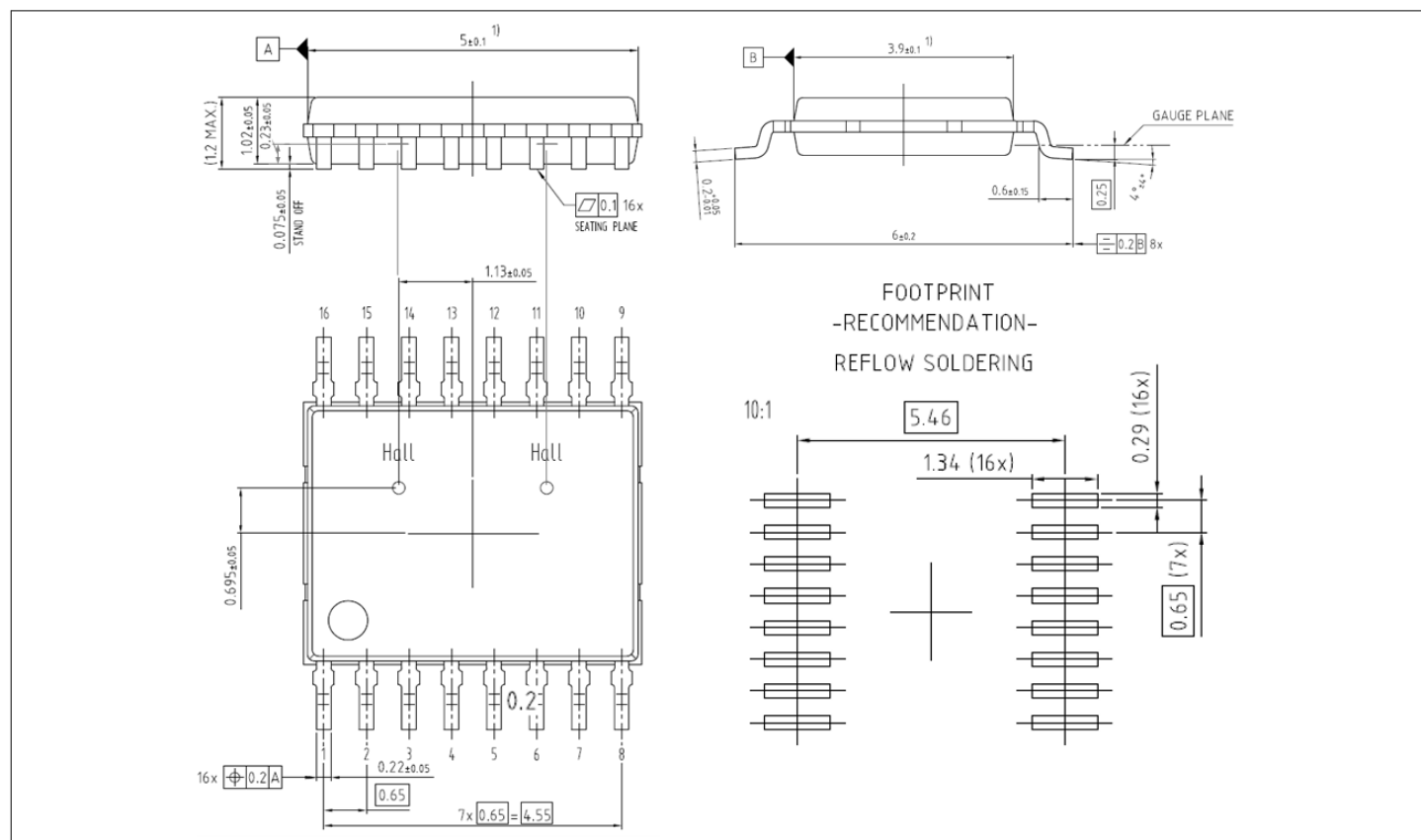
Figure 14 PG-TDSO-16 package outline. Sensing elements position not in scale
