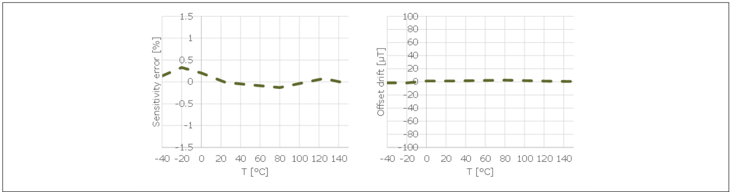
Figure 5 PG-VSON-6, semi-differential bidirectional, sensitivity S1
