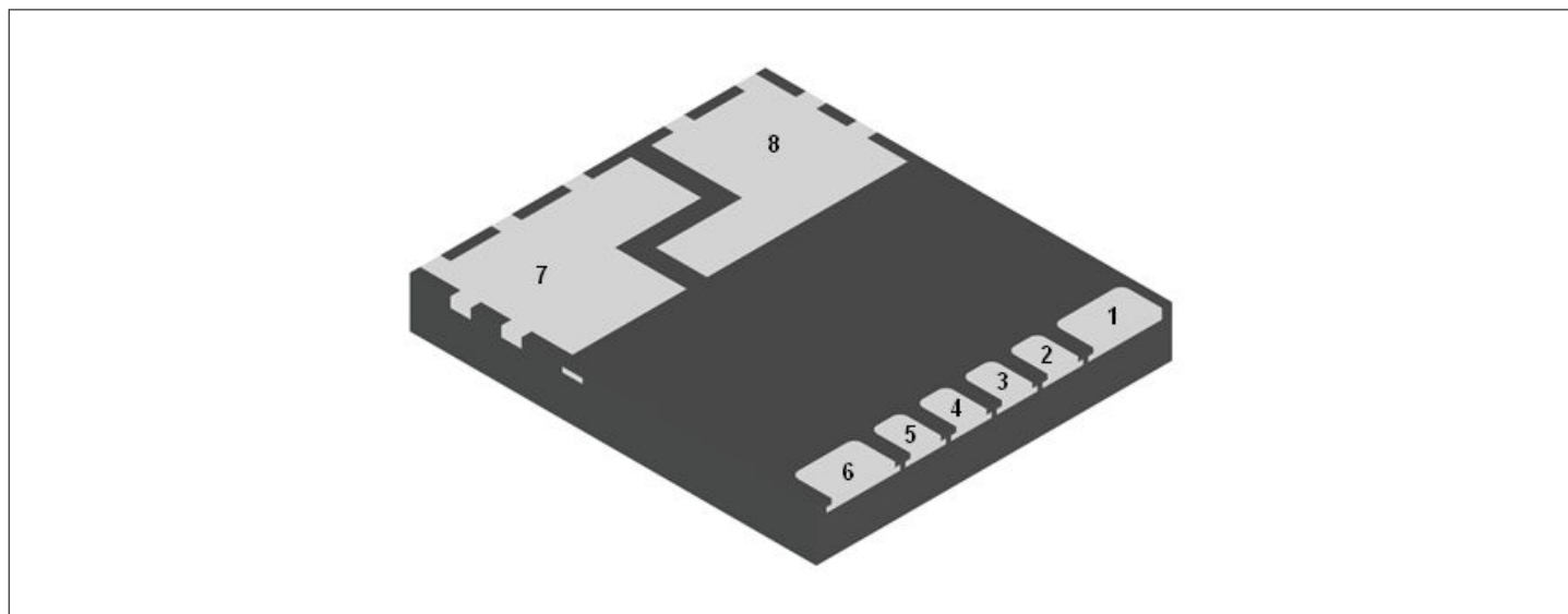
Figure 2 Pin configuration
