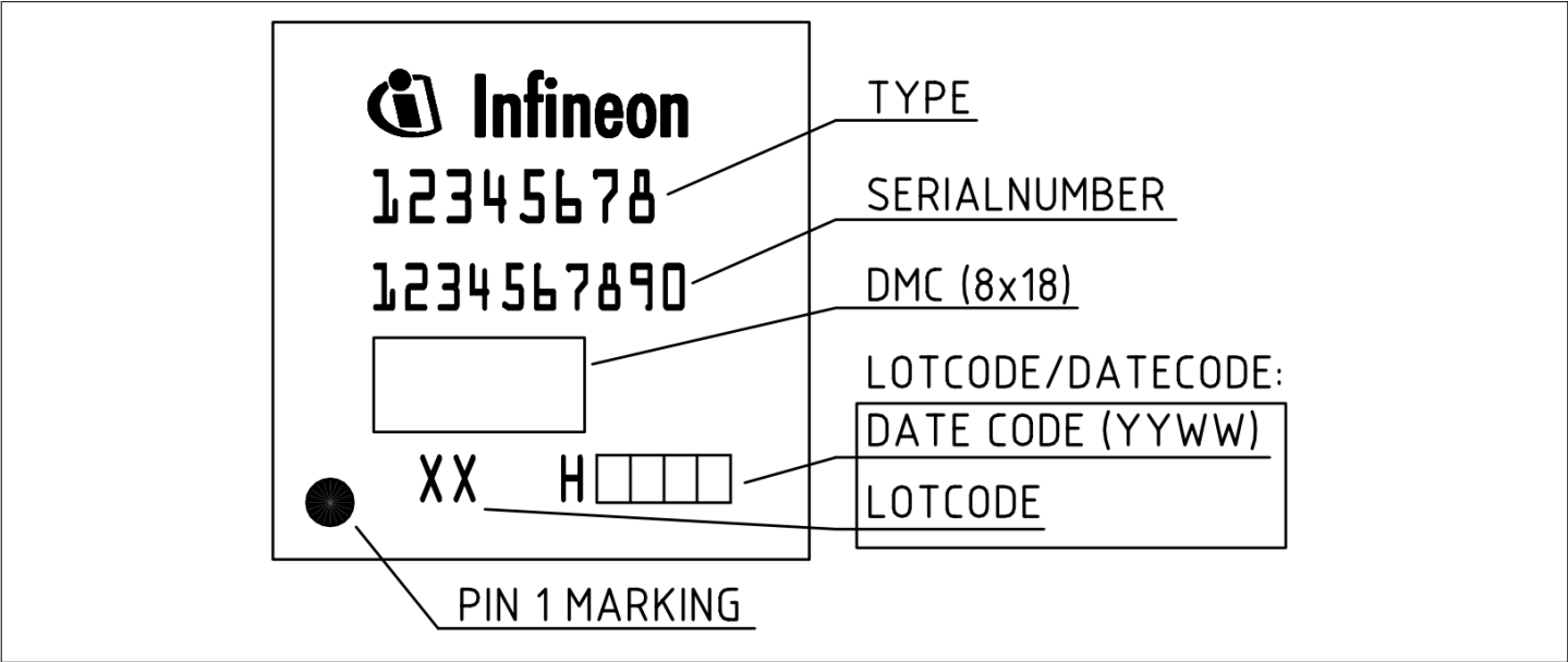
Figure 10 Package marking
