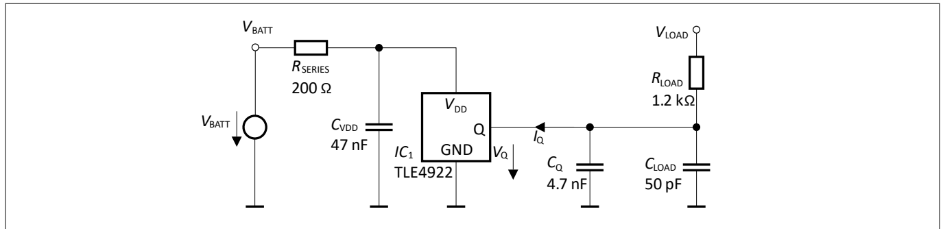
Figure 1 Application circuit TLE4922
