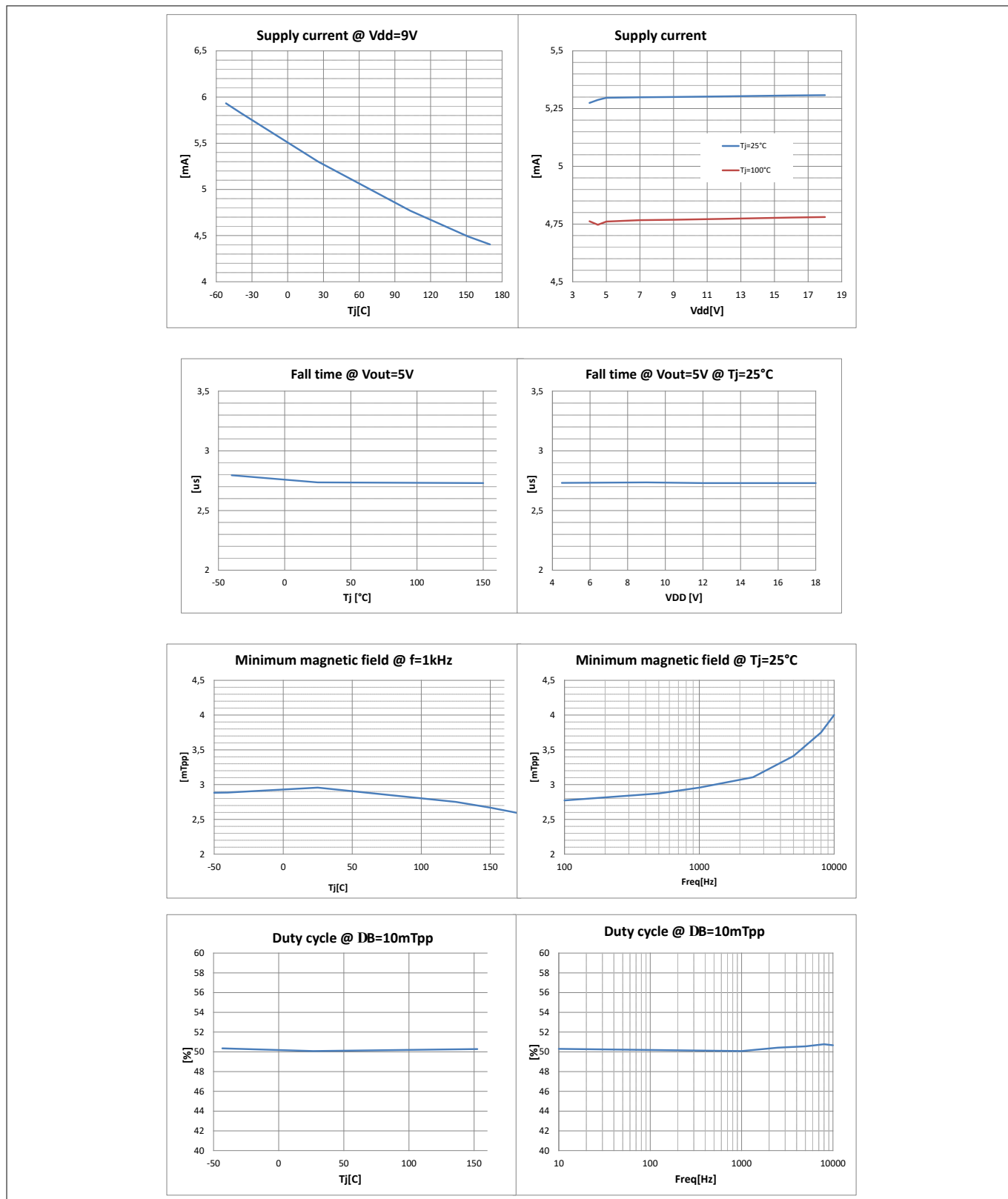
Figure 6 Typical Performance
