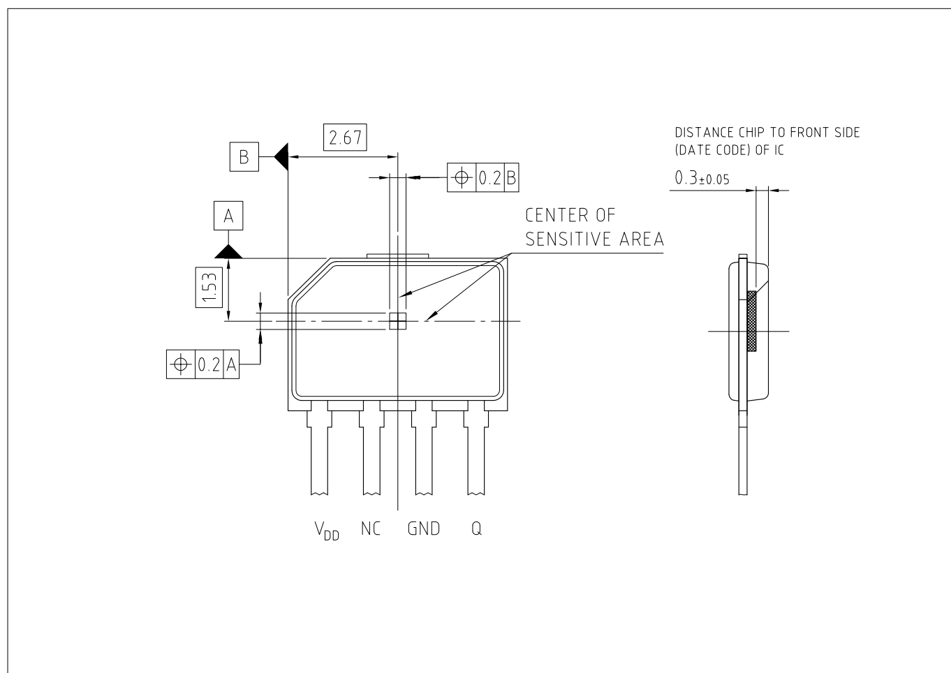
Figure 8 Pinning, Sensitive Area
