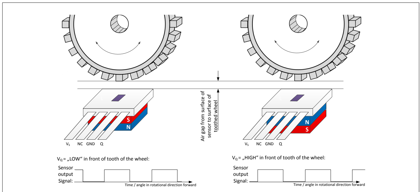
Figure 7 Changing polarity of back bias magnet will change the polarity of TLE4922 output
