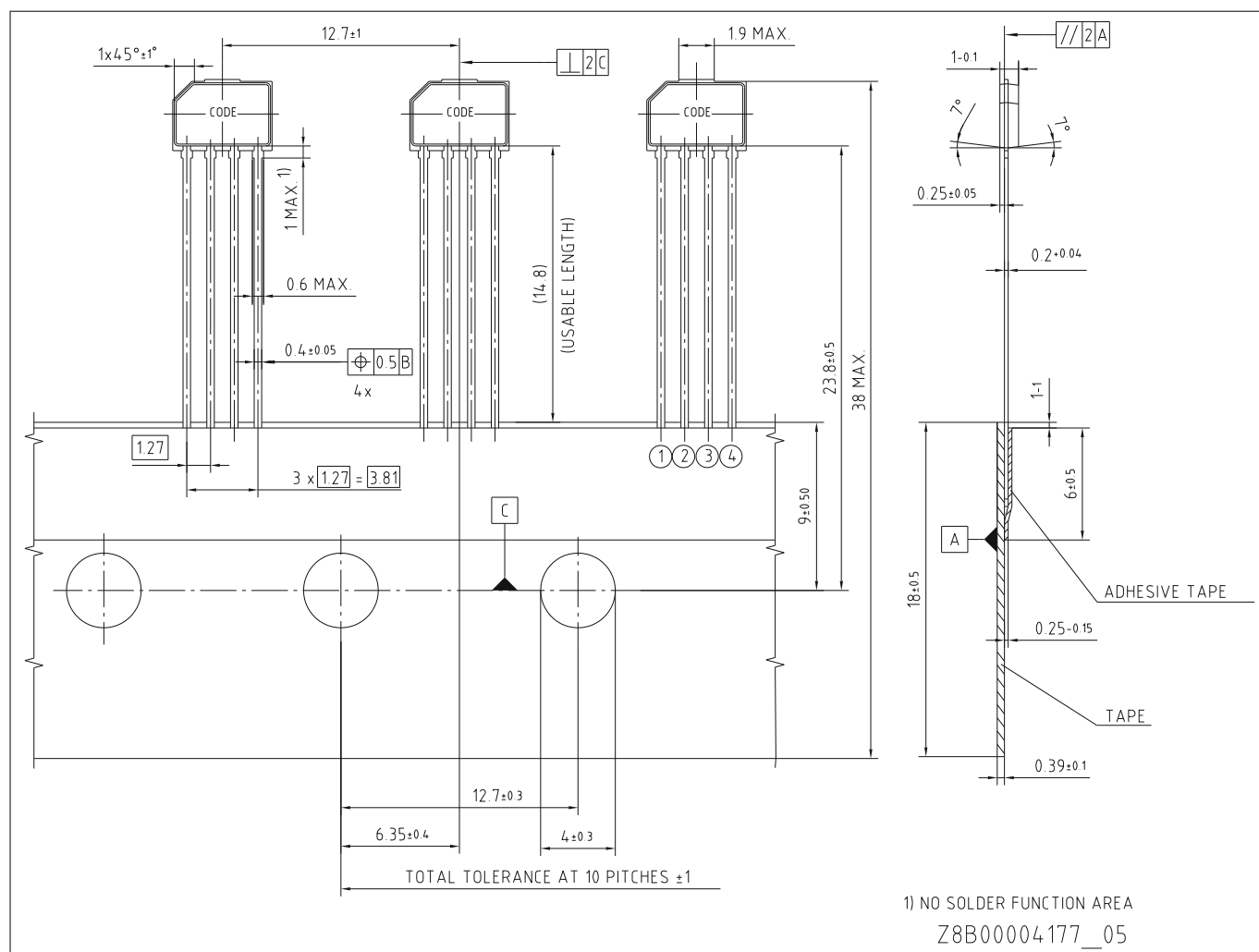
Figure 11 PG-SSO-4-1 packaging, dimensions in mm
