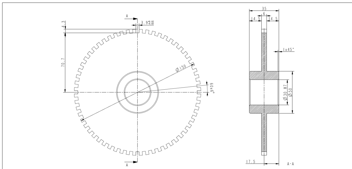
Figure 5 Infineon reference toothed wheel: dimension in mm
