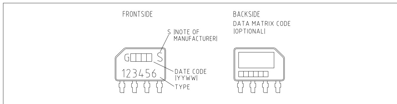
Figure 9 Marking pattern
