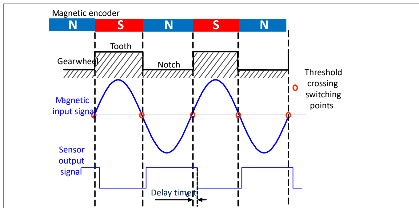
Figure 2 Phase error and delay time definition
