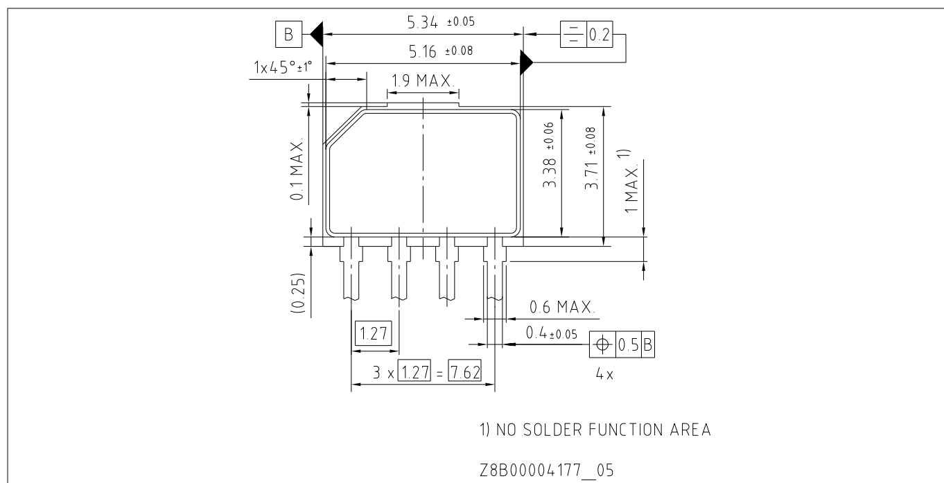
Figure 10 PG-SSO-4-1 package dimensions, dimensions in mm
