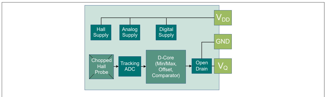
Figure 4 Block Diagram TLE4922
