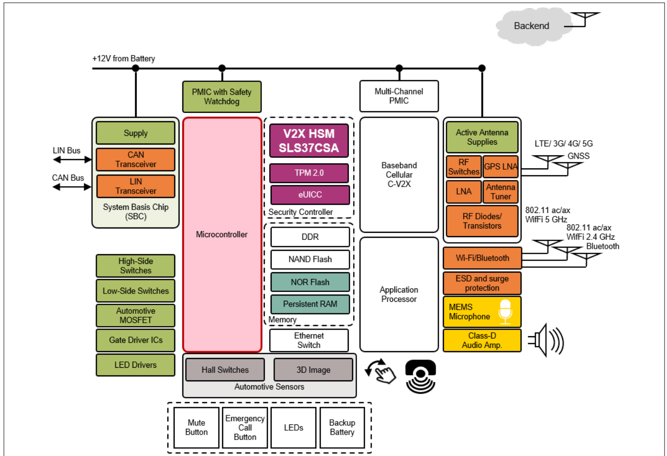
Figure 2 Exemplary Telematics Control Unit Architecture
