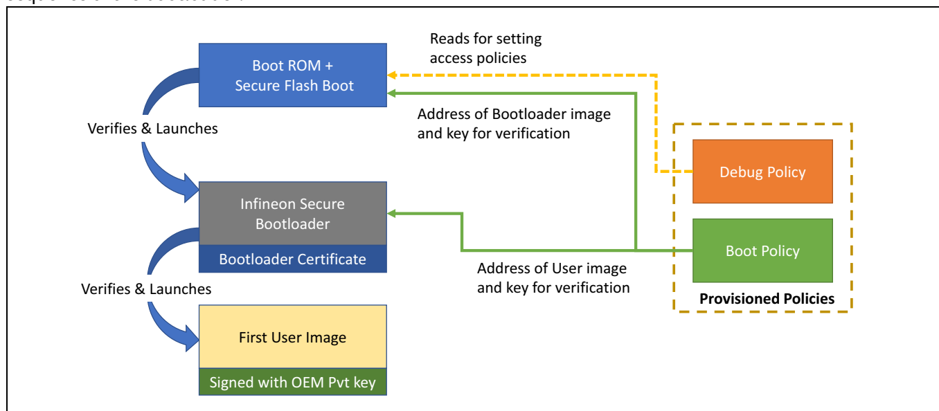
Figure 11 Bootloader Launch Sequence
