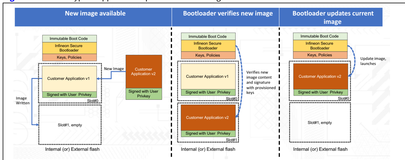
Figure 12 Bootloader Application Update Sequence
