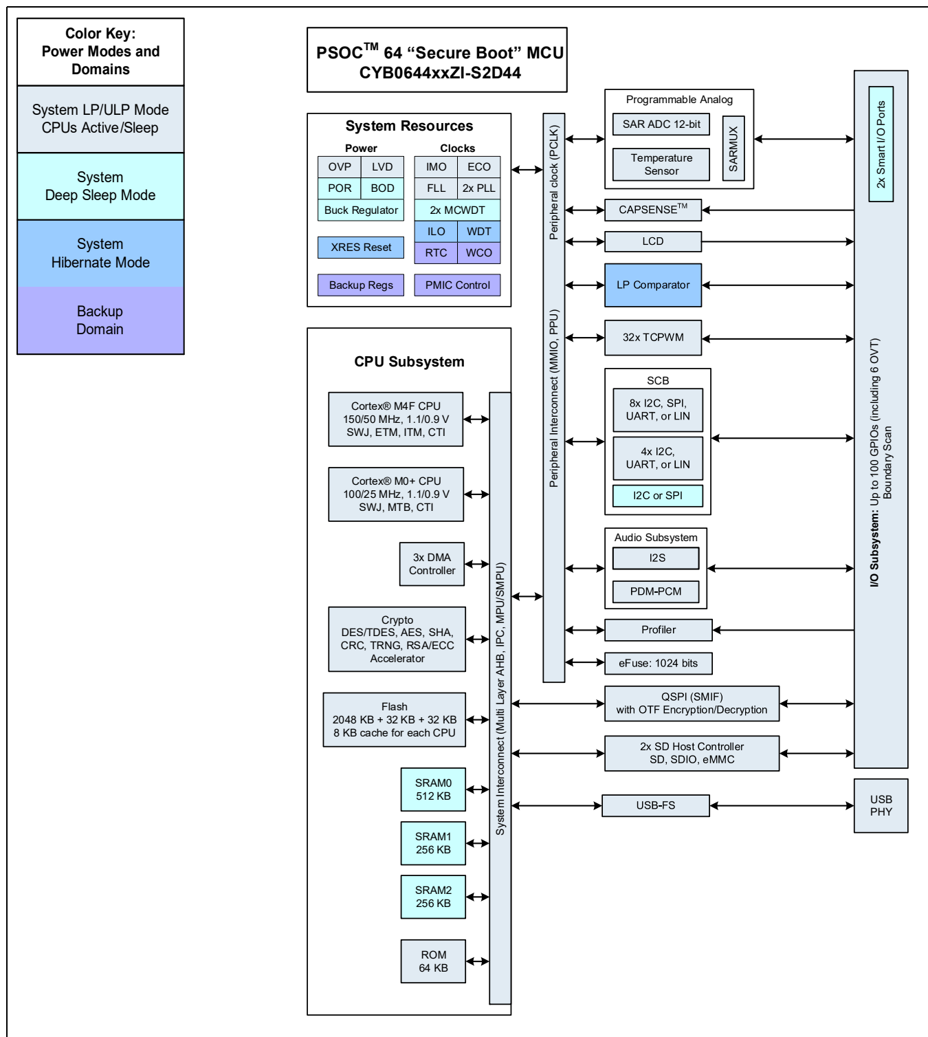
Figure 2 Block diagram
