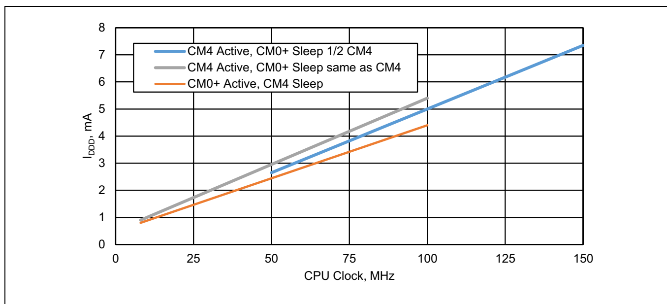
Figure 17 Typical Device Currents vs. CPU Frequency; System Low Power (LP) Mode
