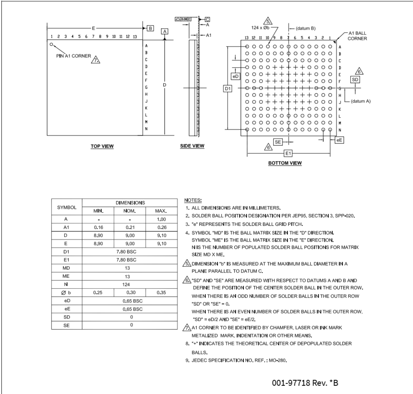
图 18 124-ball VFBGA (9.0 × 9.0 × 1.0 mm) BZ0AA/VZC124/D2A124 封装外形 (PG-VFBGA-124), 001-97718
