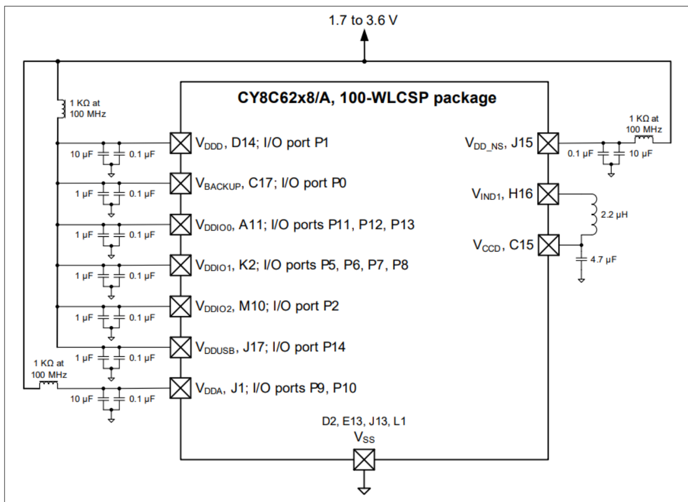
Figure 15 100-WLCSP Power connection diagram
