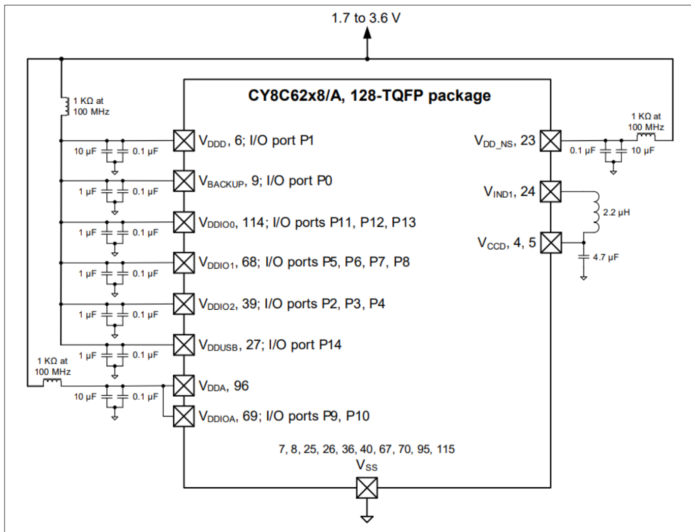
Figure 11 128-TQFP Power connection diagram
