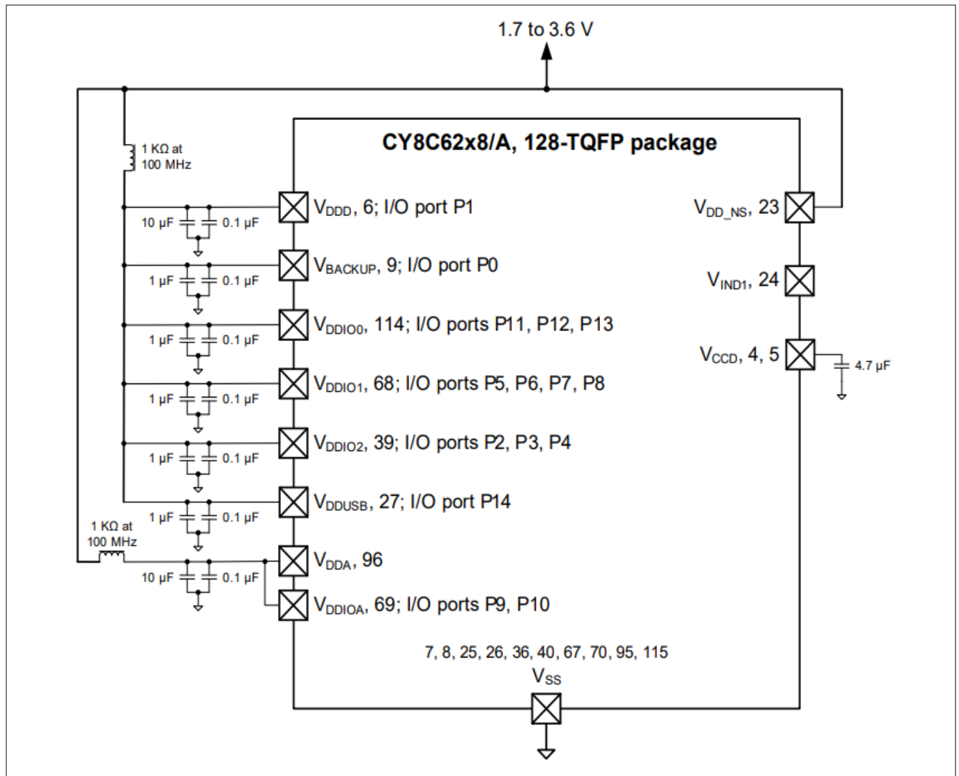
Figure 12 128-TQFP (No Buck) Power connection diagram
