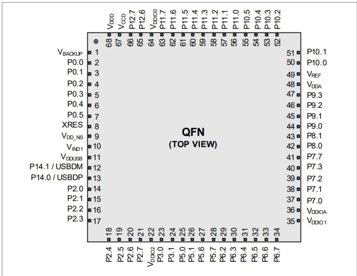
Figure 10 Device pinout for 68-pin QFN package 1)
