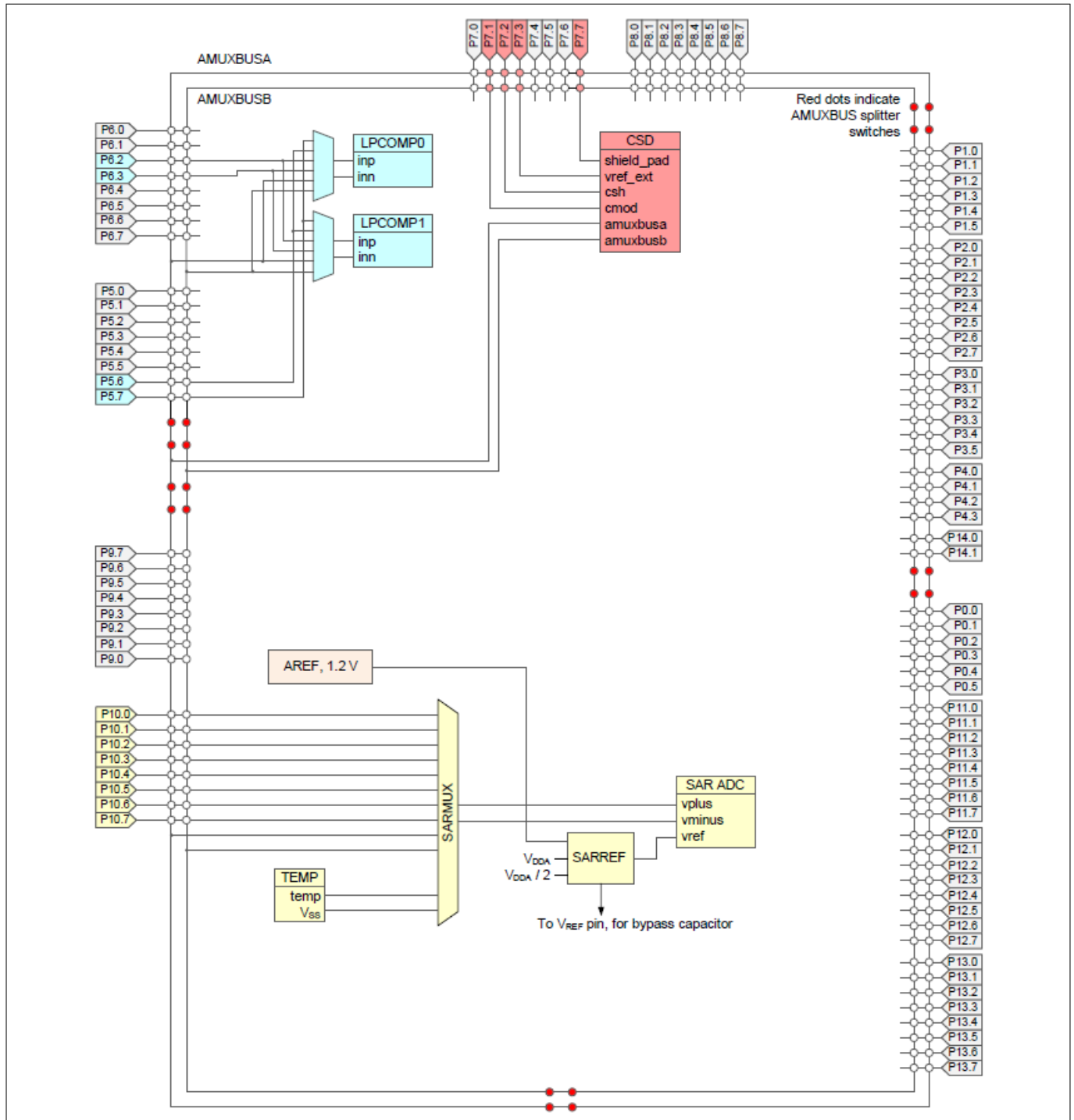
Figure 6 Analog subsystem
