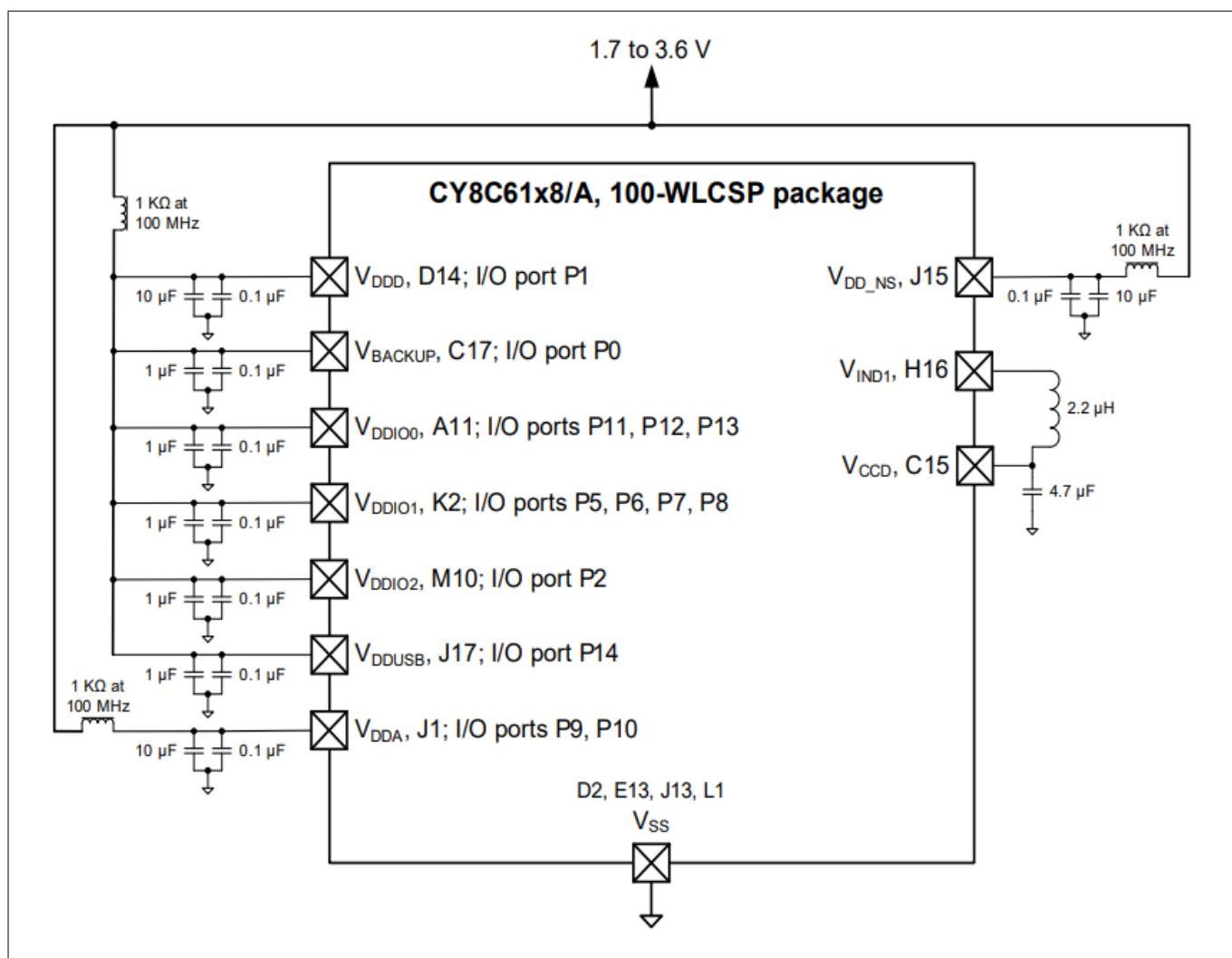
Figure 15 100-WLCSP Power connection diagram
