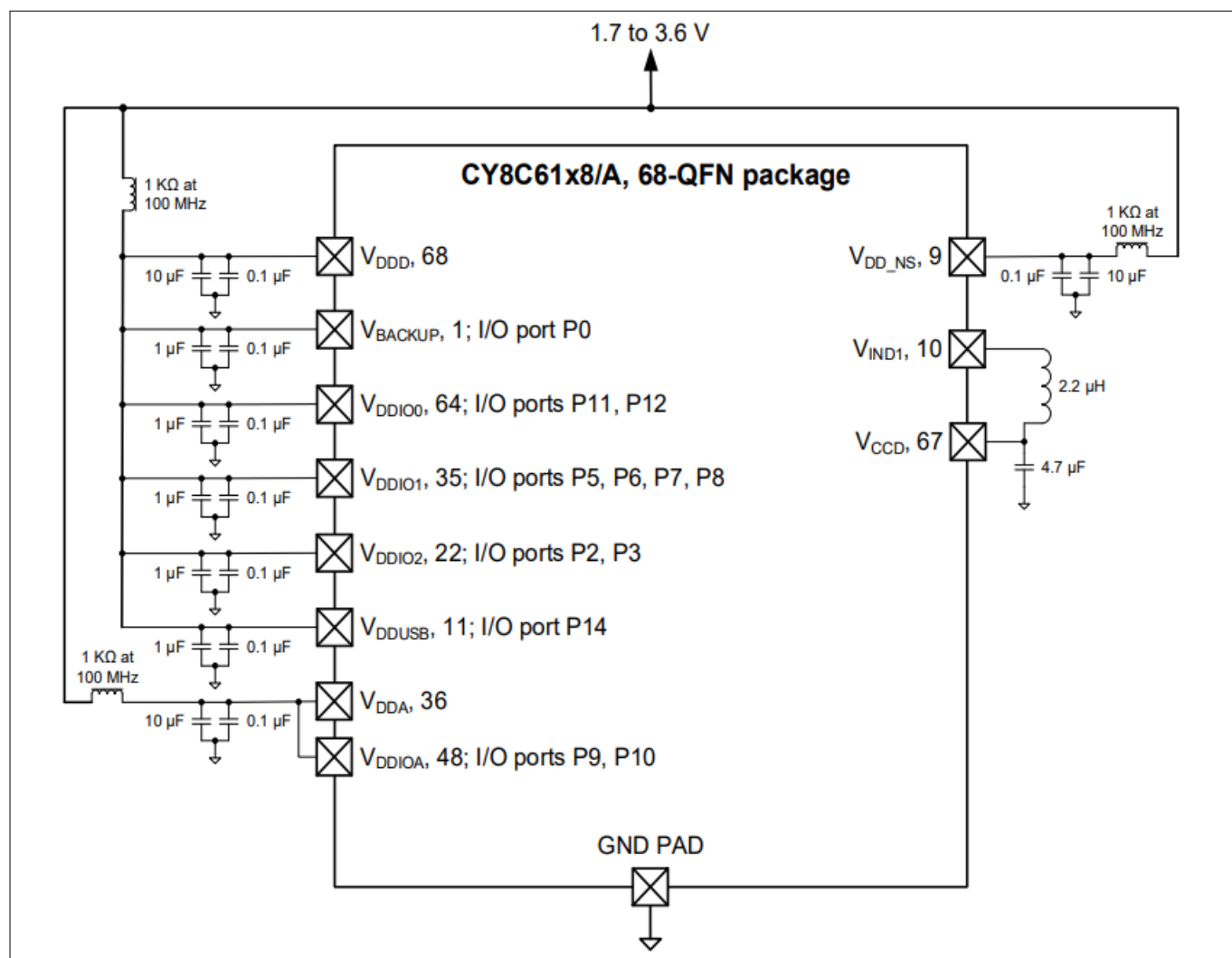
Figure 17 68-QFN Power connection diagram
