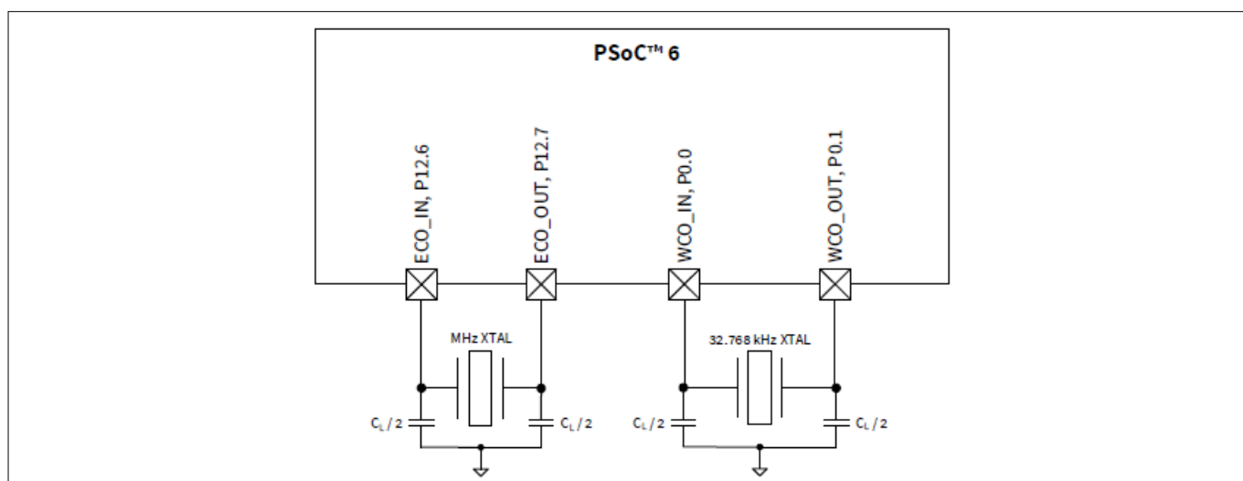
Figure 4 Oscillator circuits
