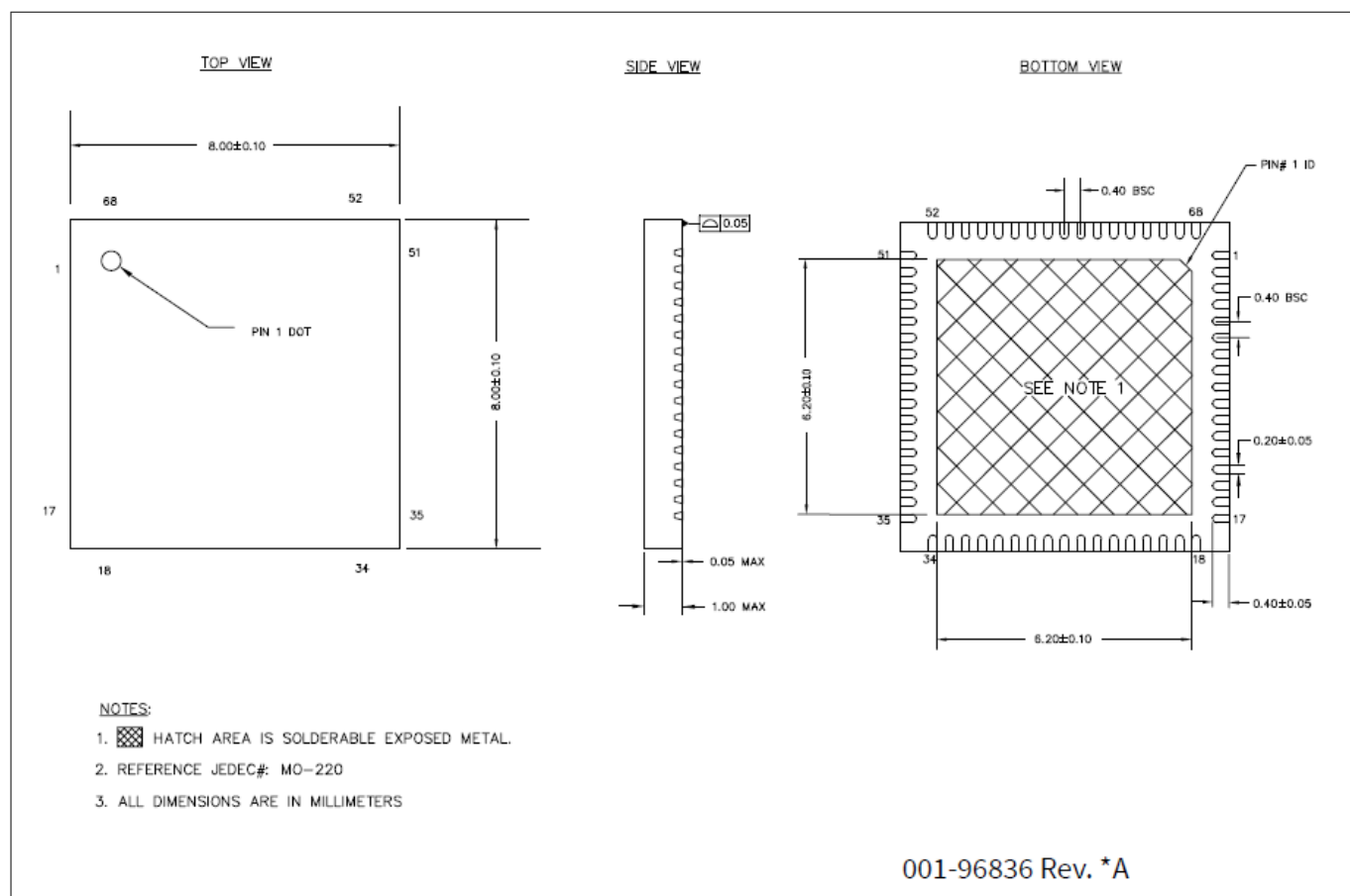
Figure 24 68-pin QFN ((8 × 8 × 1.0 mm) LT68D, 6.2 × 6.2 mm E-Pad (Sawn type)) package outline (PG-VQFN-68)
