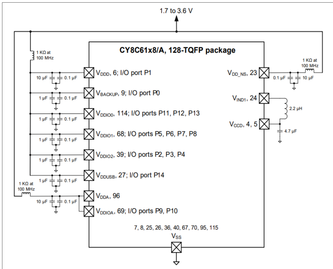
Figure 11 128-TQFP Power connection diagram
