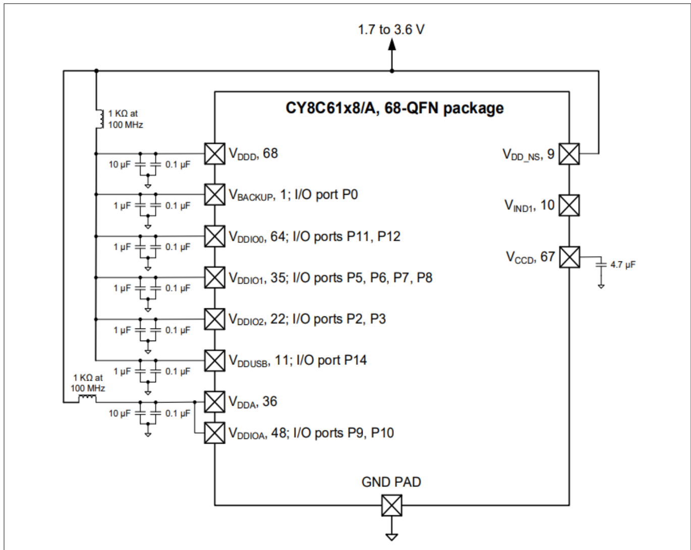
Figure 18 68-QFN (No Buck) Power connection diagram
