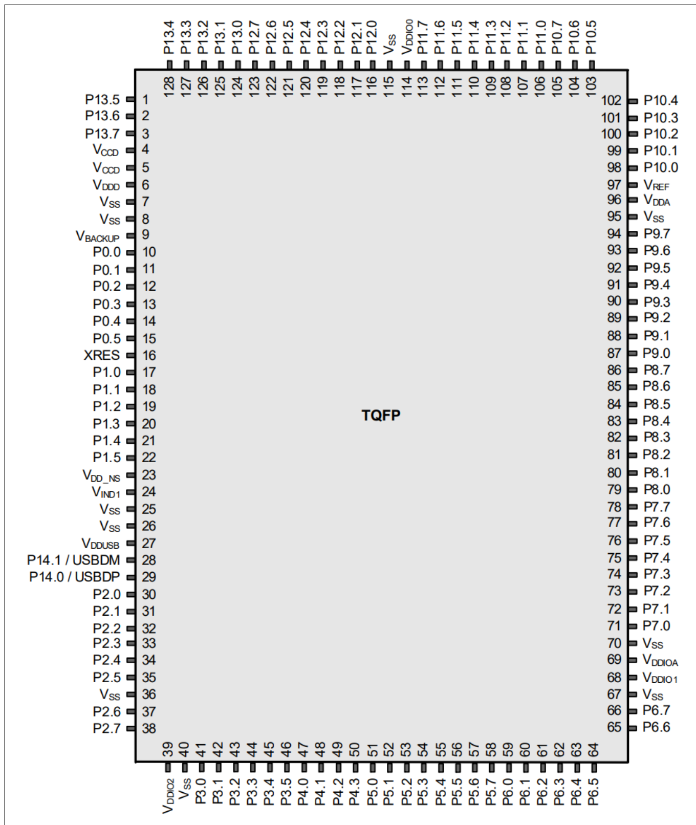
Figure 9 Device pinout for 128-pin TQFP package
