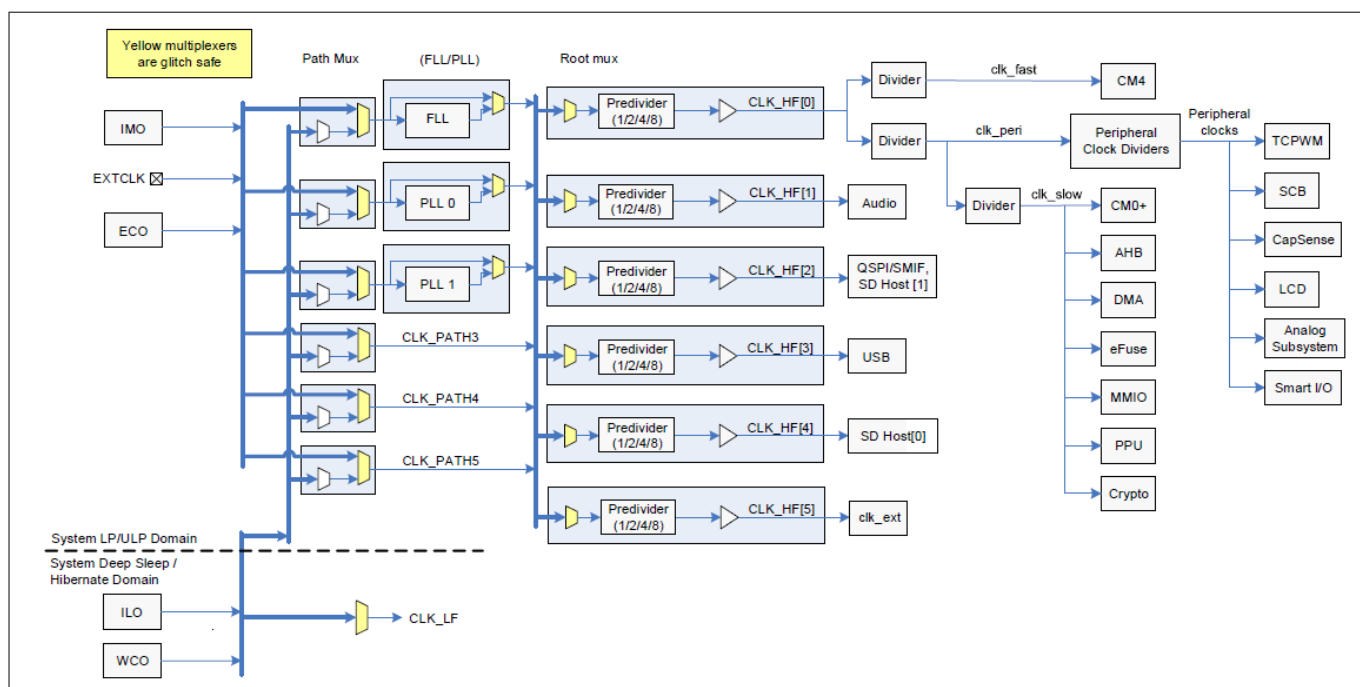
Figure 3 Clocking diagram
