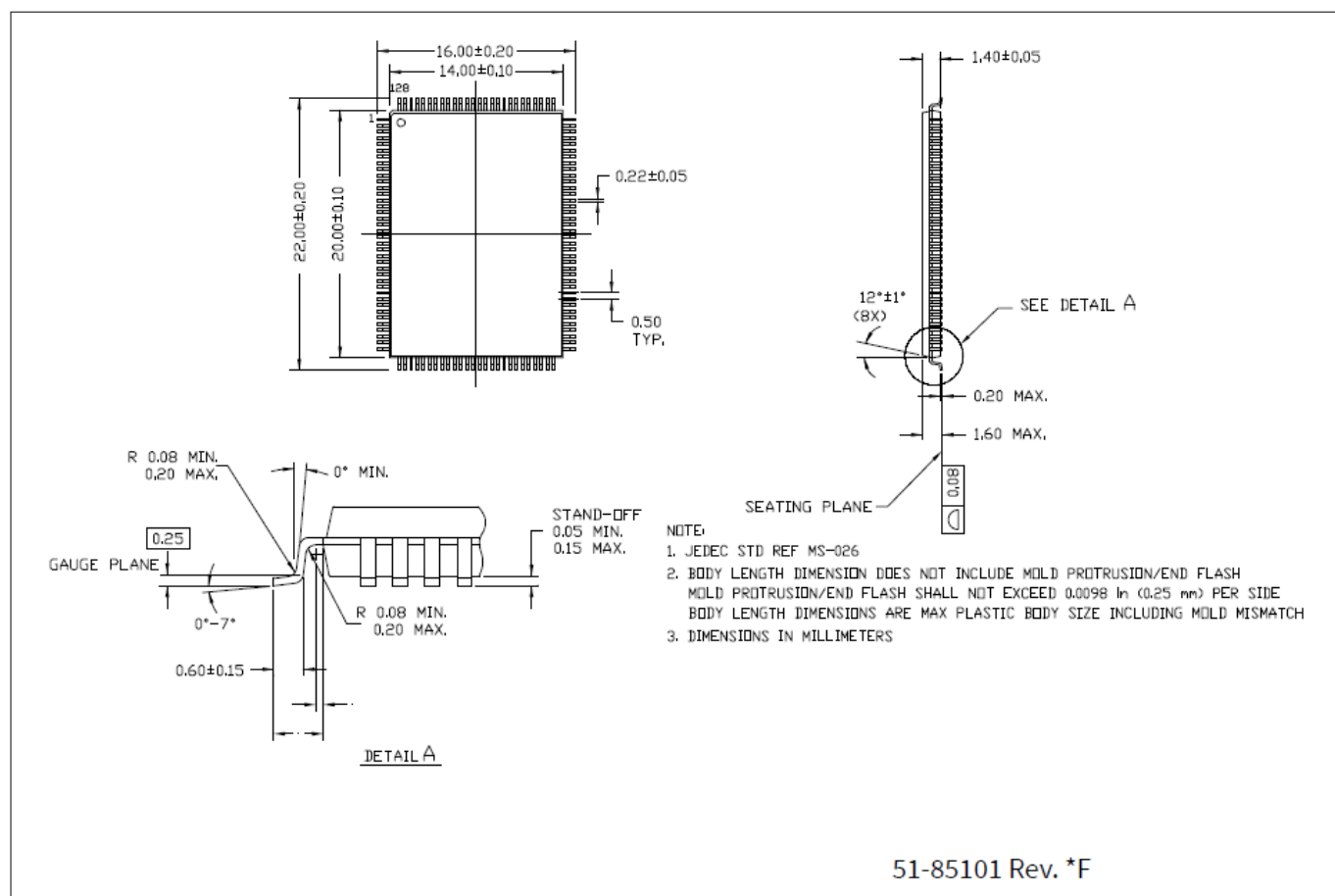
Figure 22 128-pin TQFP (14.0 × 20.0 × 1.4 mm) A128RA package outline (PG-TQFP-128)
