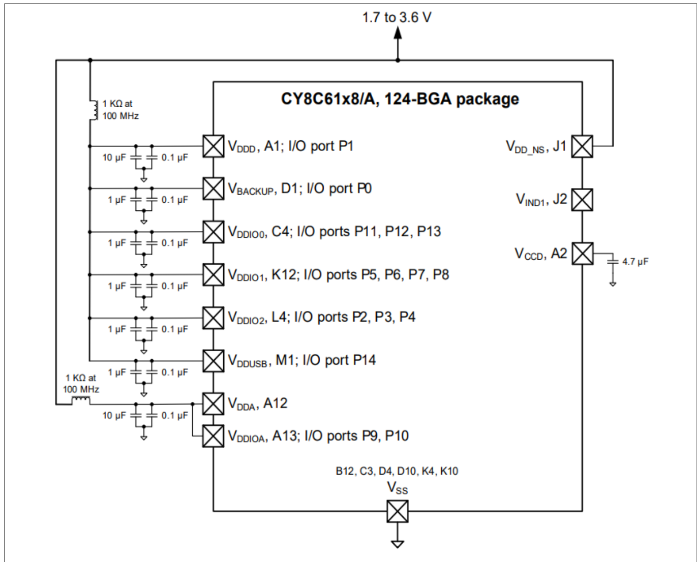
Figure 14 124-BGA (No Buck) Power connection diagram
