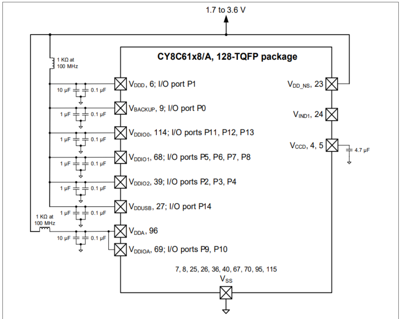
Figure 12 128-TQFP (No Buck) Power connection diagram
