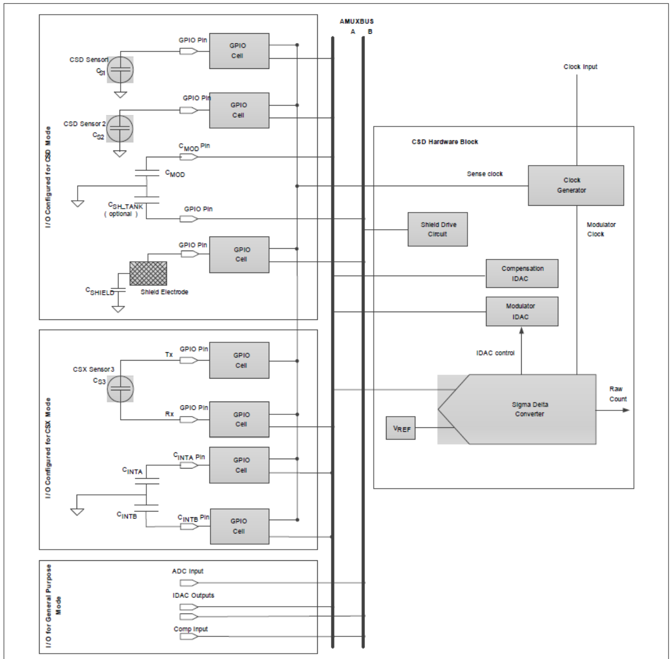
Figure 7 CAPSENSE™ hardware subsystem
