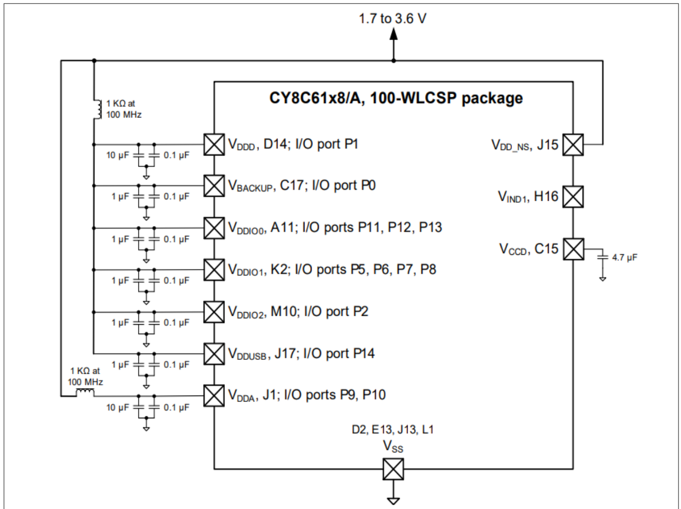
Figure 16 100-WLCSP (No Buck) Power connection diagram
