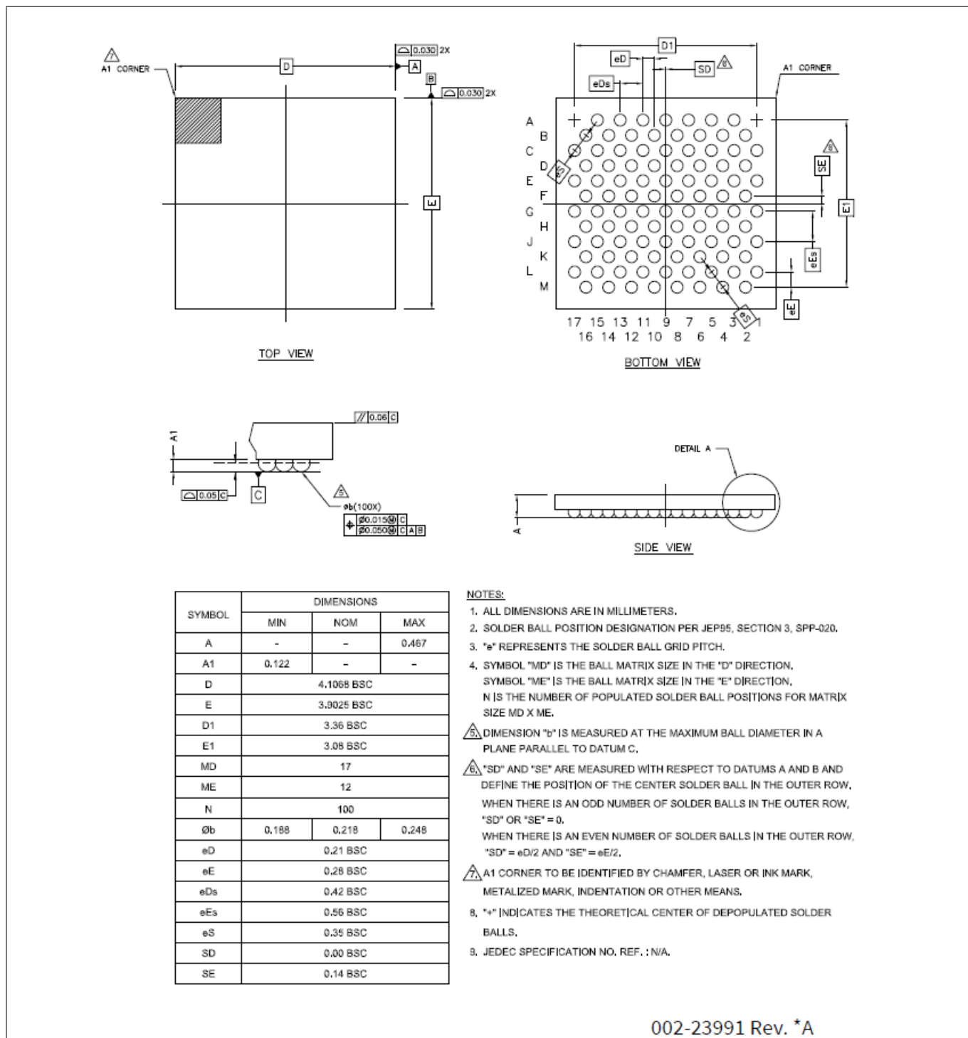
Figure 23 100-ball WLCSP (4.1068 × 3.9025 × 0.467 mm) FN100 (PSOC6A-2M) package outline (SG-XFWLB-100)
