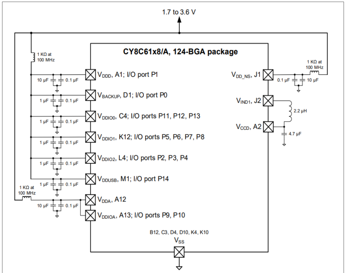
Figure 13 124-BGA Power connection diagram
