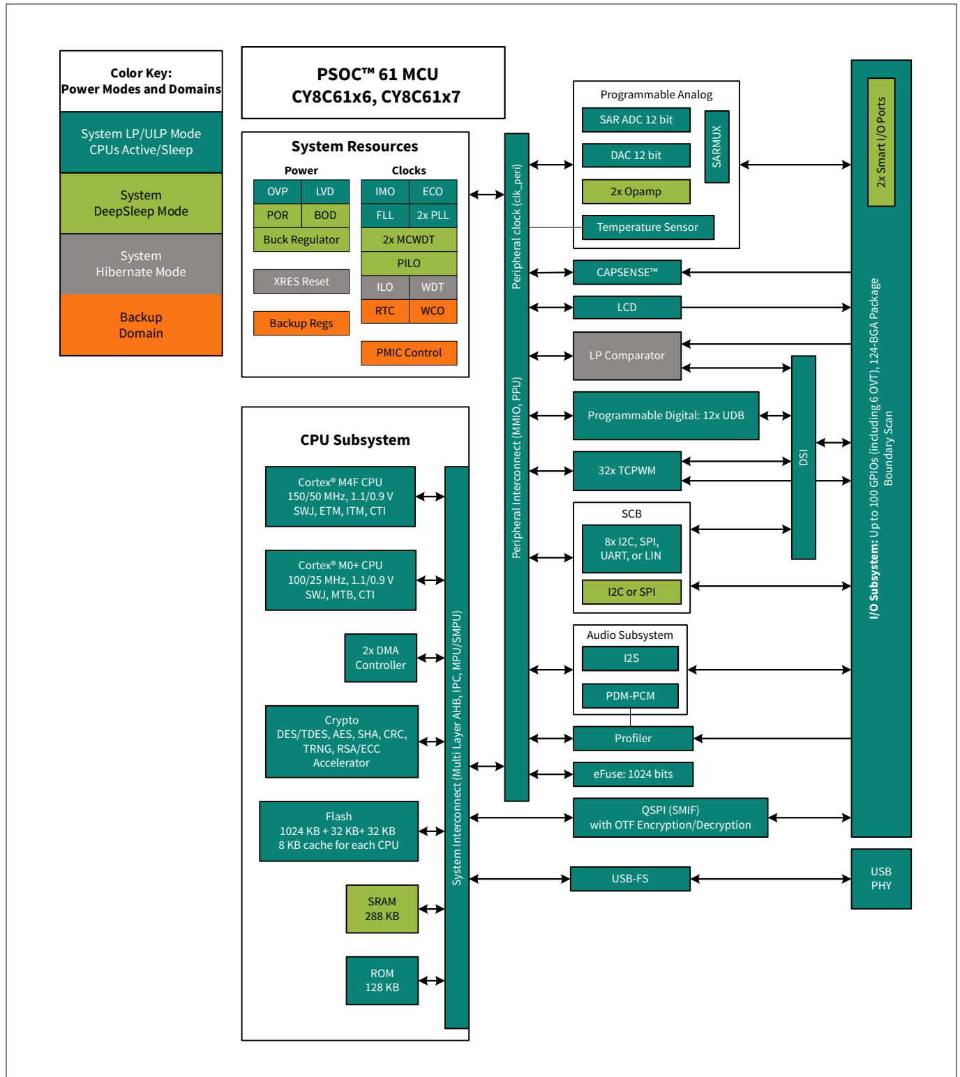
Figure 3 Block diagram
