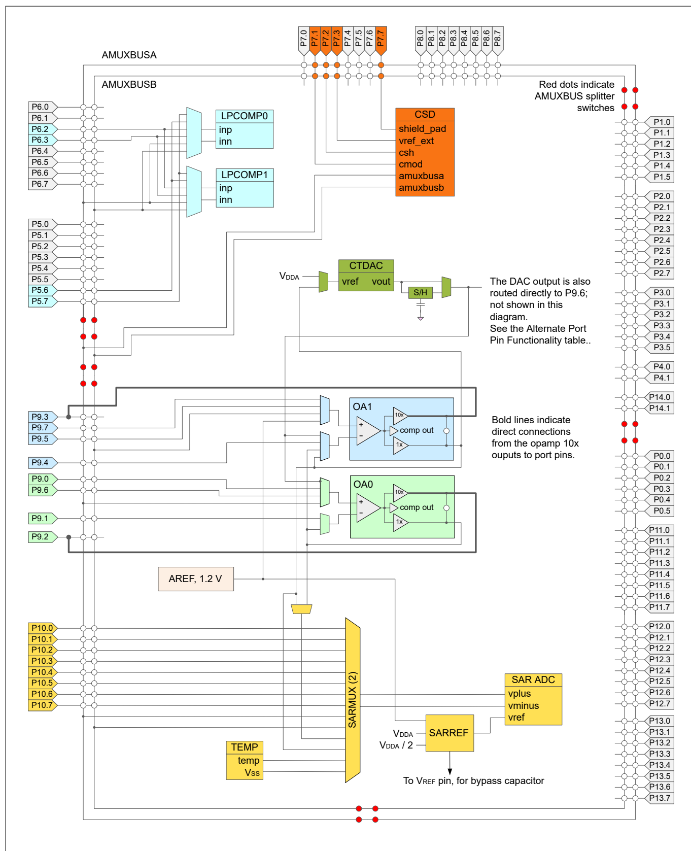
Figure 7 Analog subsystem
