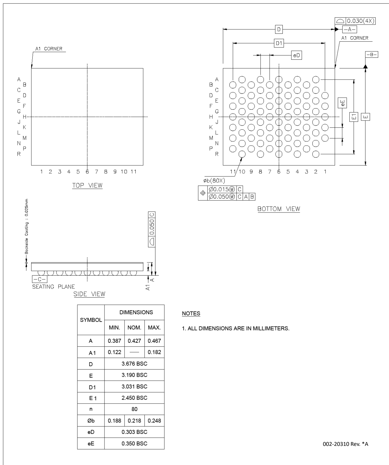
Figure 20 80-ball WLCSP 3.676 × 3.190 × 0.467 mm FN80B, package outline (SG-XFWLB-80)
