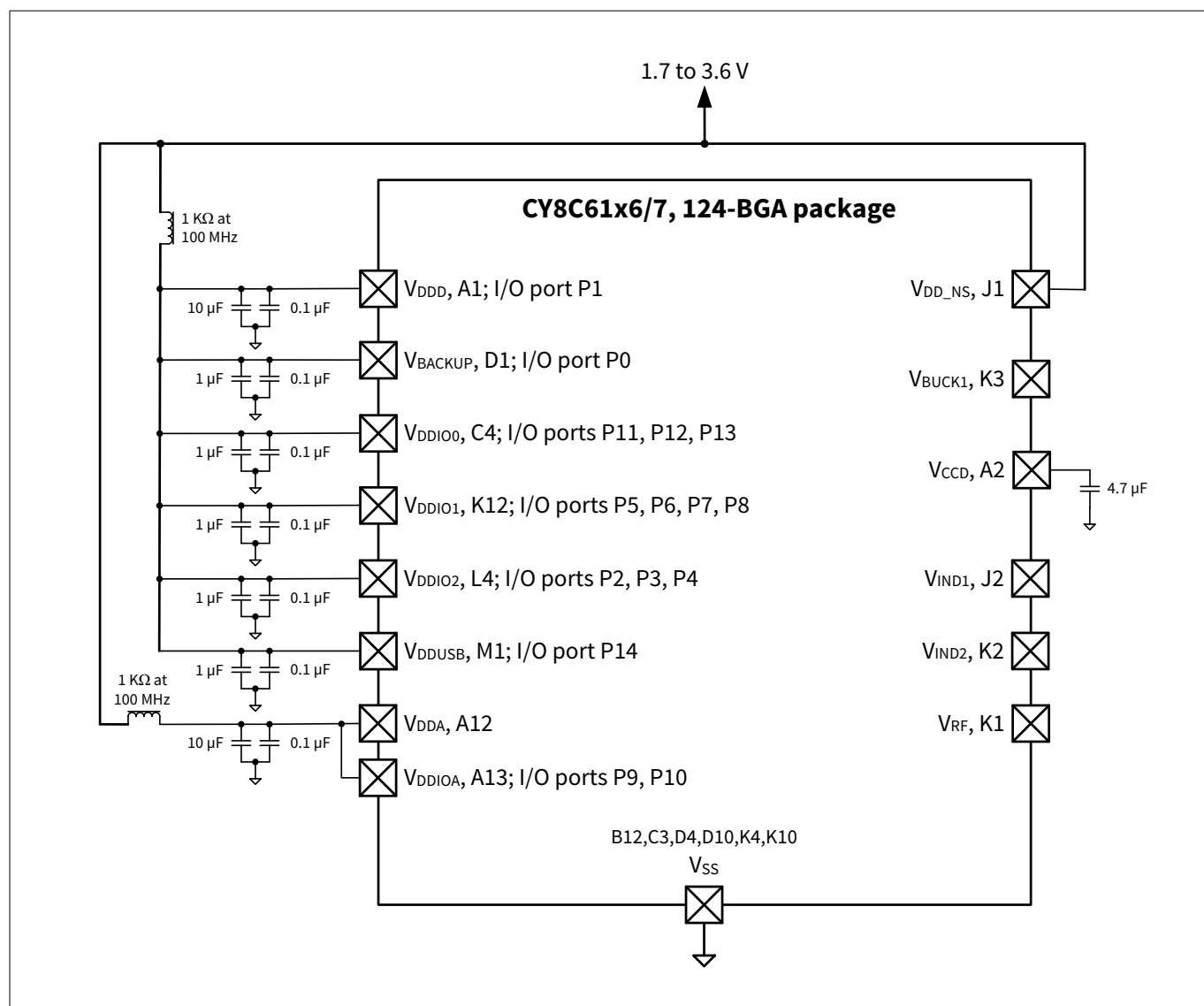
Figure 12 124-BGA (No buck) power connection diagram
