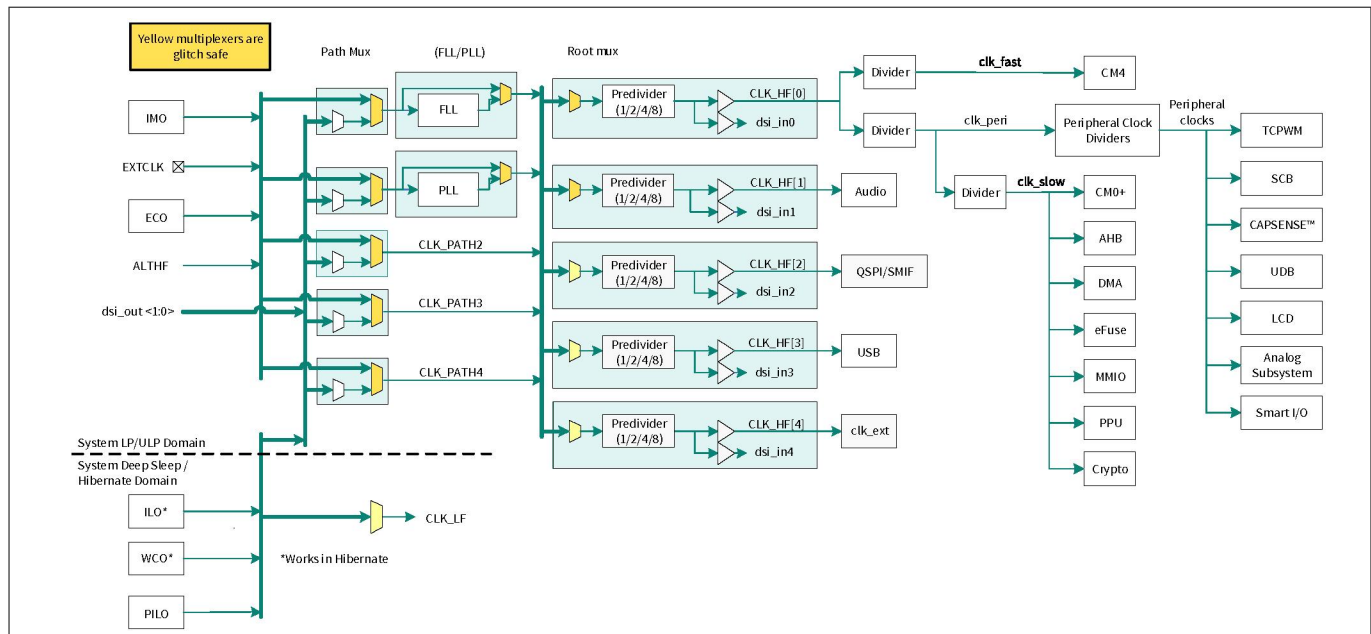
Figure 4 Clocking diagram
