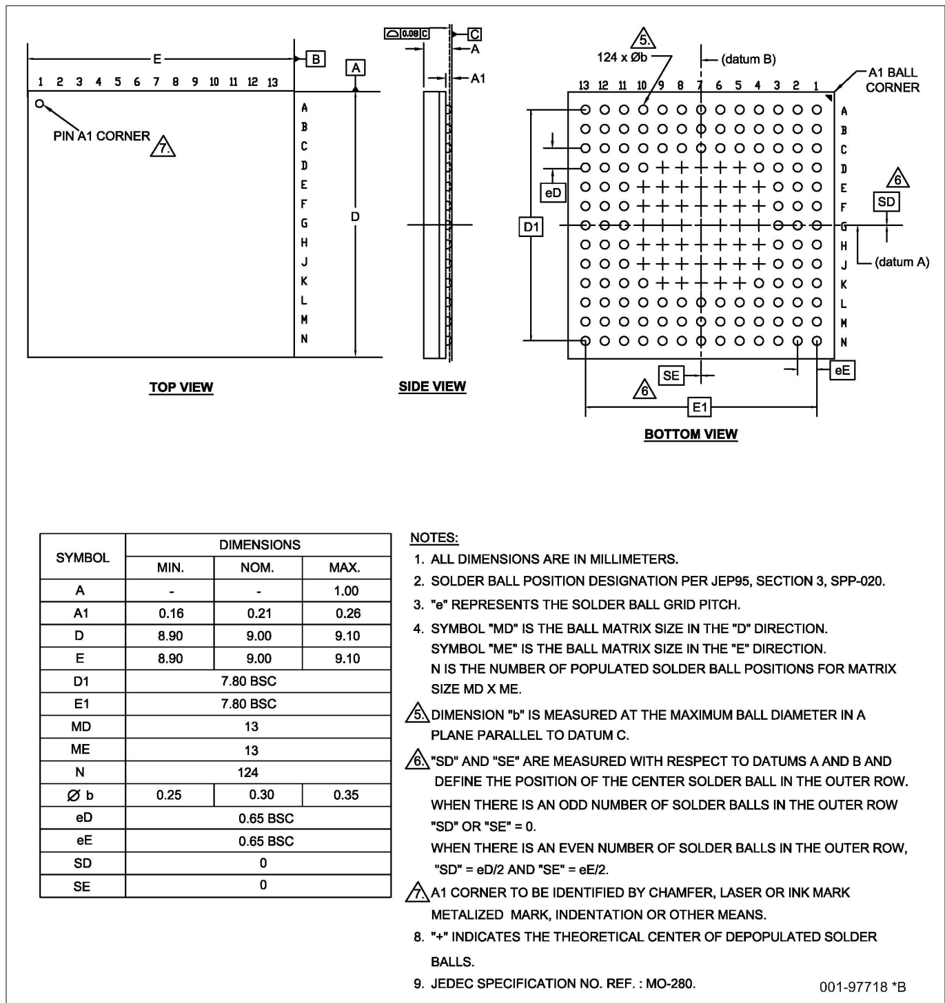
Figure 19 124-BGA 9.0 x 9.0 x 1.0 mm (PG-VFBGA-124-800)
