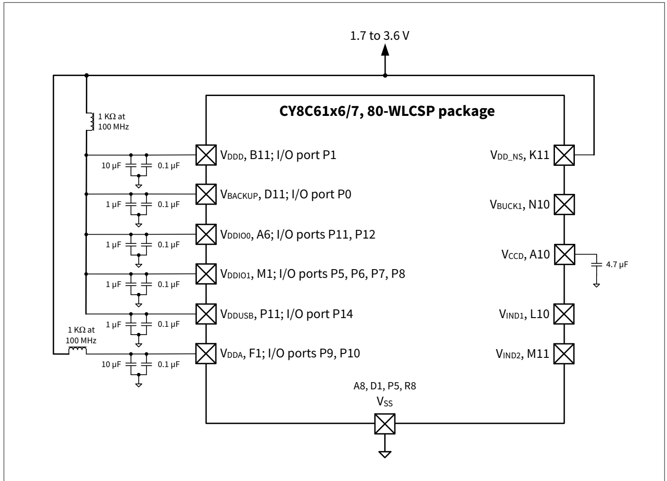
Figure 14 80-WLCSP (no buck) power connection diagram
