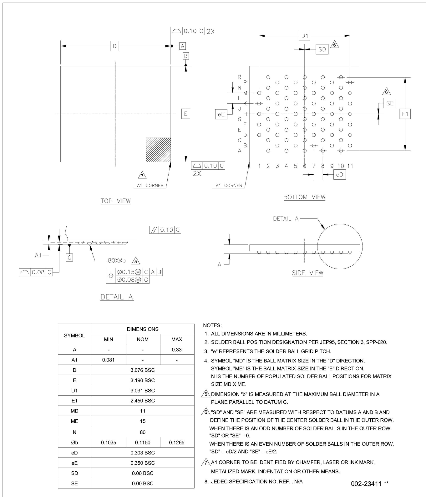
Figure 22 80-ball WLCSP 3.676 × 3.190 × 0.33 mm FL80A, package outline (SG-XFWLB-80)
