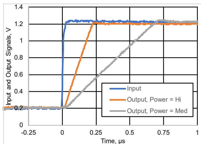
Figure 17 Opamp step response, rising
