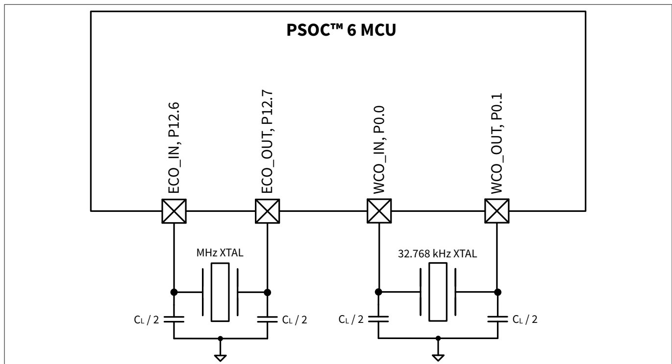
Figure 5 Oscillator circuits
