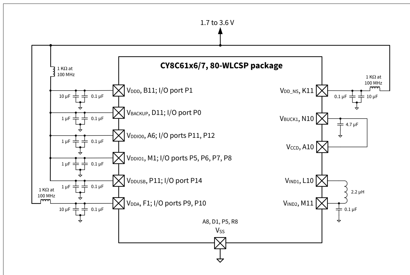
Figure 13 80-WLCSP power connection diagram
