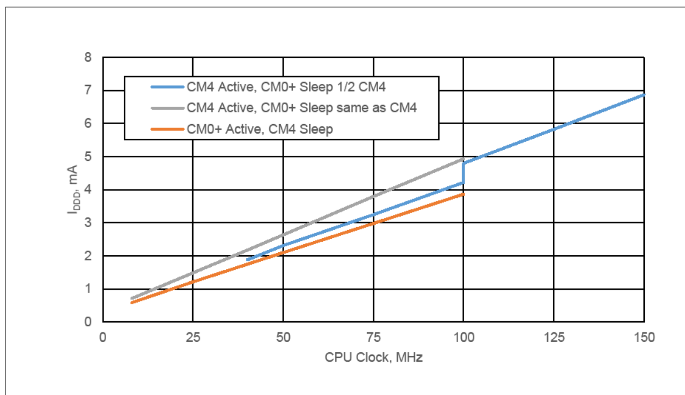
Figure 16 Typical device currents vs. CPU frequency; System Low Power (LP) mode 3)
