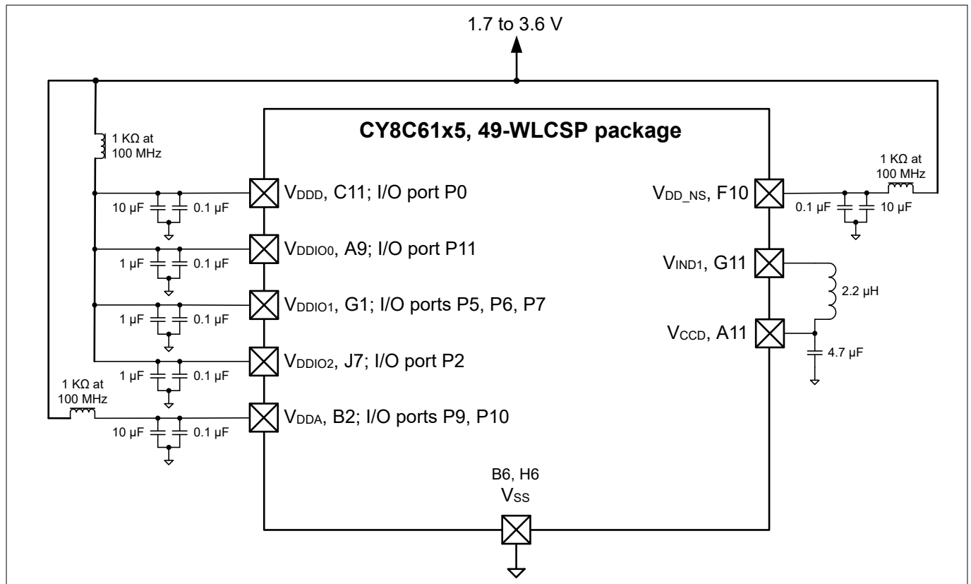
Figure 15 49-WLCSP power connection diagram
