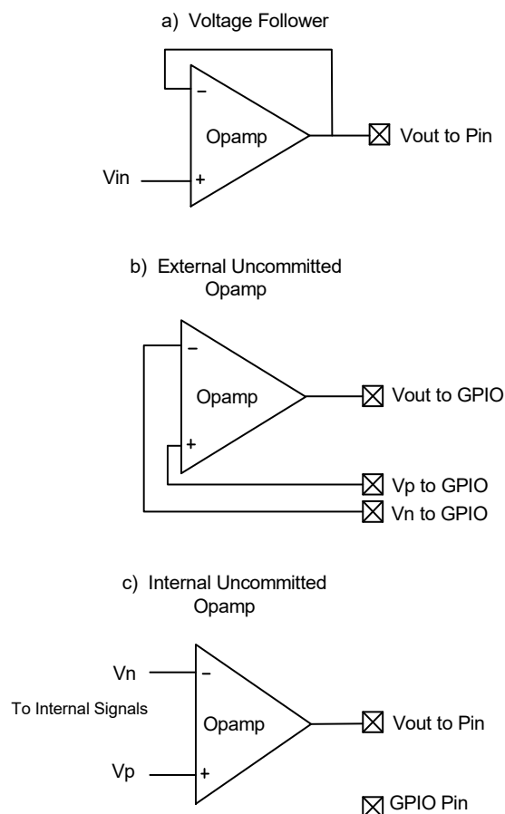
Figure 8-8. Opamp Configurations
