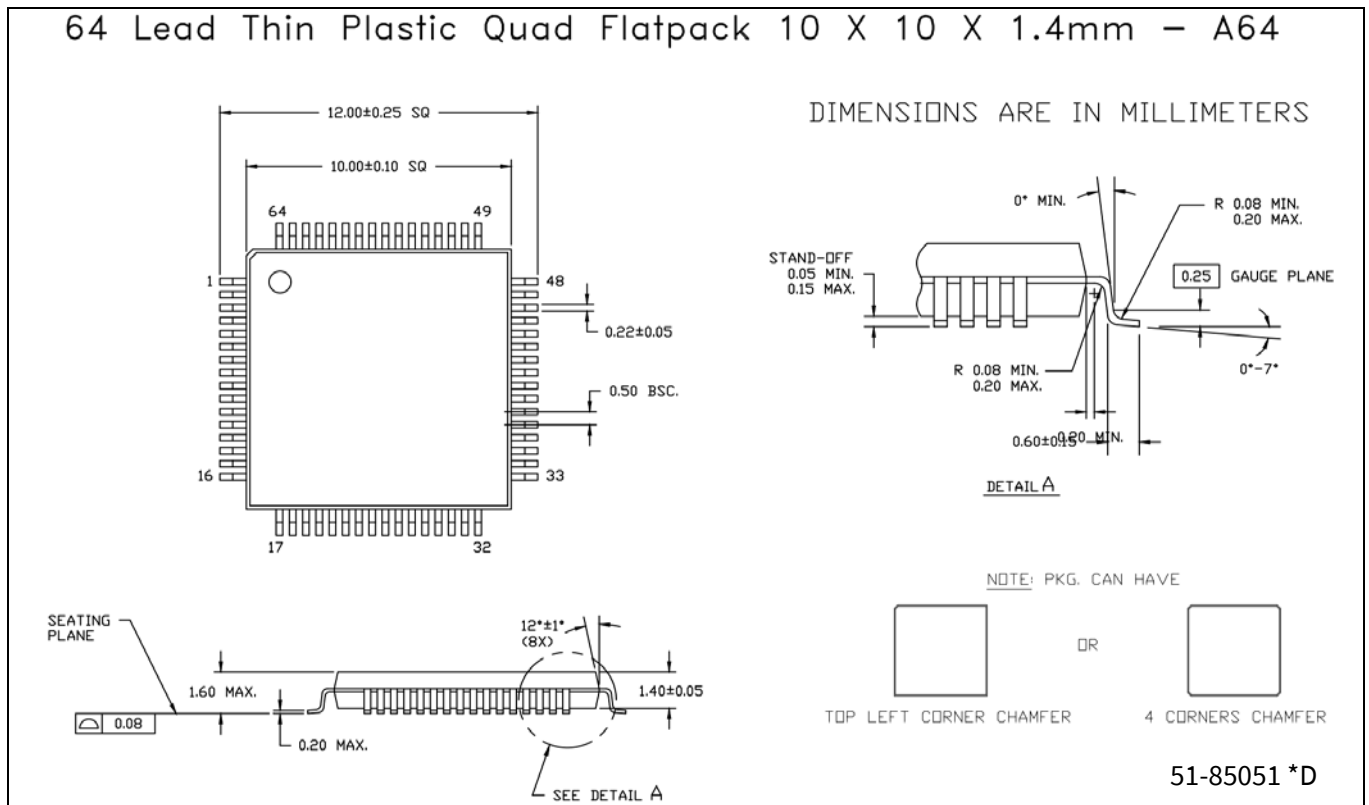
Figure 8 64LD TQFP 10X10X1.4 MM A64SB, PACKAGE OUTLINE, (PG-TQFP-64)
