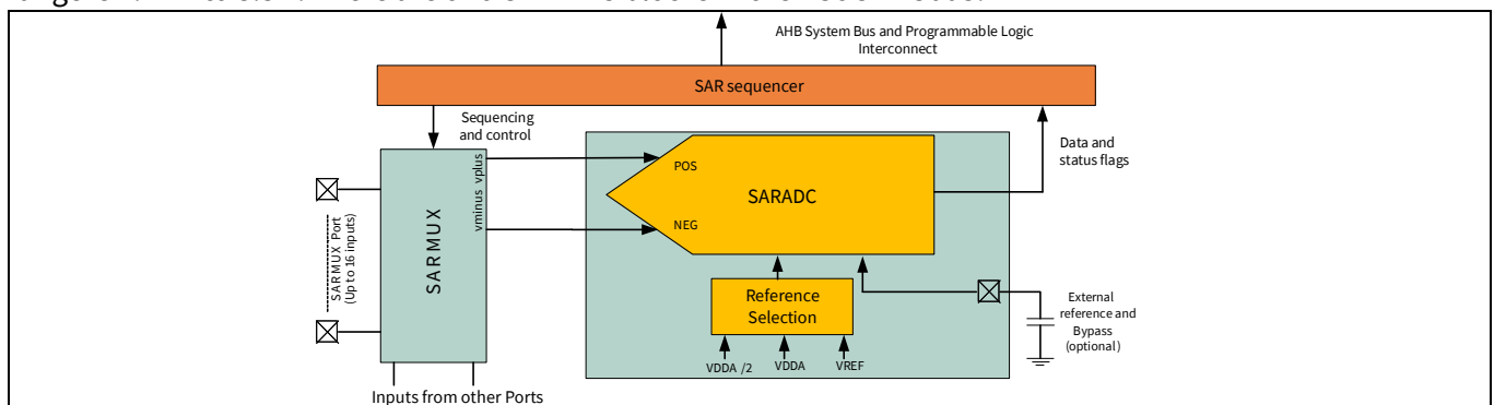
Figure 4 SAR ADC
