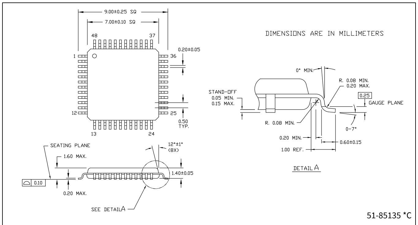
Figure 9 48LD TQFP 7X7X1.4 MM A48, PACKAGE OUTLINE, (PG-TQFP-48)
