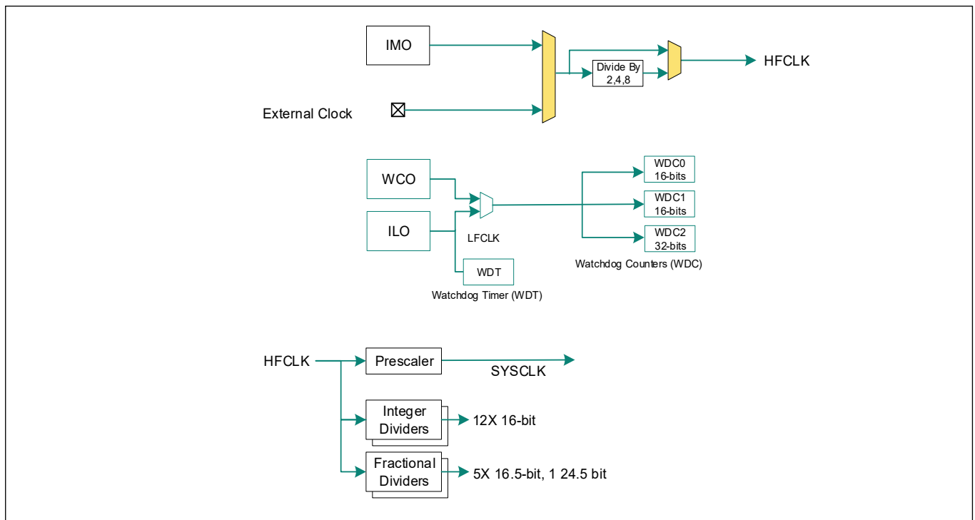
Figure 3 MCU clocking architecture
