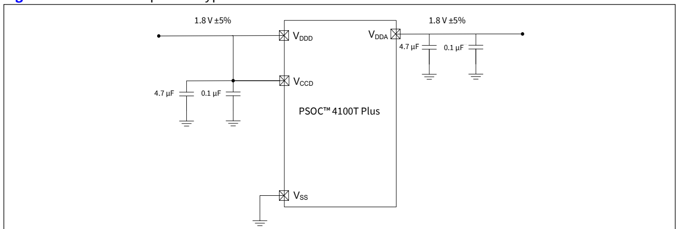
Figure 5 External supply of 1.8 V \pm 5%
