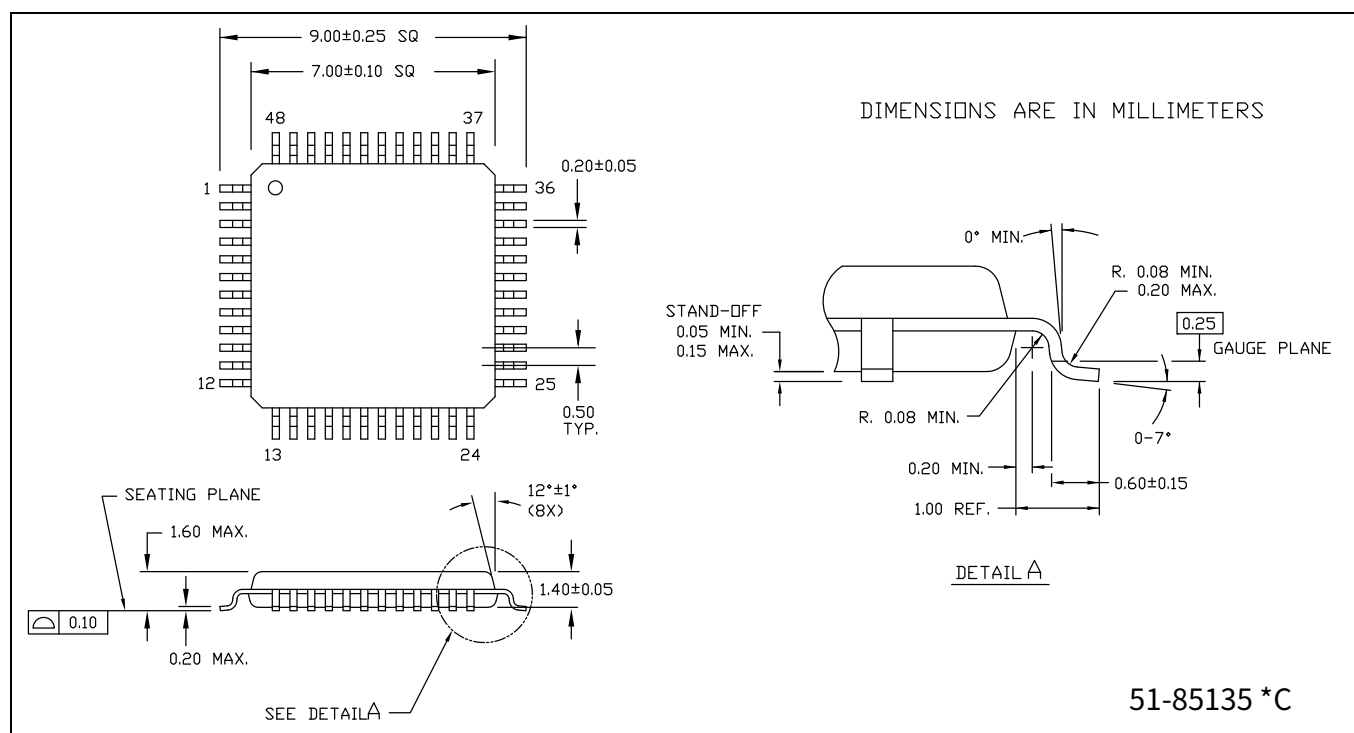
Figure 10 48 Pin 7 × 7 × 1.4 mm TQFP 封装外形 (PG-TQFP-48-800)
