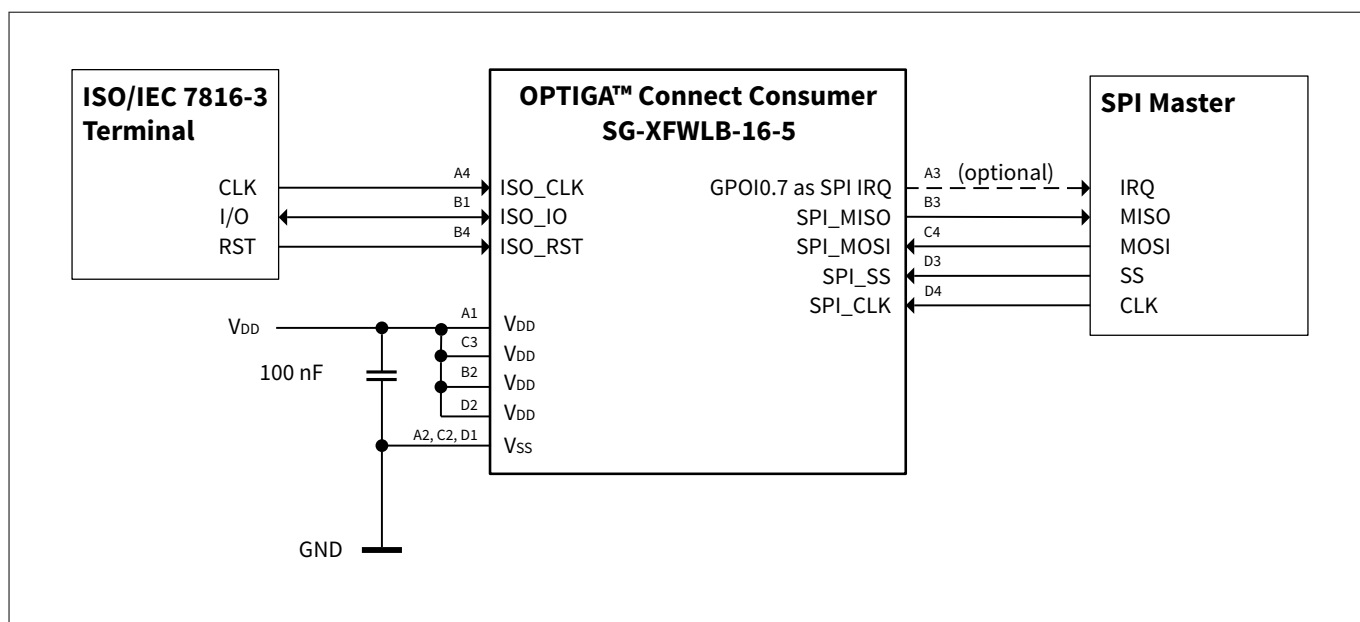
Figure 16 Reference schematics for SG-XFWLB-16-5 ISO + SPI + SPI IRQ
