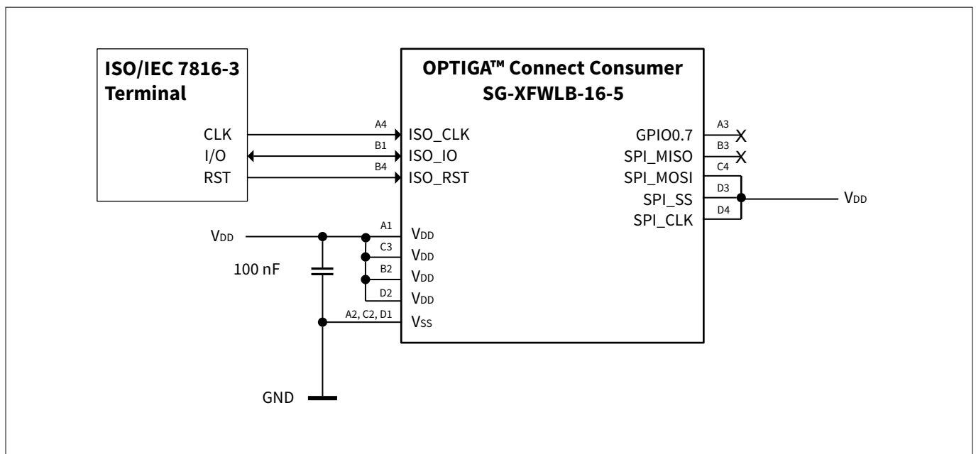
Figure 15 Reference schematics for SG-XFWLB-16-5 ISO only
