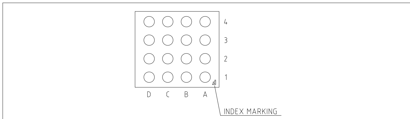
Figure 11 SG-XFWLB-16-5 PIN layout
