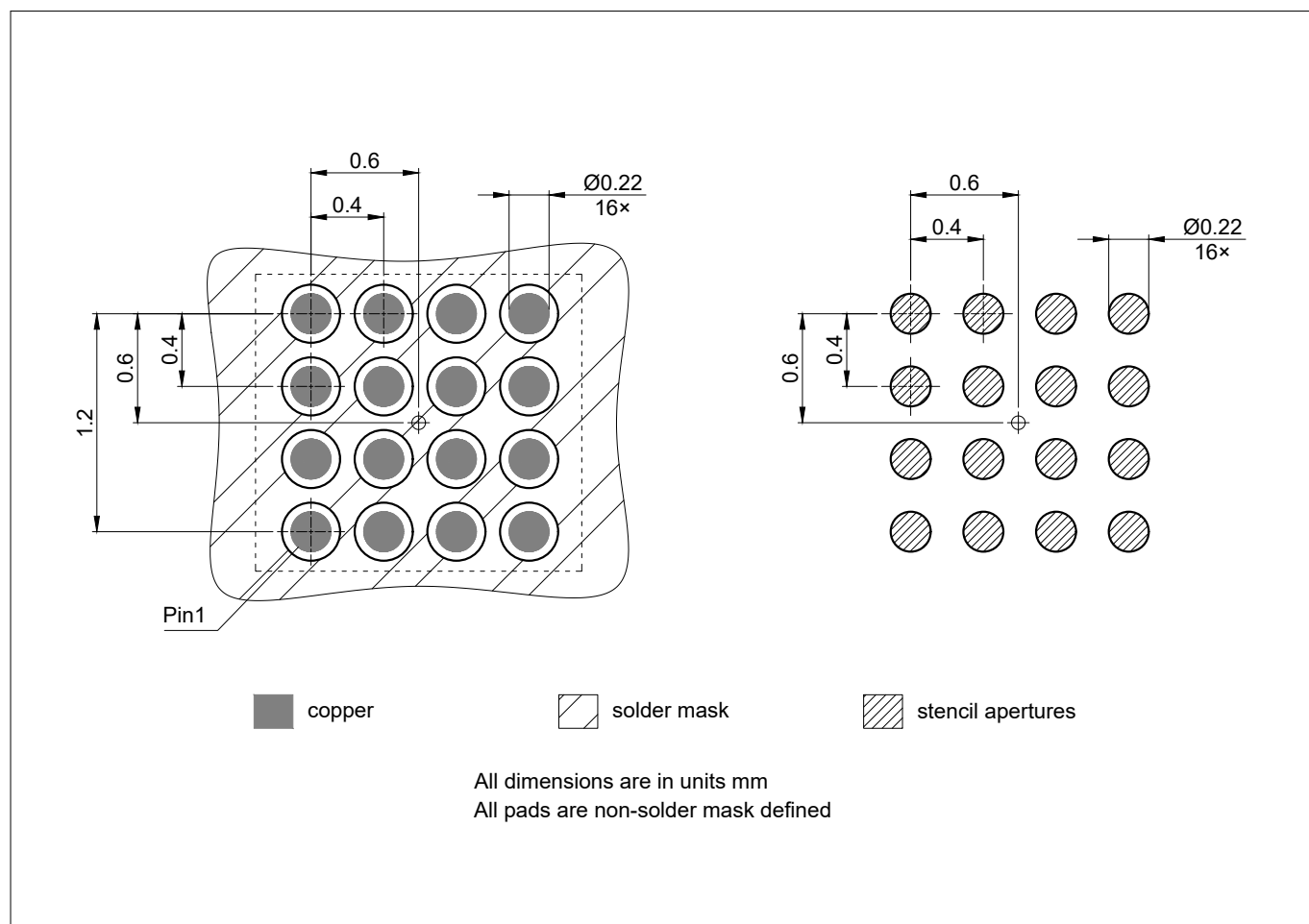
Figure 8 SG-XFWLB-16-5 package footprint
