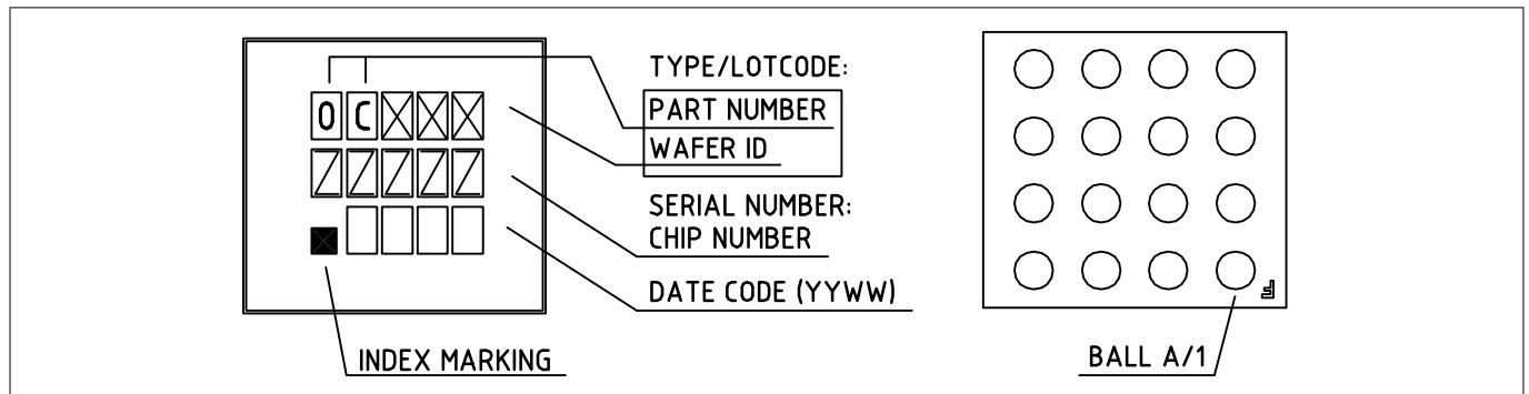
Figure 10 SG-XFWLB-16-5 sample marking pattern
