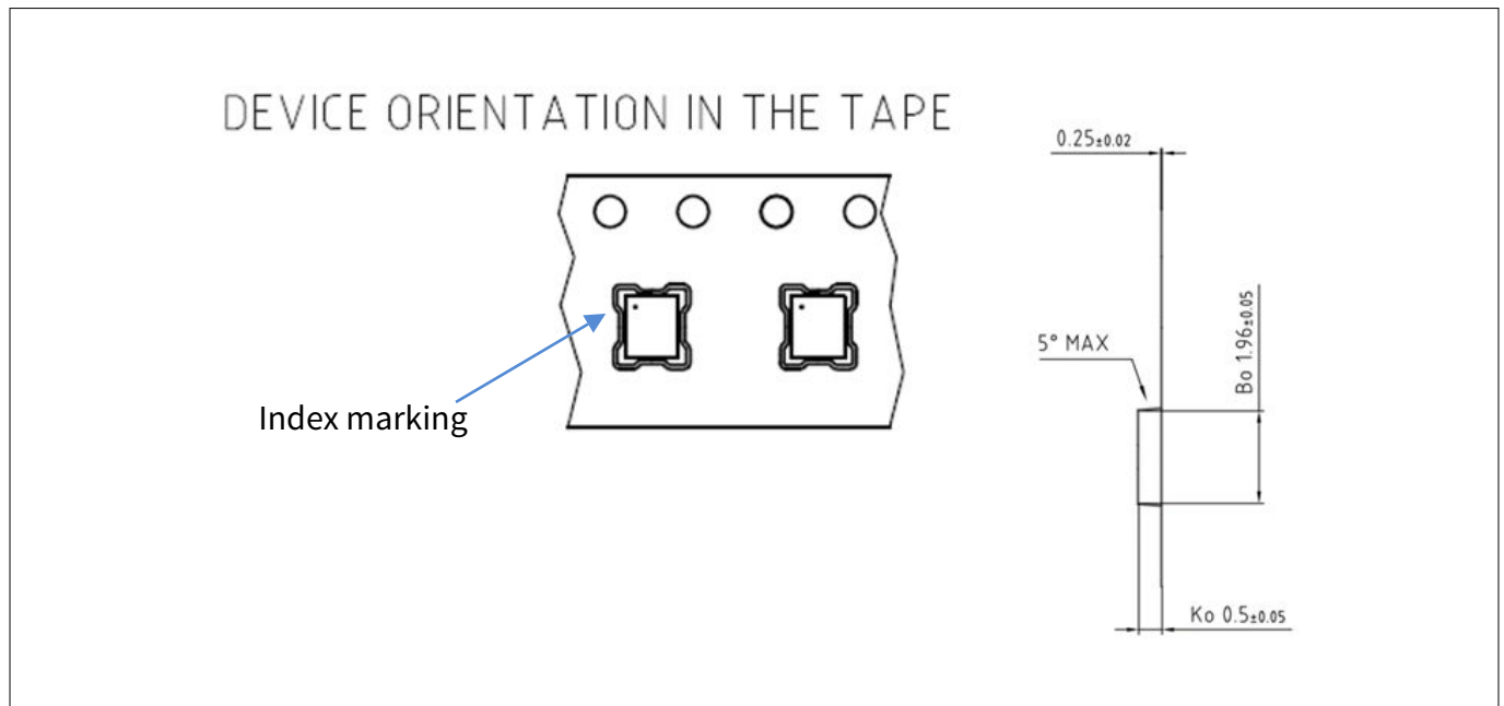
Figure 9 SG-XFWLB-16-5 tape and reel packing
