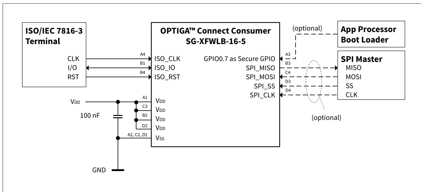
Figure 17 Reference schematics for SG-XFWLB-16-5 ISO + SPI + SECURE GPIO
