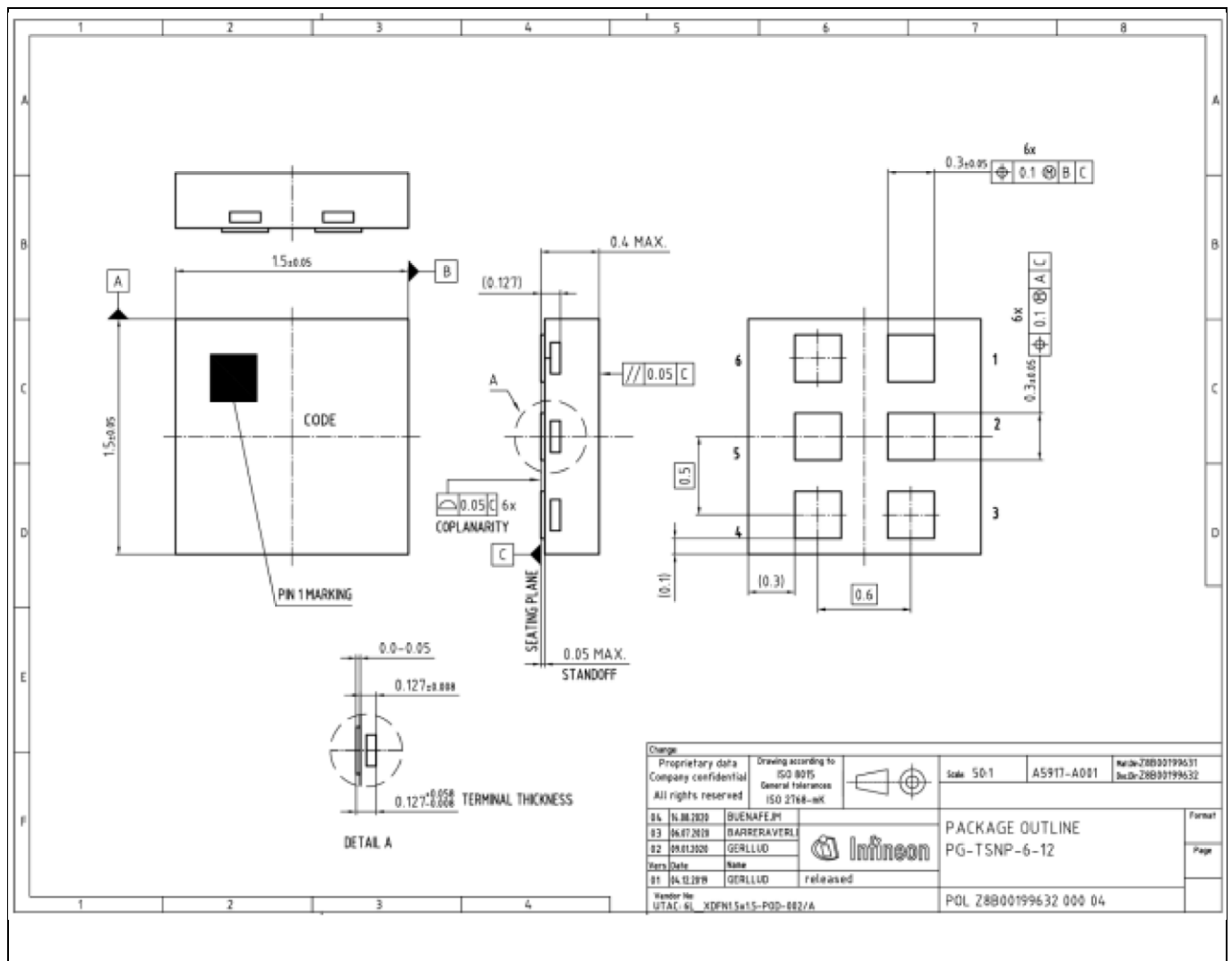
Figure 5 Package Dimensions
