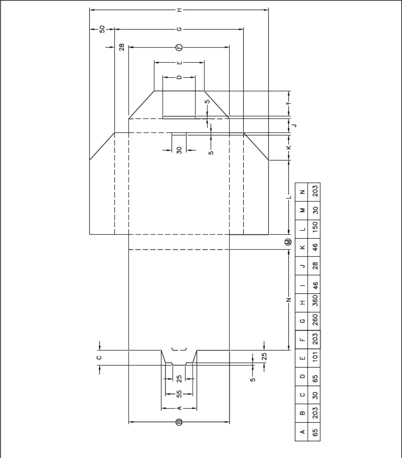
Figure 9 Box specification
