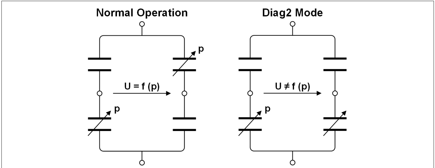
Figure 29 Diag2 functionality
