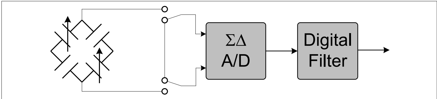
Figure 28 Diag1 functionality
