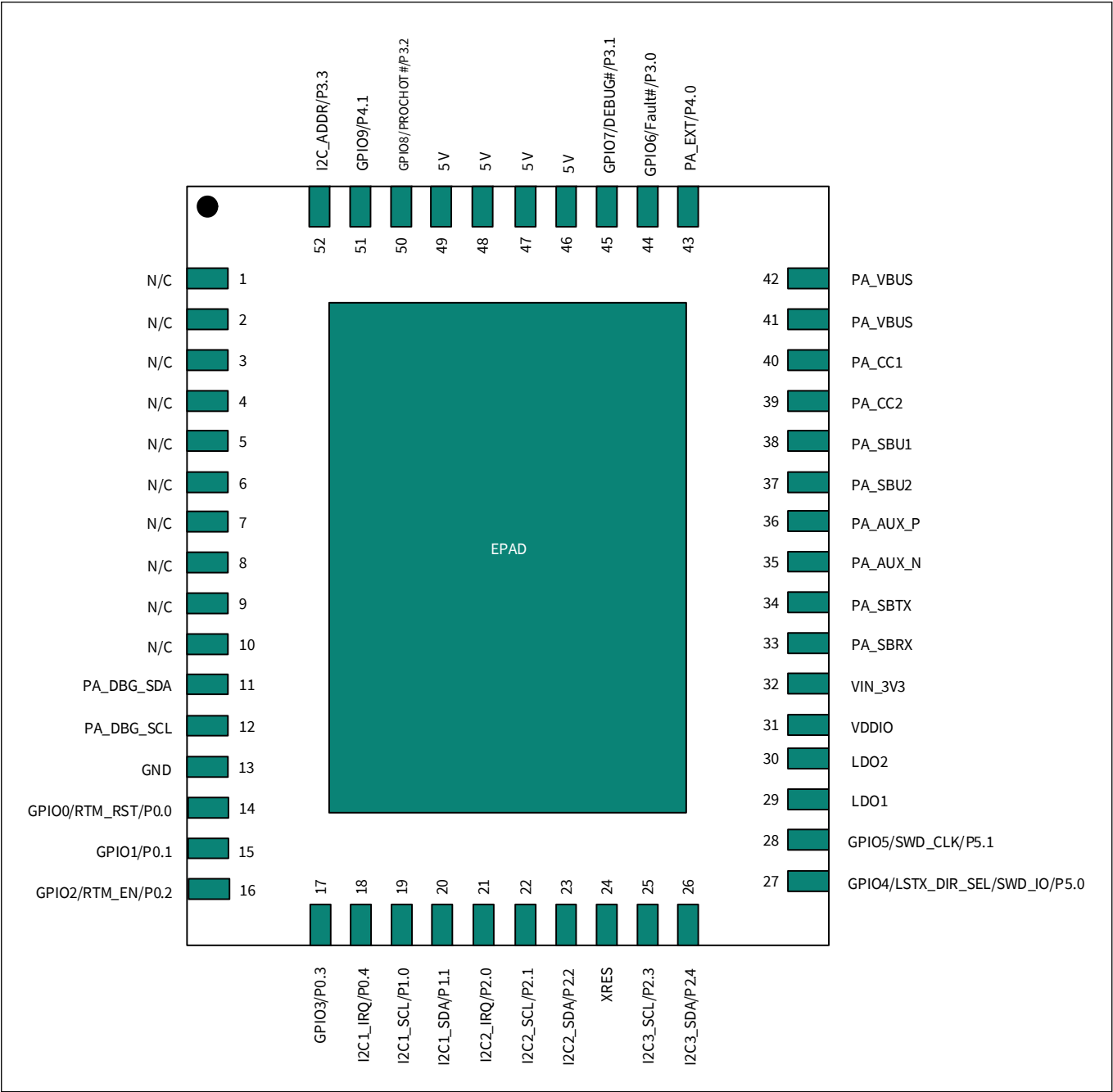
Figure 7 EZ-PD™ CCG6_CFP single-port 52-pin QFN pinout
