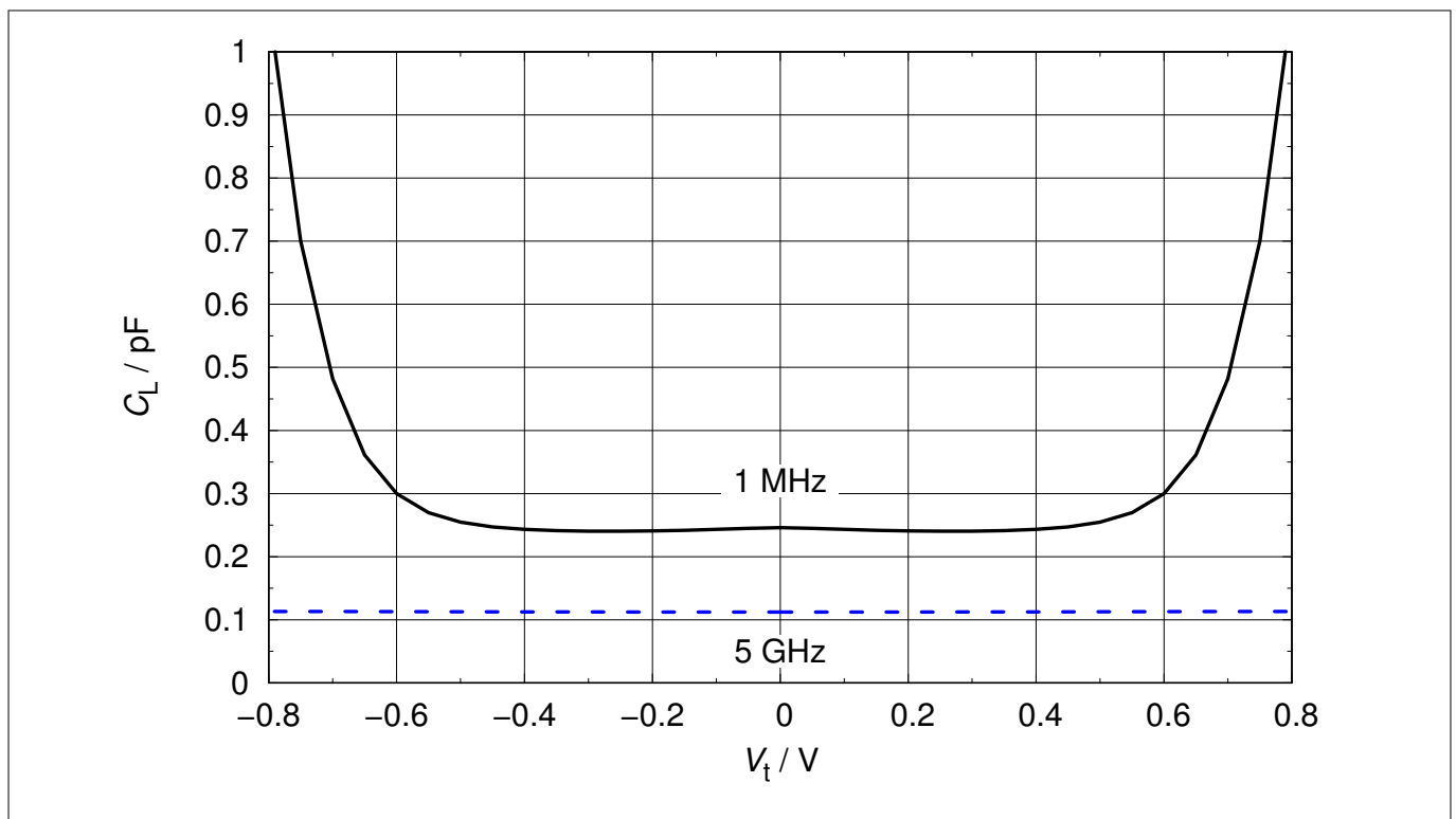
Figure 4 Line capacitance: C_L = f(V_t) , f = 1\text{ MHz}, 5\text{ GHz}
