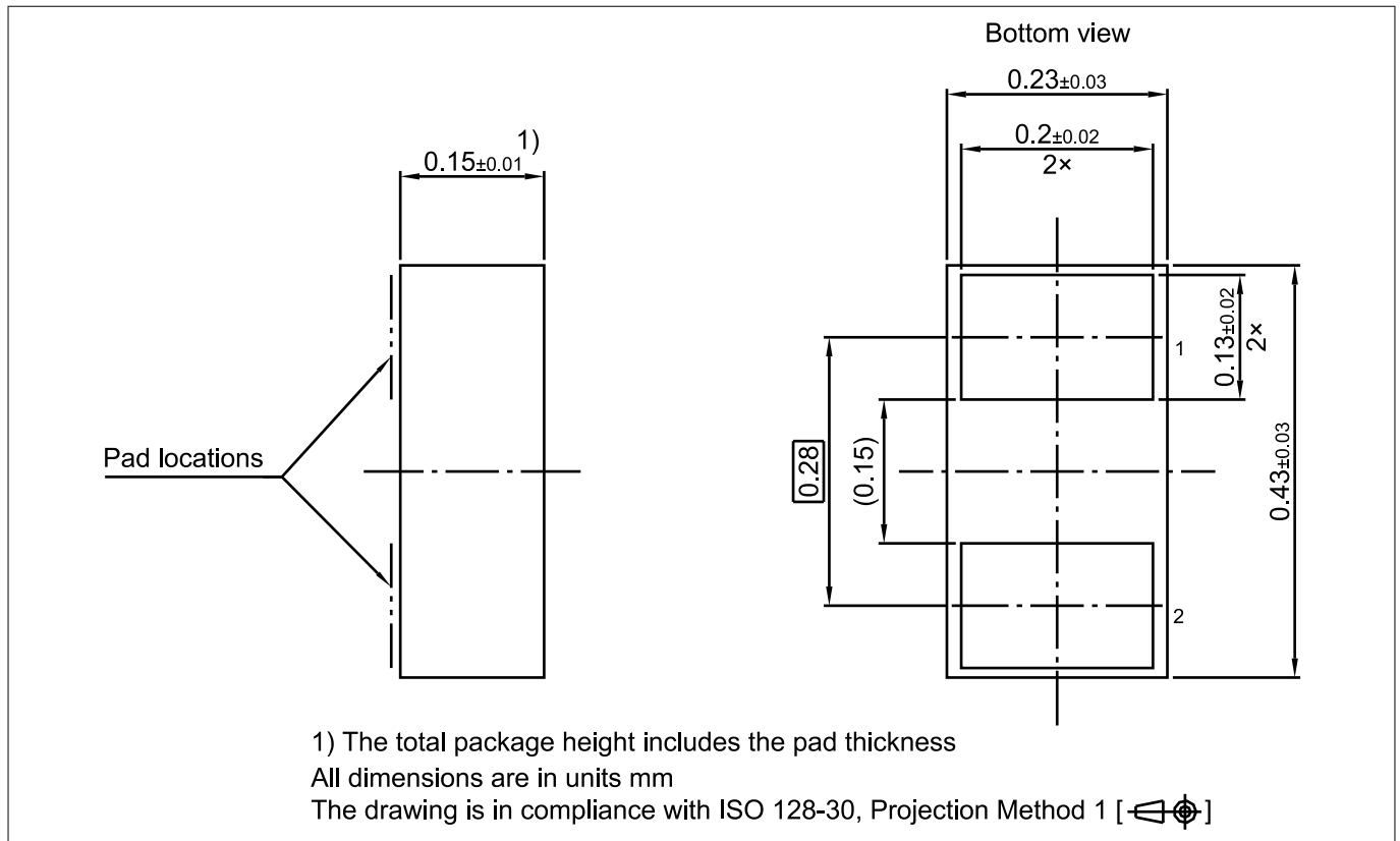
Figure 13 WLL-2-2 package
