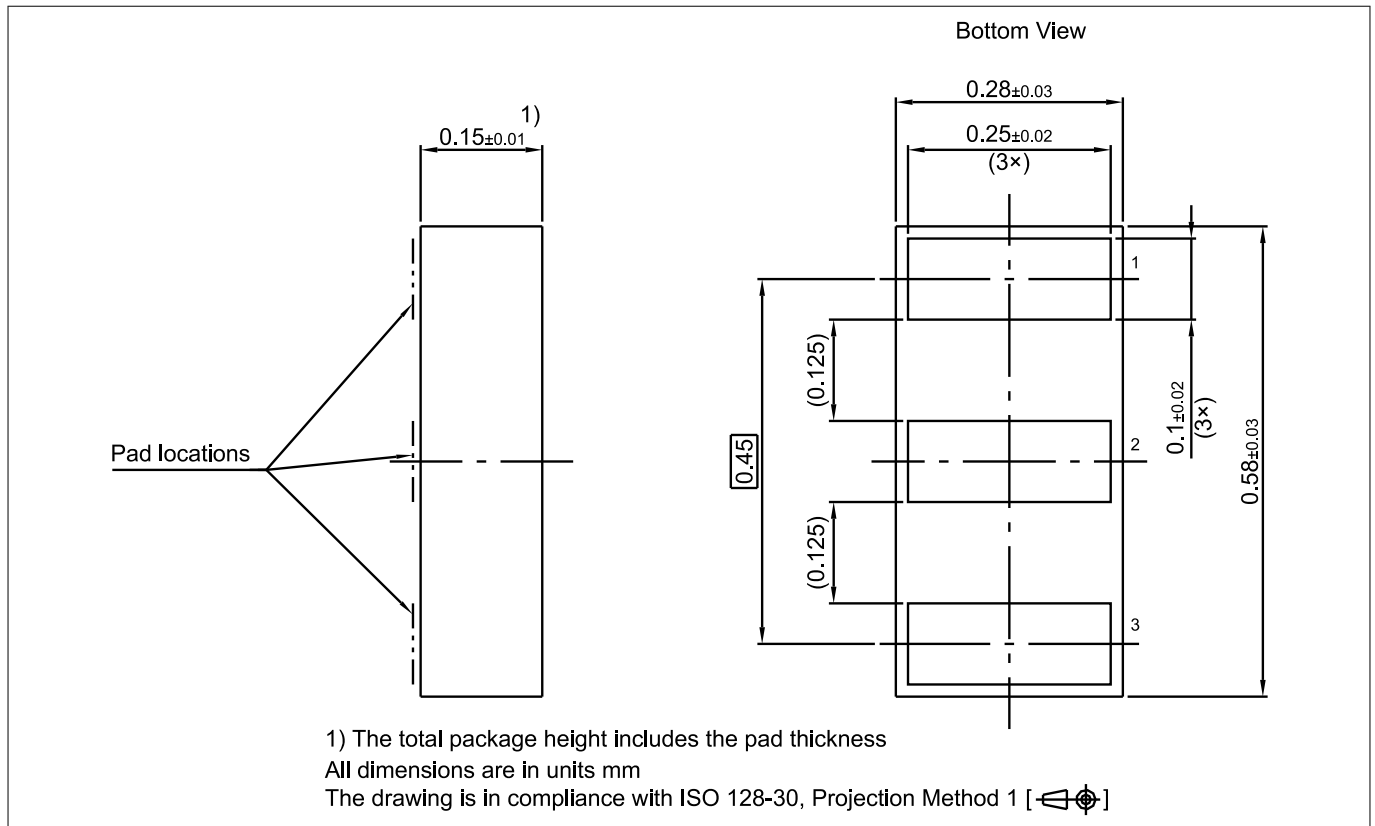
Figure 12 WLL-3-1 package
