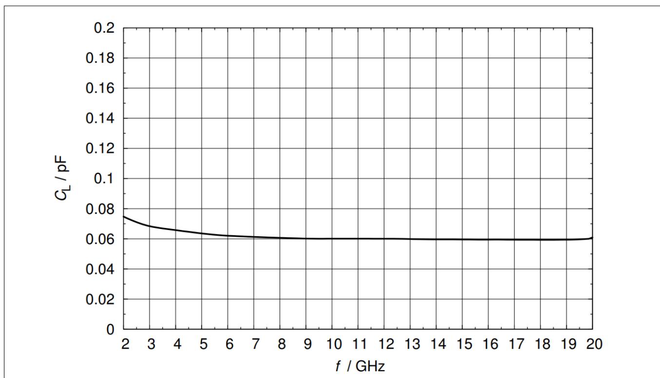
图5 线路电容: C_L = f(f) , V_t = 0\text{V}
