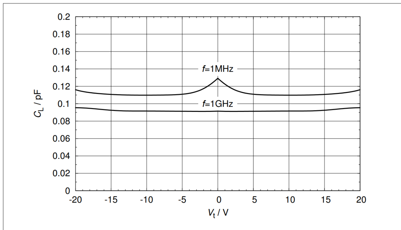
图4 线路电容 C_L = f(V_t) , f = 1\text{MHz} , 1\text{GHz}
