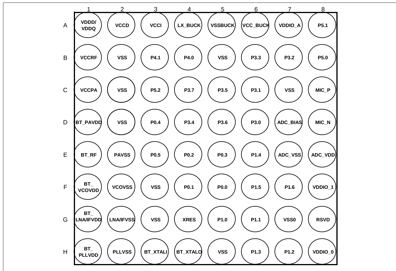
Figure 7 Device pinout for 64-BGA package
