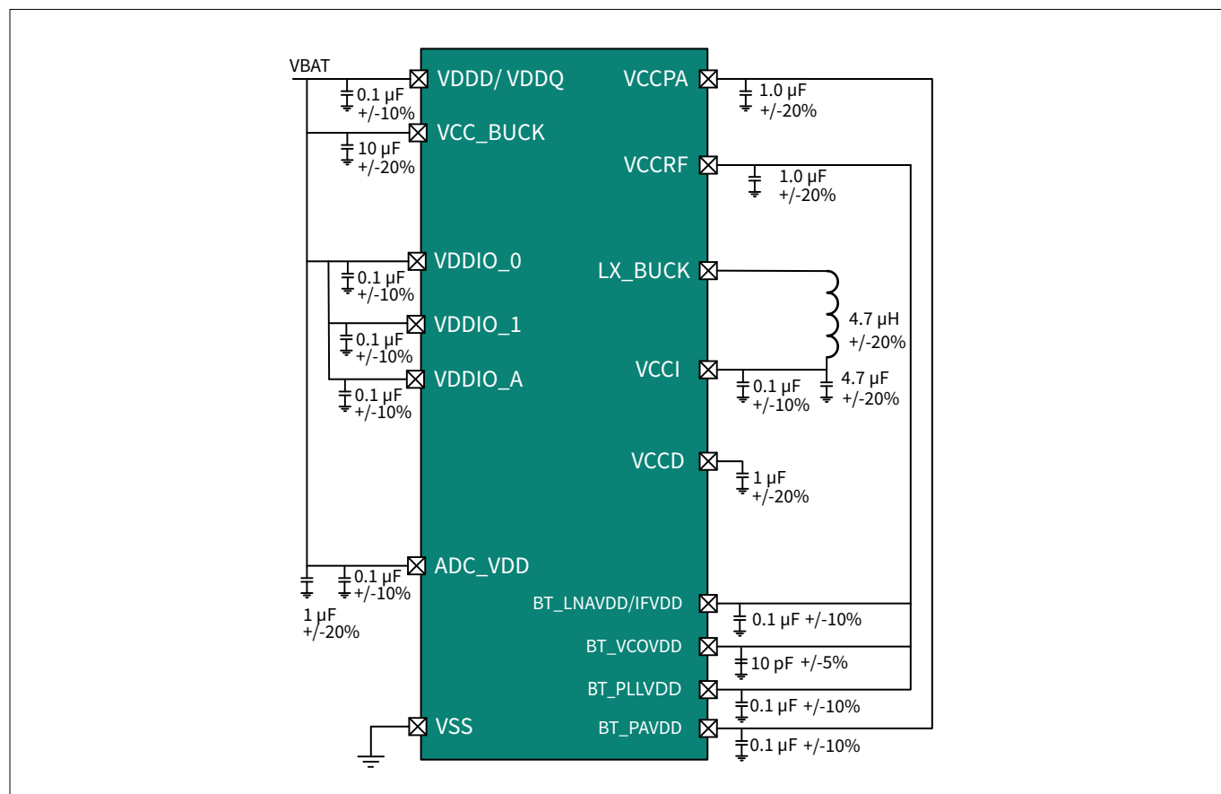
Figure 8 CYW20829 power topology
