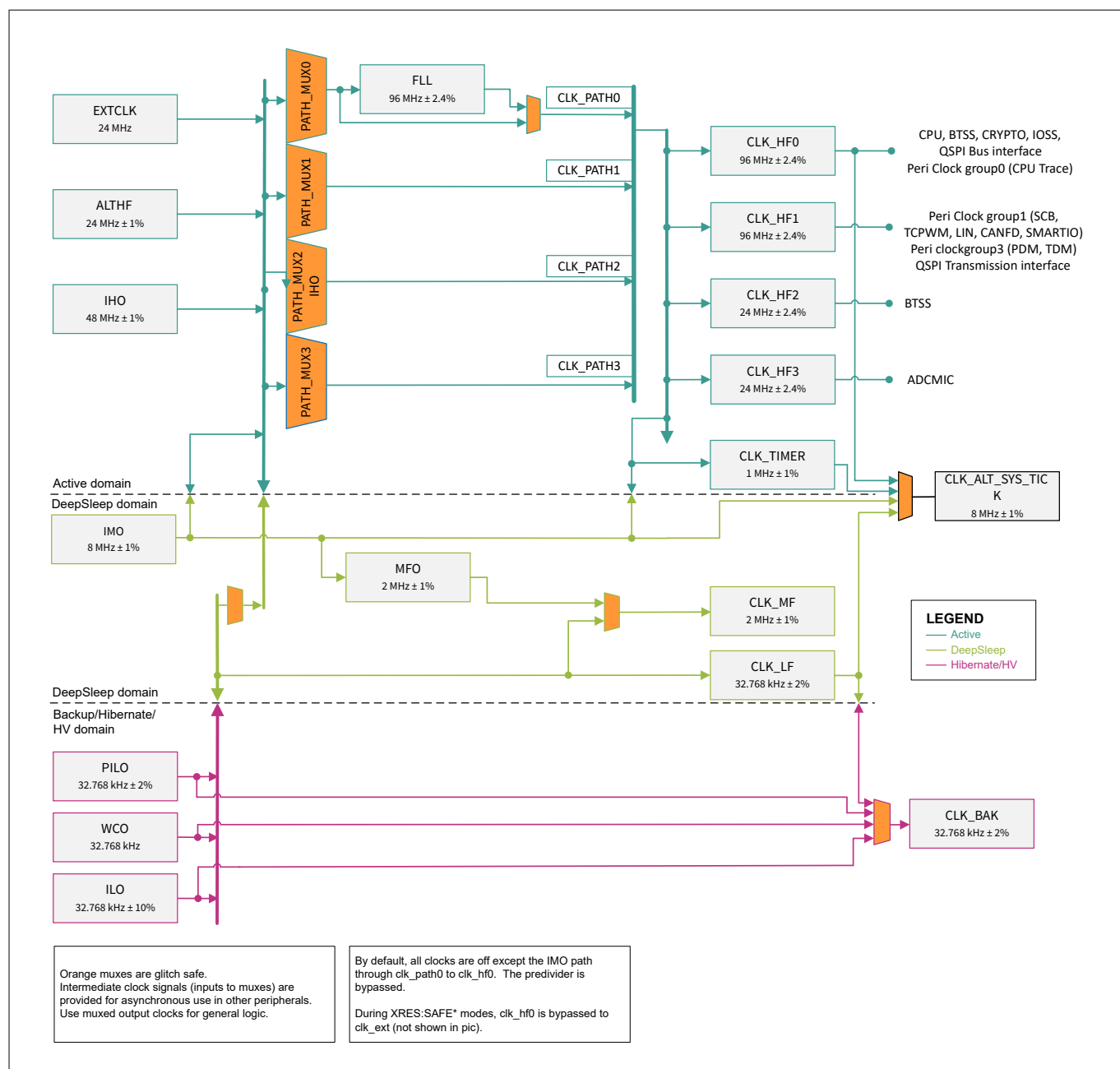
Figure 3 CYW20829 clocking diagram with corresponding oscillators
