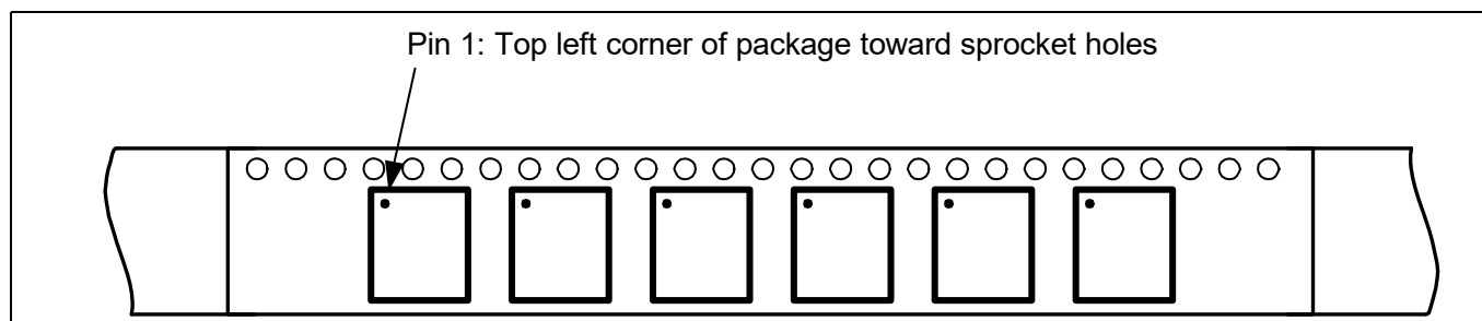
Figure 17 Pin 1 orientation
