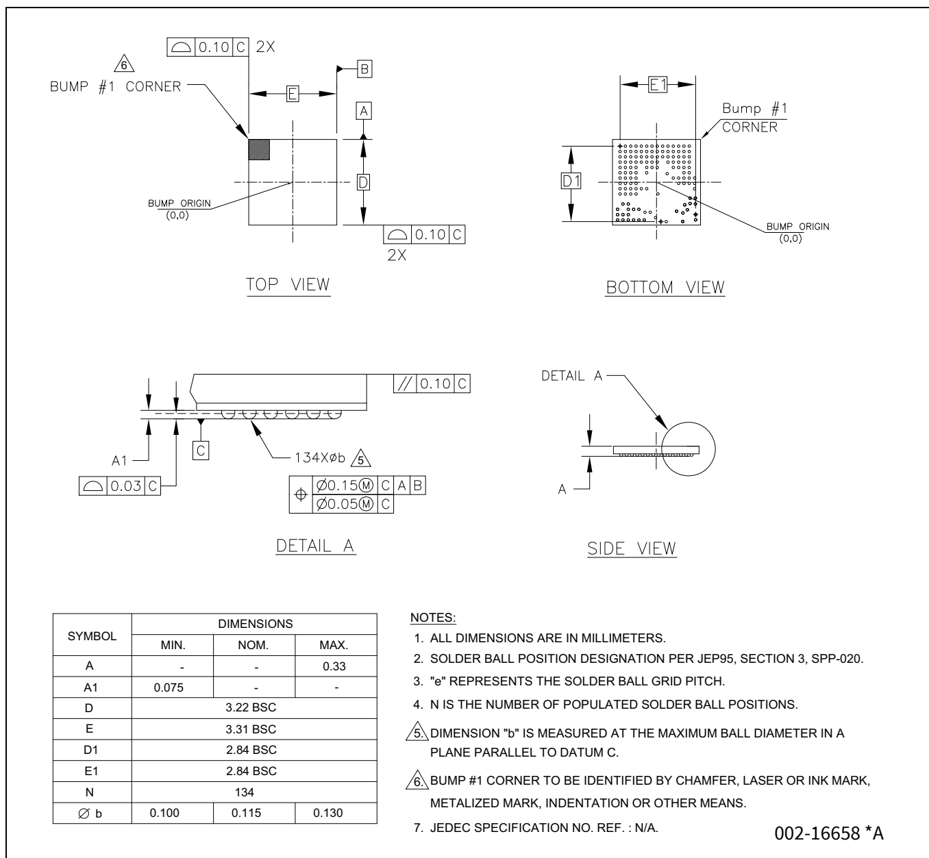
Figure 15 134-ball WLCSP (3.31 mm x 3.22 mm x 0.33 mm) (SG-XFWLB-134) package outline
