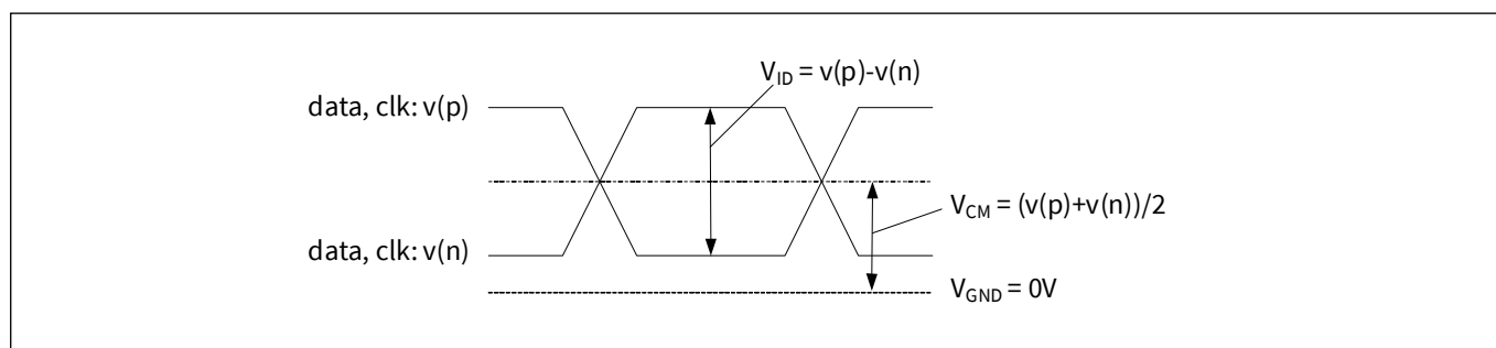
Figure 8 LVDS VCM and VID illustration
