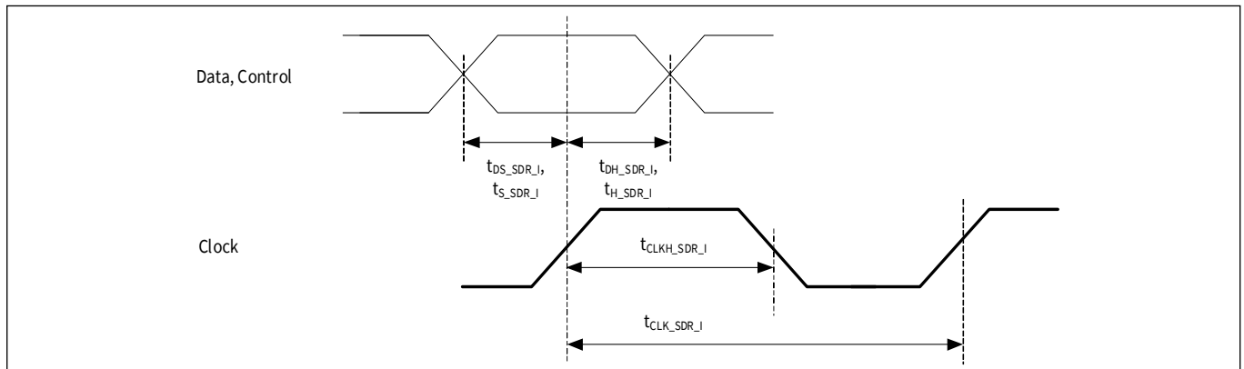
Figure 11 LVC MOS SDR input only clock and data timing
