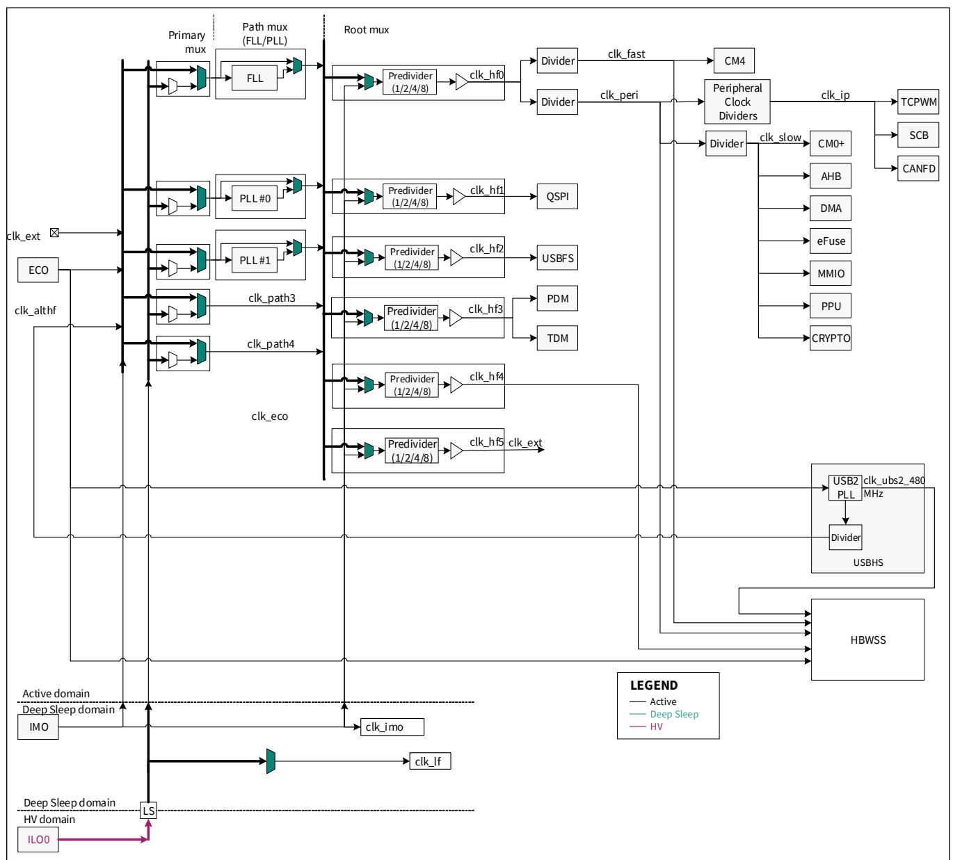
Figure 2 Clocking diagram
