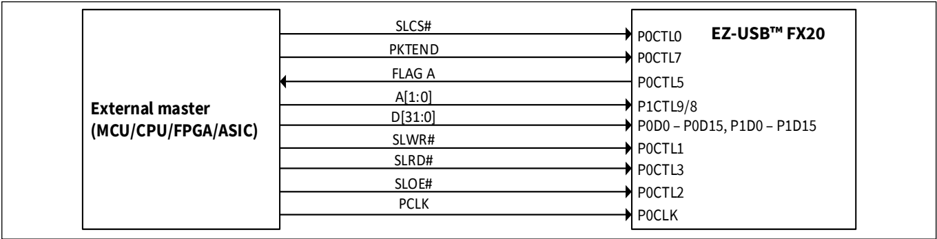
Figure 18 Slave FIFO write interface example
