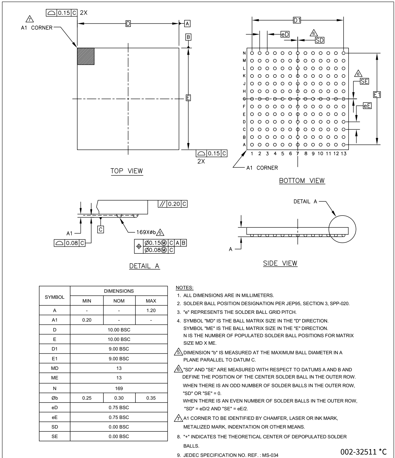
Figure 23 169-ball FBGA (10 × 10 × 1.2 mm) FCA169 package outline (PG-TFPGA-169), package outline
