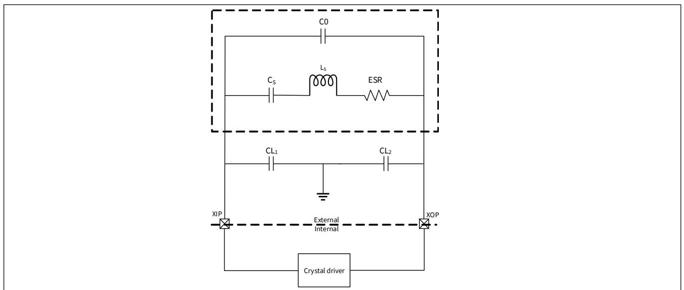
Figure 3 Oscillator circuits
