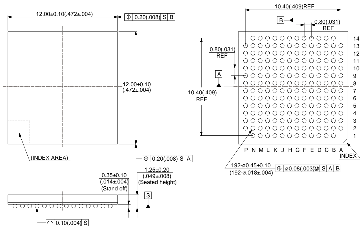
192-ball plastic FBGA (BGA-192P-M06)
