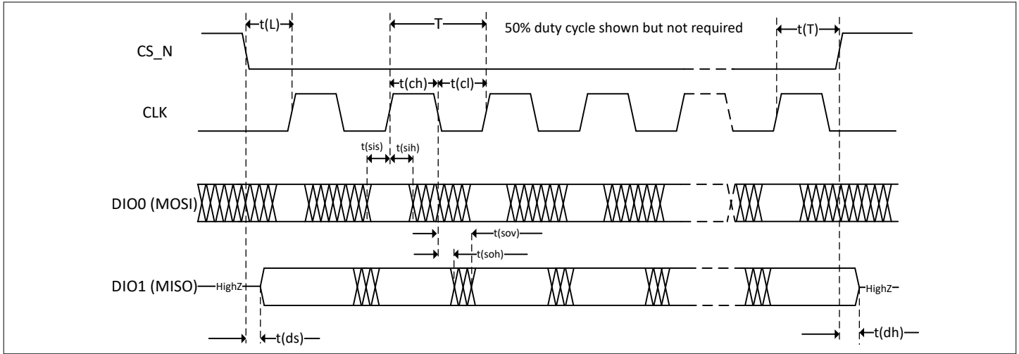
Figure 3 SPI standard timing
