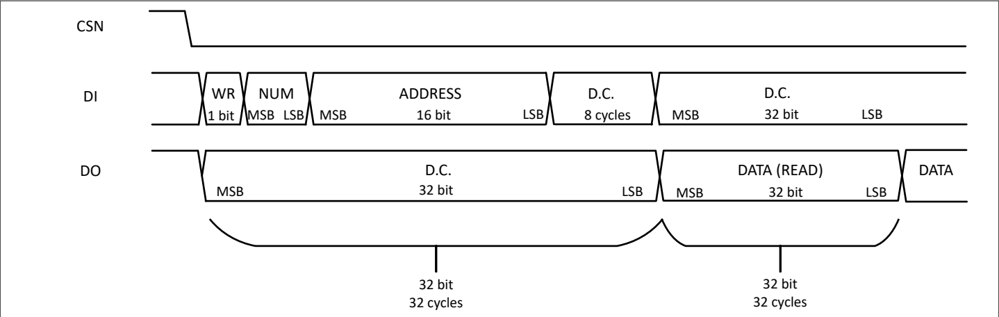
Figure 5 Standard SPI read transaction
