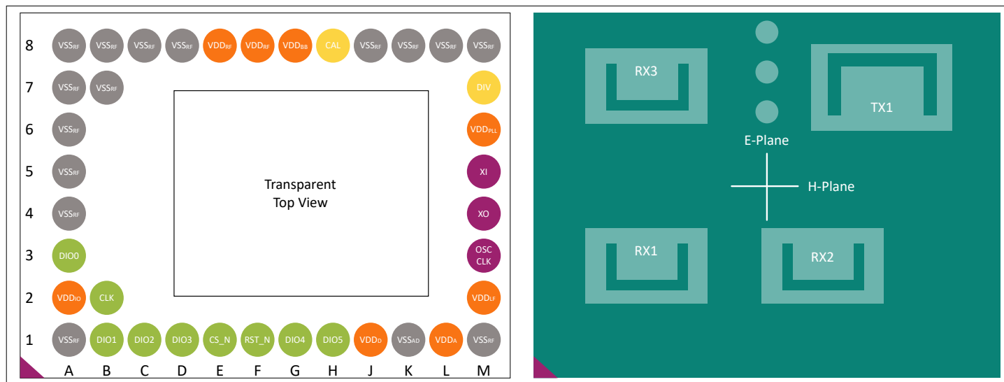
Figure 1 BGT60CUTR13AIP pin out in bottom view (left) and antenna numbers assignment in top view (right)
