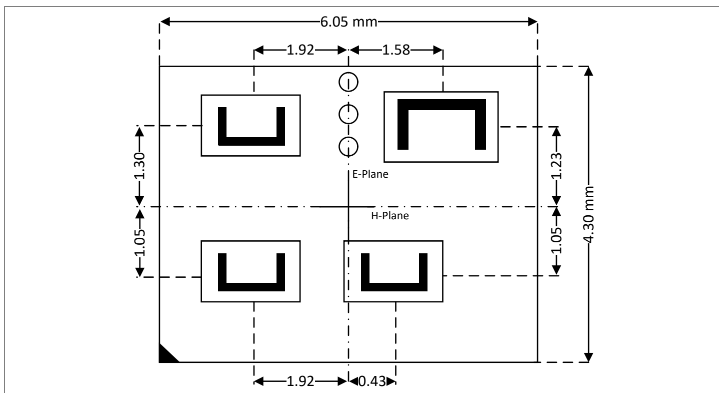
Figure 15 Device top view
