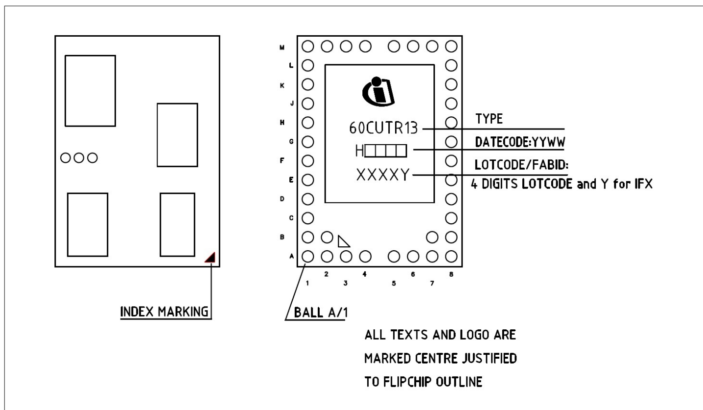
Figure 18 Marking layout of PG-VF2BGA-38-1
