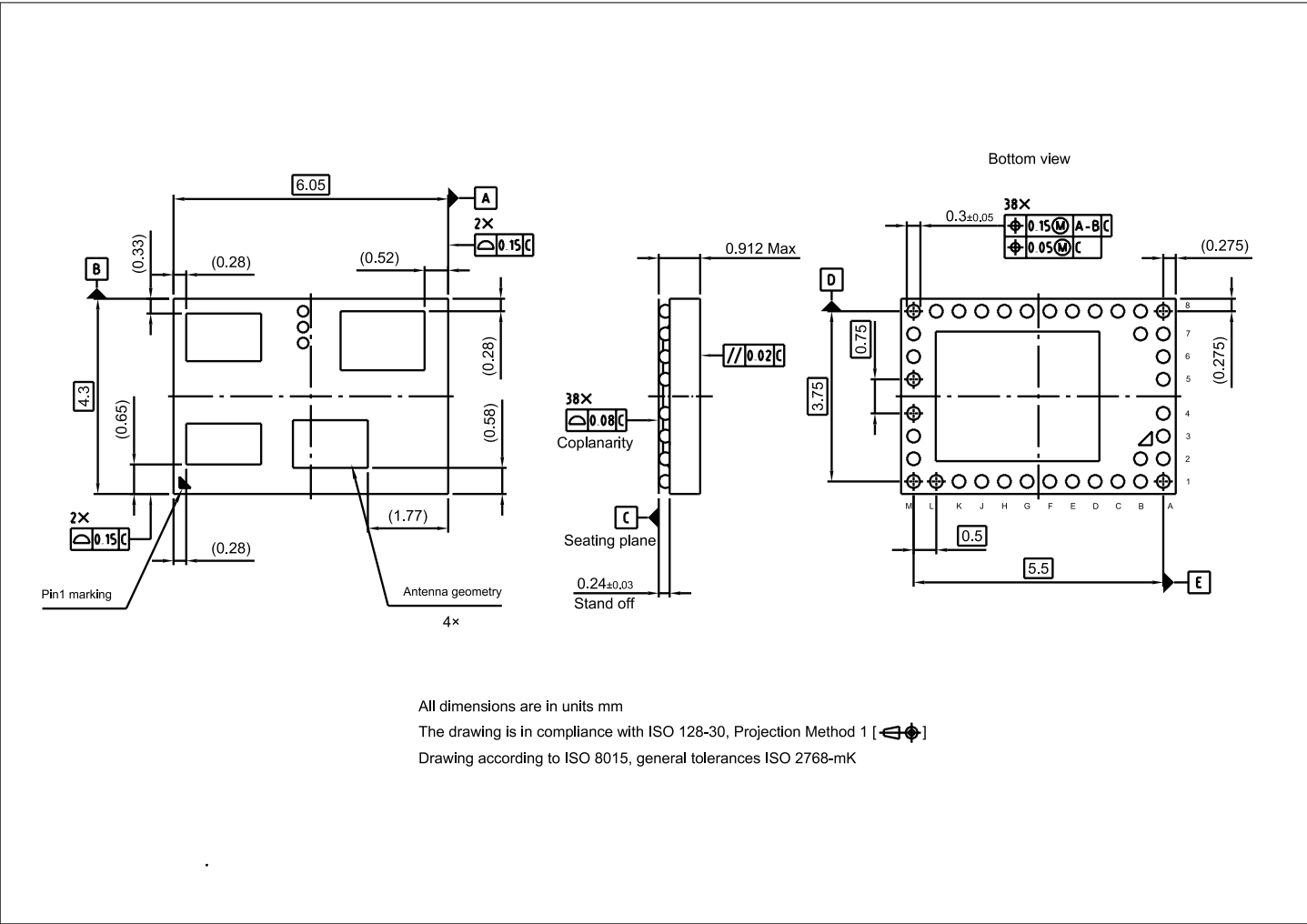
Figure 17 Package outline of PG-VF2BGA-38-1
