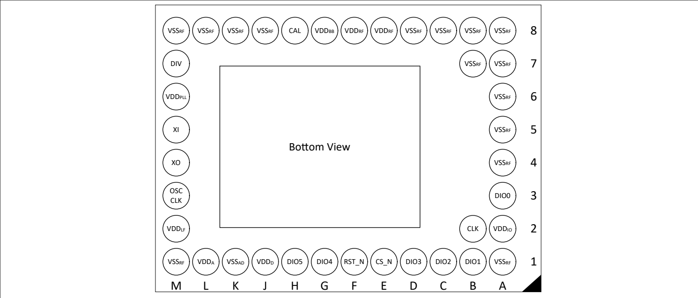
Figure 16 Device bottom view
