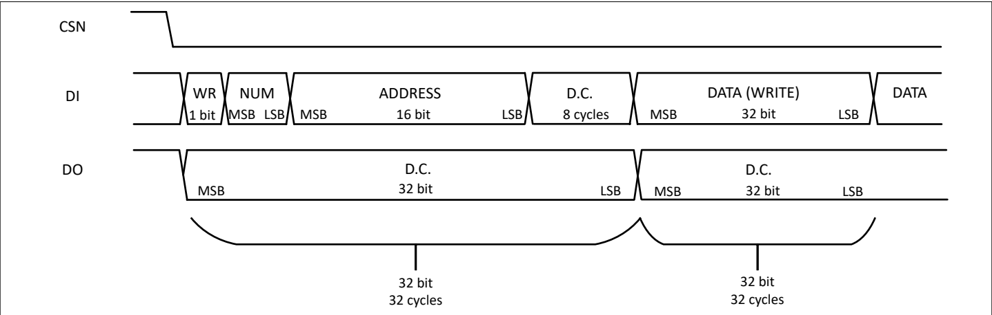
Figure 6 Standard SPI write transaction
