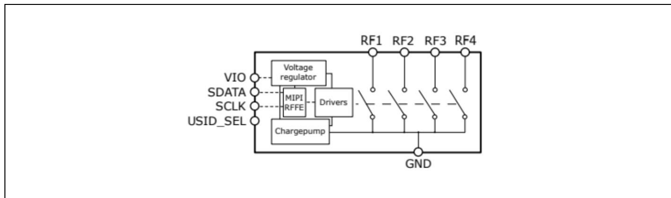
Figure 1 BGS4149M2MN10 Block diagram
