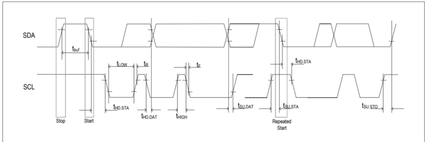
Figure 6 I²C timing diagram
