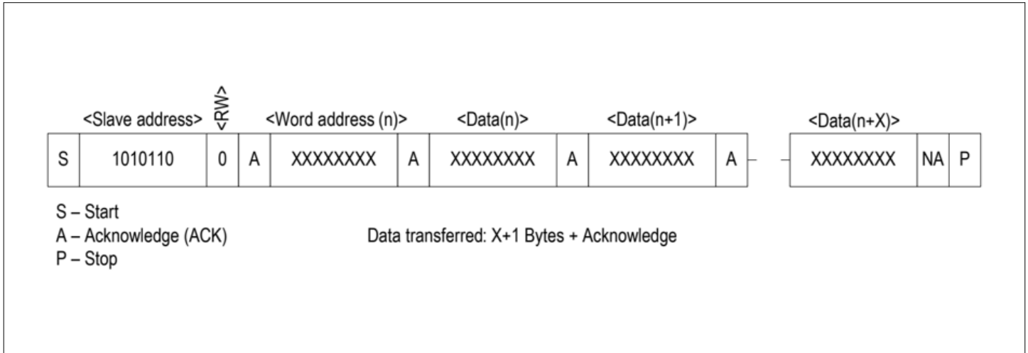
Figure 8 Data write - slave receiver mode
