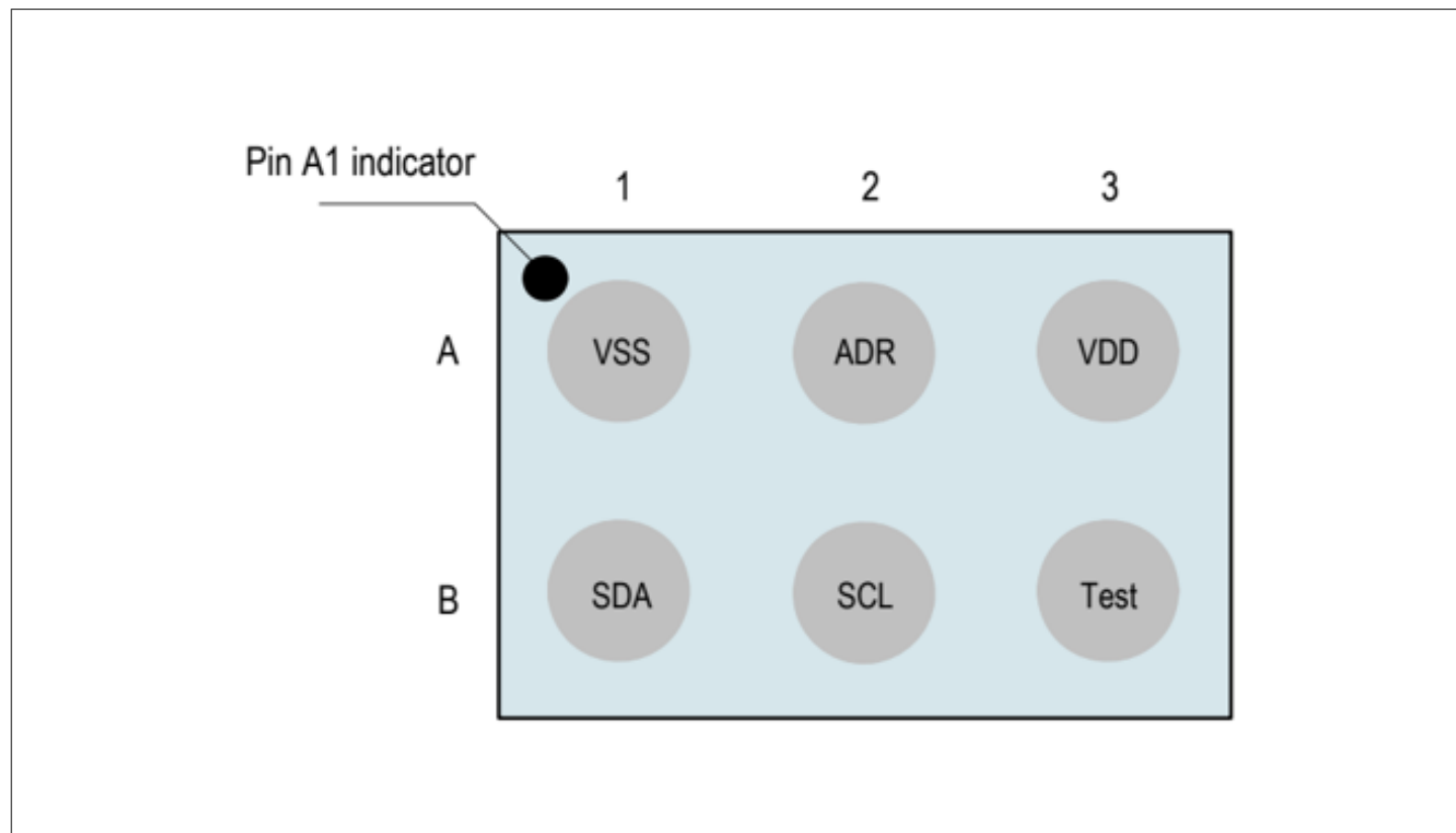
Figure 2 Pin configuration of AS5510 in WLCSP package(top view)
