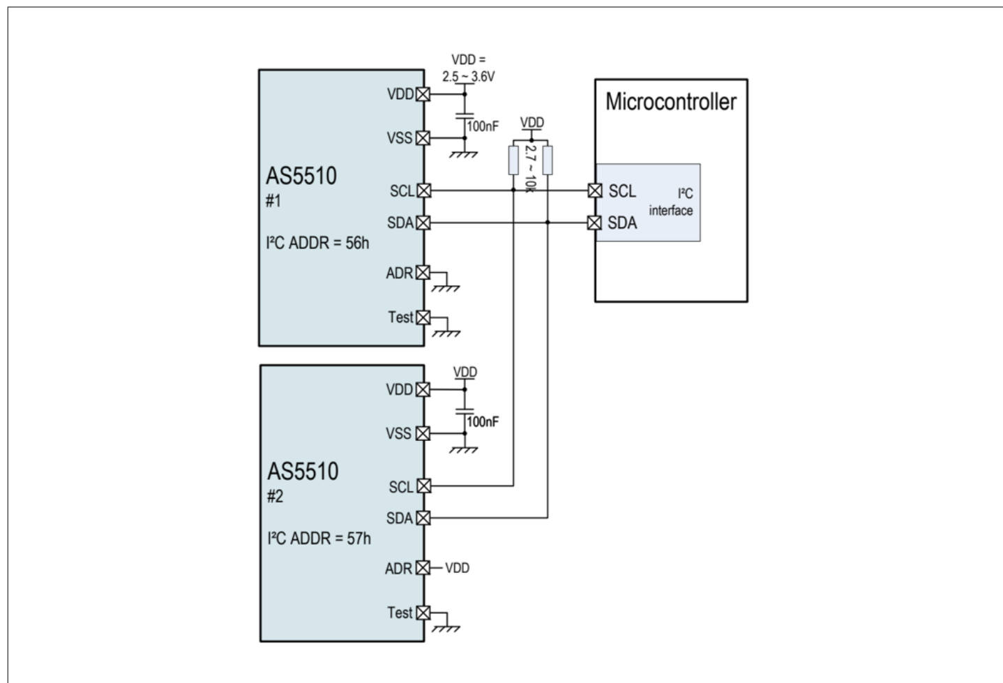
Figure 5 Typical application circuit
