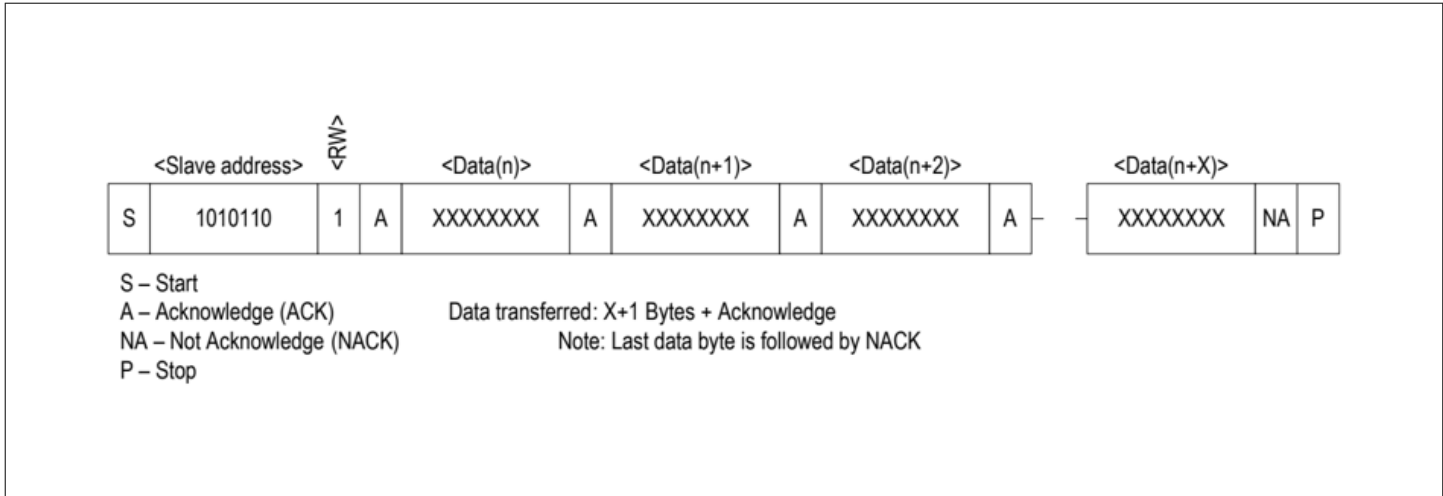
Figure 9 Data read (from current pointer location) - slave transmitter mode
