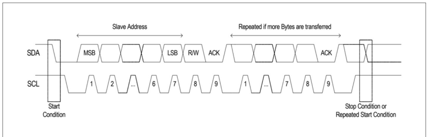
Figure 7 Data read (write pointer, then read) - slave receive and transmit
