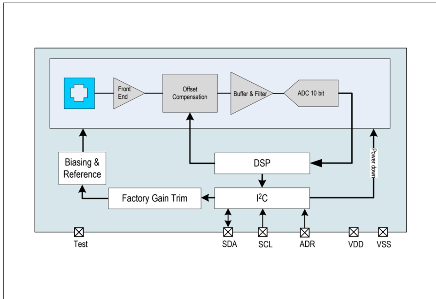
Figure 1 AS5510 Block diagram
