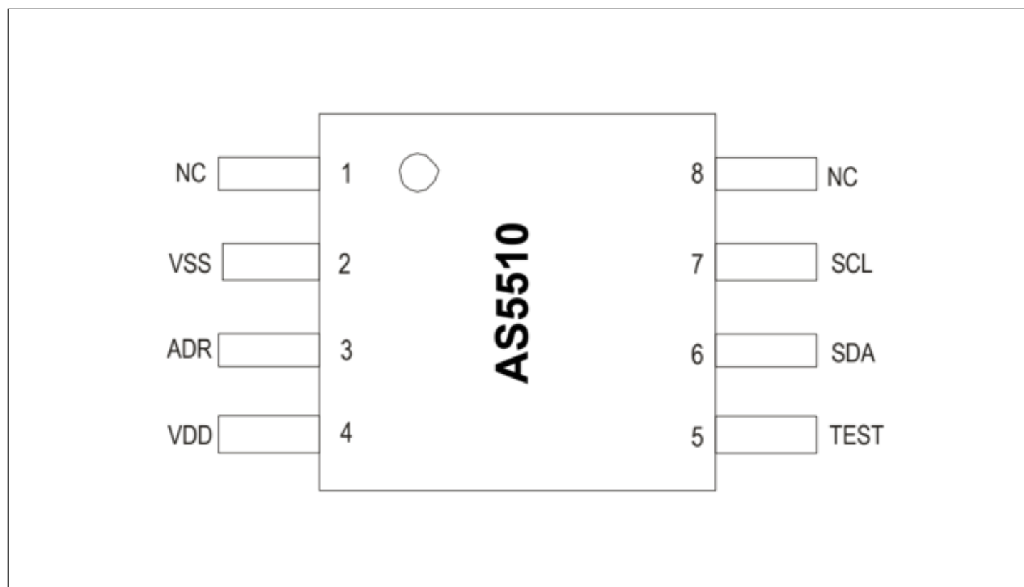
Figure 3 Pin configuration of AS5510 in SOIC8 package(top view)
