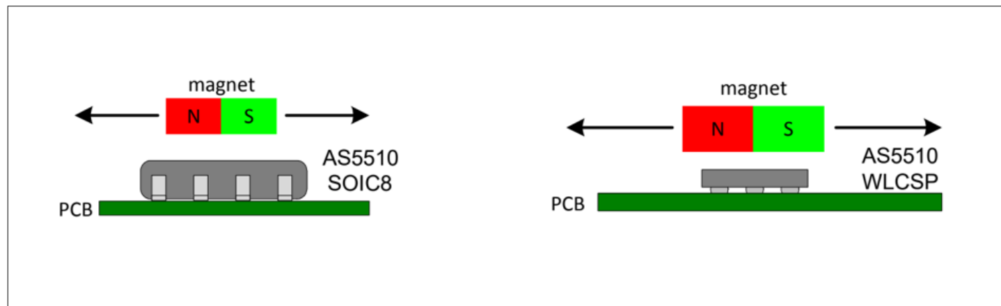
Figure 4 Linear position sensor AS5510 + magnet
