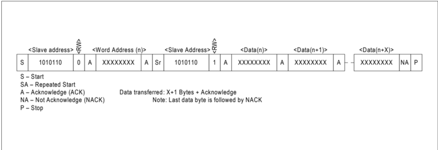
Figure 10 Data read (write pointer, then read) - slave receive and transmit
