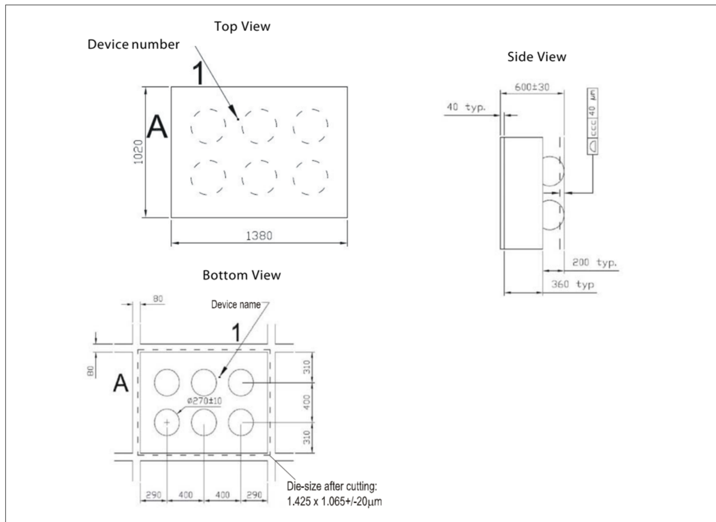
Figure 11 Package dimensions (WLCSP)
