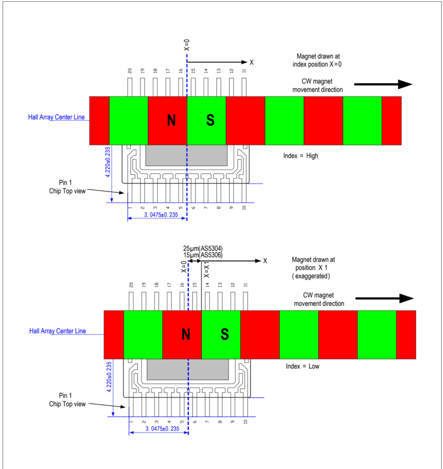
Figure 6 Magnet placement for index pulse generation
