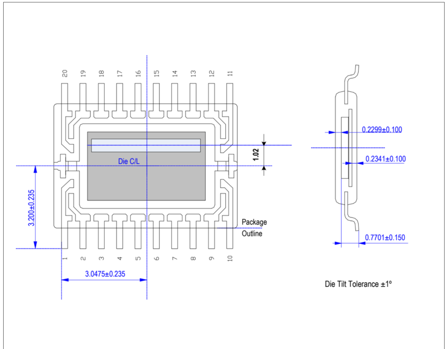
Figure 16 Sensor in package
