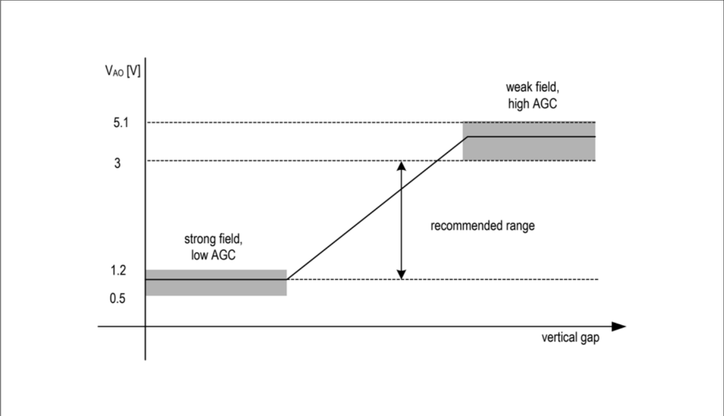
Figure 11 AO vs. AGC, magnetic field strength, magnet-to-IC gap
