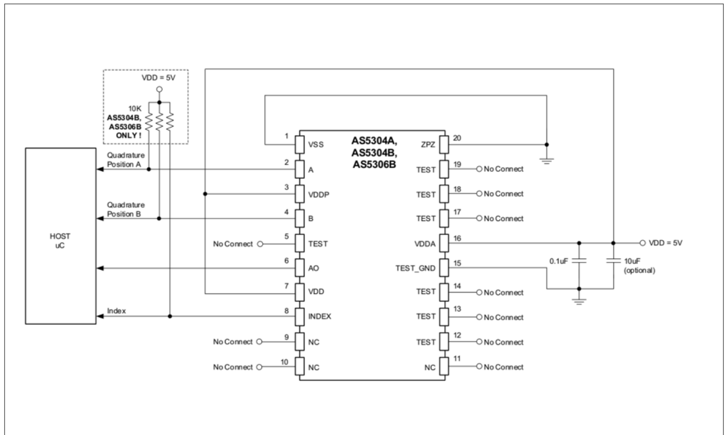
Figure 4 Electrical connection of the AS5304/AS5306
