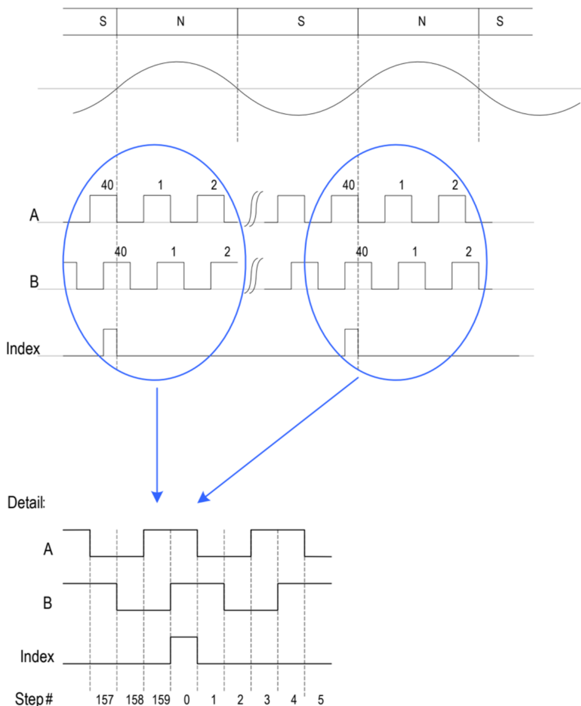
Figure 5 Quadrature A/B and index output
