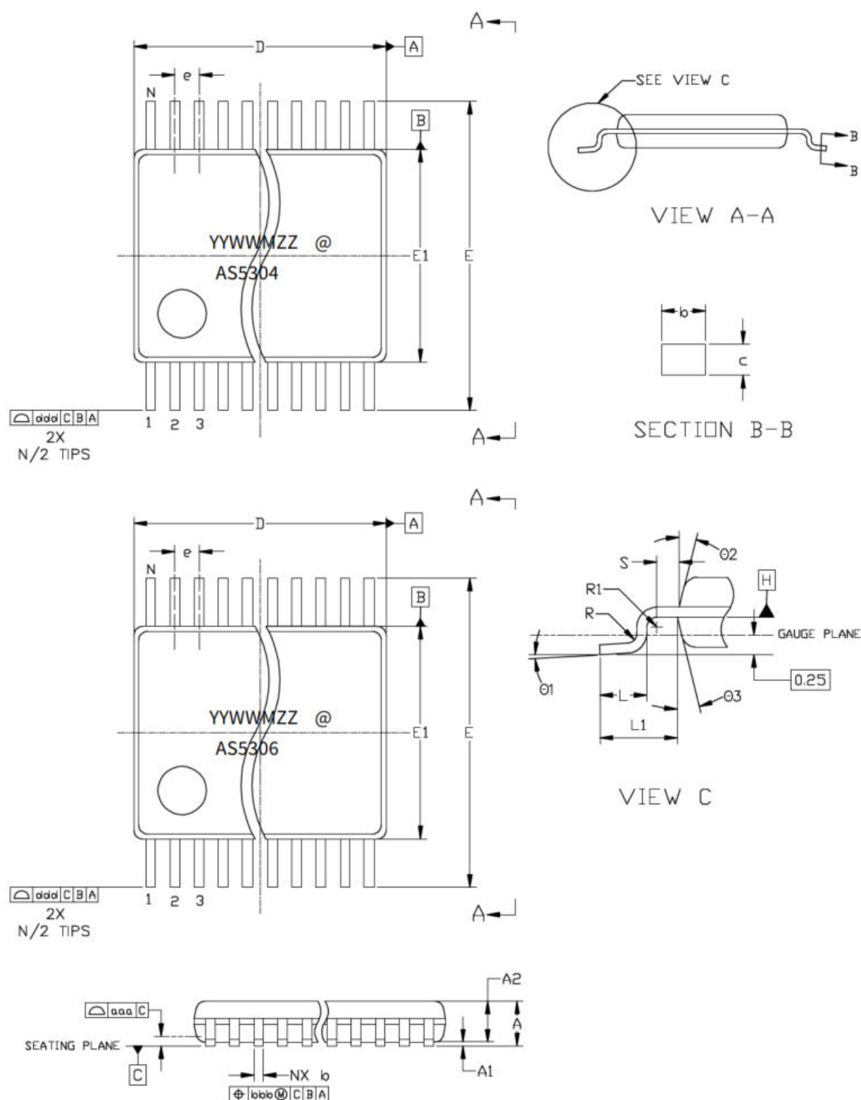
Figure 14 Packaging drawings
