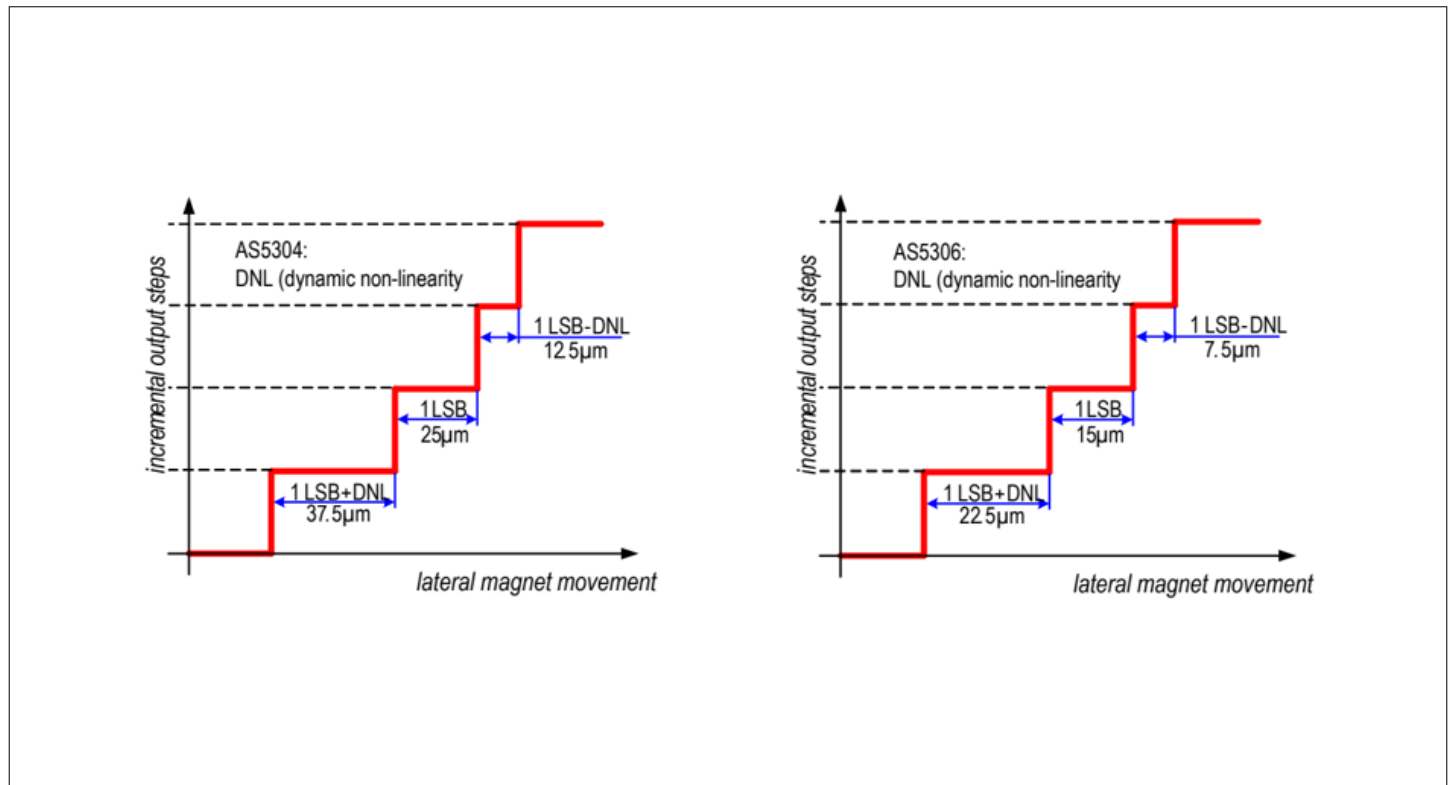
Figure 10 DNL of AS5304 (left) and AS5306 (right)
