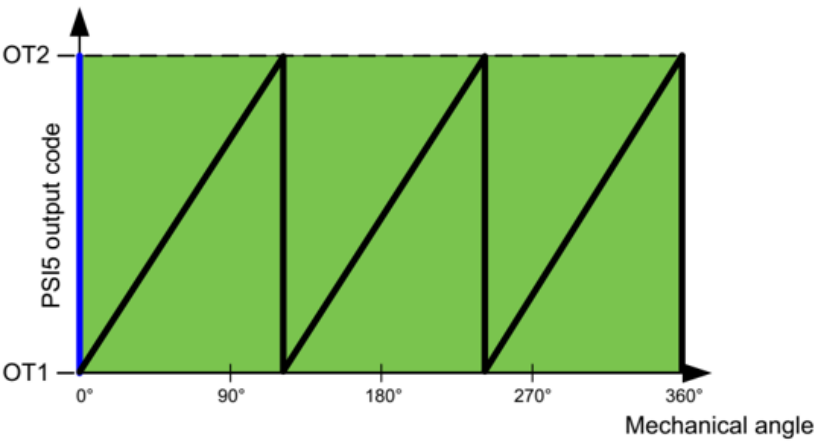
Figure 14 Triple quadrant
