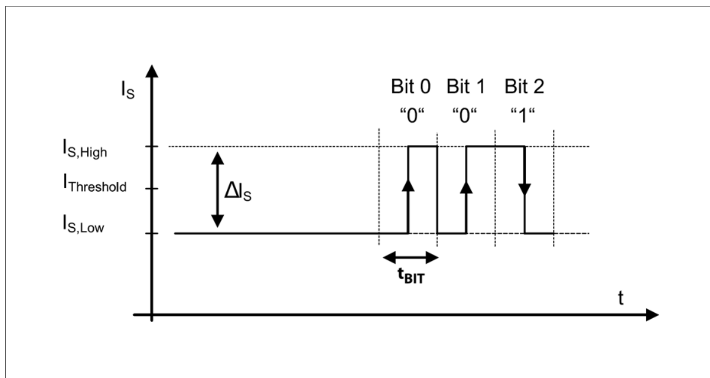
Figure 16 Bit encoding using supply current modulation
