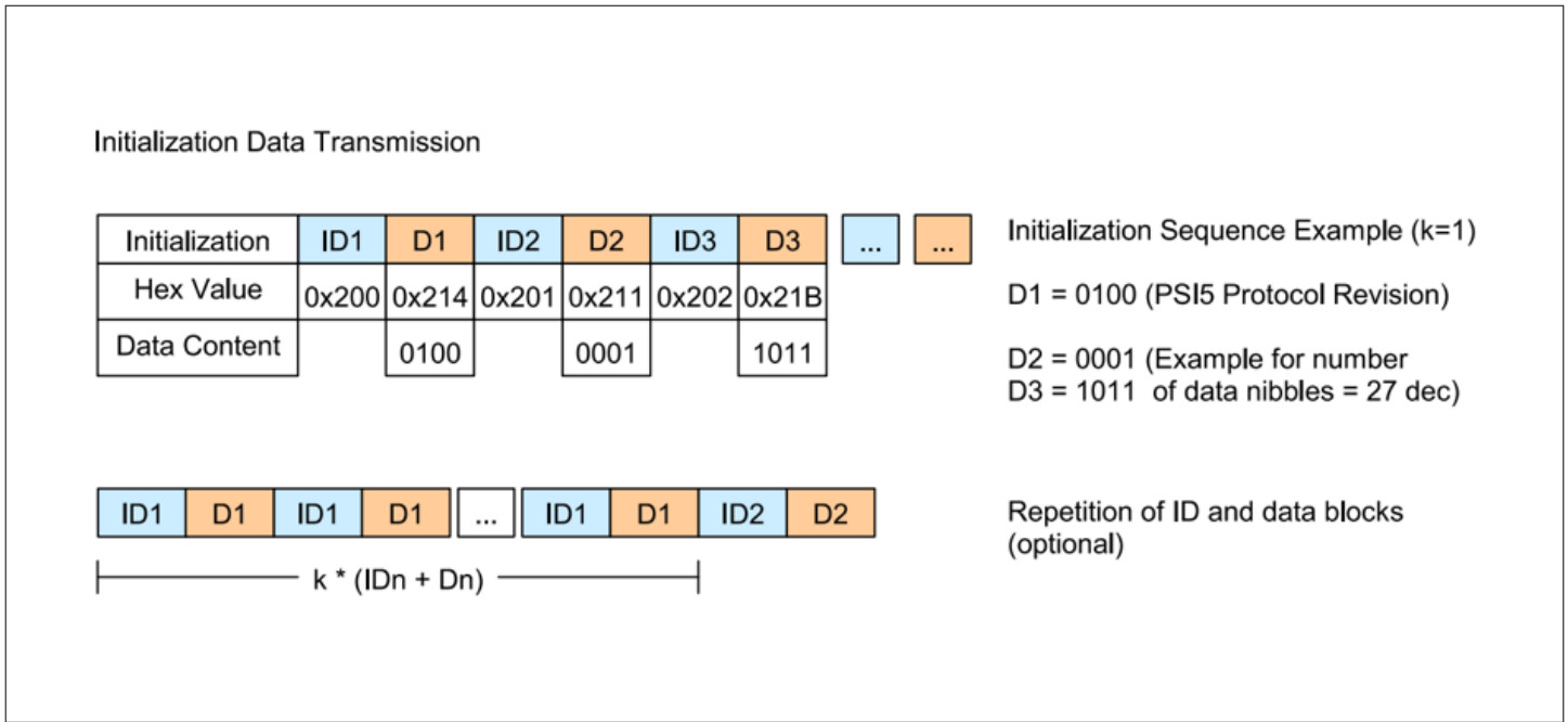
Figure 25 Startup sequence
