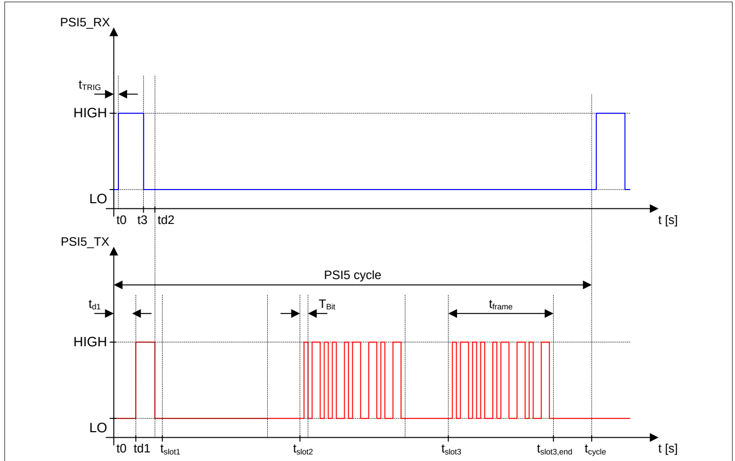
Figure 20 Synchronous mode P10P-500/3L with discharge pulse
