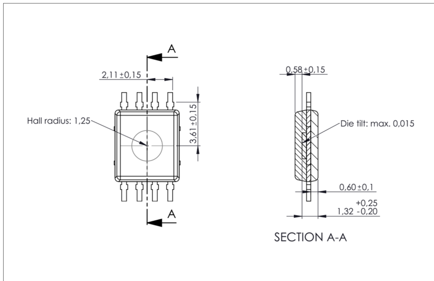
Figure 33 SIP die placement and hall array position
