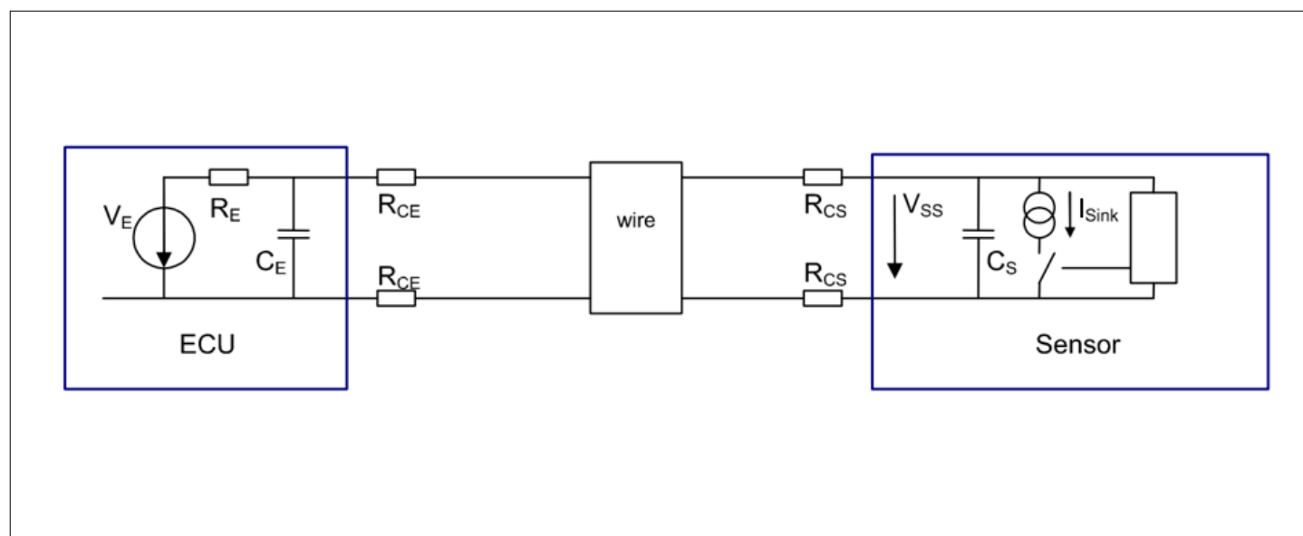
Figure 26 Asynchronous single sensor configuration
