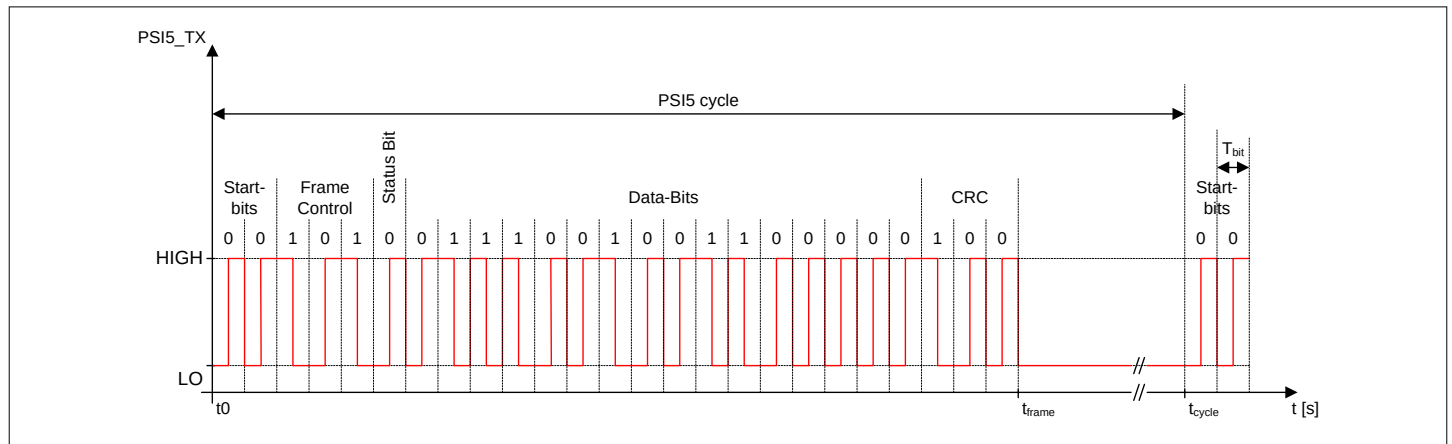
Figure 22 Asynchronous modes A20CRC-200/1H and A20CRC-300/1L
