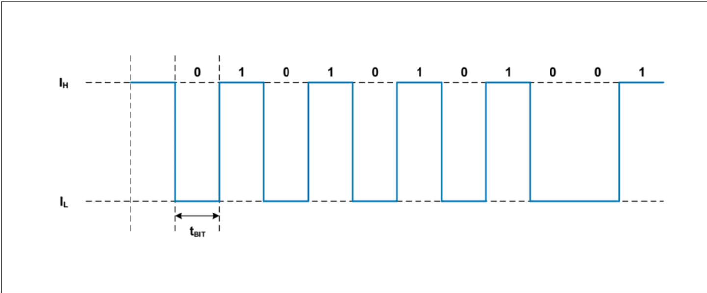
Figure 7 Bit encoding of sensor-to-programmer communication
