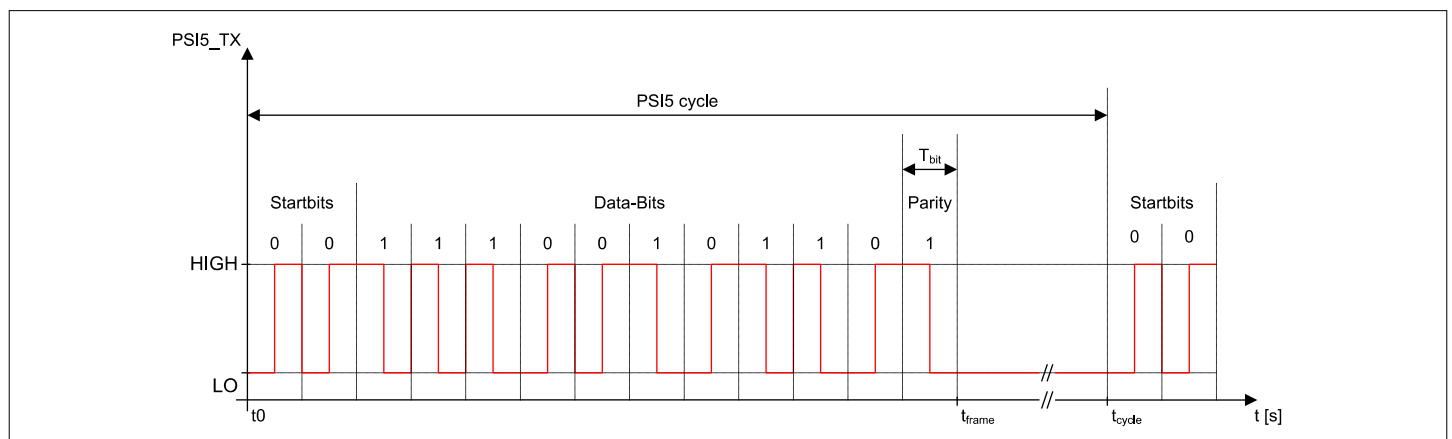
Figure 21 Asynchronous modes A10P- 50/1L and A10P-500/1L
