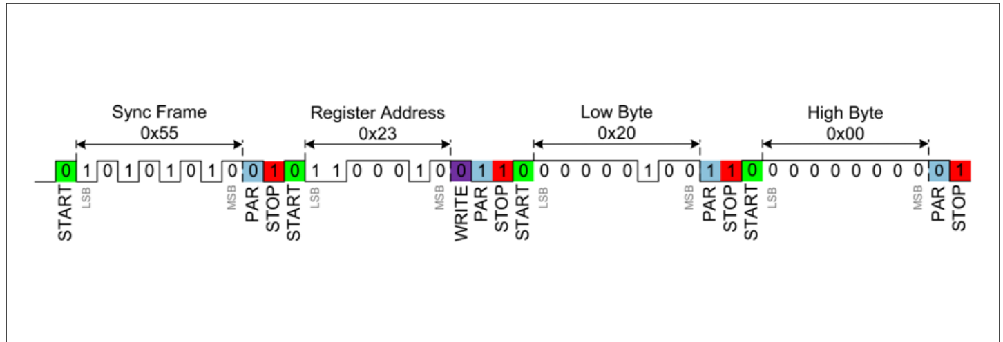
Figure 9 Example of WRITE (Reg[0x23] = 0x20 and Reg [0x24] = 0x00)
