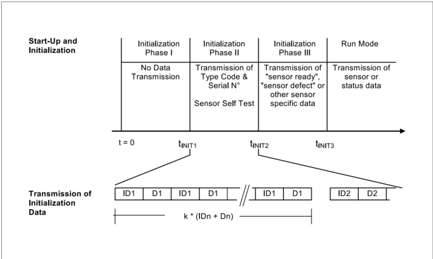
Figure 23 Start-up and initialization
