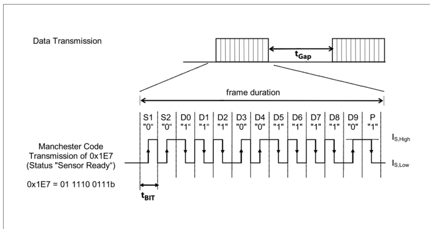
Figure 17 Example of a 10-bit data frame
