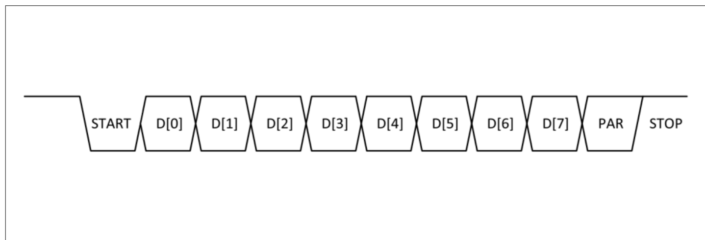
Figure 8 UART protocol frame
