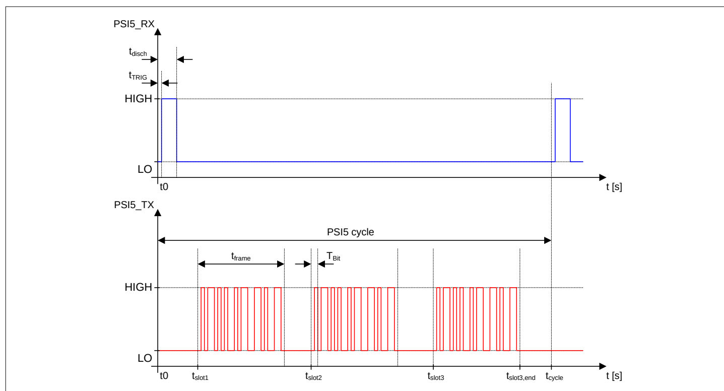
Figure 19 Synchronous mode P10P-500/3L
