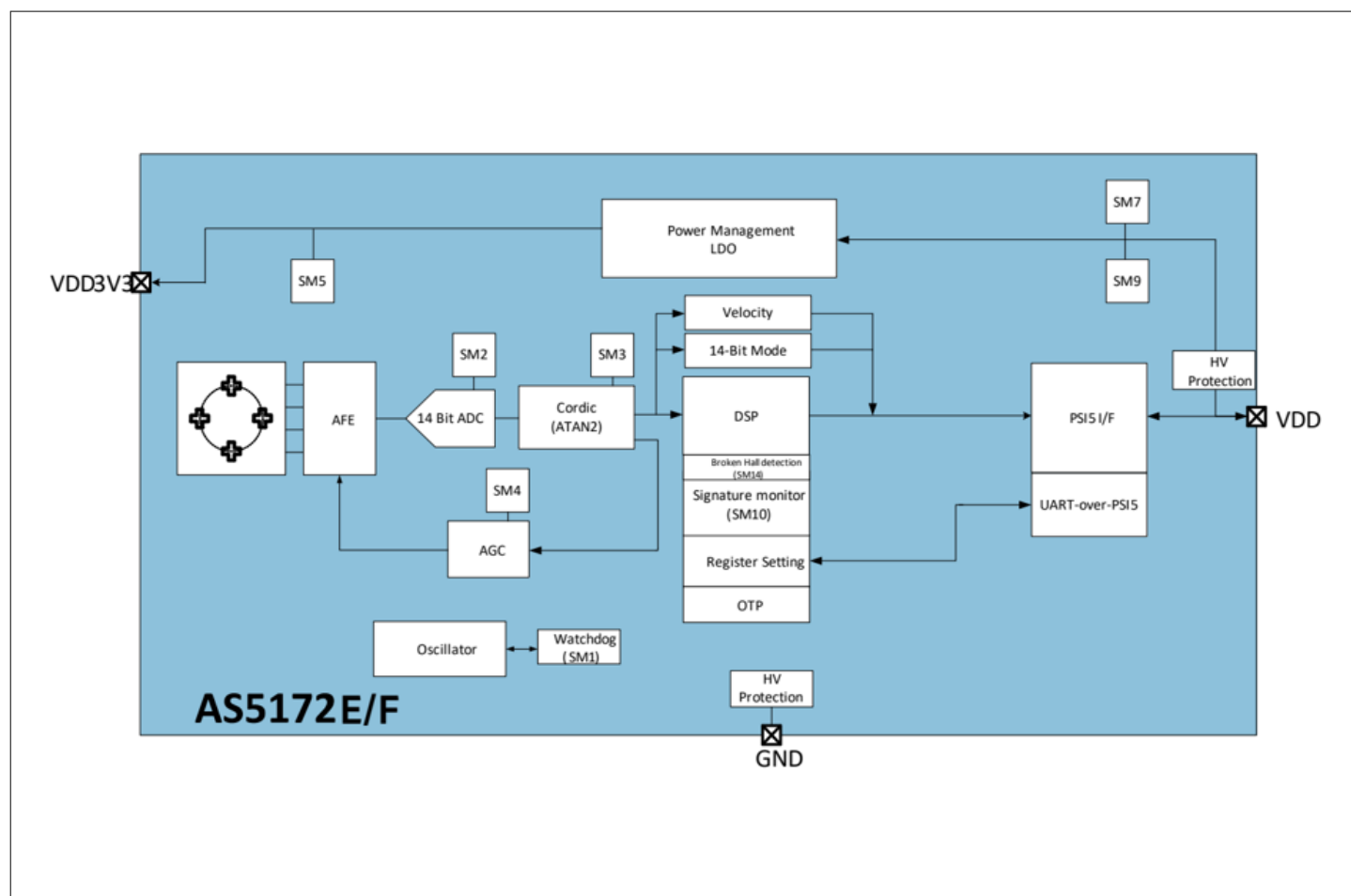
Figure 1 Functional blocks of the AS5172E/F
