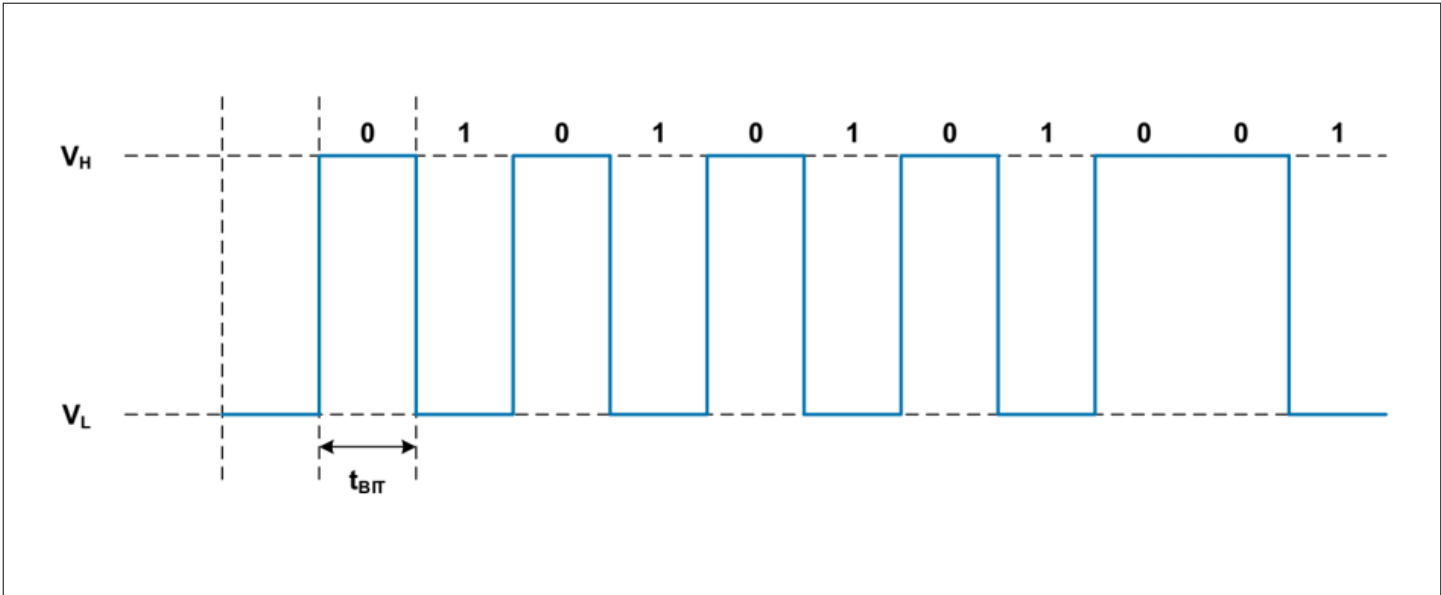
Figure 6 Bit encoding of programmer-to-sensor communication
