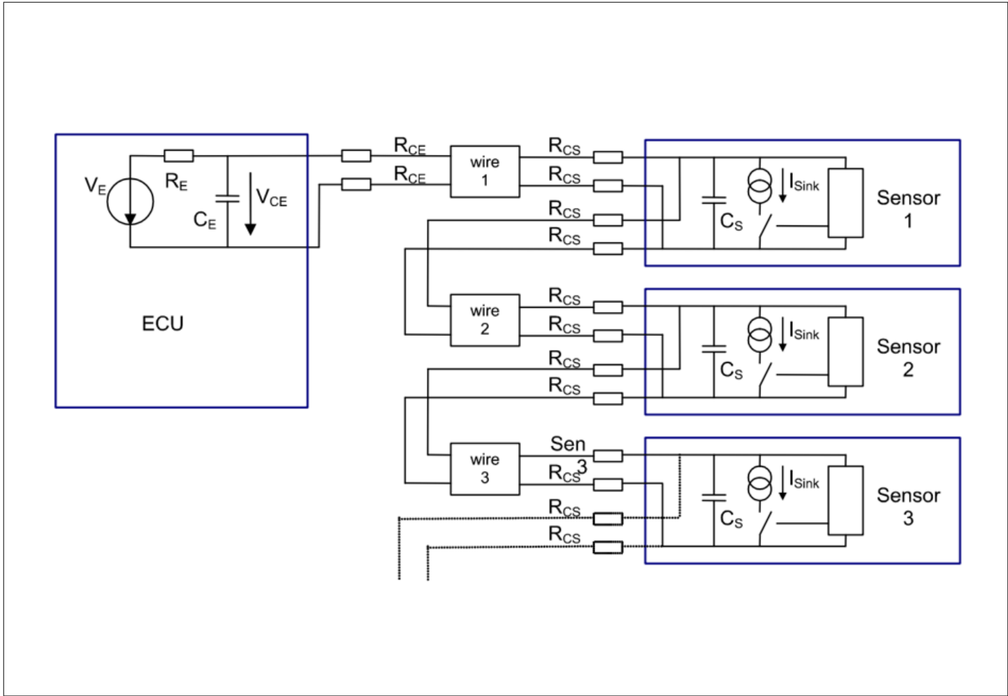
Figure 28 Synchronous universal bus mode (PSI5-U)
