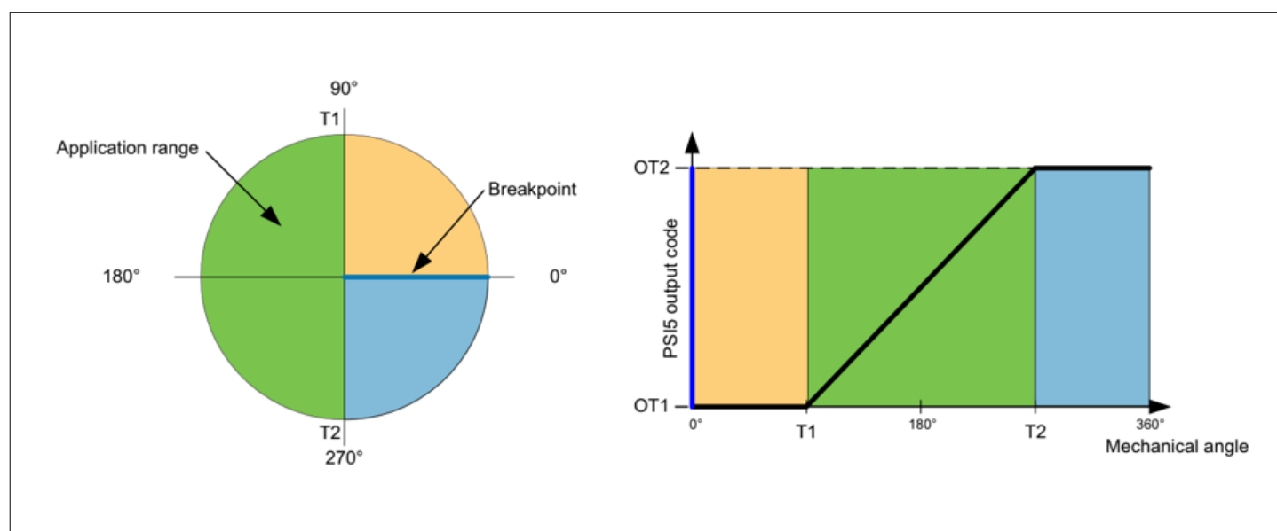
Figure 11 Transfer function
