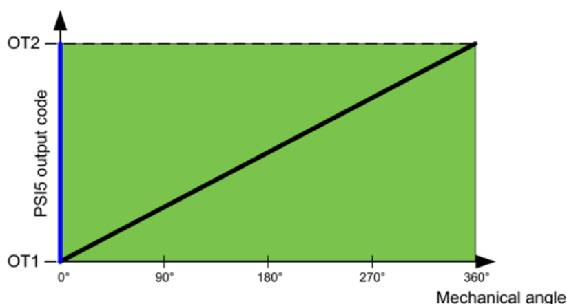
Figure 12 Single quadrant
