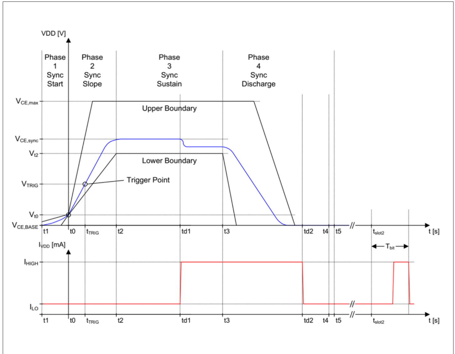
Figure 5 Synchronization signal from ECU with discharge by the AS5172E/F
