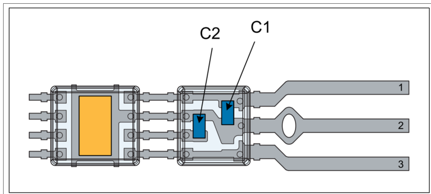
Figure 29 AS5172E/F components
