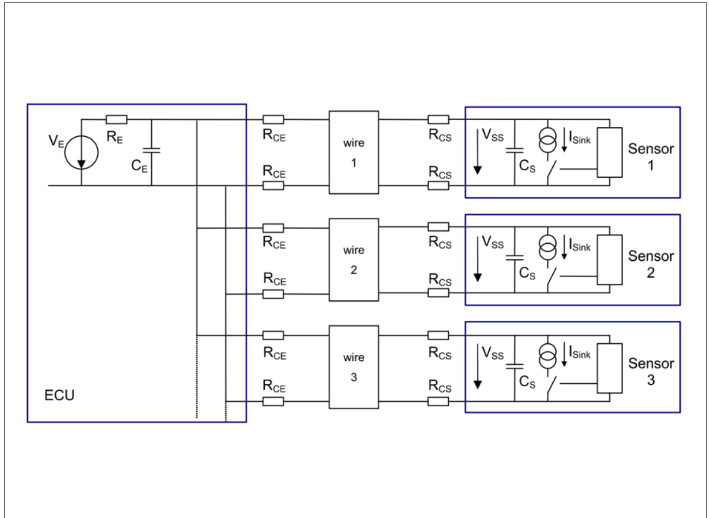
Figure 27 Synchronous parallel bus mode (PSI5-P)
