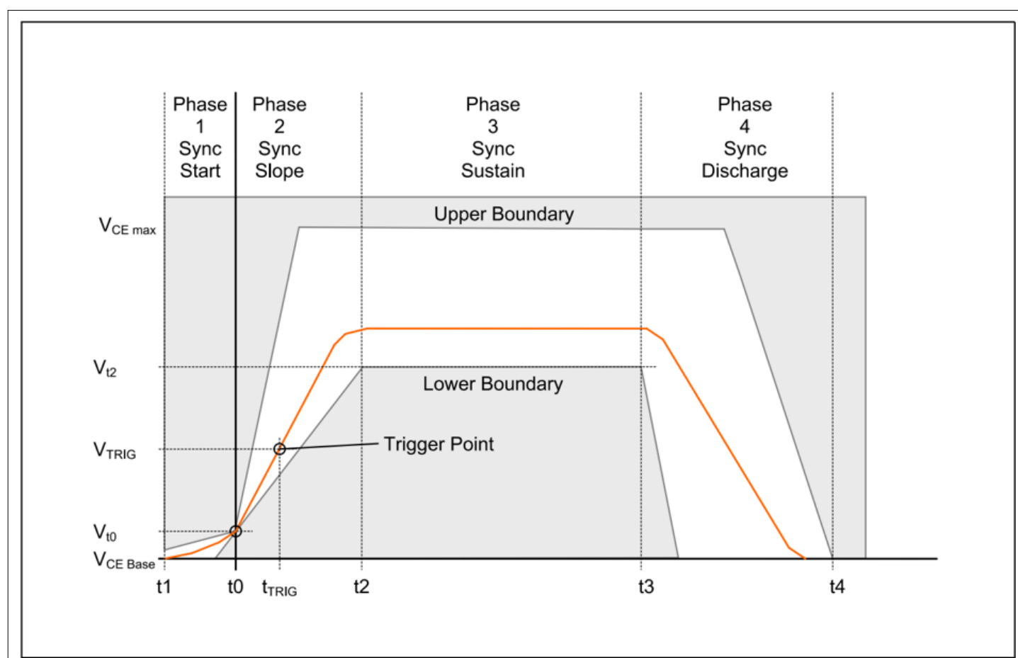
Figure 3 Synchronization signal
