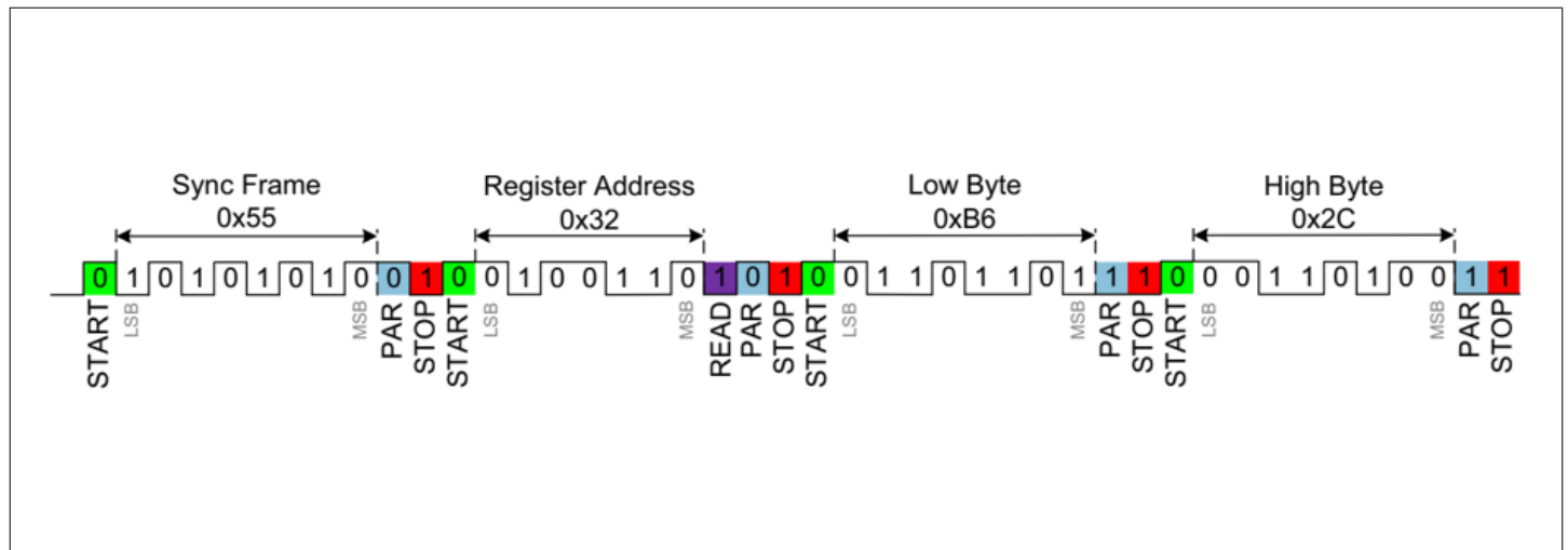
Figure 10 Example of READ (Reg[0x32] = 0xB6 and Reg [0x33] = 0x2C)
