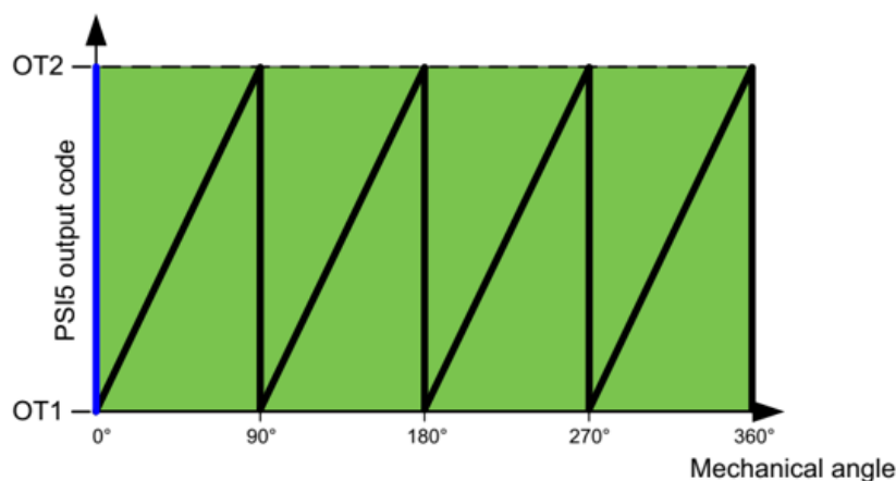
Figure 15 Quadruple quadrant
