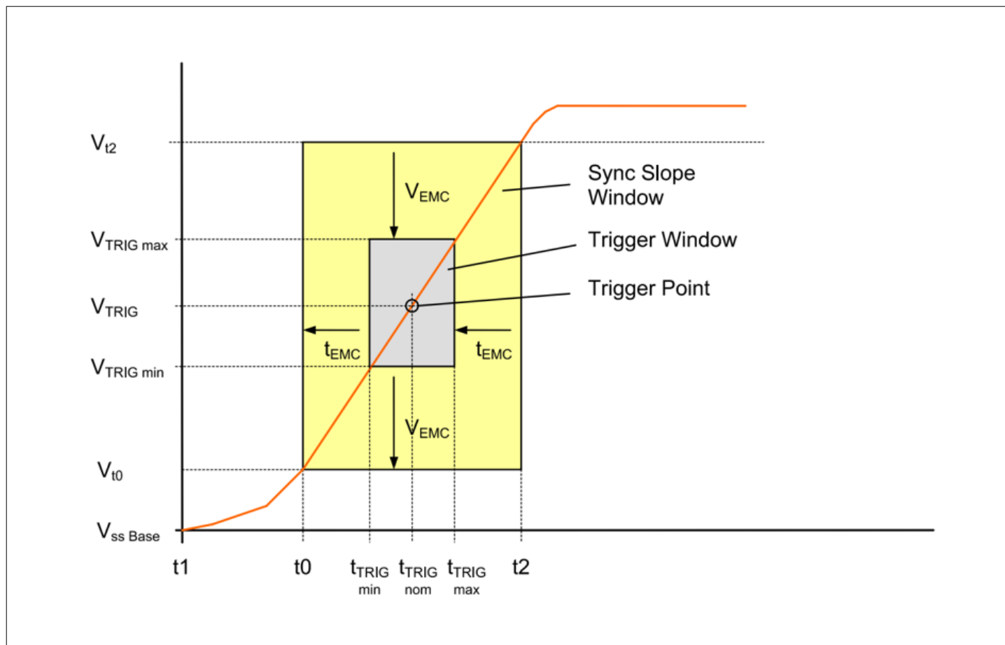
Figure 4 Trigger window
