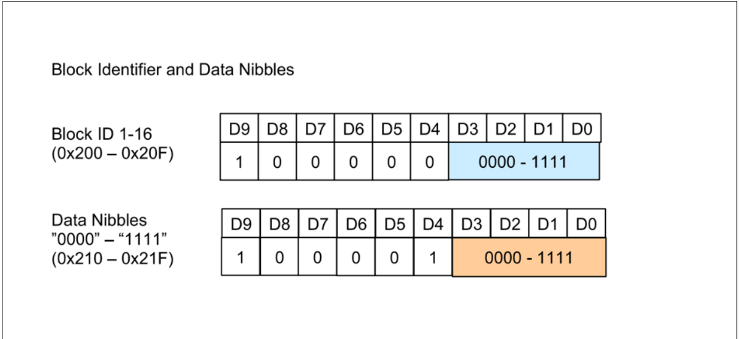
Figure 24 Block ID and data nibbles
