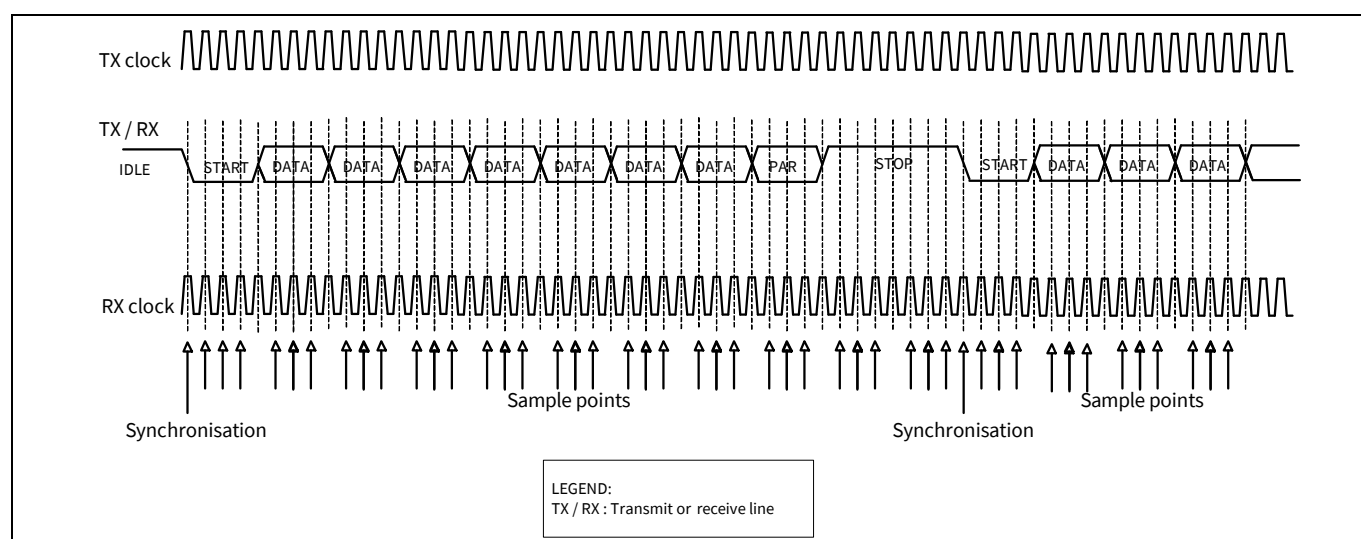
Figure 23-22. UART, standard protocol (multiple samples)
