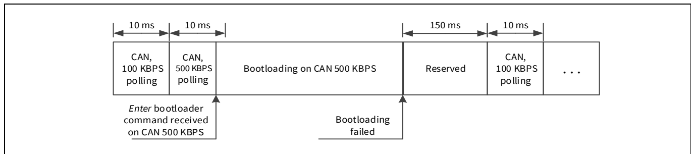
Figure 36-5. An example of a failed bootloading
