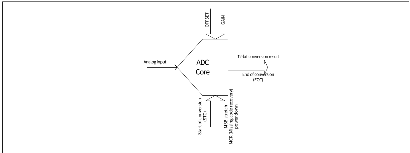
Figure 33-2. ADC core block diagram
