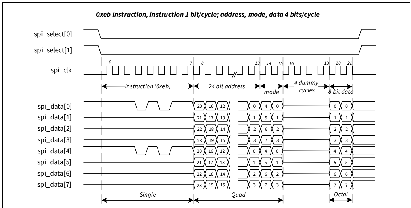
Figure 30-20. 0xeb instruction, instruction 1-bit/cycle; Address, mode, data 4-bits/cycle
