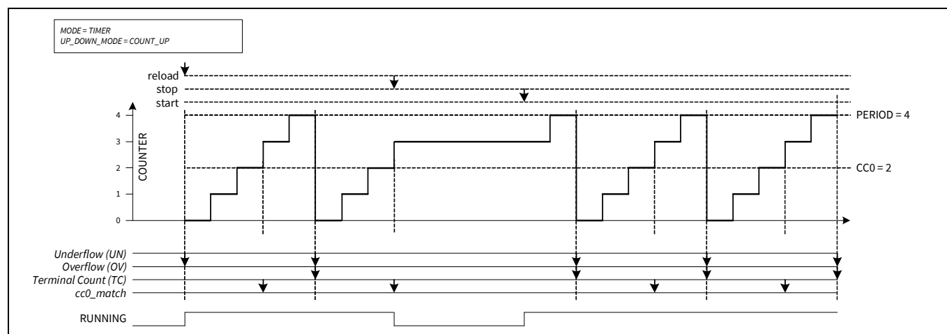
Figure 25-12. Counter start/stopped/continued
