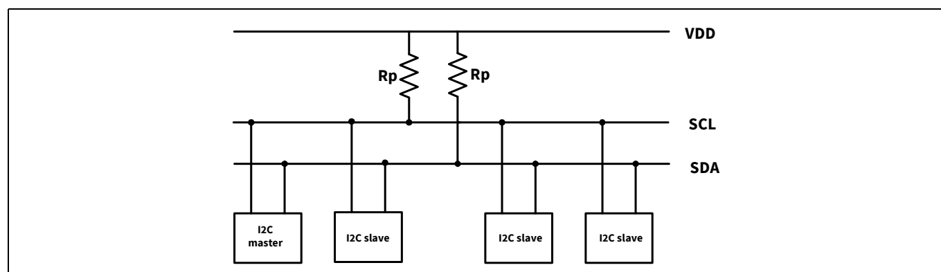
Figure 23-36. I 2 C interface block diagram
