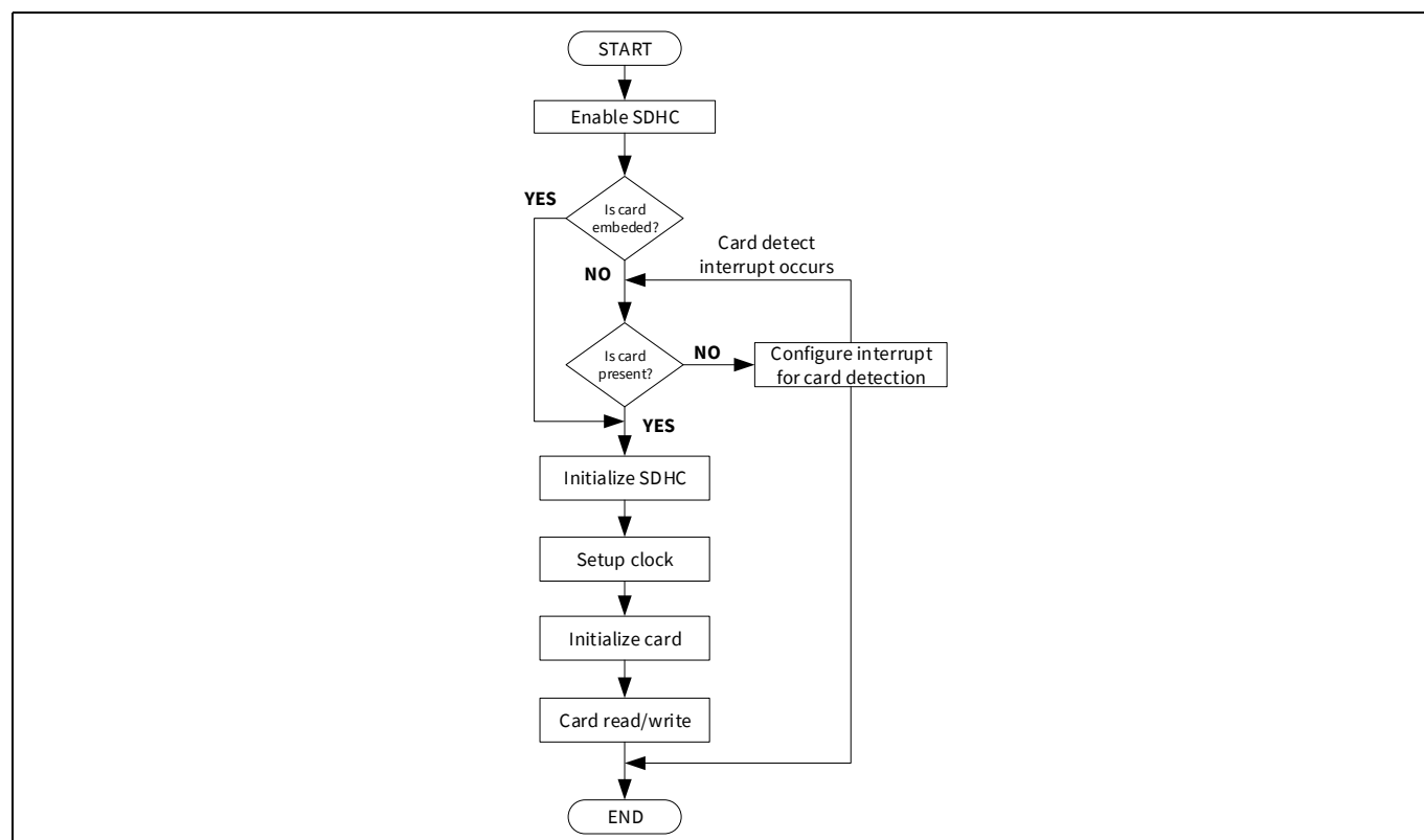
Figure 31-5. SDHC programming sequence
