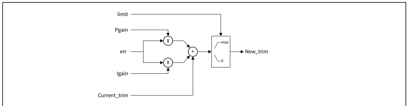
Figure 18-6. FLL error correction diagram
