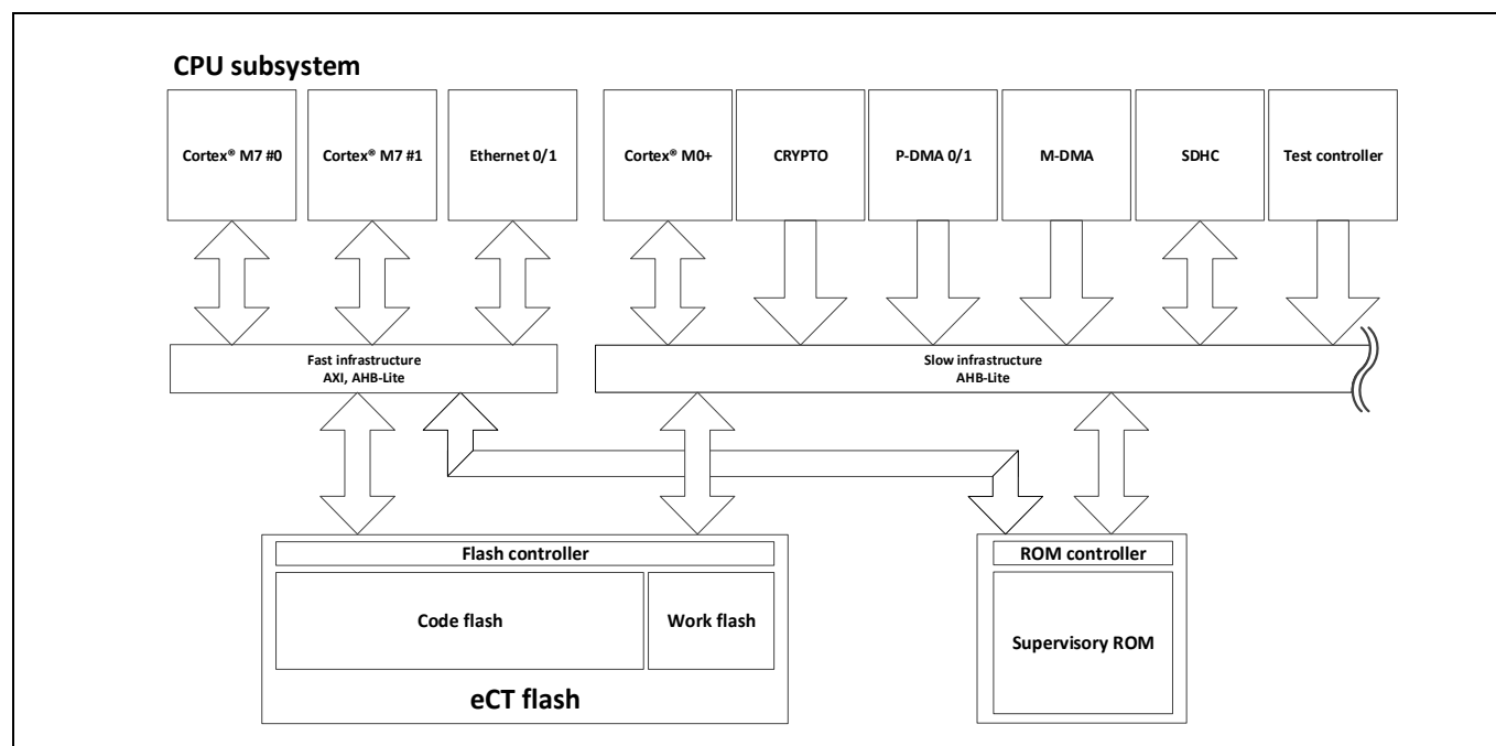
Figure 9-1. Position of work flash
