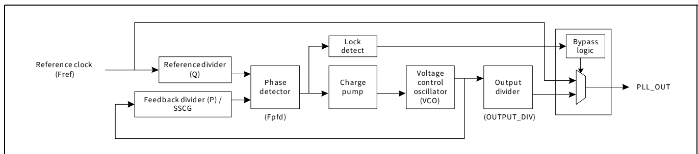
Figure 18-4. PLL with SSCG and fractional operation
