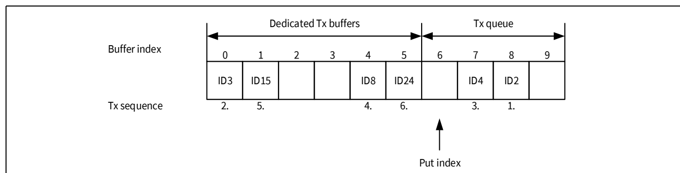
Figure 24-13. Example of mixed configuration dedicated TX buffers/TX queue
