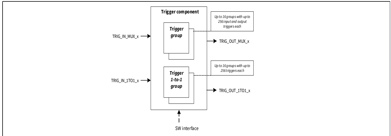
Figure 28-2. Trigger configuration parameters
