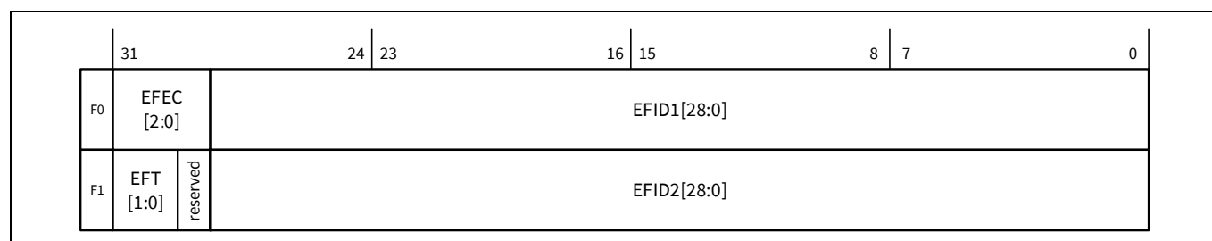
Figure 24-22. Extended message ID filter
