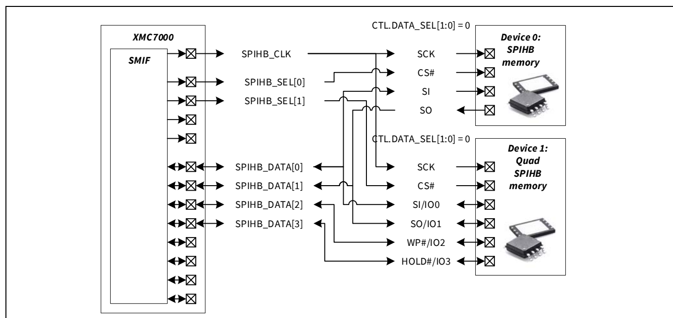
Figure 30-15. Single SPI device 0 to SPIHB_DATA[1:0], Quad SPI device 1 connected to SPIHB_DATA[3:0]
