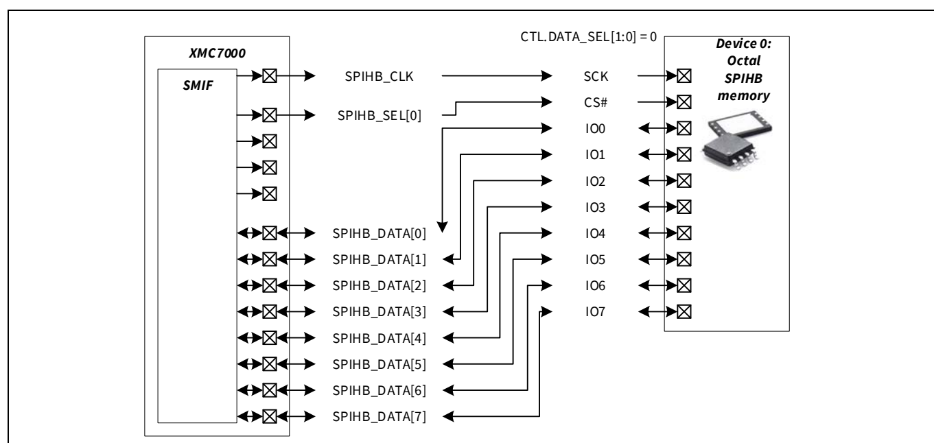
Figure 30-17. Octal SPI device 0 to SPIHB_DATA[7:0]
