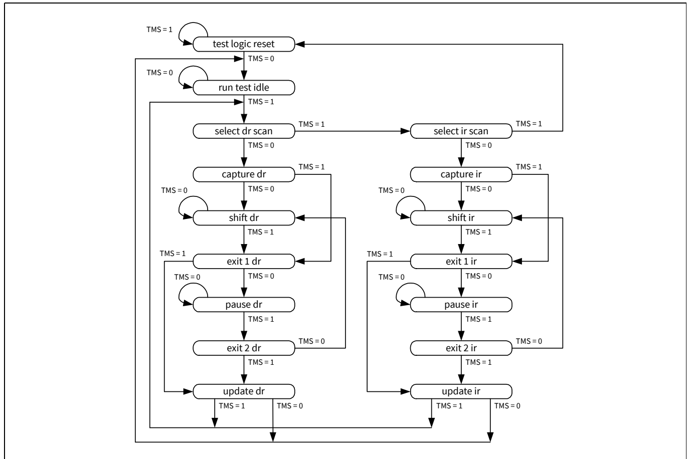
Figure 34-4. TAP state machine
