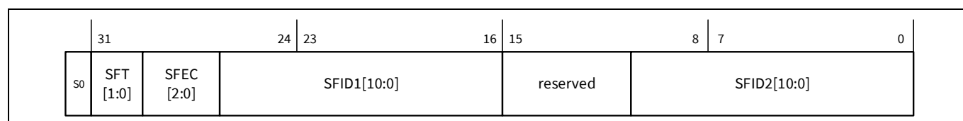
Figure 24-21. Standard message ID filter
