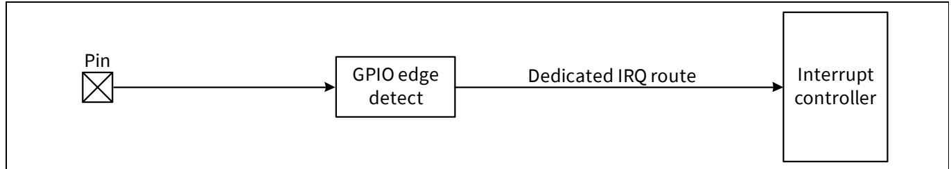
Figure 22-6. Interrupt signal routing
