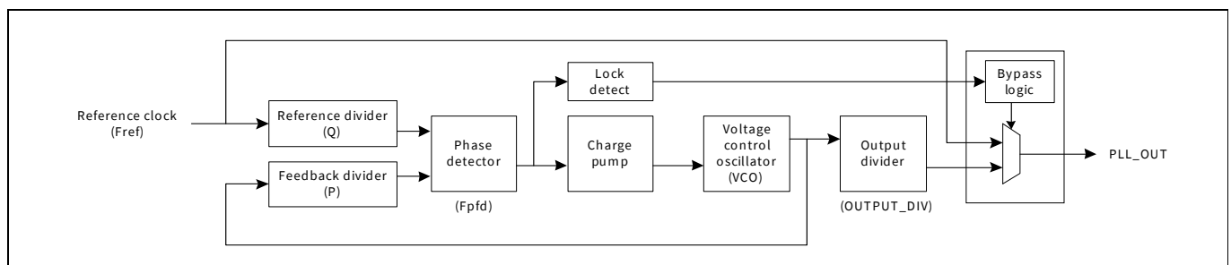
Figure 18-3. PLL without SSCG and fractional operation
