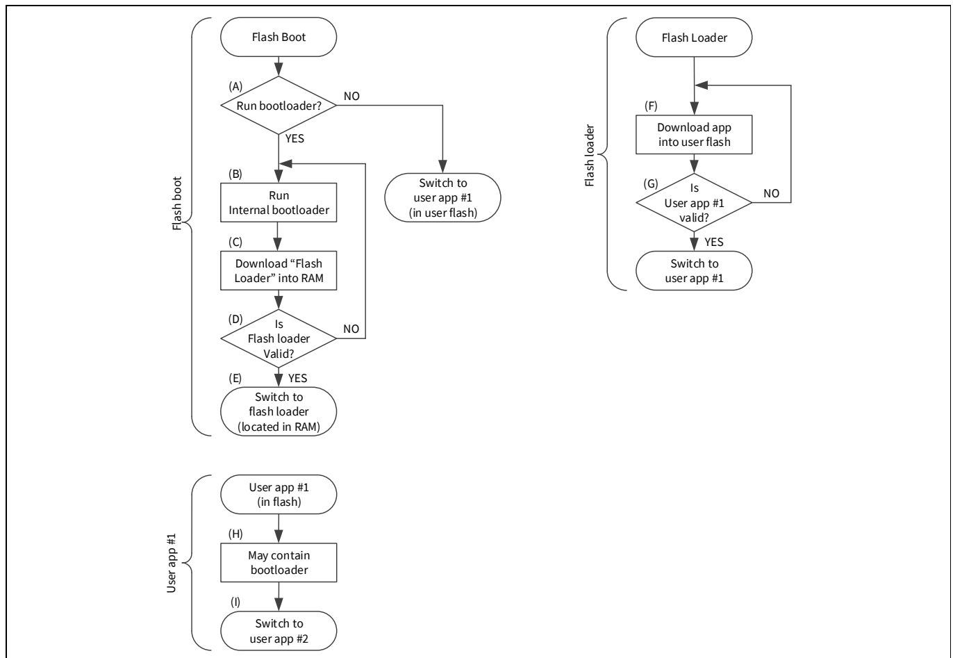
Figure 36-12. Startup and bootloading sequence
