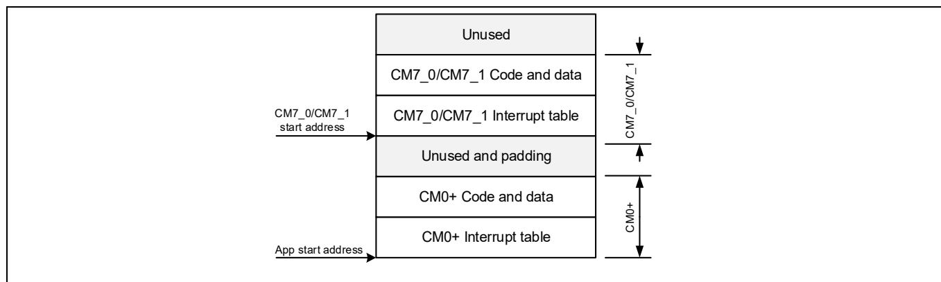
Figure 36-8. Basic application format structure
