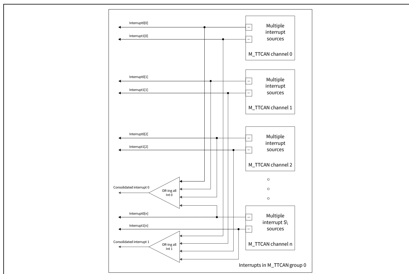
Figure 24-2. Interrupts in M_TTCAN group
