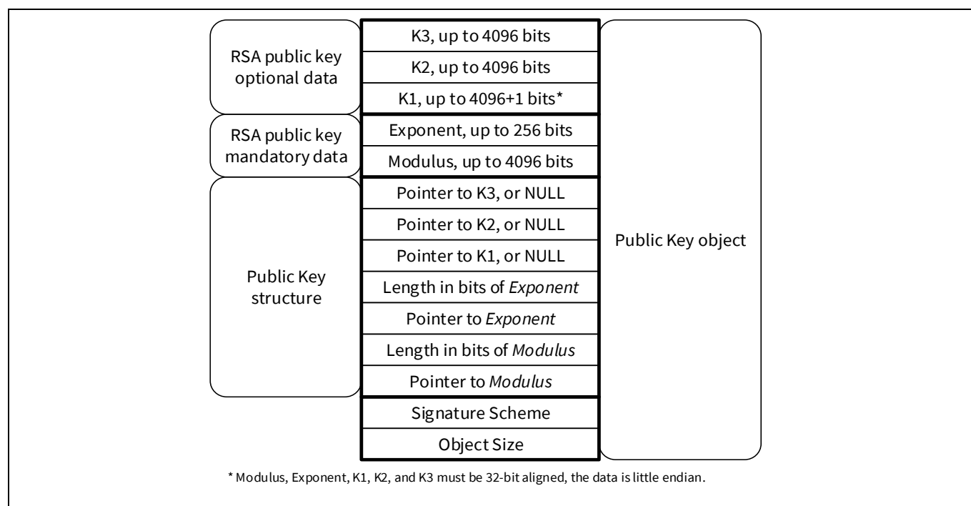
Figure 36-10. Public key format
