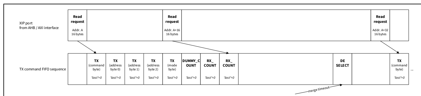
Figure 30-6. Read sequence with continuous merging enabled - merging always possible, but continuous transfer merge timeout occurs
