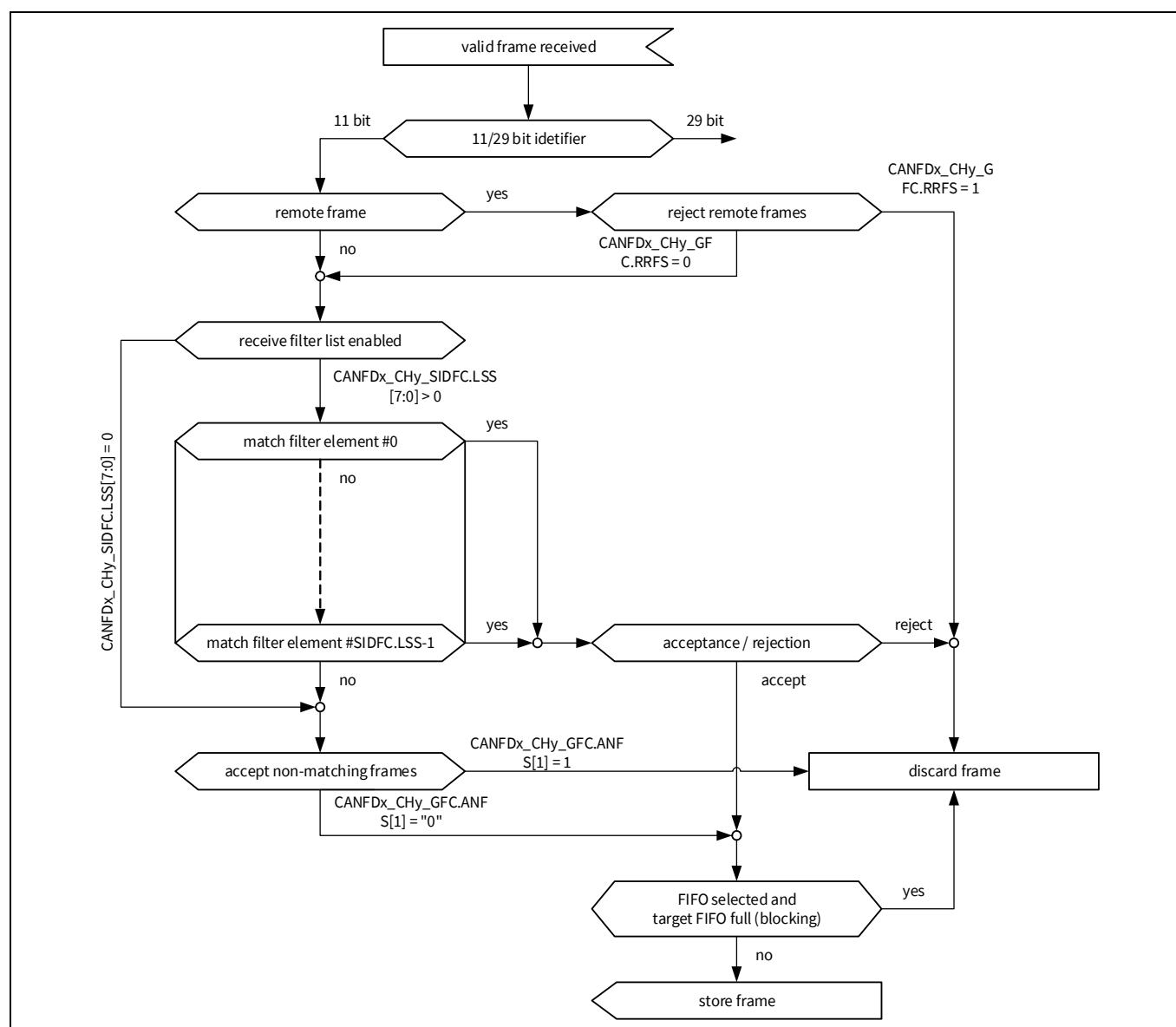
Figure 24-7. Standard message ID filter
