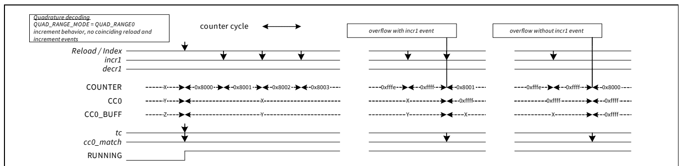
Figure 25-25. Overflow coincides with increment
