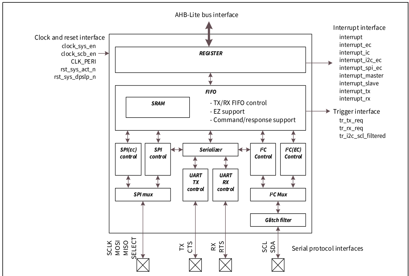
Figure 23-1. SCB block diagram
