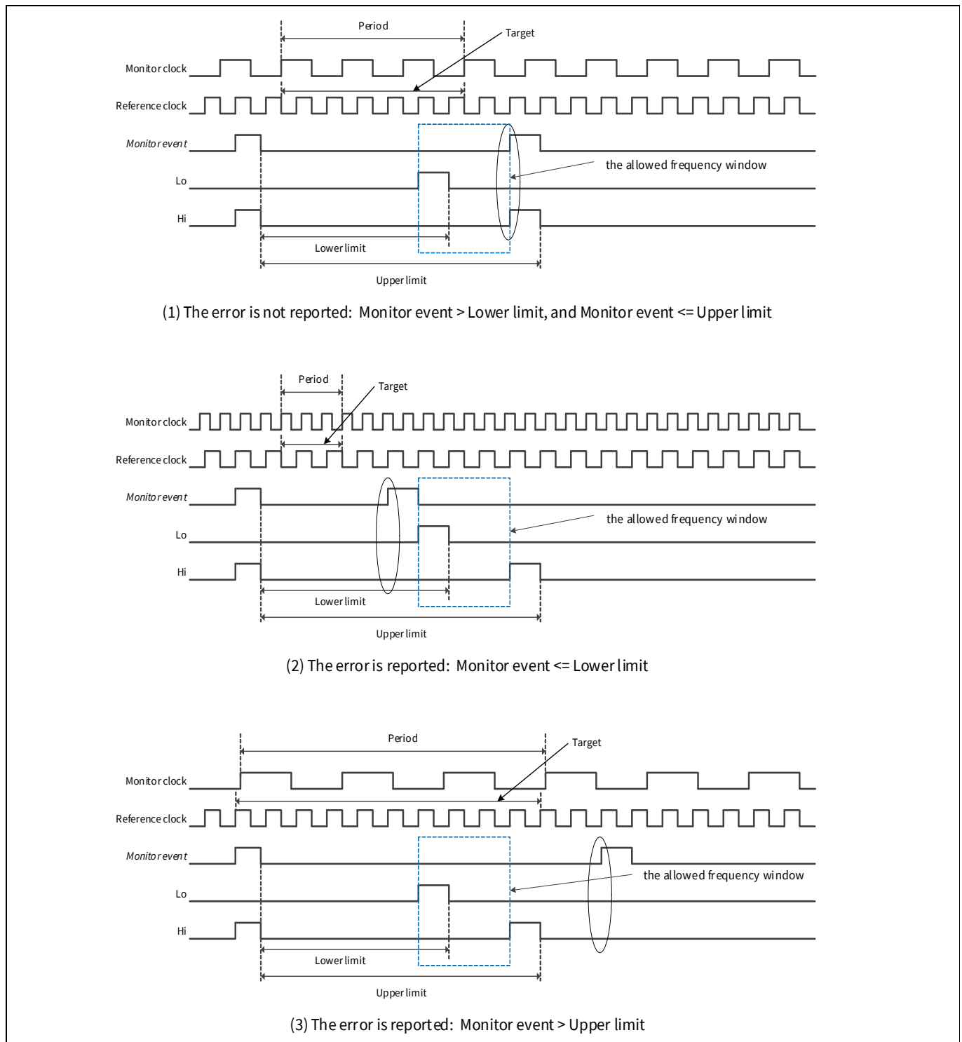
Figure 18-13. An example of CSV operation signal
