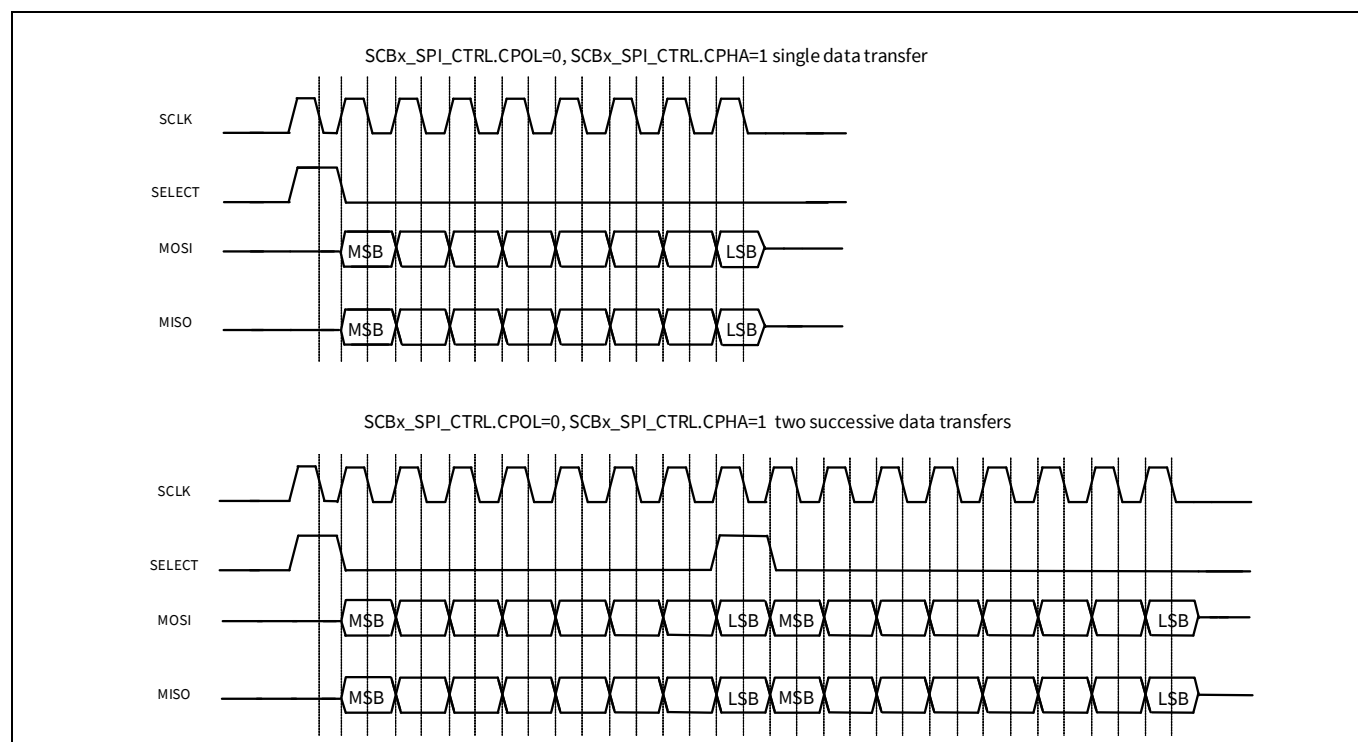
Figure 23-9. SPI TI data transfer example
