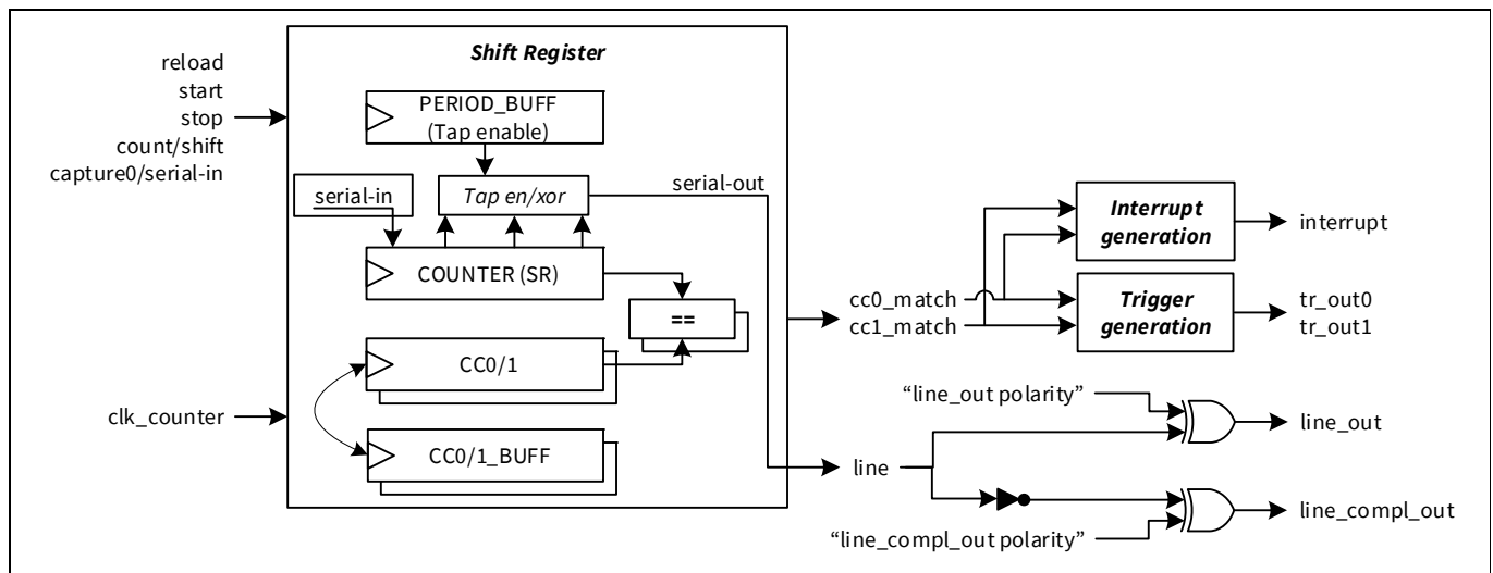
Figure 25-64. SR function diagram
