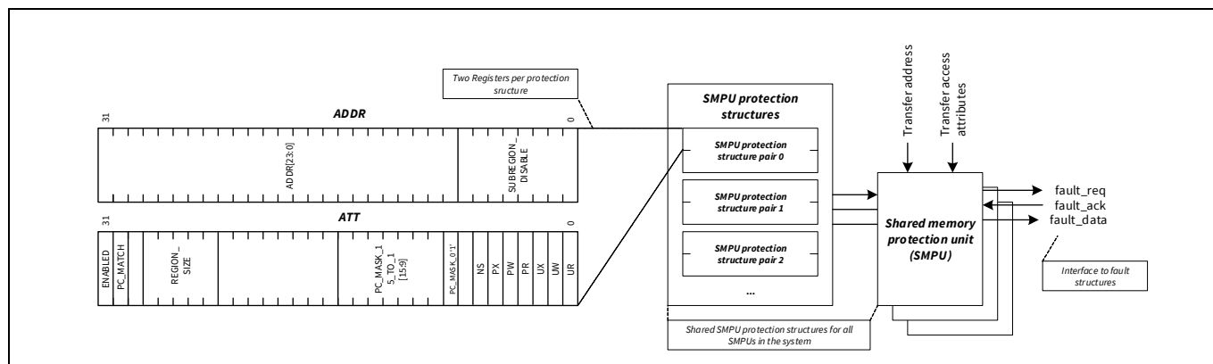
Figure 6-4. SMPU functionality
