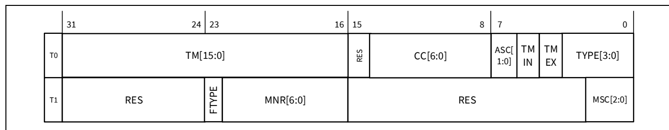
Figure 24-23. Trigger memory element
