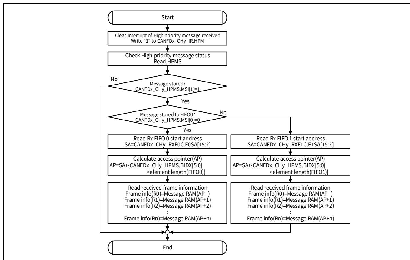
Figure 24-48. High priority message handling
