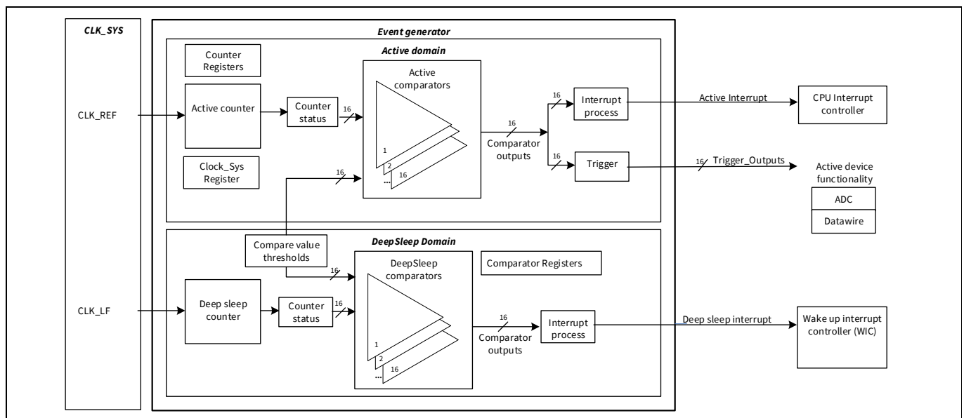
Figure 27-1. EVTGEN block diagram
