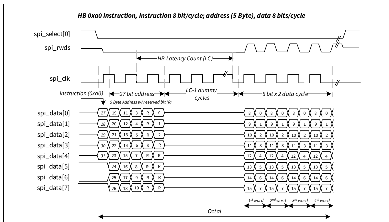
Figure 30-22. HYPERBUS™ transfer waveform
