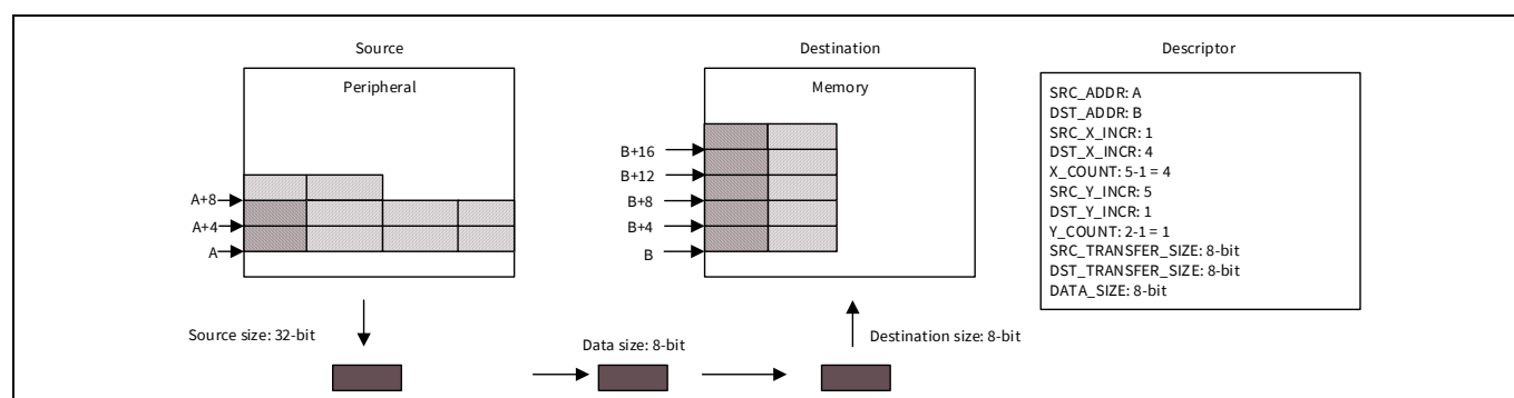
Figure 7-17. M-DMA inverse direction transfer
