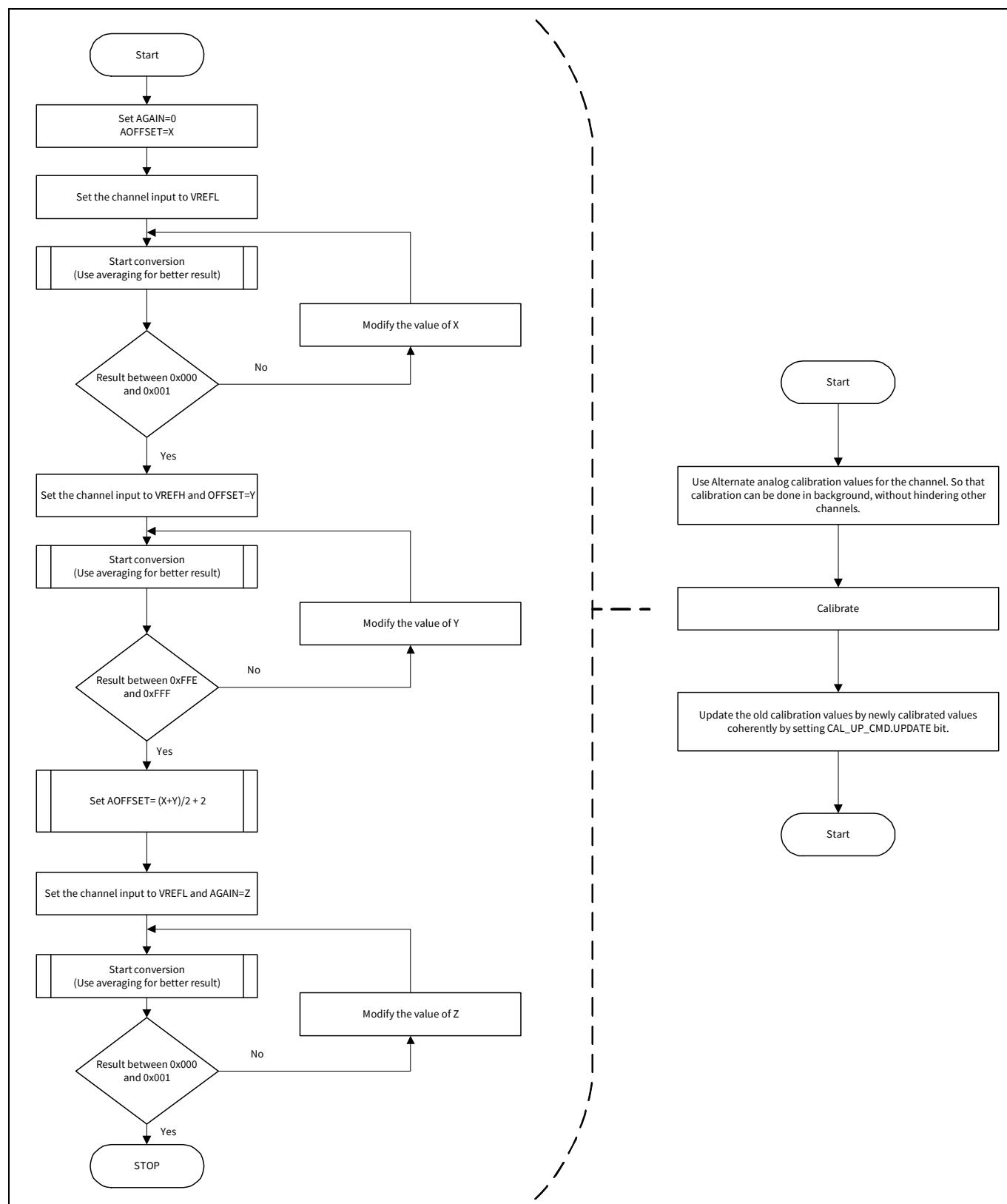
Figure 33-11. Calibration flow diagram
