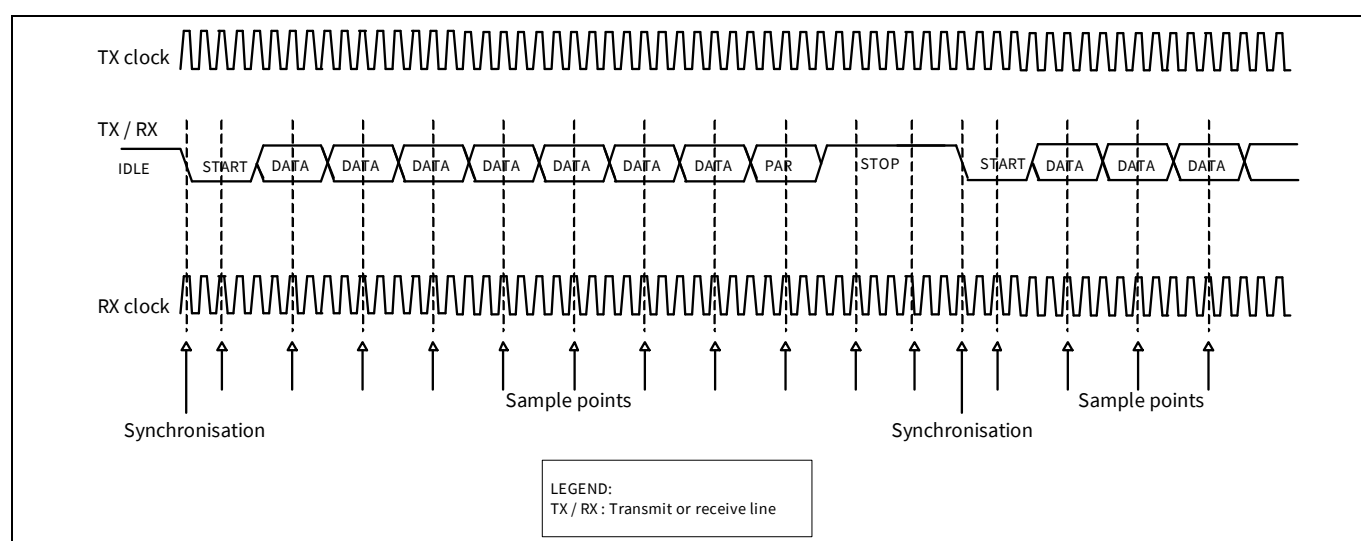
Figure 23-21. UART, standard protocol example (single sample)
