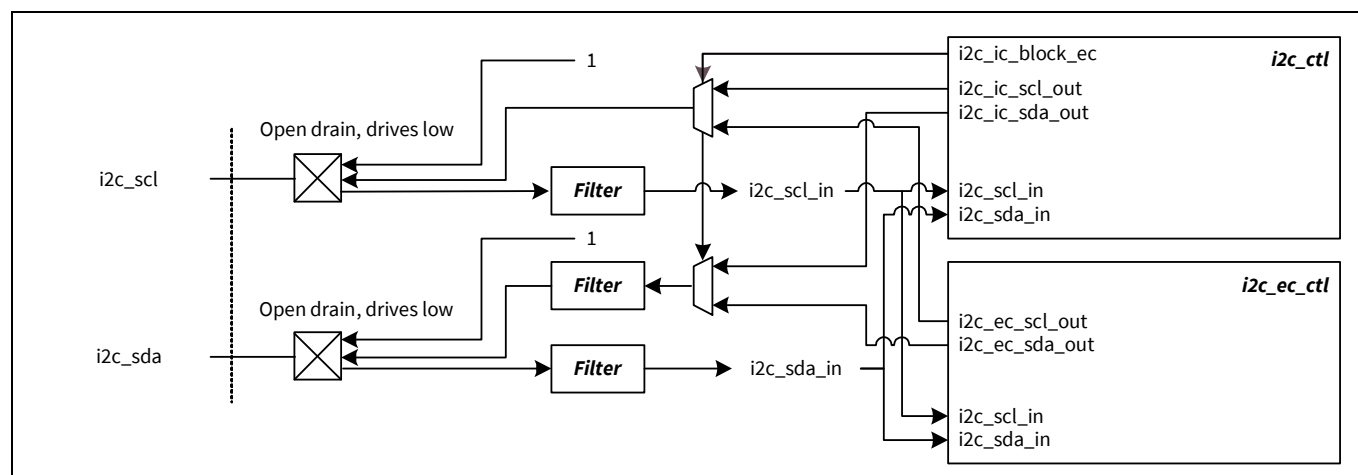
Figure 23-42. I 2 C I/O pad connections
