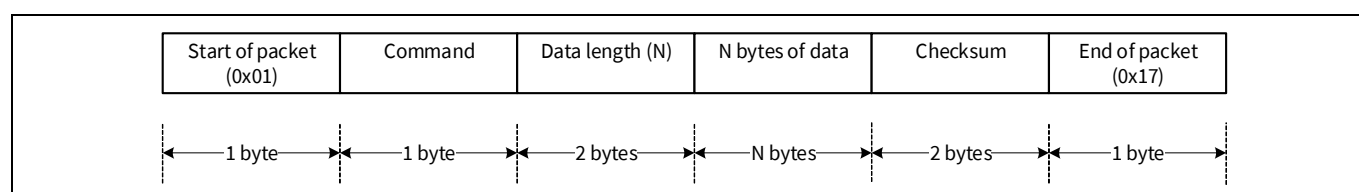
Figure 36-1. Bootloader command packet structure
