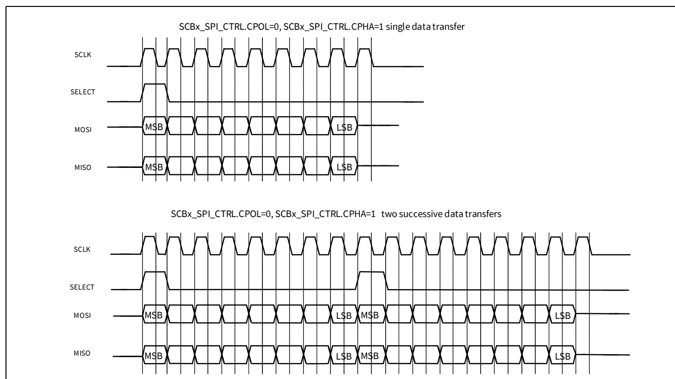
Figure 23-10. SPI TI data transfer example
