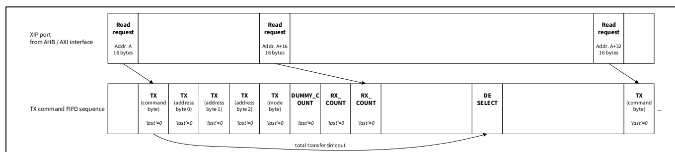
Figure 30-7. Read sequence with continuous merging enabled - merging always possible, but total transfer merge timeout occurs
