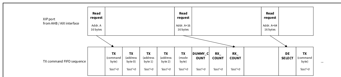
Figure 30-5. Read sequence with continuous merging enabled - merging possible once
