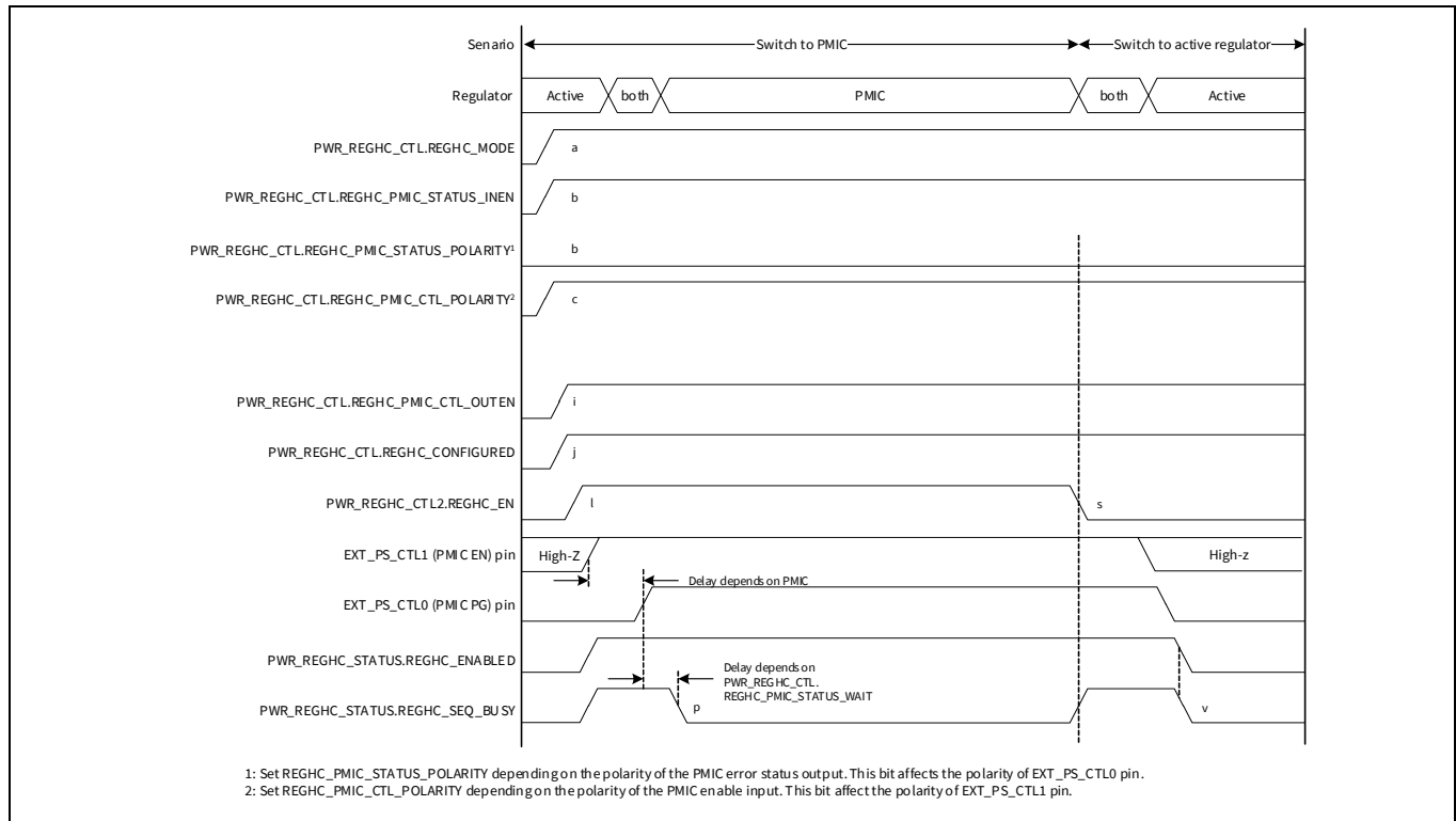
Figure 16-6. Transitions between active regulator and external PMIC
