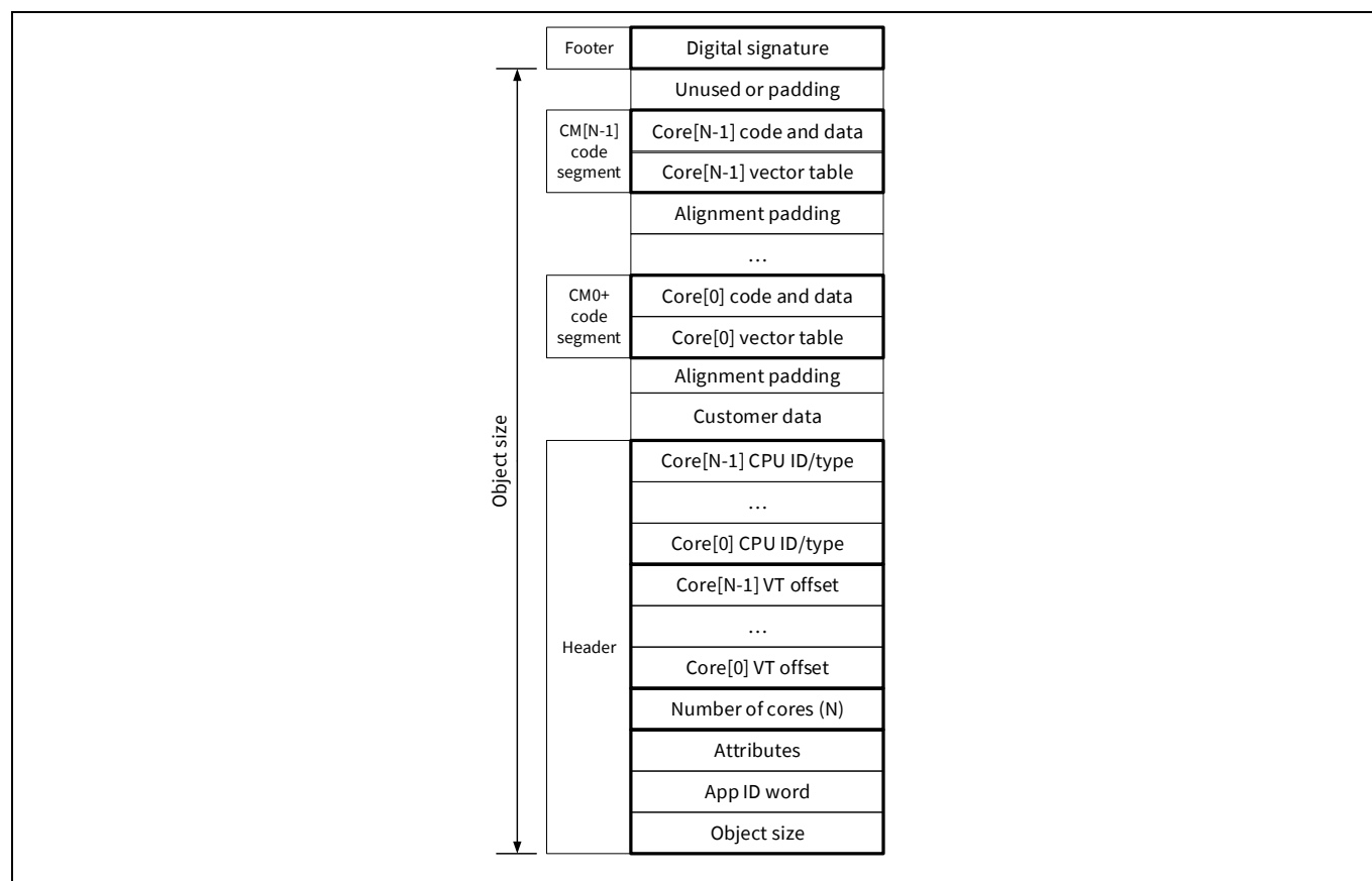
Figure 36-9. CySAF structure
