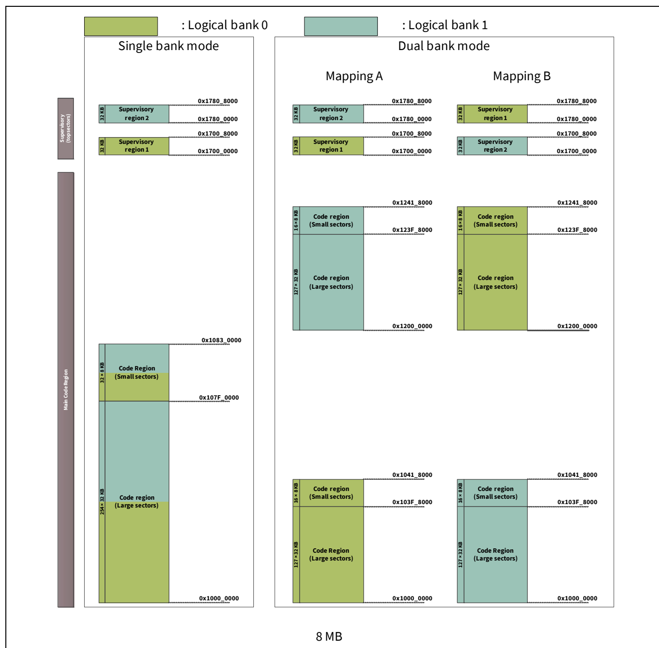
Figure 8-9. Code flash memory mapping (8 MB)
