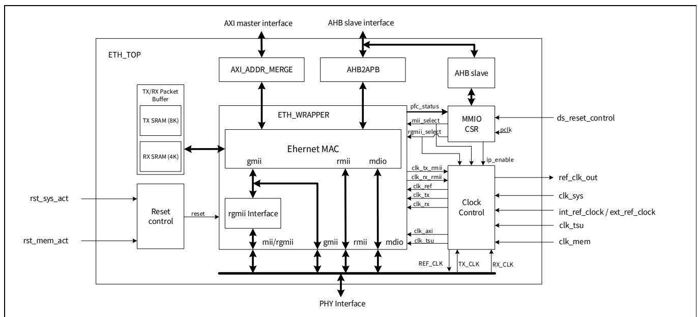
Figure 29-1. Ethernet MAC block diagram
