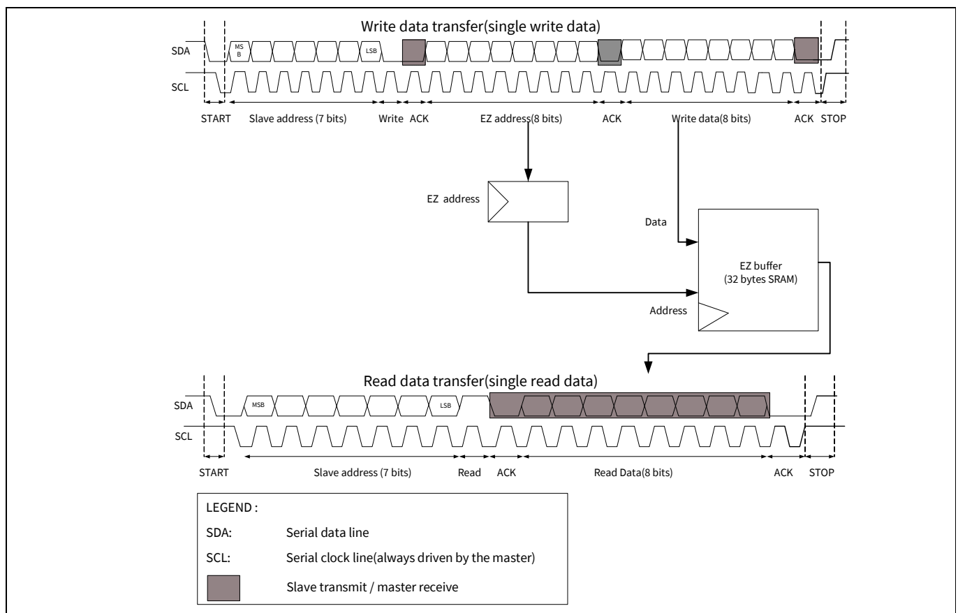
Figure 23-39. EZI2C write and read data transfer
