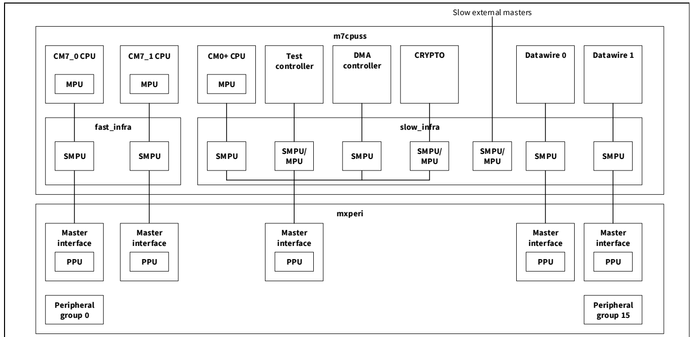
Figure 6-1. Protection unit locations
