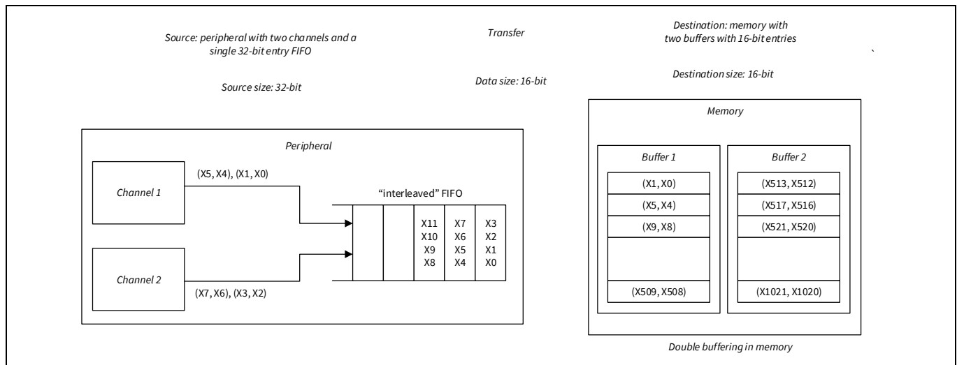
Figure 7-8. 2D transfer
