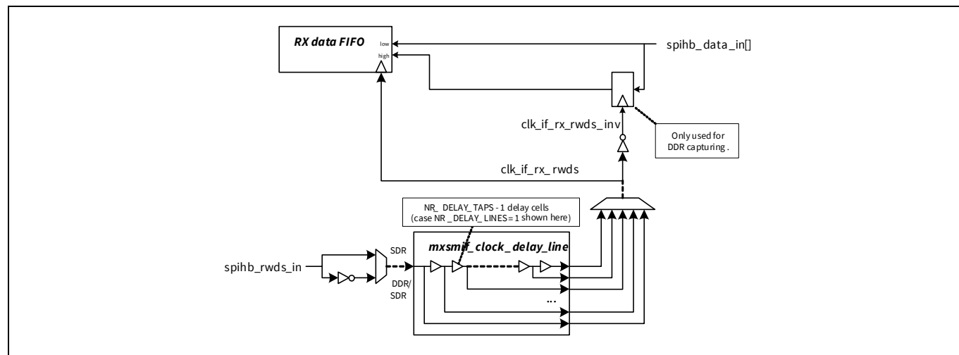
Figure 30-29. RWDS-based capture scheme
