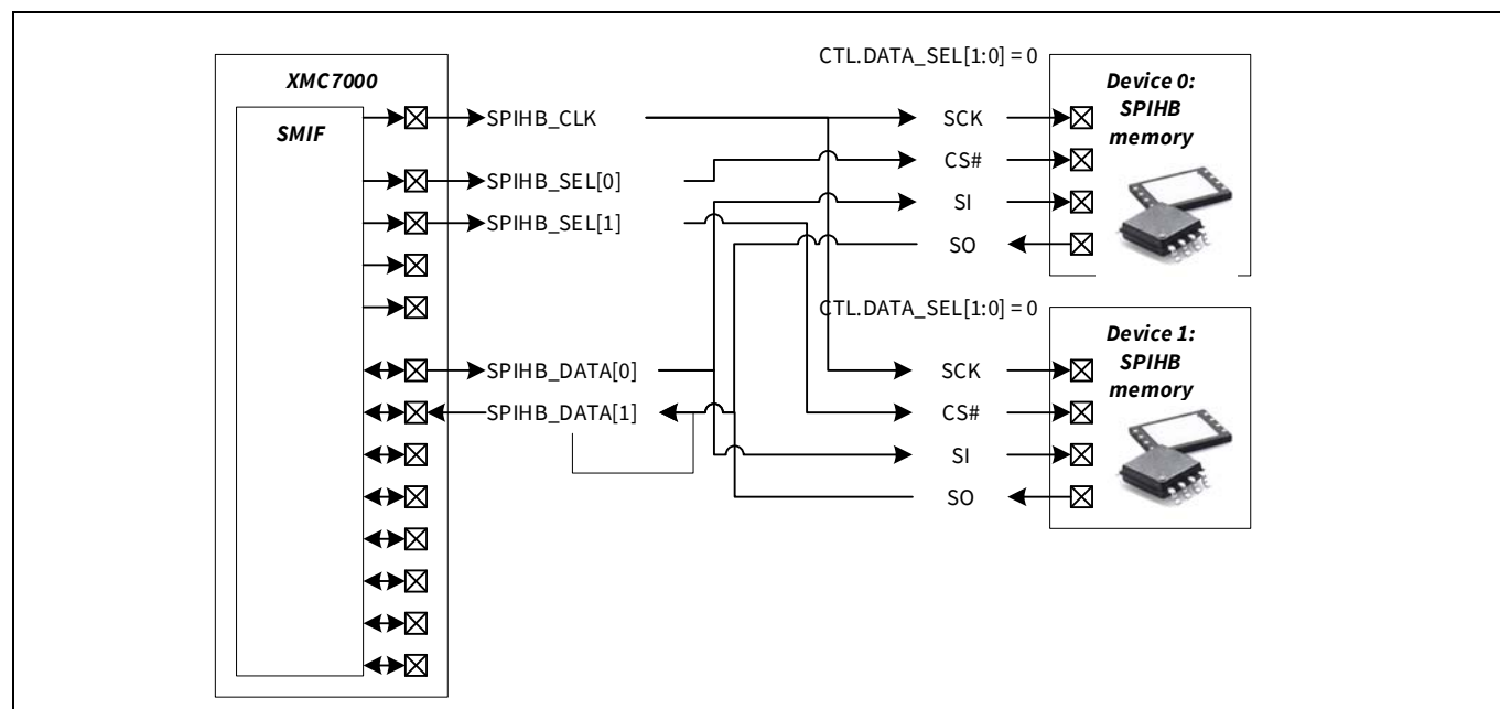
Figure 30-12. Single SPI device 0 to SPIHB_DATA[1:0], single SPI device 1 connected to SPIHB_DATA[1:0]
