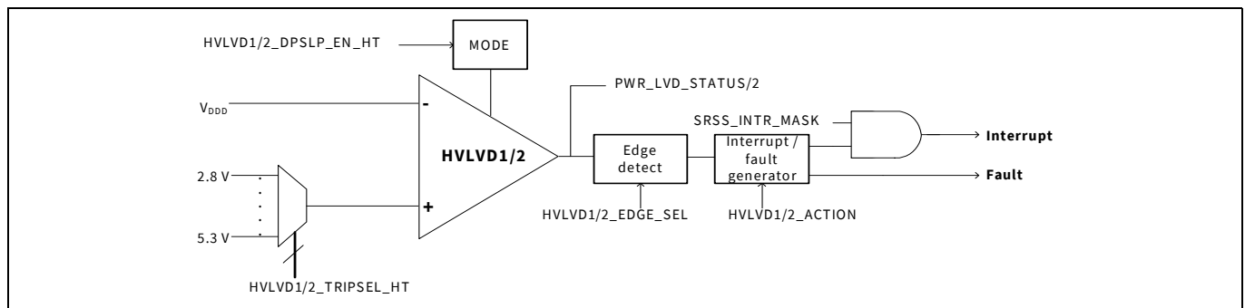
Figure 16-8. XMC7000 LVD block
