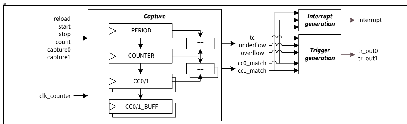
Figure 25-18. Capture functionality
