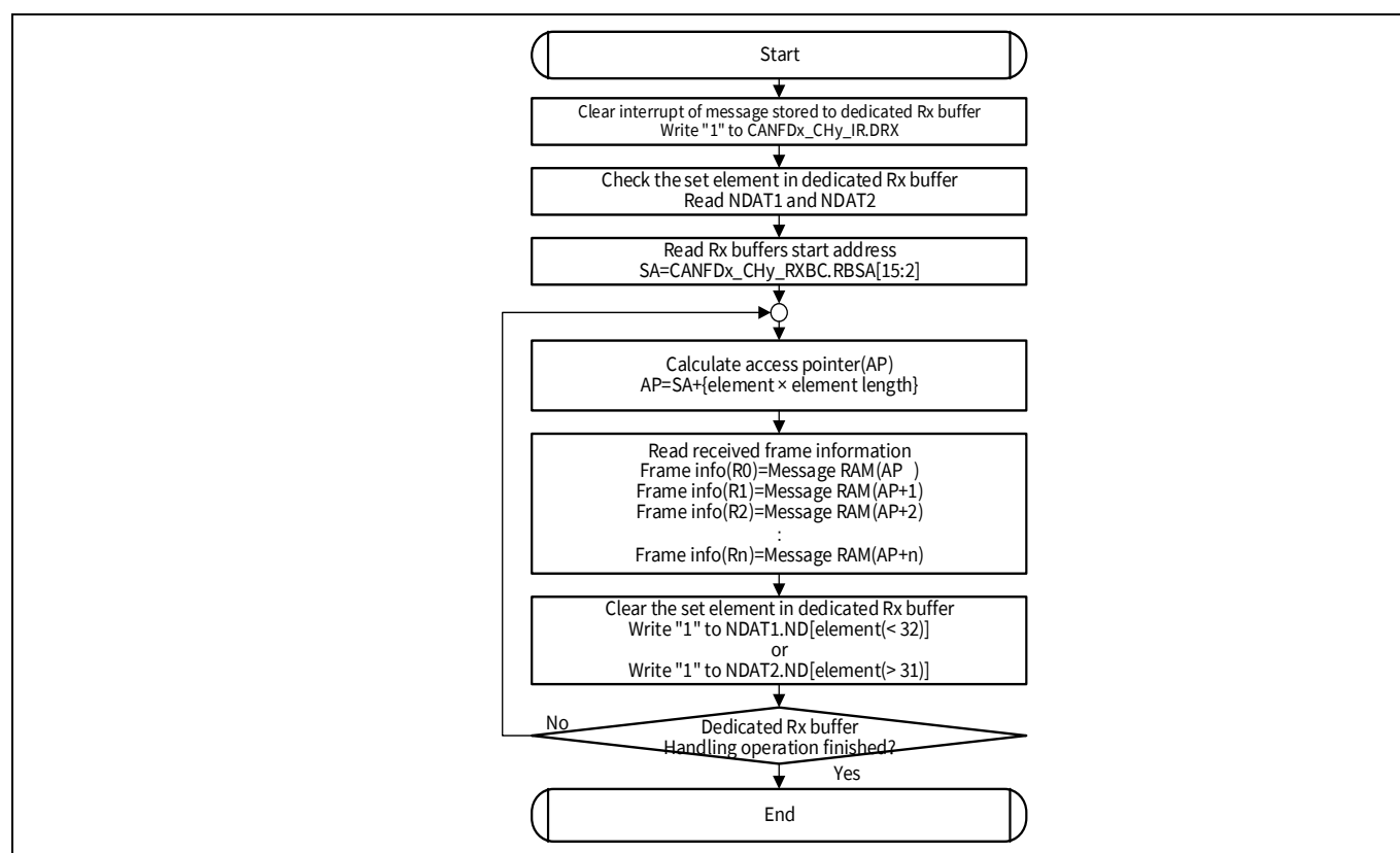
Figure 24-47. Dedicated RX buffer handling
