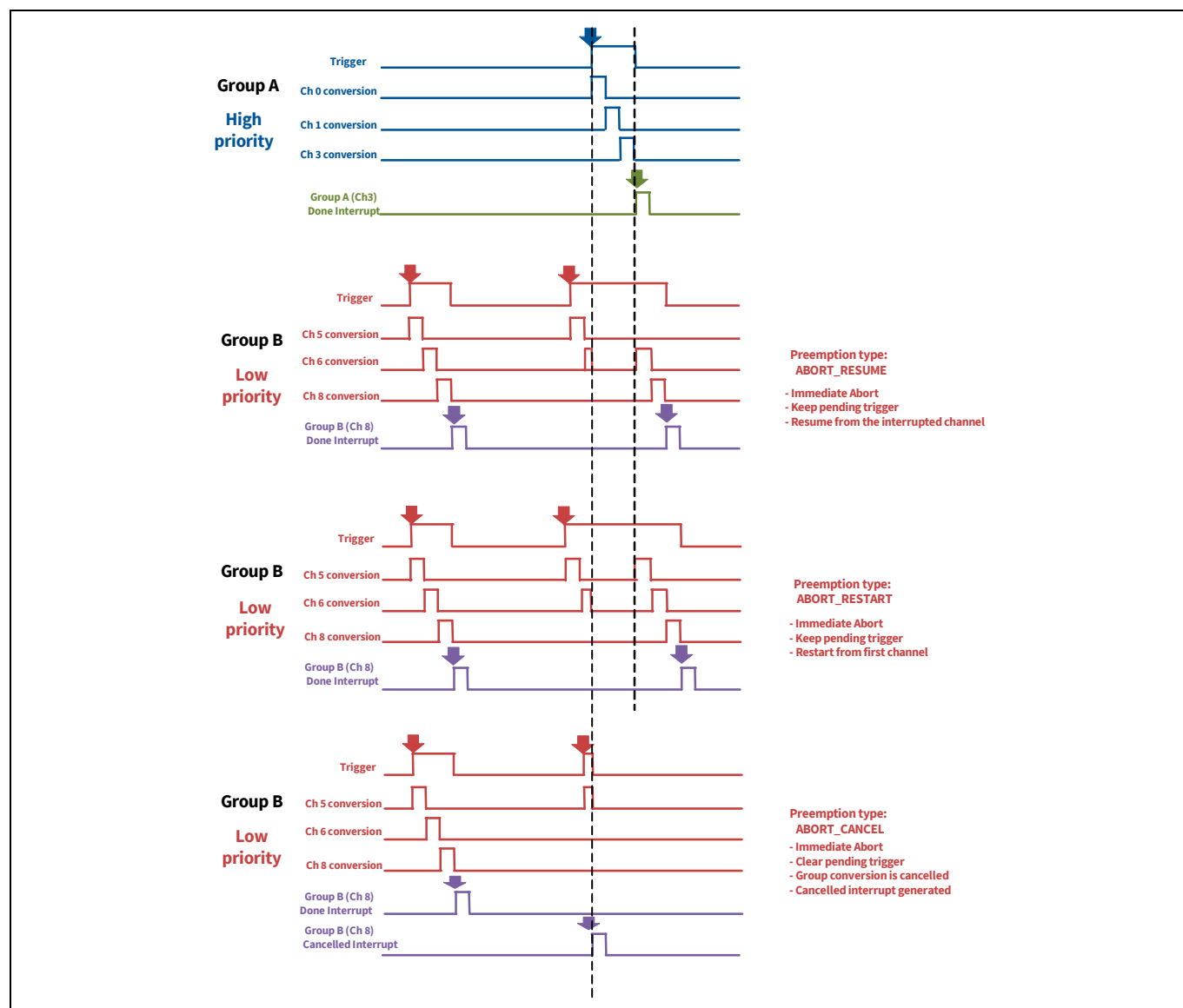
Figure 33-9. Preemption types: A low priority group B behavior with different preemption types
