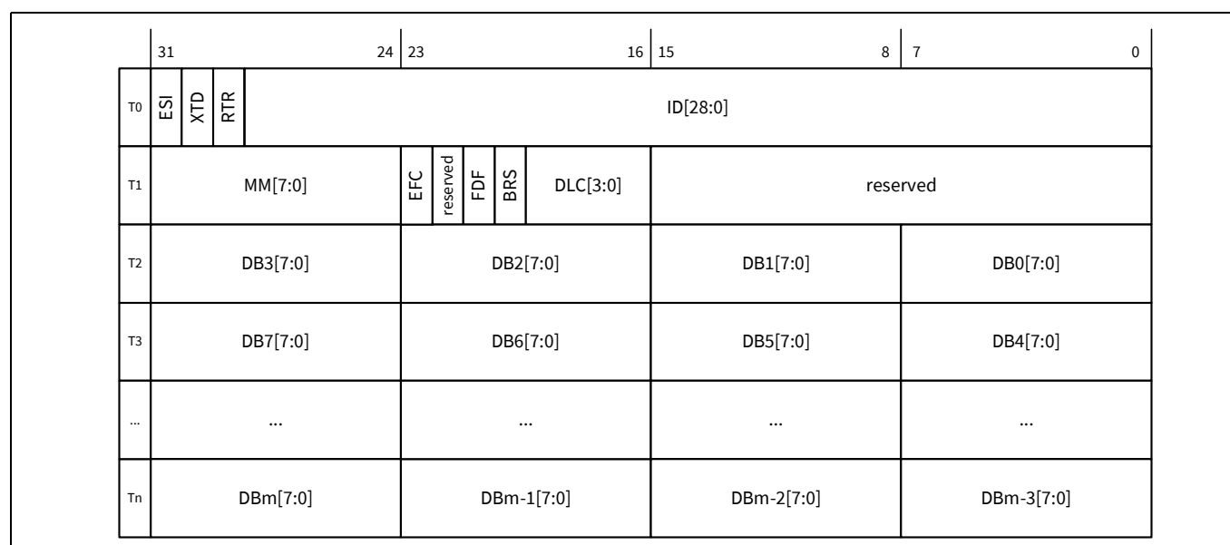
Figure 24-19. TX buffer element
