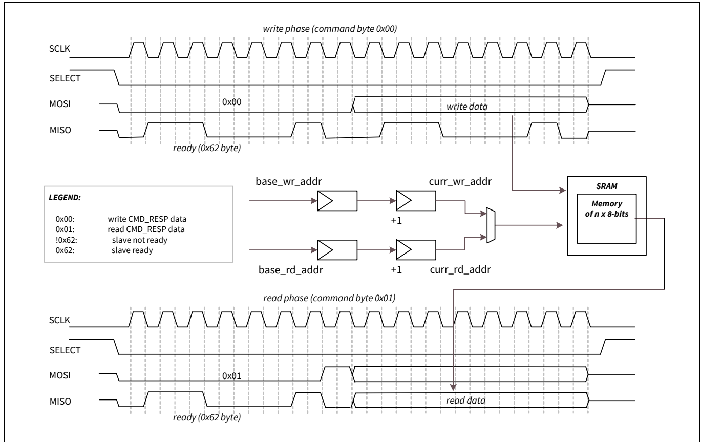
Figure 23-13. Command-response mode example
