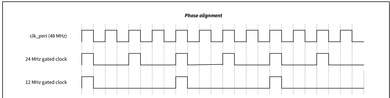
Figure 18-10. Phase-aligned clock dividers
