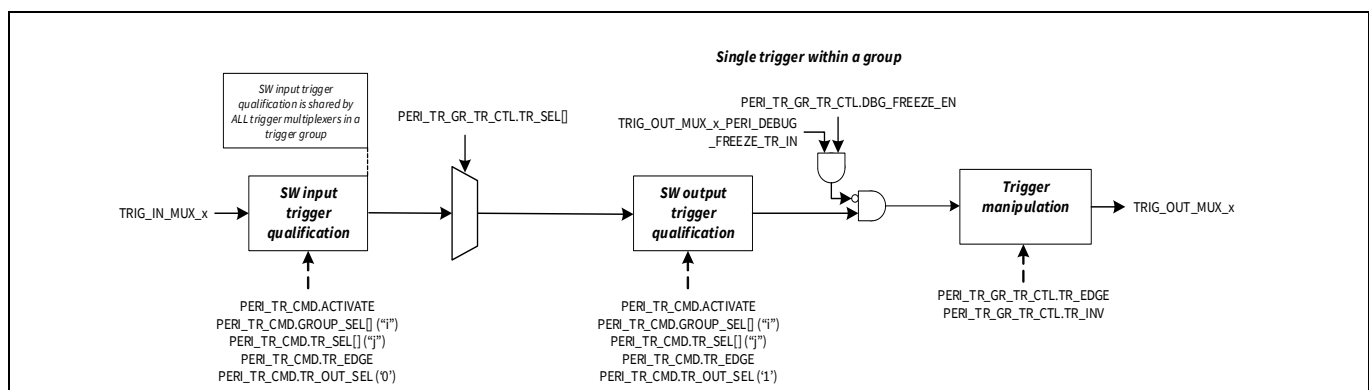
Figure 28-5. Multiplexer trigger group
