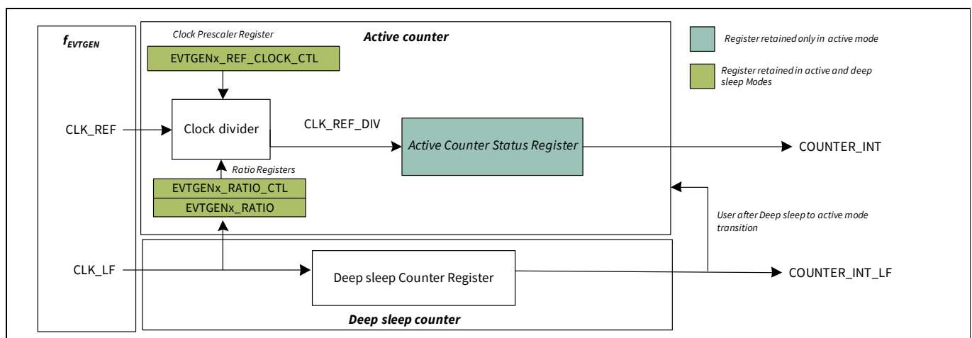
Figure 27-2. Counter block diagram
