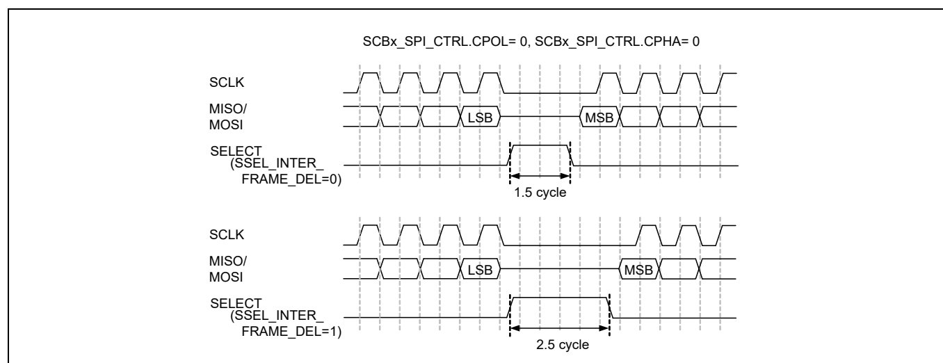
Figure 23-16. SELECT INTER-FRAME deselect time
