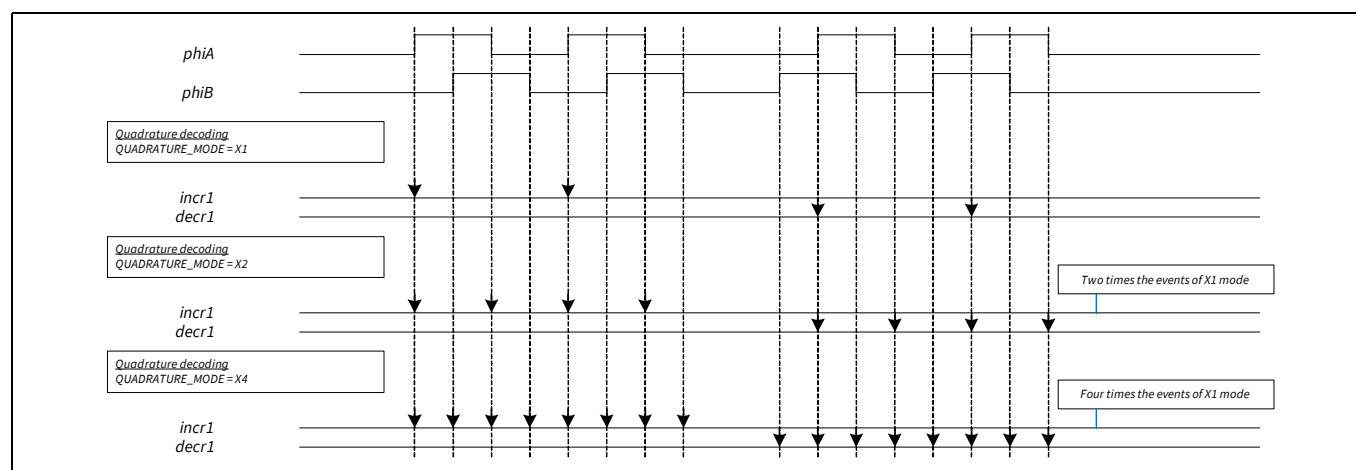
Figure 25-21. Quadrature mode waveforms (X1, X2, and X4 mode)
