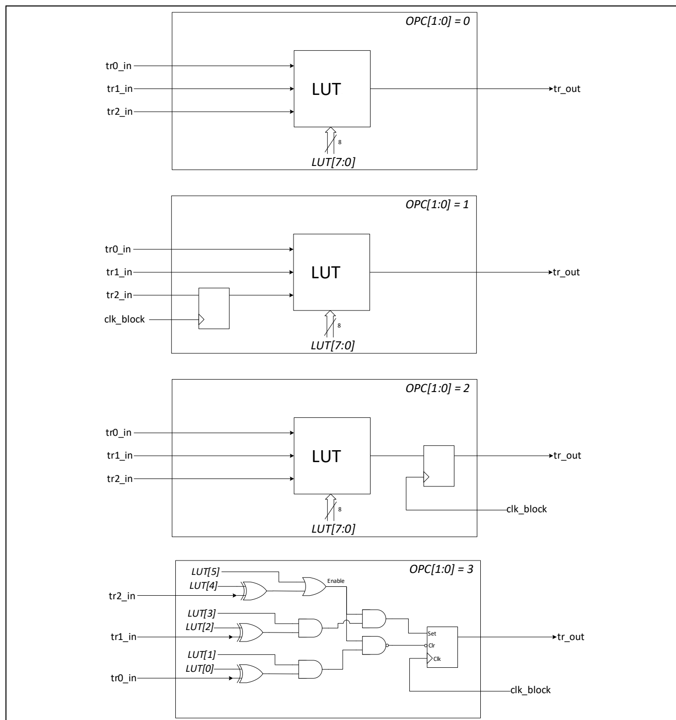
Figure 22-10. Smart I/O LUT configuration
