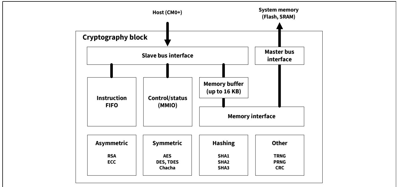
Figure 26-1. High-level block diagram
