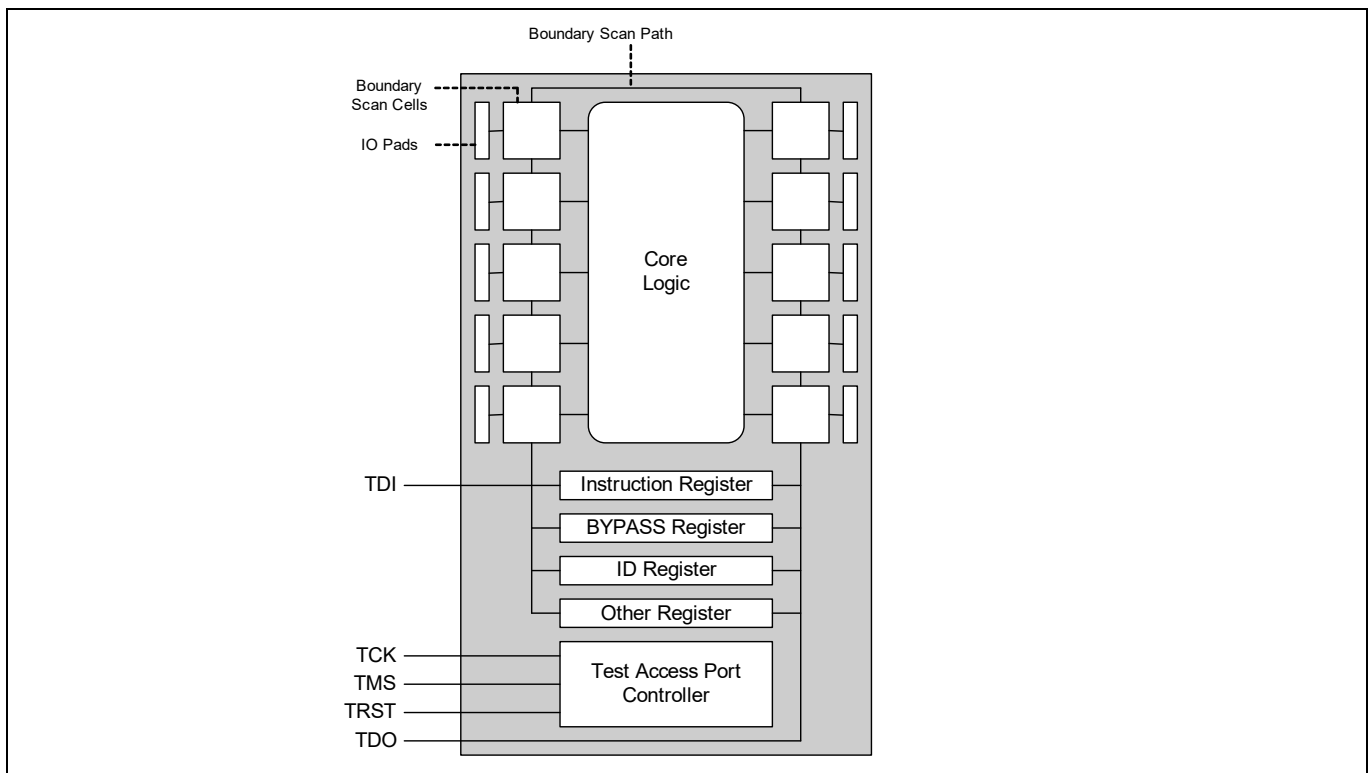
Figure 34-3. JTAG interface architecture
