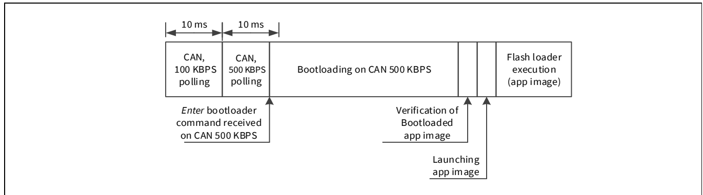
Figure 36-4. Successful bootloading on CAN 500 kbps
