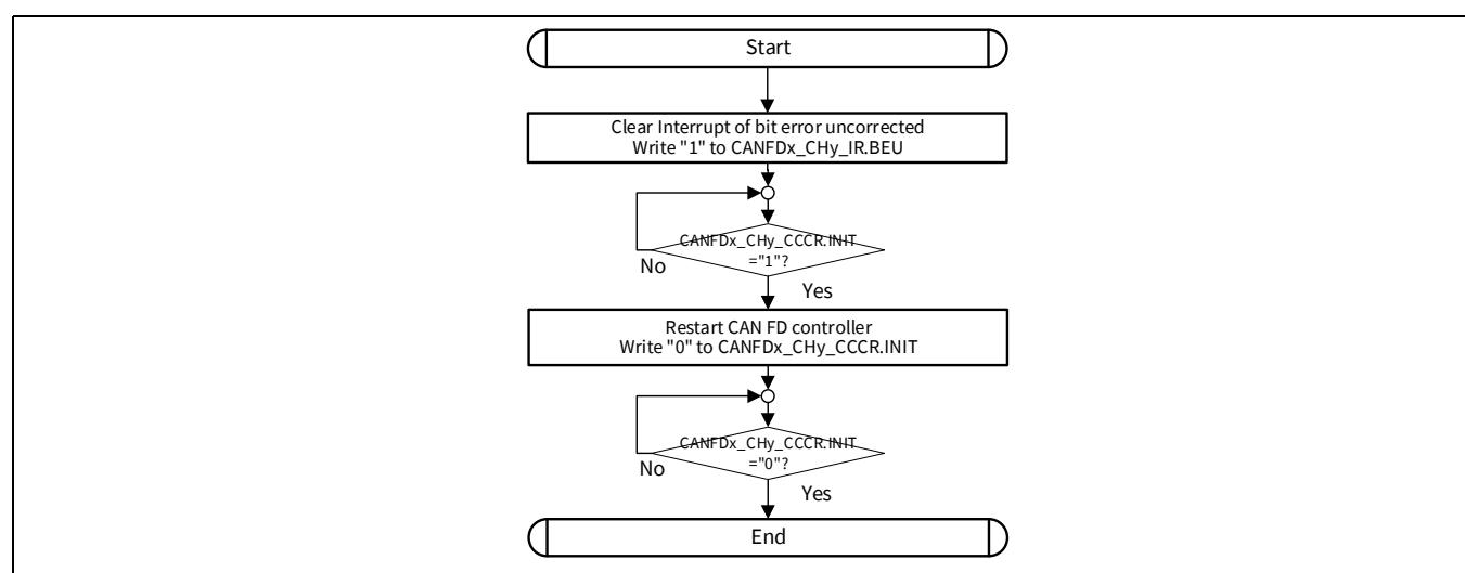
Figure 24-44. Bit error handling
