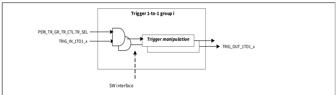
Figure 28-4. Trigger one-to-one group
