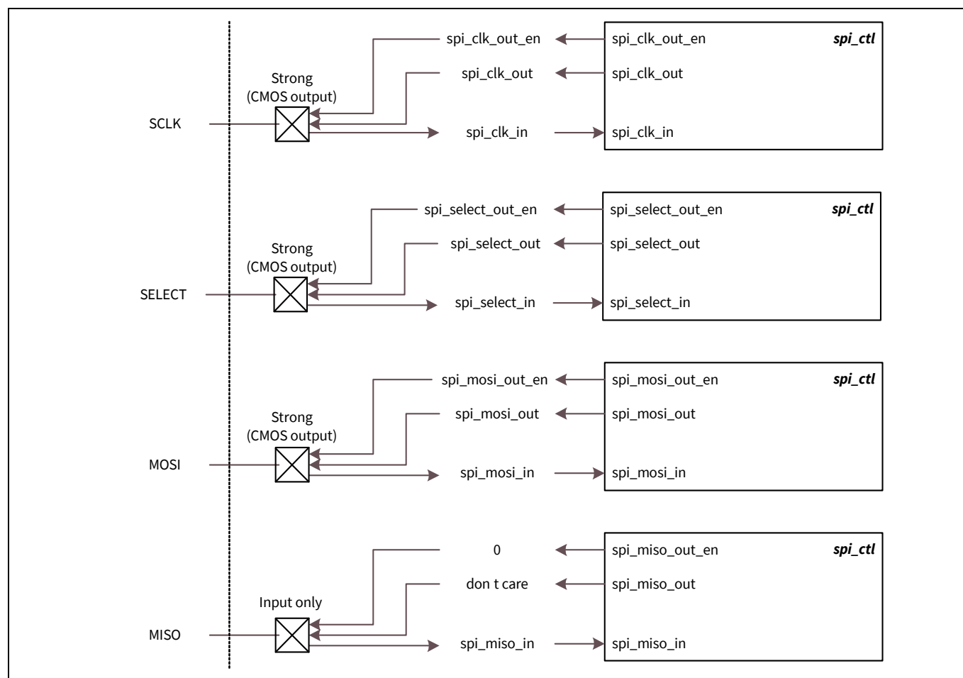
Figure 23-17. SPI master I/O pad connections
