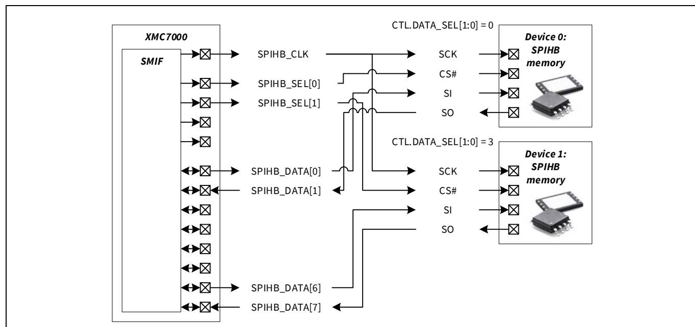
Figure 30-11. Single SPI device 0 to SPIHB_DATA[1:0], single SPI device 1 connected to SPIHB_DATA[7:6]
