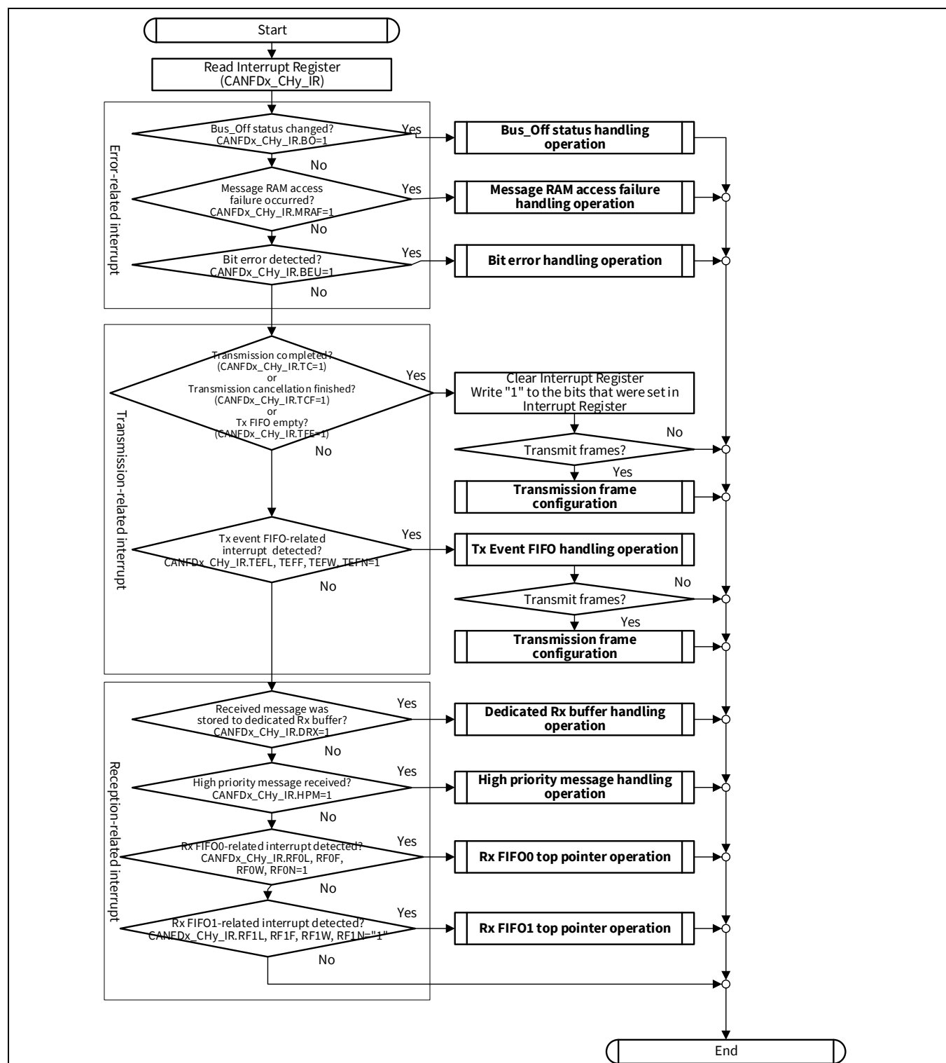
Figure 24-42. Interrupt handling
