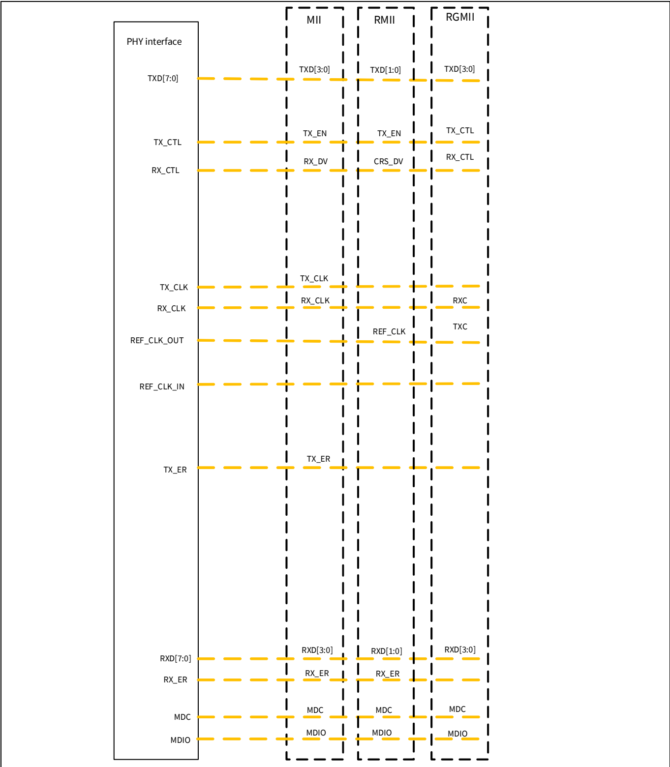
Figure 29-3. PHY interface
