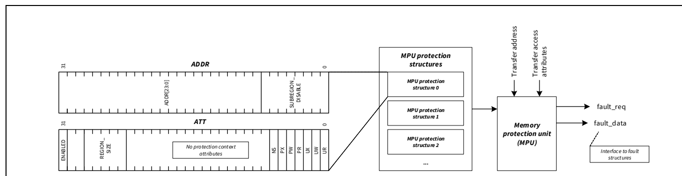
Figure 6-3. MPU functionality
