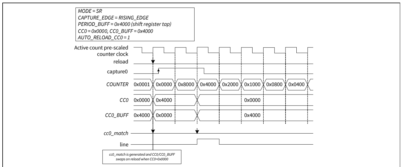
Figure 25-66. SR shift when PERIOD_BUFF = 0x4000
