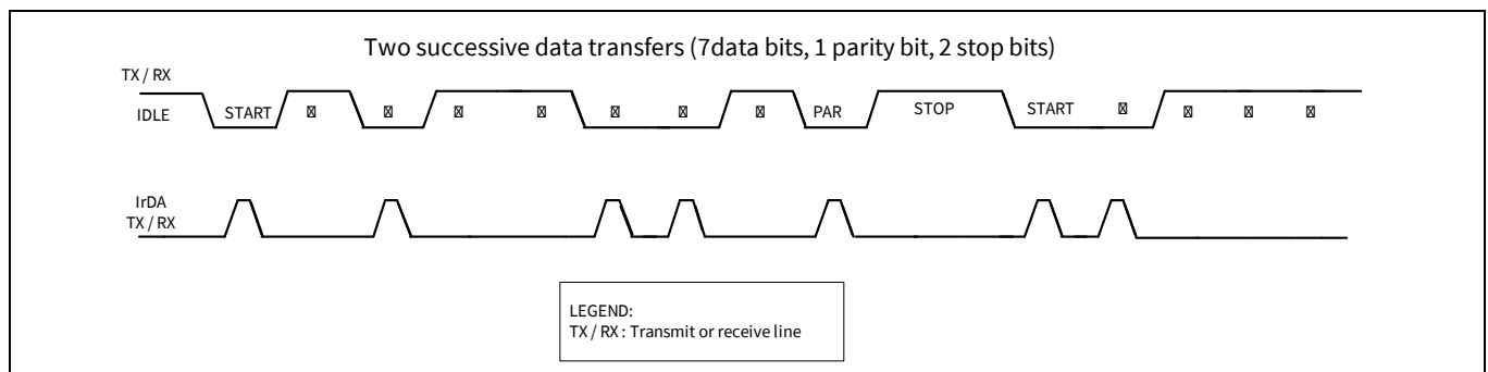
Figure 23-30. IrDA example
