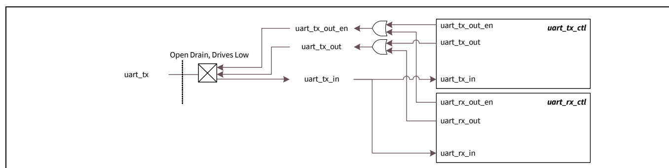
Figure 23-34. SmartCard mode I/O pad connections
