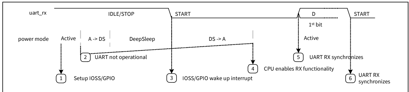
Figure 23-24. UART start skip and wakeup from deep sleep
