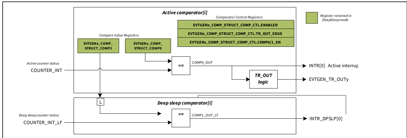
Figure 27-4. Comparator structure
