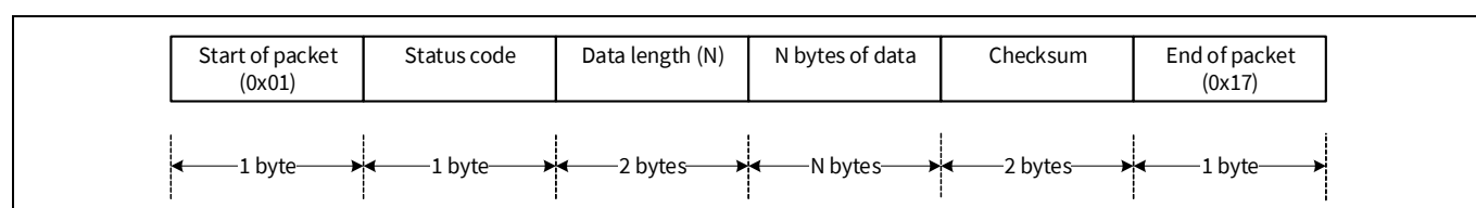
Figure 36-2. Bootloader response packet structure
