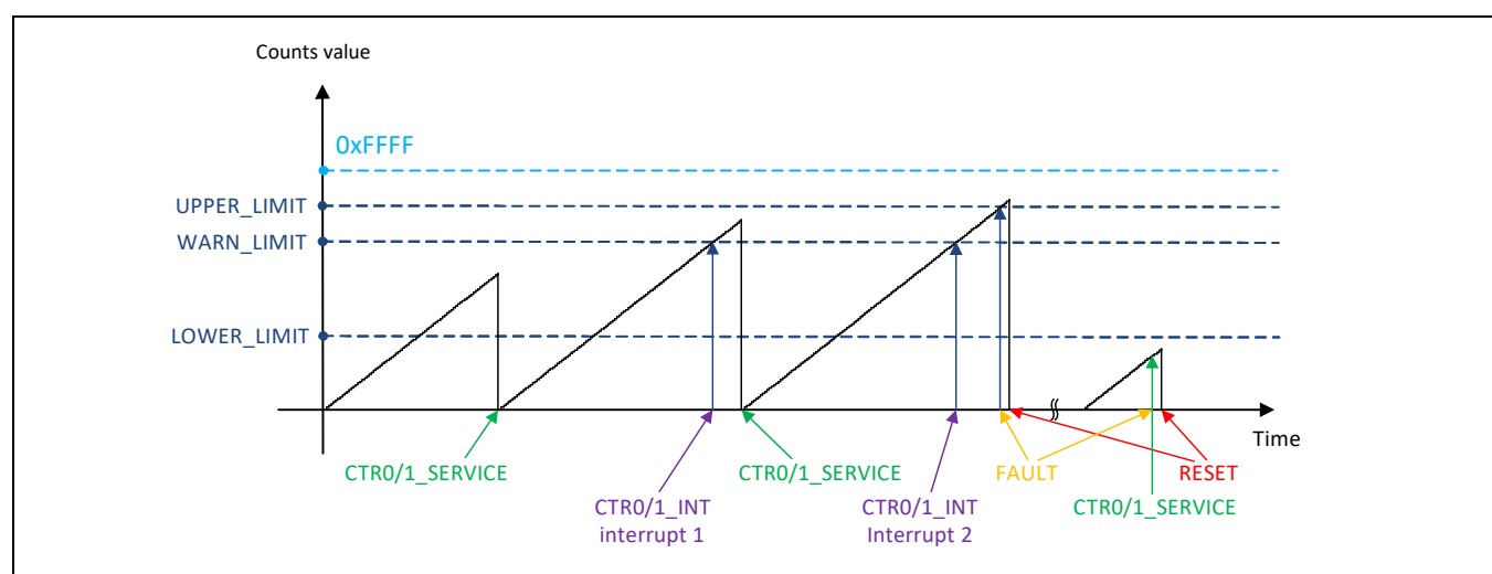
Figure 20-8. Subcounter 0/1 operation in window mode with FAULT and RESET action
