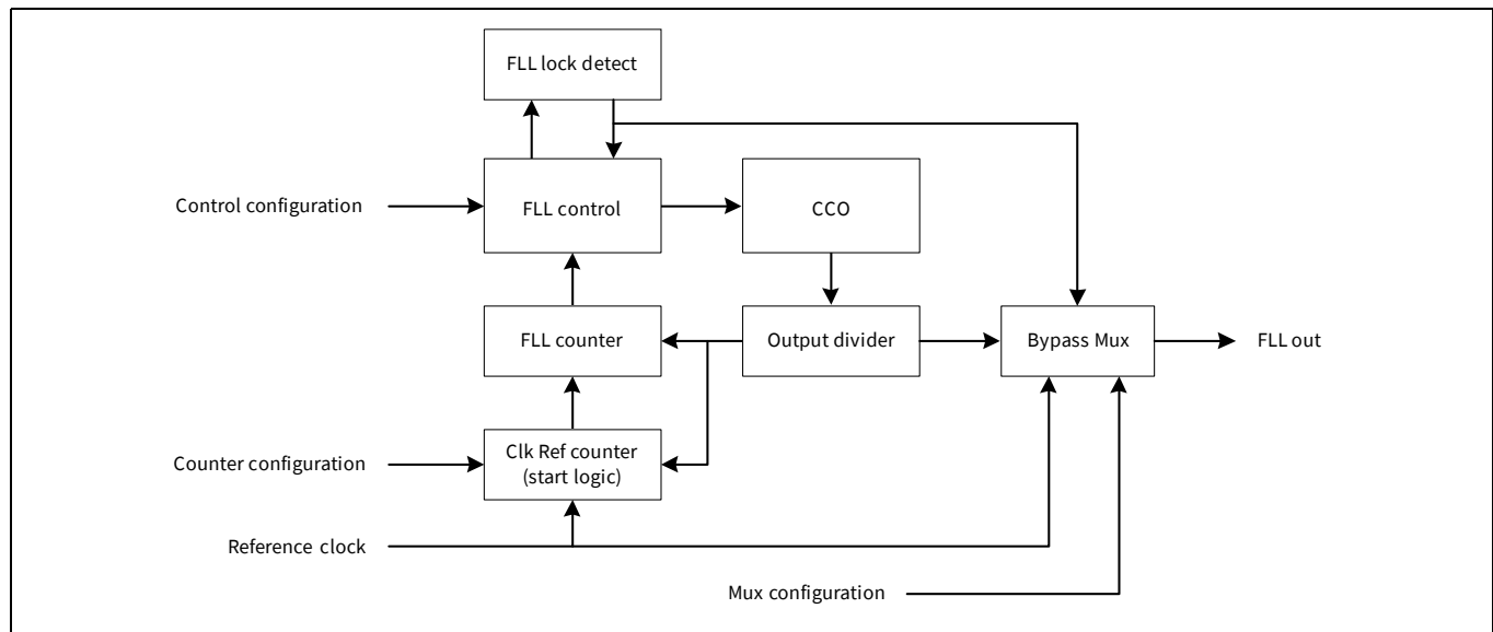
Figure 18-5. FLL block diagram
