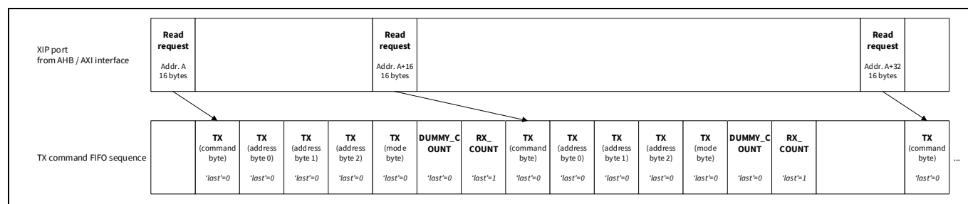
Figure 30-3. Read sequence with continuous merging disabled
