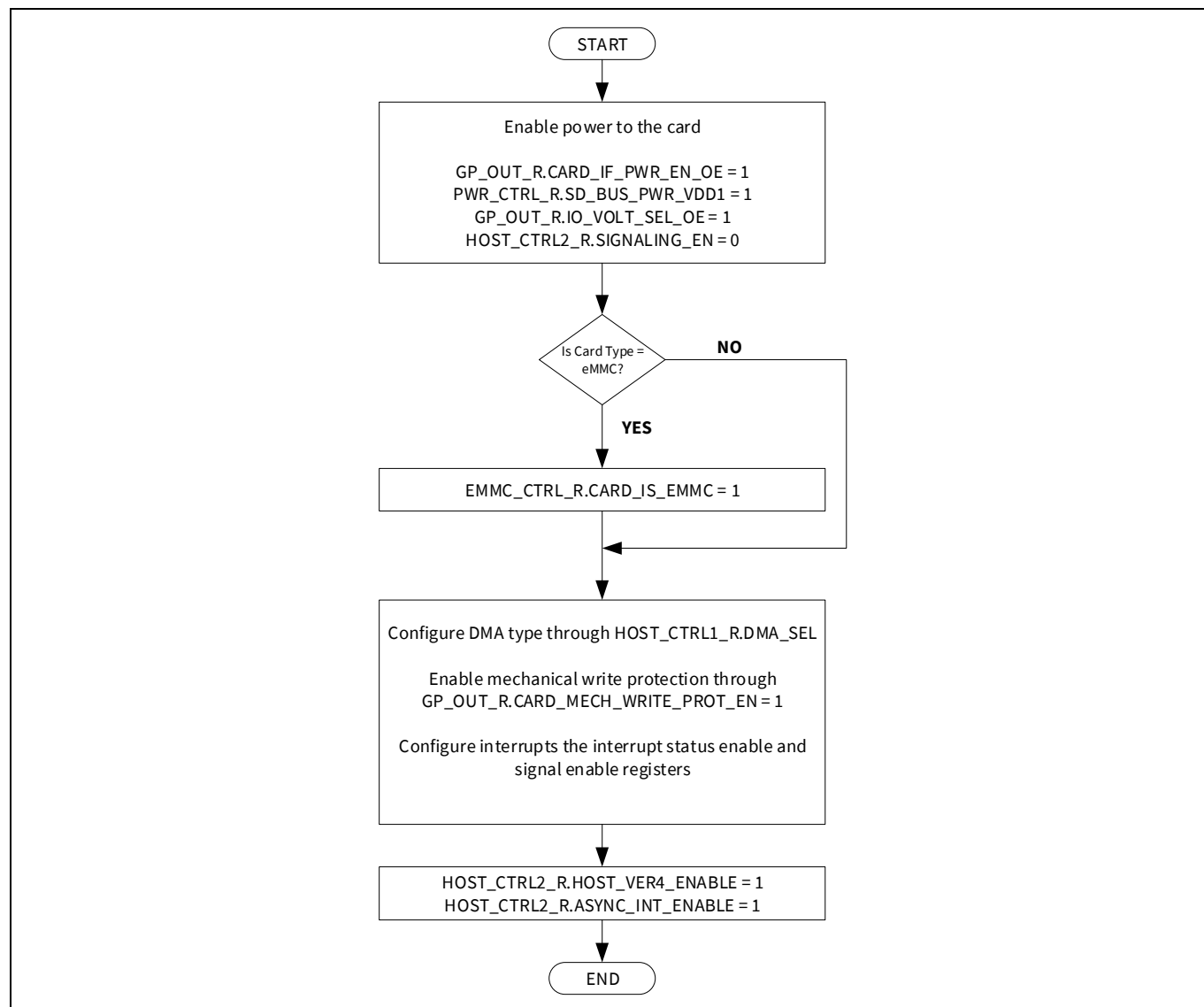
Figure 31-9. SDHC setup
