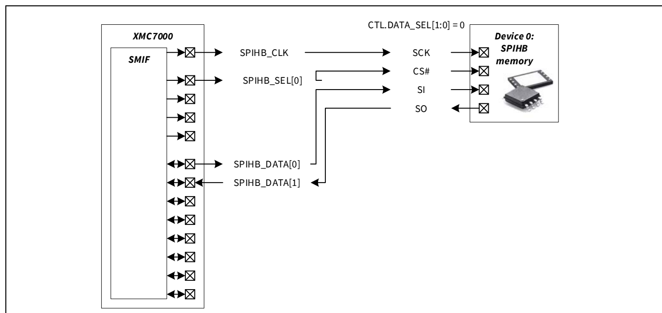
Figure 30-8. Single SPI device 0 connected to SPIHB_DATA[1:0]
