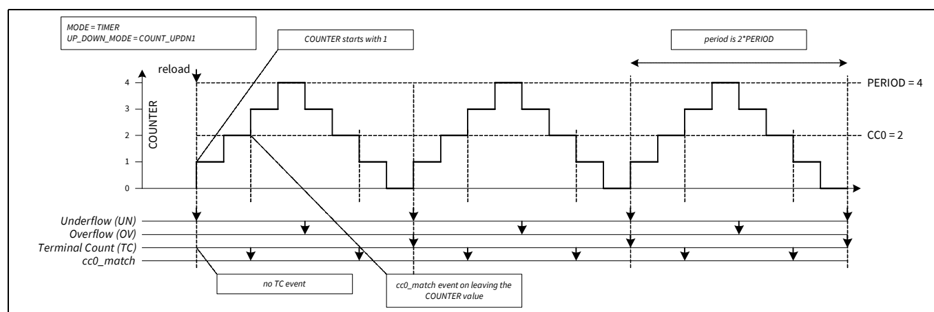
Figure 25-15. Timer in up/down counting mode 1
