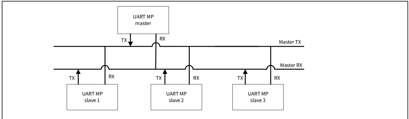
Figure 23-27. UART MP mode bus connections
