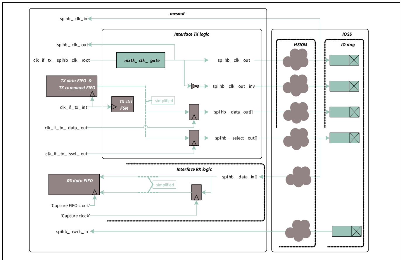
Figure 30-27. TX/RX interface to external memory devices
