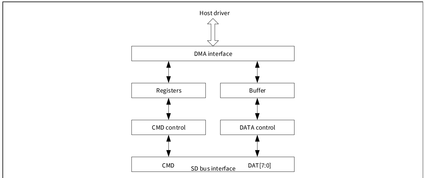
Figure 31-4. Data flow
