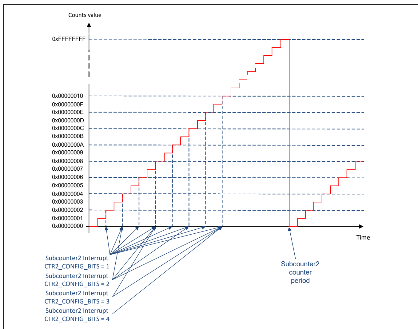
Figure 20-9. Subcounter 2 operation
