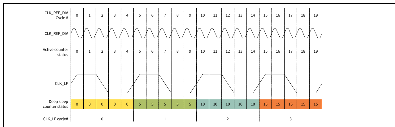
Figure 27-3. Active and Deep sleep counter status with ratio = 5
