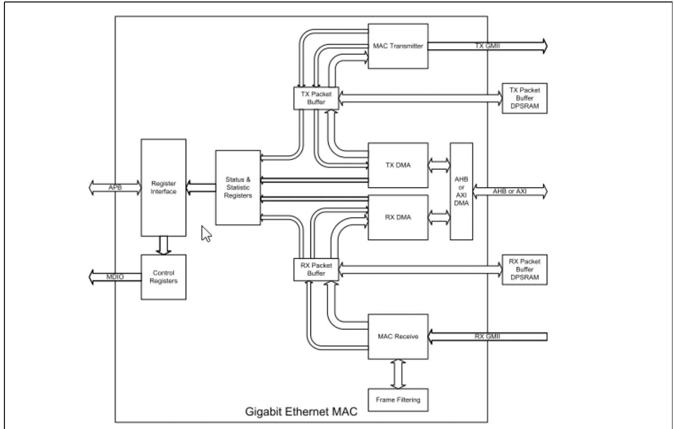
Figure 29-2. EMAC data path structure
