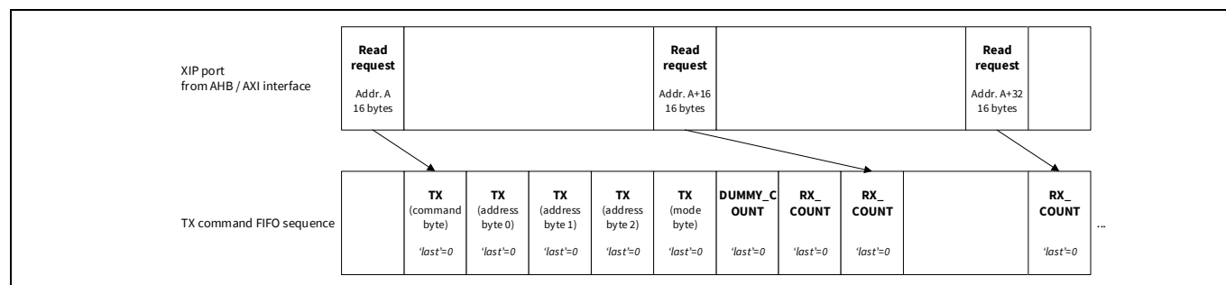
Figure 30-4. Read sequence with continuous merging enabled - merging always possible
