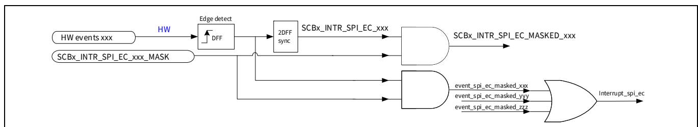
Figure 23-4. SCBx_INTR_SPI_EC and interrupt_spi_ec generation
