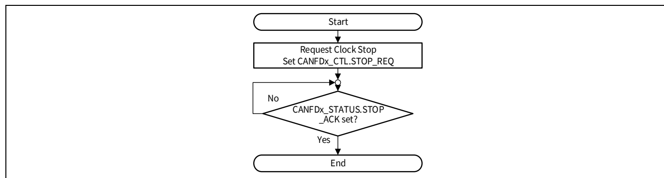
Figure 24-29. Clock stop request procedure
