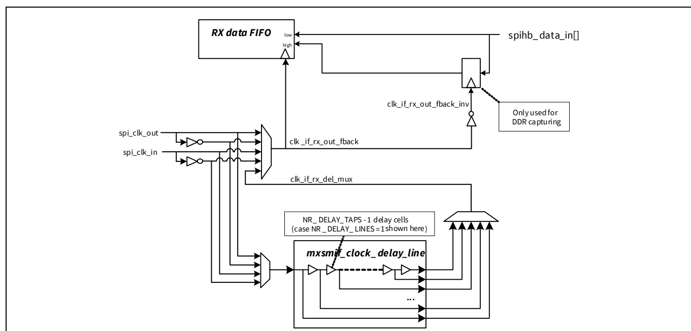
Figure 30-28. Output/feedback clock-based capture scheme
