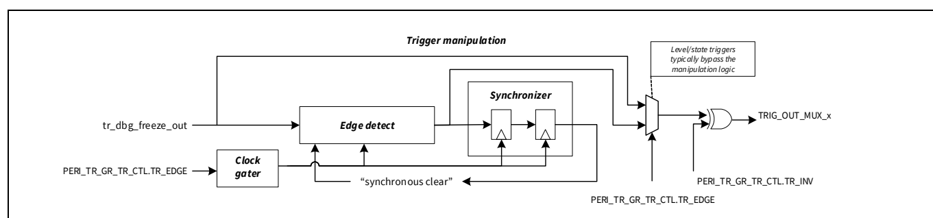
Figure 28-9. Trigger manipulation
