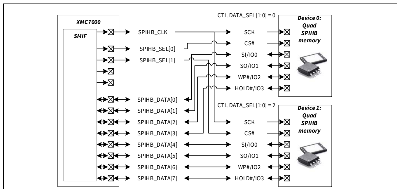
Figure 30-16. Quad SPI device 0 to SPIHB_DATA[3:0], Quad SPI device 1 connected to SPIHB_DATA[7:4]
