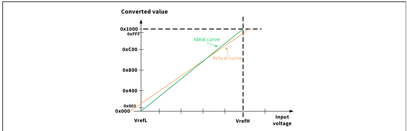
Figure 33-10. Analog to digital transfer curve
