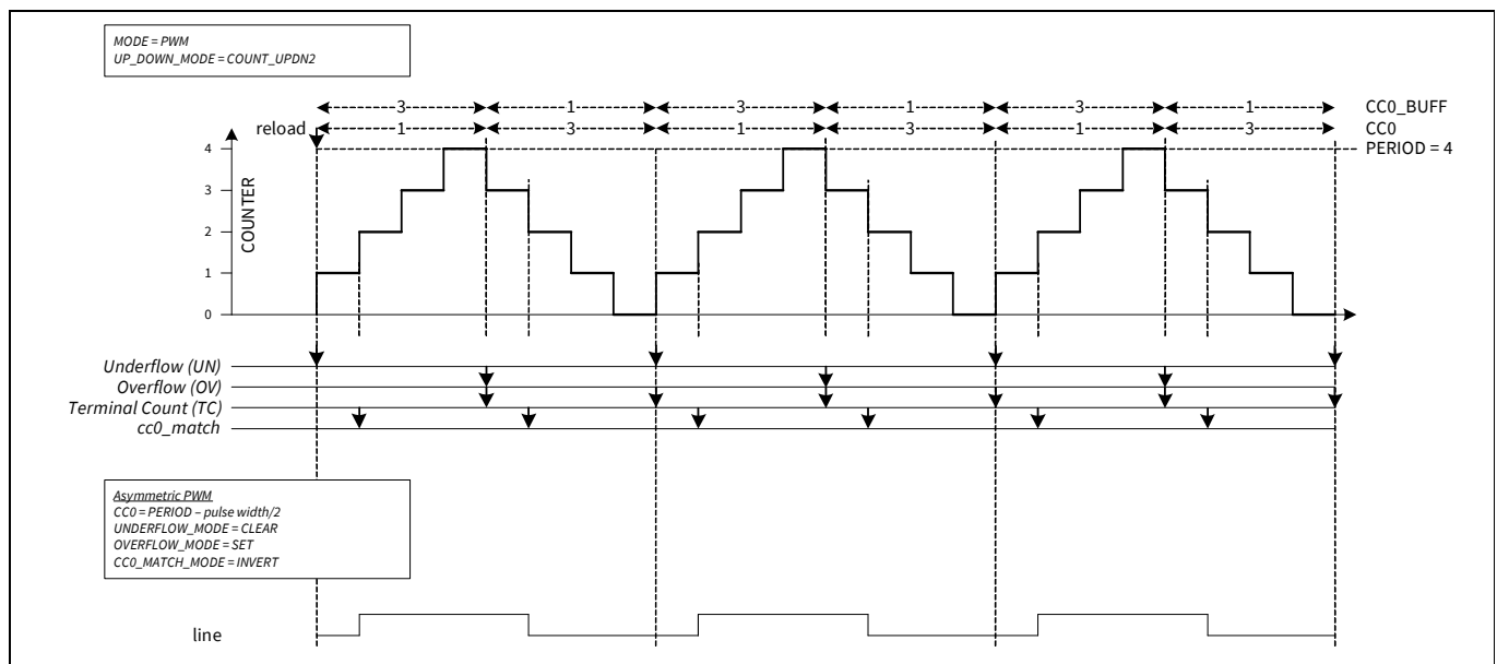
Figure 25-50. Asymmetric PWM
