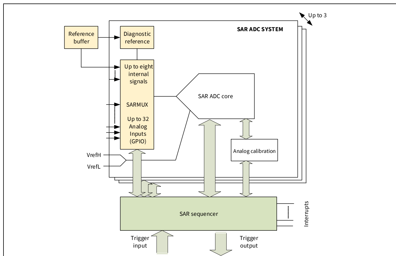
Figure 33-1. SAR ADC system block diagram
