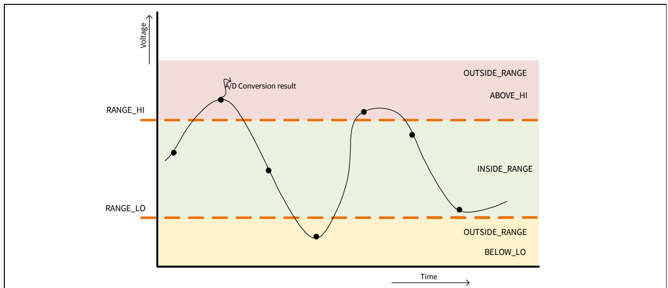
Figure 33-6. Range detection, threshold, and events
