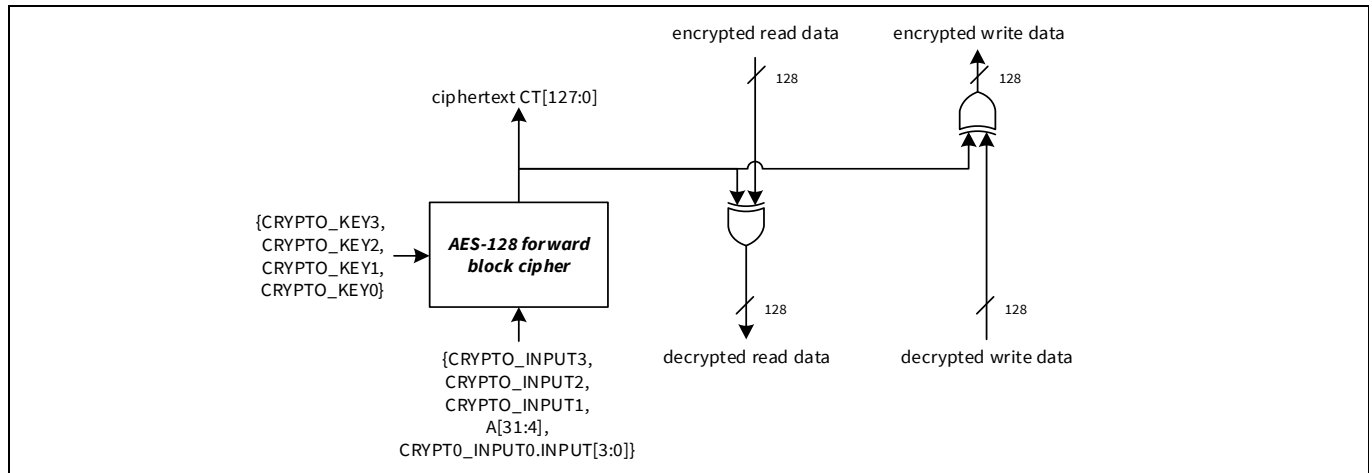
Figure 30-26. Cryptography in XIP mode
