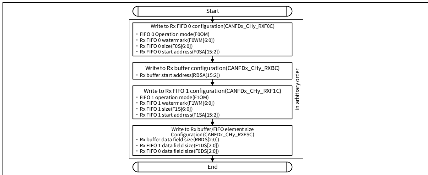
Figure 24-37. RX FIFO and RX buffer configuration
