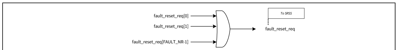
Figure 15-2. Fault reset
