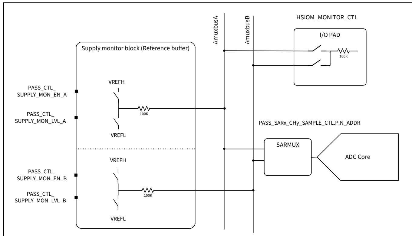
Figure 33-14. Power monitoring block diagram
