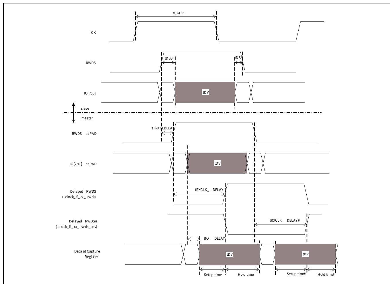
Figure 30-30. Capturing data with RWDS
