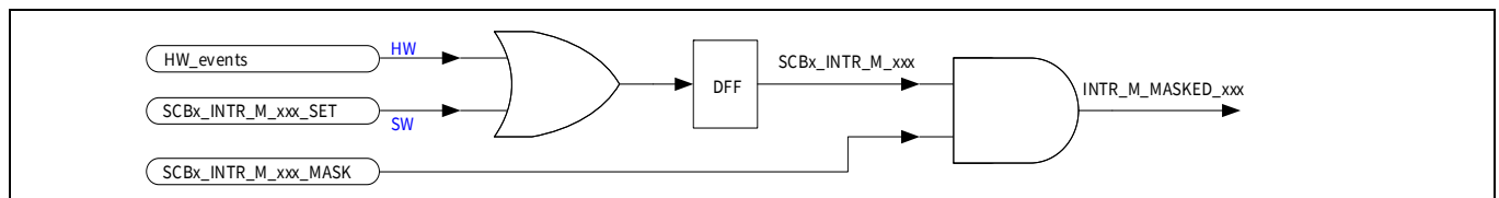
Figure 23-3. SCBx_INTR_M generation
