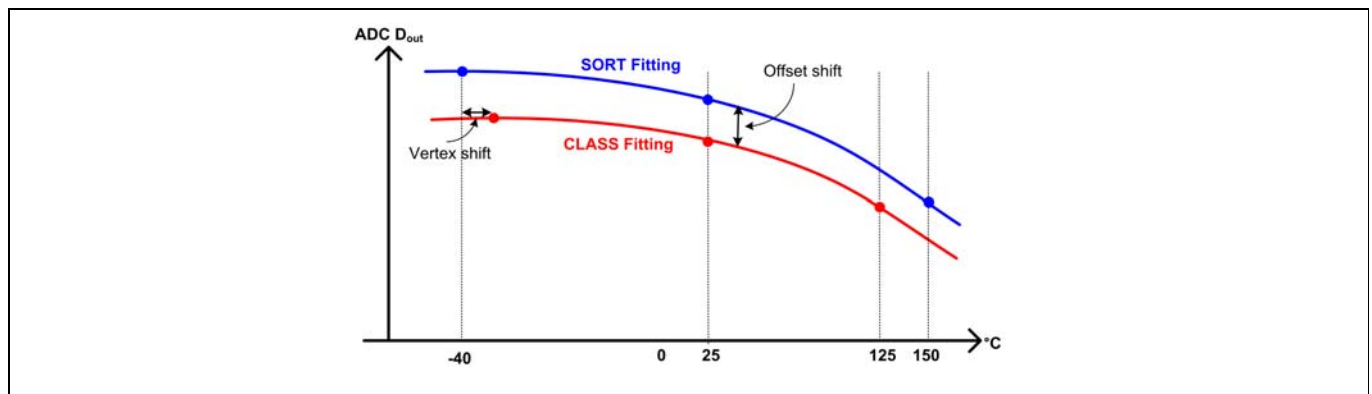
Figure 33-12. SORT and CLASS relationship
