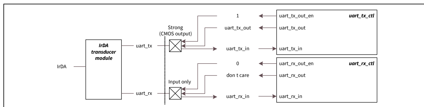
Figure 23-35. IrDA mode I/O pad connections
