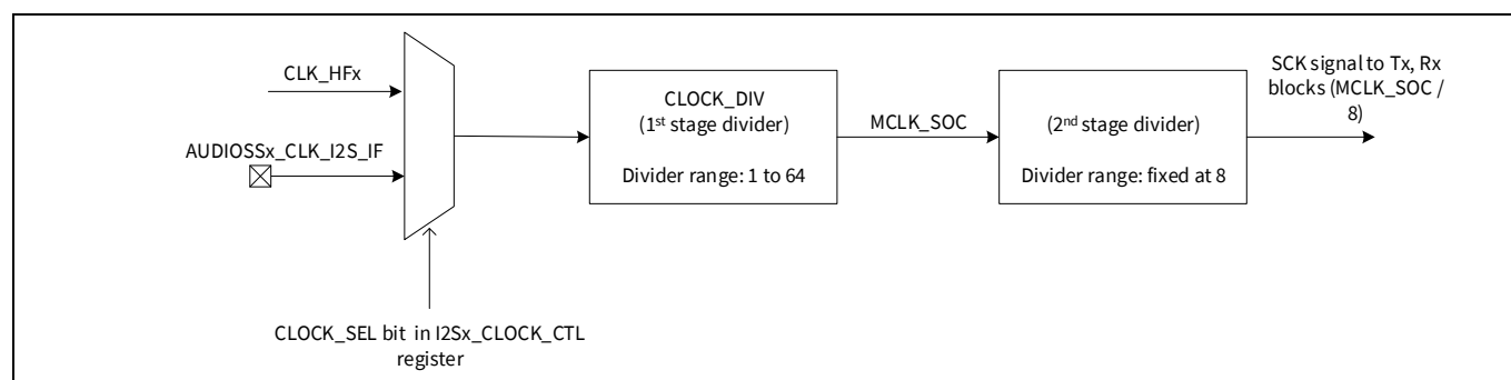
Figure 32-6. Clocking divider structure
