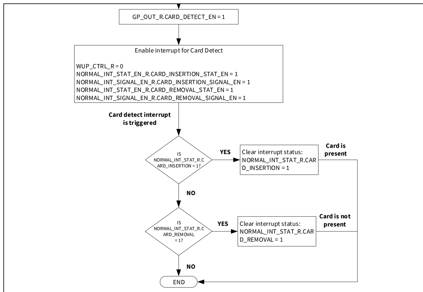
Figure 31-8. Card detection through interrupt
