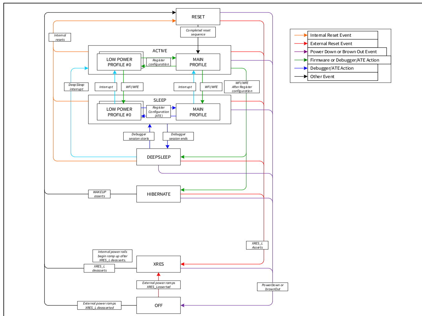
Figure 17-1. Power mode transition
