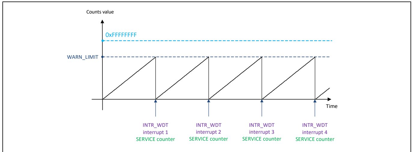
Figure 20-4. WDT counter operation with WARN interrupt only
