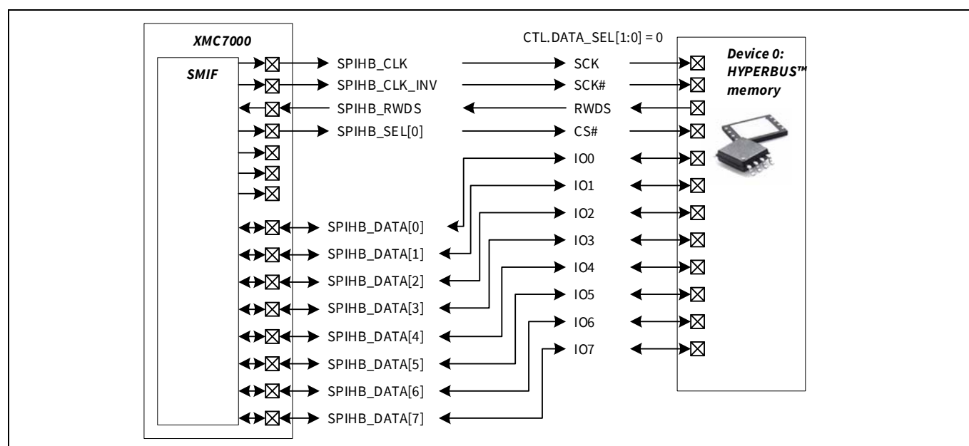
Figure 30-18. HYPERBUS™ SPI device 0 to SPIHB_DATA[7:0]
