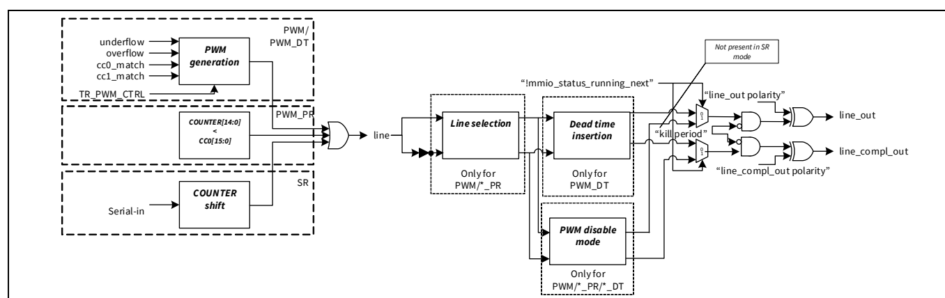
Figure 25-7. PWM output generation process in PWM/PWM_DT/PWM_PR/SR mode
