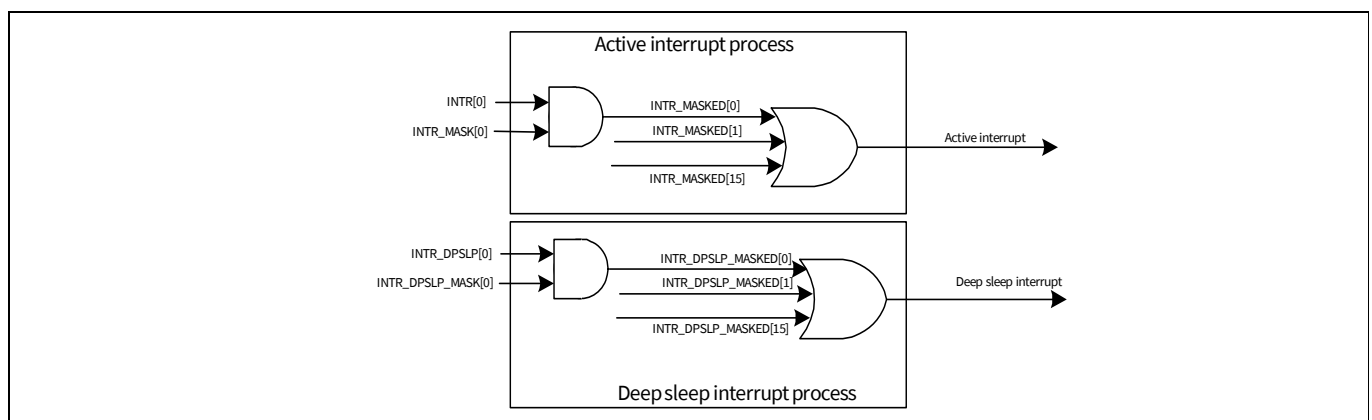
Figure 27-5. Interrupt process
