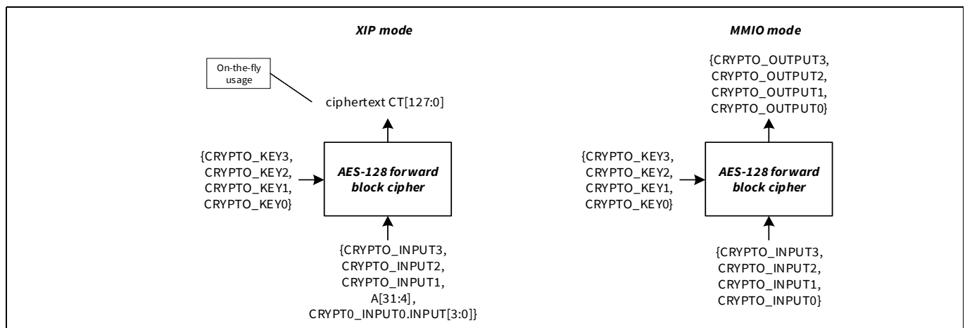
Figure 30-25. Cryptography in XIP and MMIO mode
