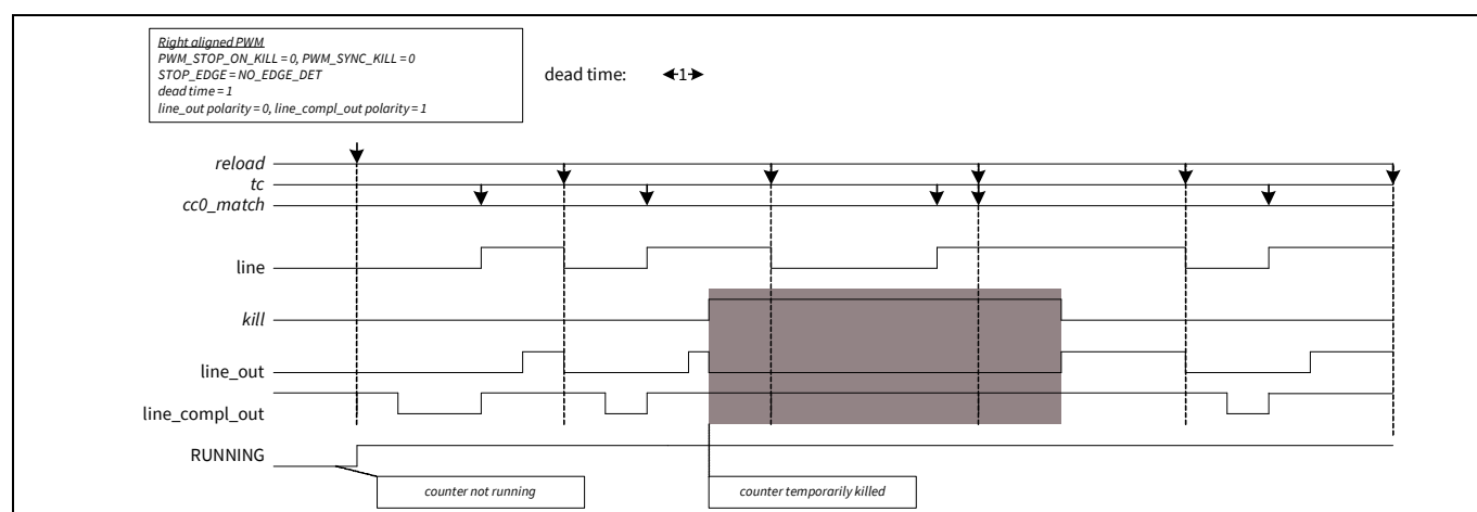
Figure 25-61. Dead time and kill
