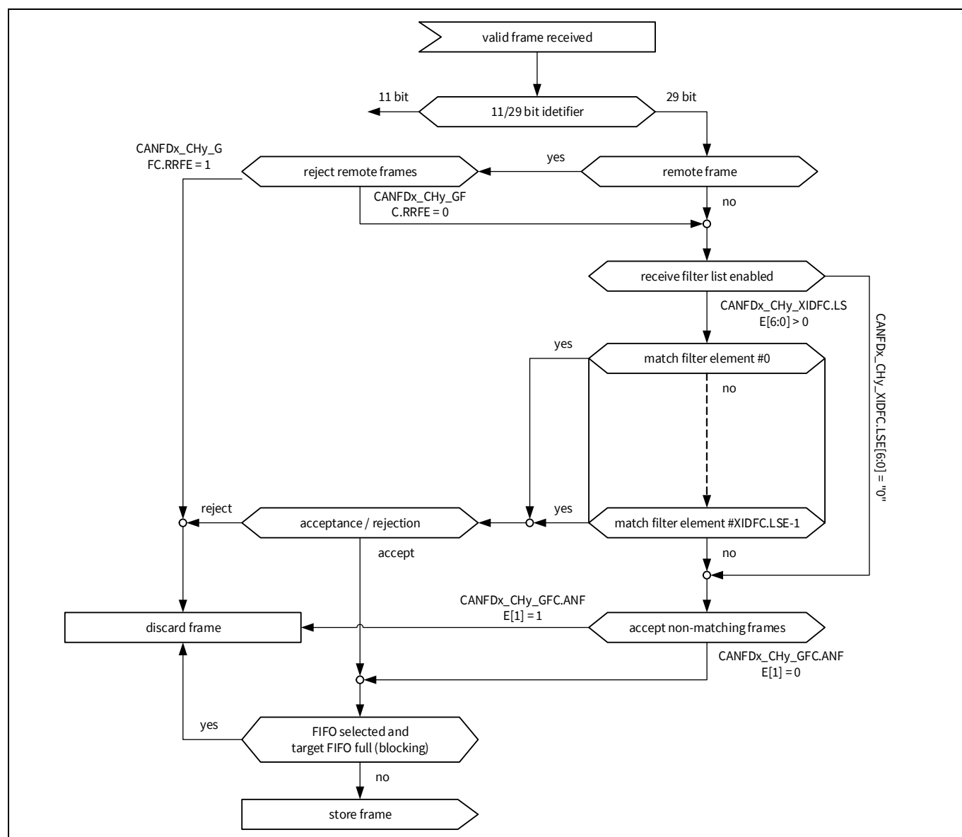
Figure 24-8. Extended message ID filter path
