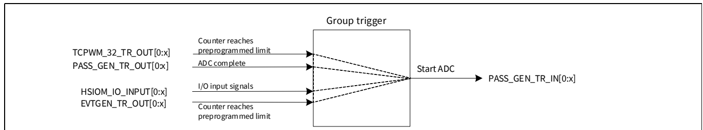
Figure 28-6. Example of group trigger
