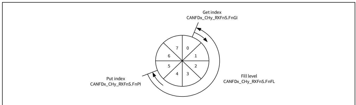
Figure 24-9. RX FIFO status
