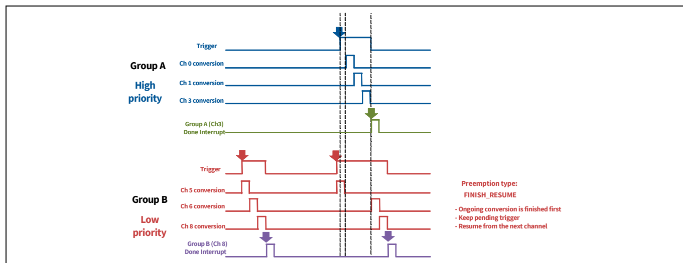
Figure 33-8. Preemption types: A low priority group B behavior with FINISH_RESUME preemption type
