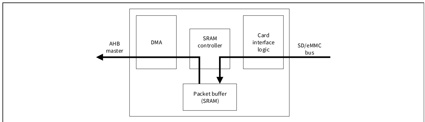
Figure 31-3. Data flow in a read transfer
