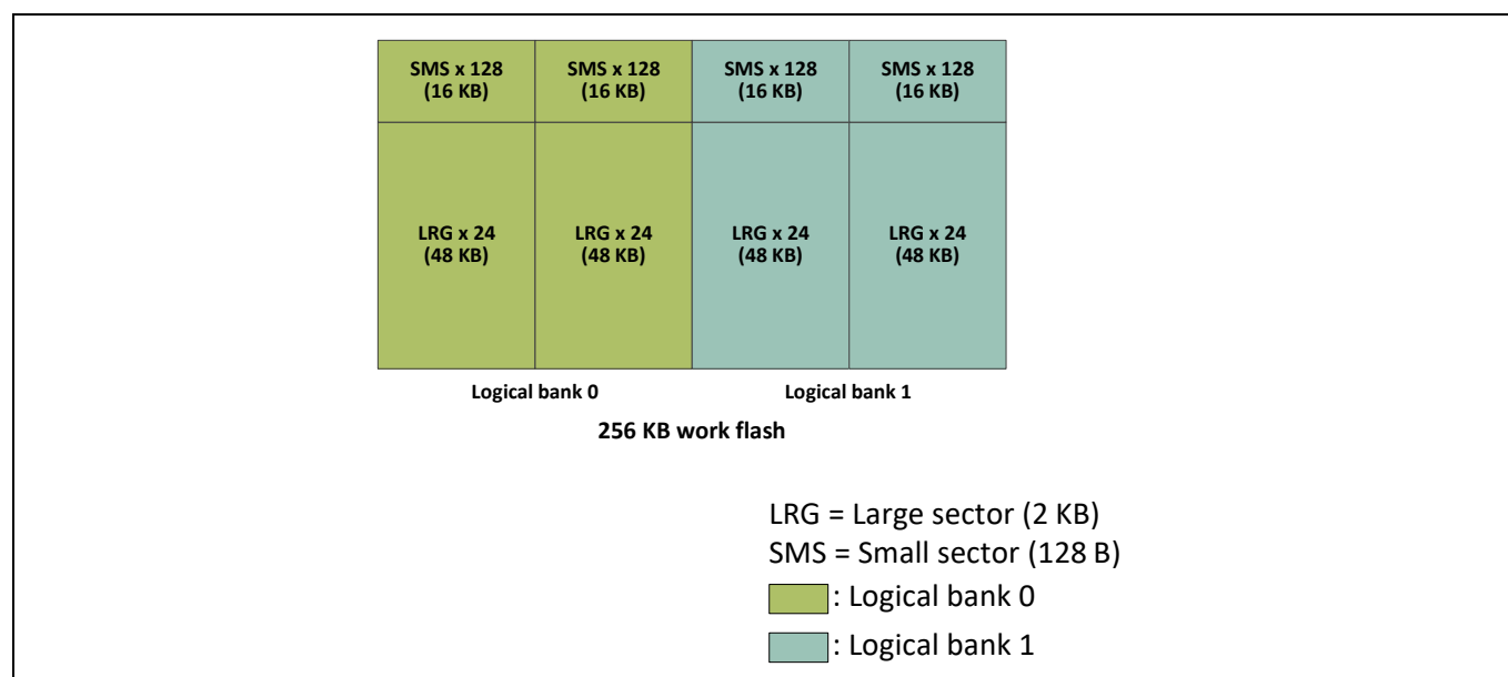
Figure 9-4. Work flash array organization
