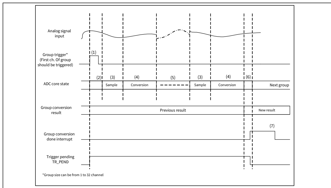
Figure 33-3. ADC conversion timing flow
