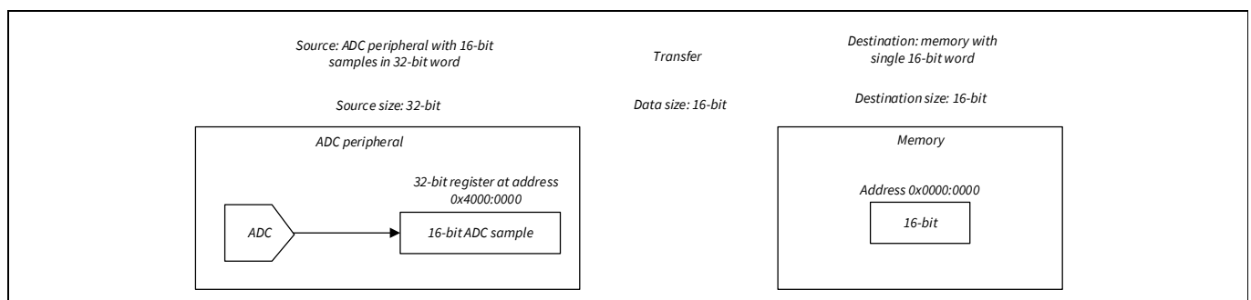
Figure 7-7. Single transfer
