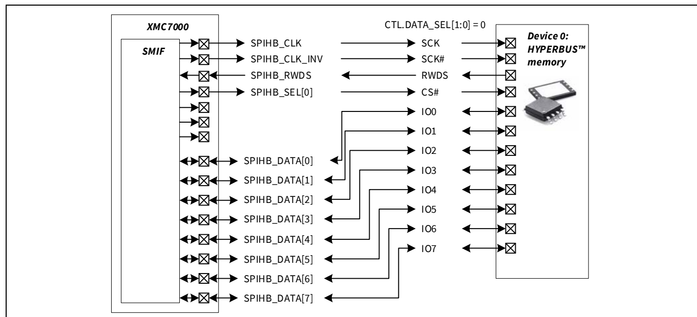
Figure 30-21. HYPERBUS™ device connection
