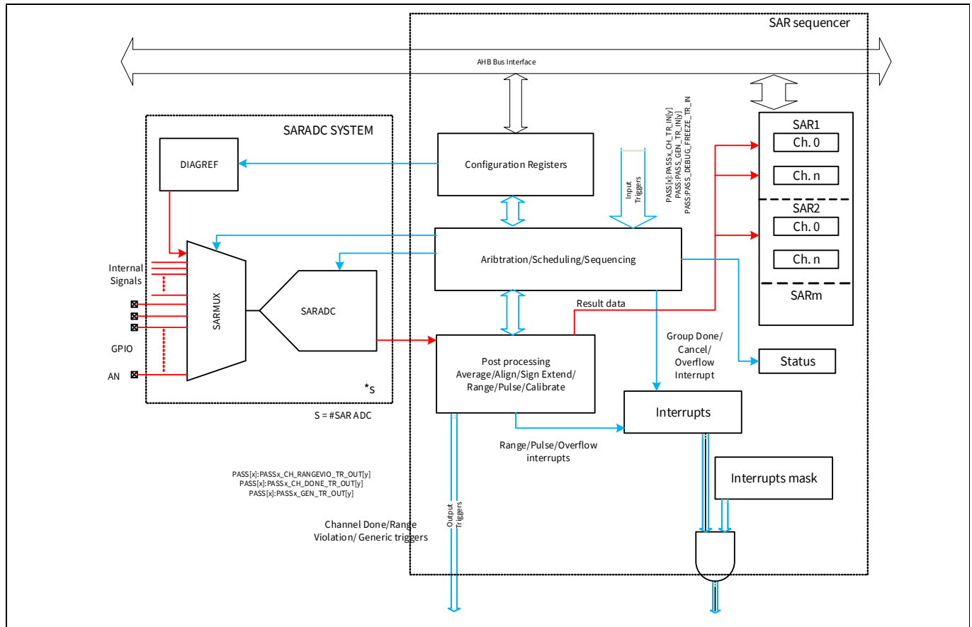
Figure 33-5. SAR sequencer block diagram
