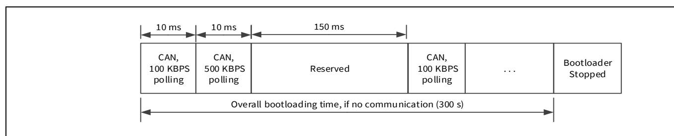
Figure 36-3. Polling CAN with no bootloader commands
