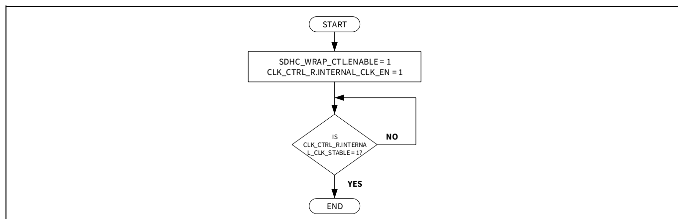
Figure 31-6. SDHC enable sequence
