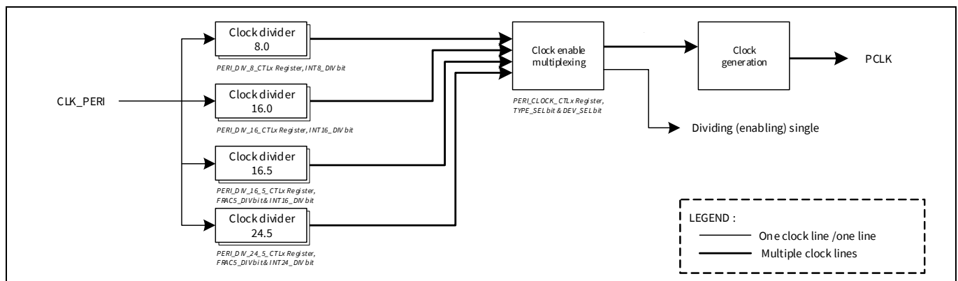
Figure 18-8. Peripheral clock divider
