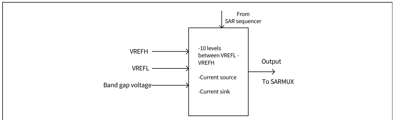
Figure 33-13. Diagnostic reference block diagram
