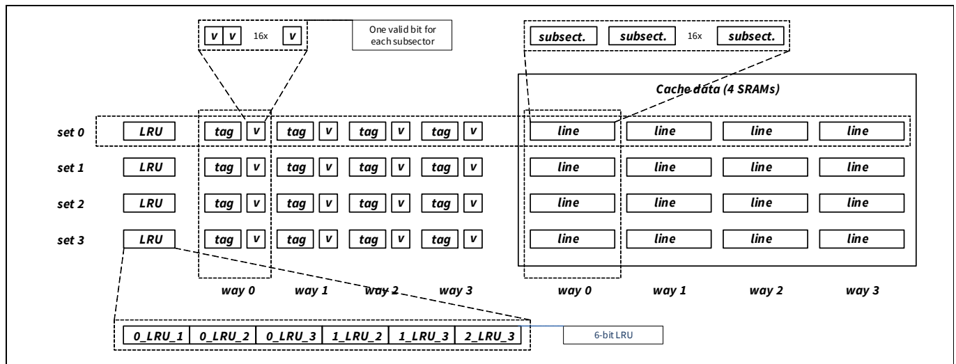
Figure 30-24. Cache organization
