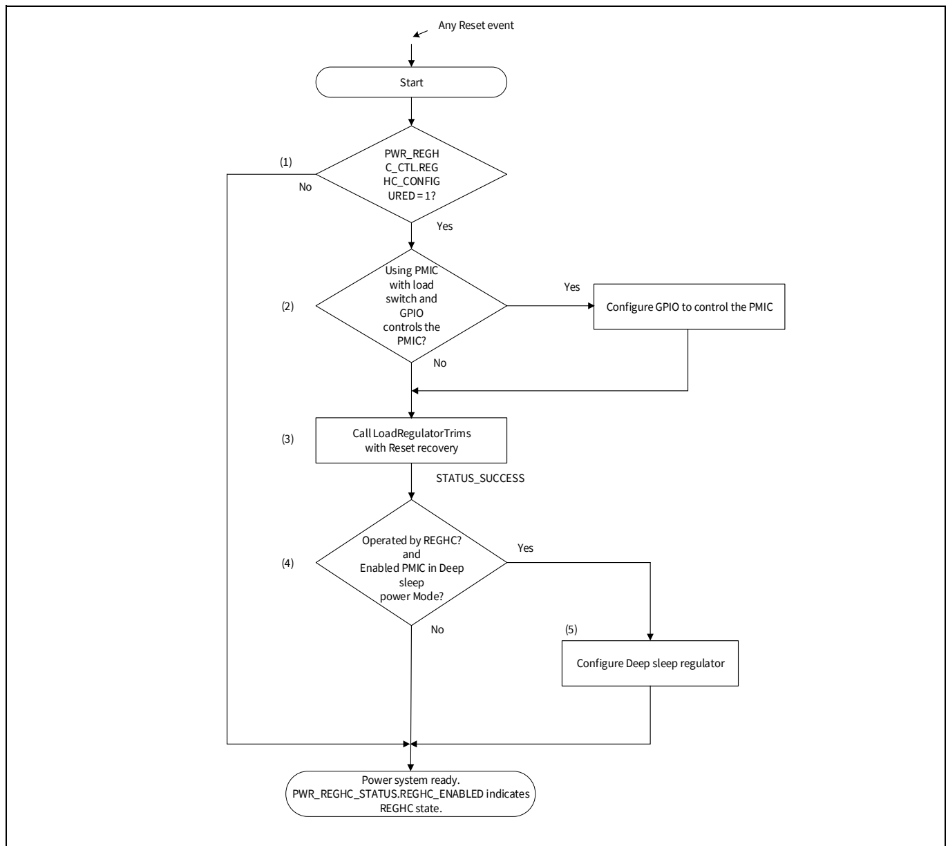
Figure 16-7. Reset recovery flow
