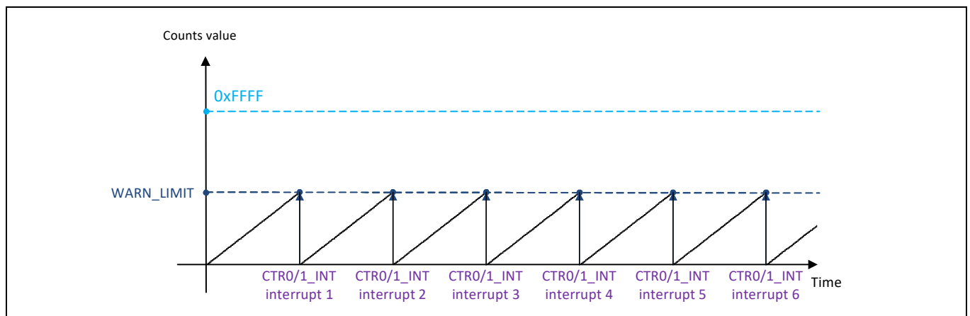
Figure 20-7. Subcounter 0/1 operation with WARN interrupt only ( MCWDTx_CTRy_CONFIG.AUTO_SERVICE = 1 )
