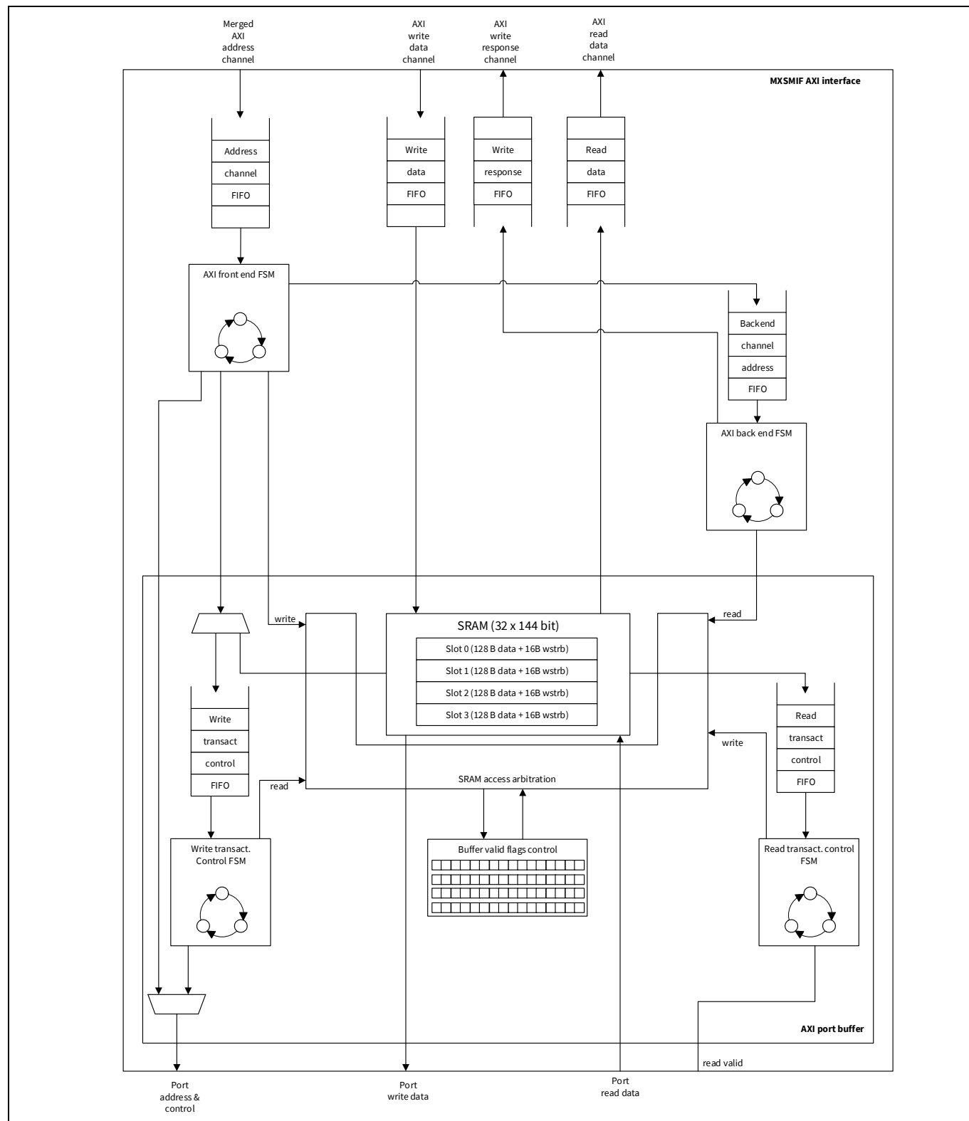
Figure 30-23. AXI slave interface block
