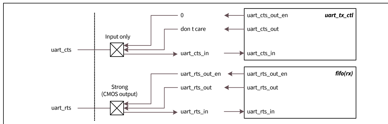
Figure 23-32. Standard UART mode, flow control I/O pad connection
