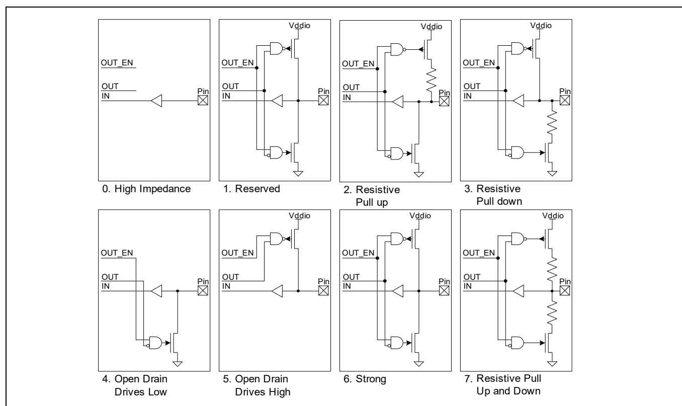
Figure 22-4. GPIO port, drive mode block diagram
