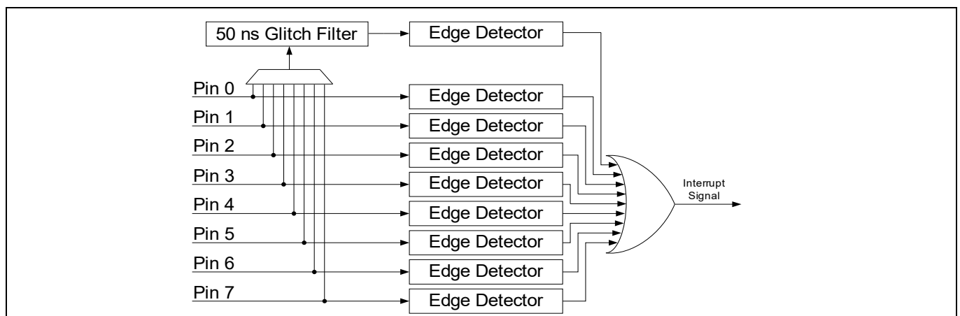
Figure 22-7. GPIO edge detect block architecture
