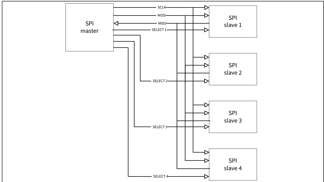
Figure 23-6. SPI example
