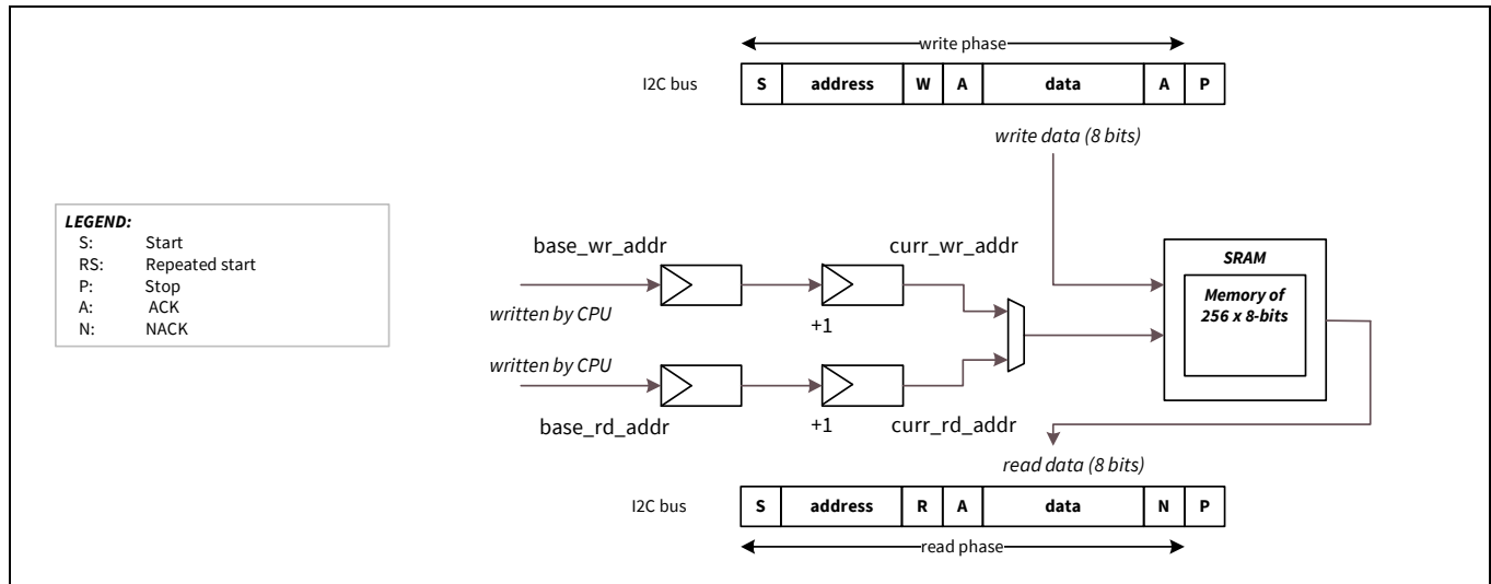
Figure 23-40. I 2 C command-response mode
