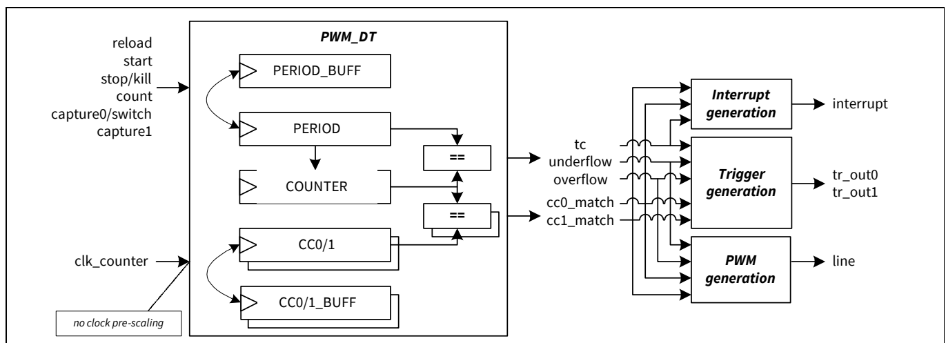
Figure 25-59. PWM with dead time functionality
