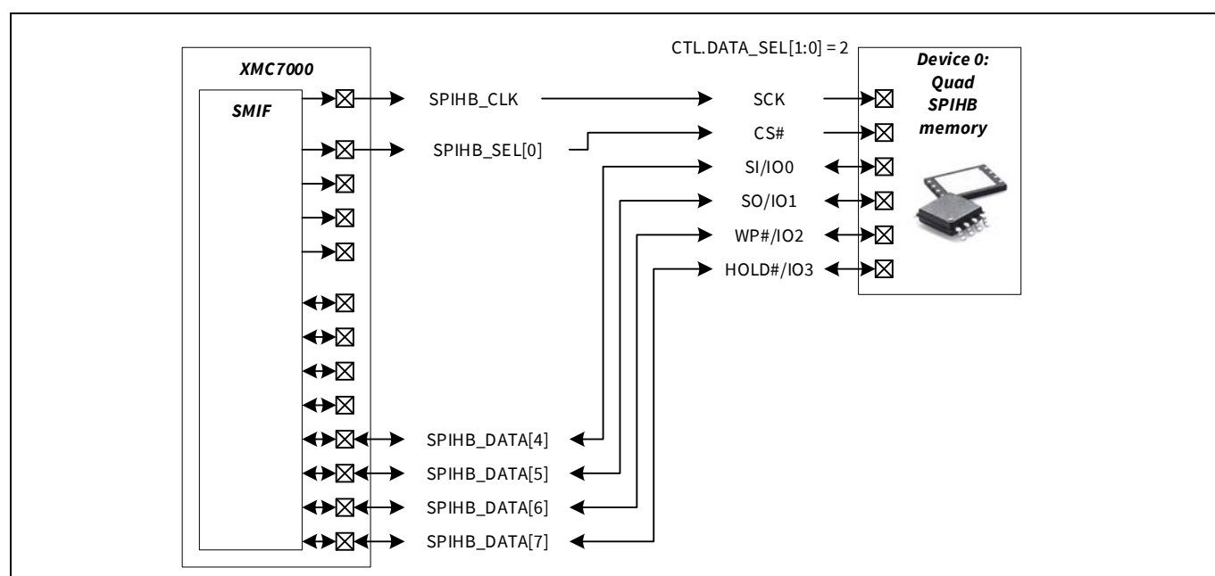
Figure 30-13. Quad SPI device 0 connected to SPIHB_DATA[7:4]
