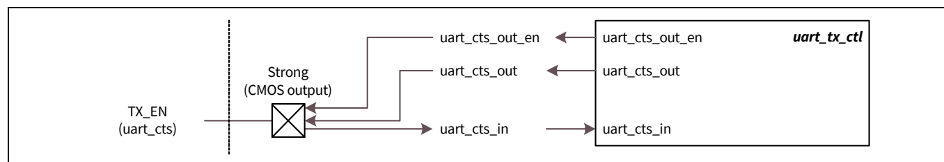
Figure 23-33. Standard UART mode, CTS Reused as TX_EN for RS485
