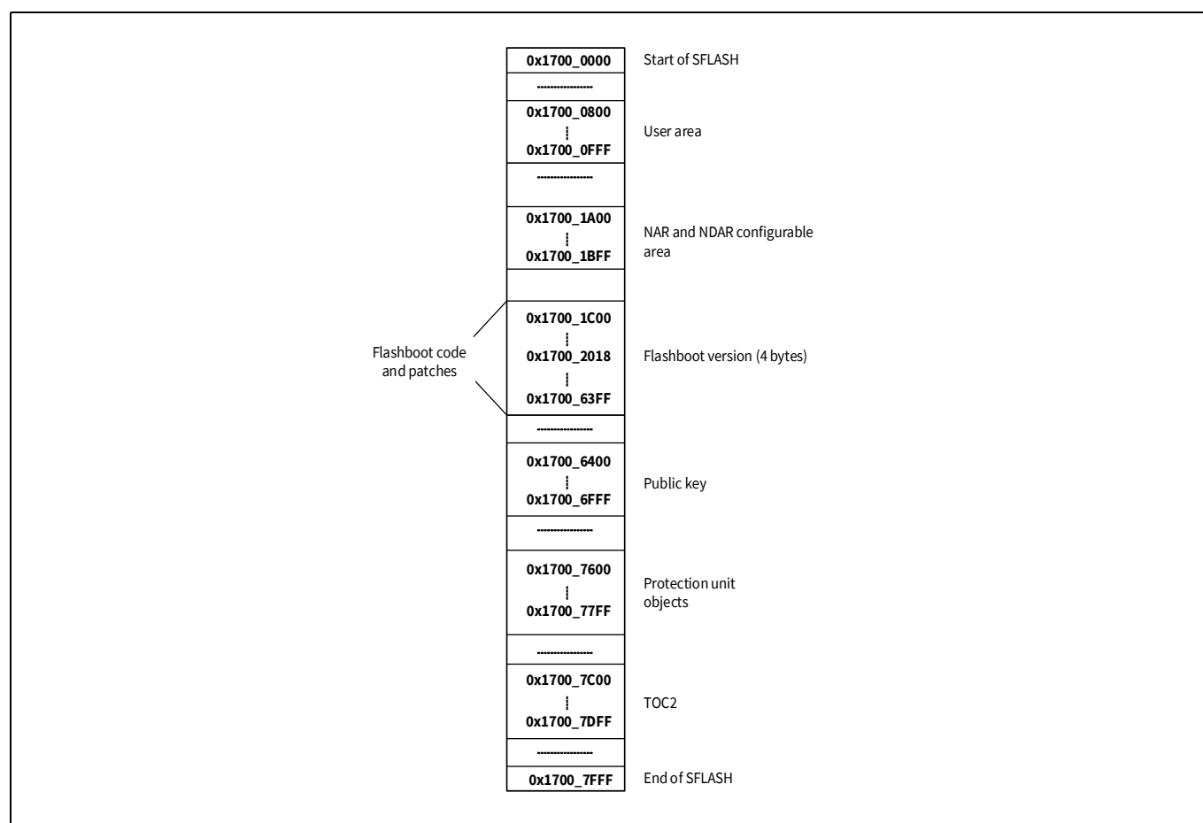
Figure 36-6. SFlash address mapping
