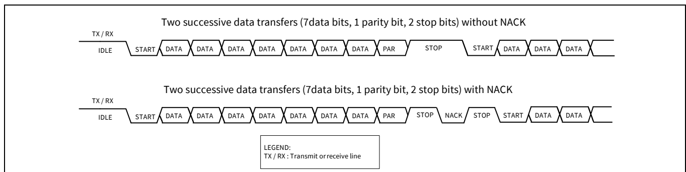
Figure 23-29. SmartCard example
