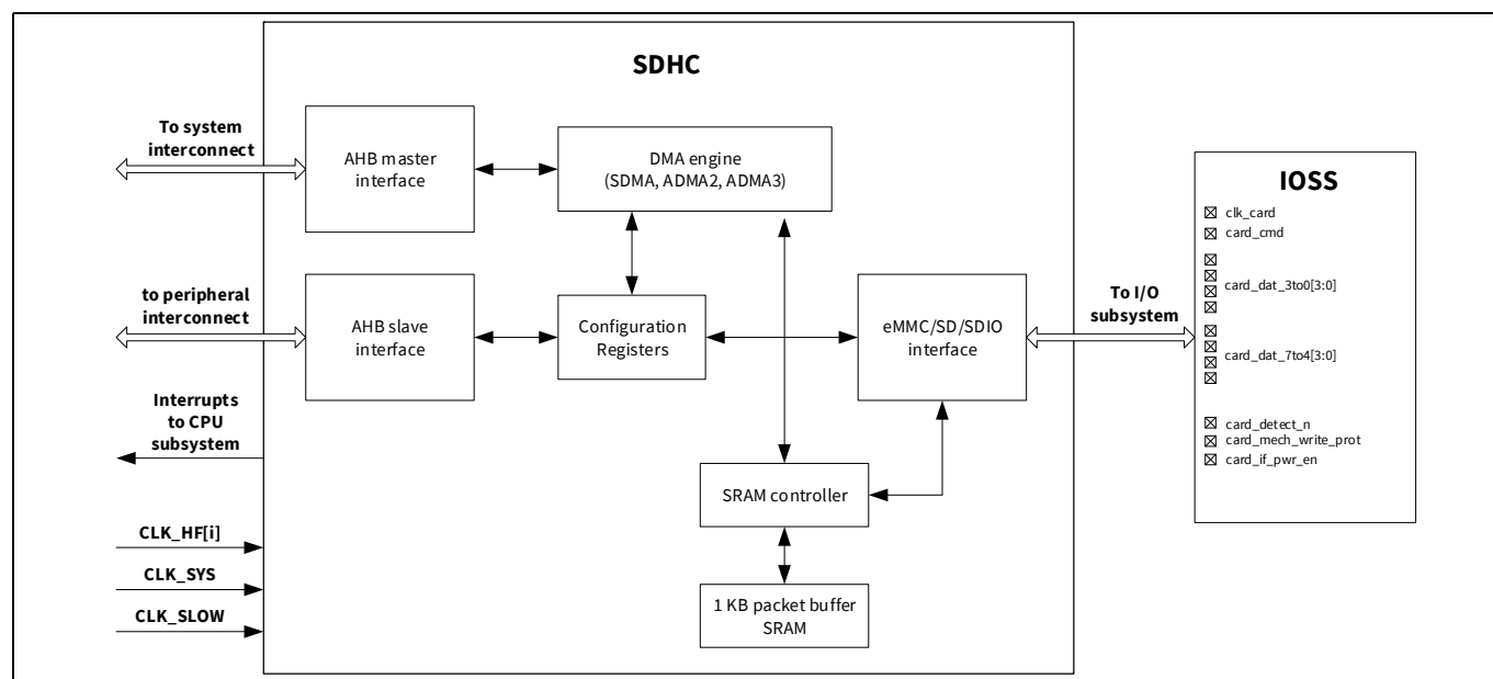
Figure 31-2. SDHC block diagram
