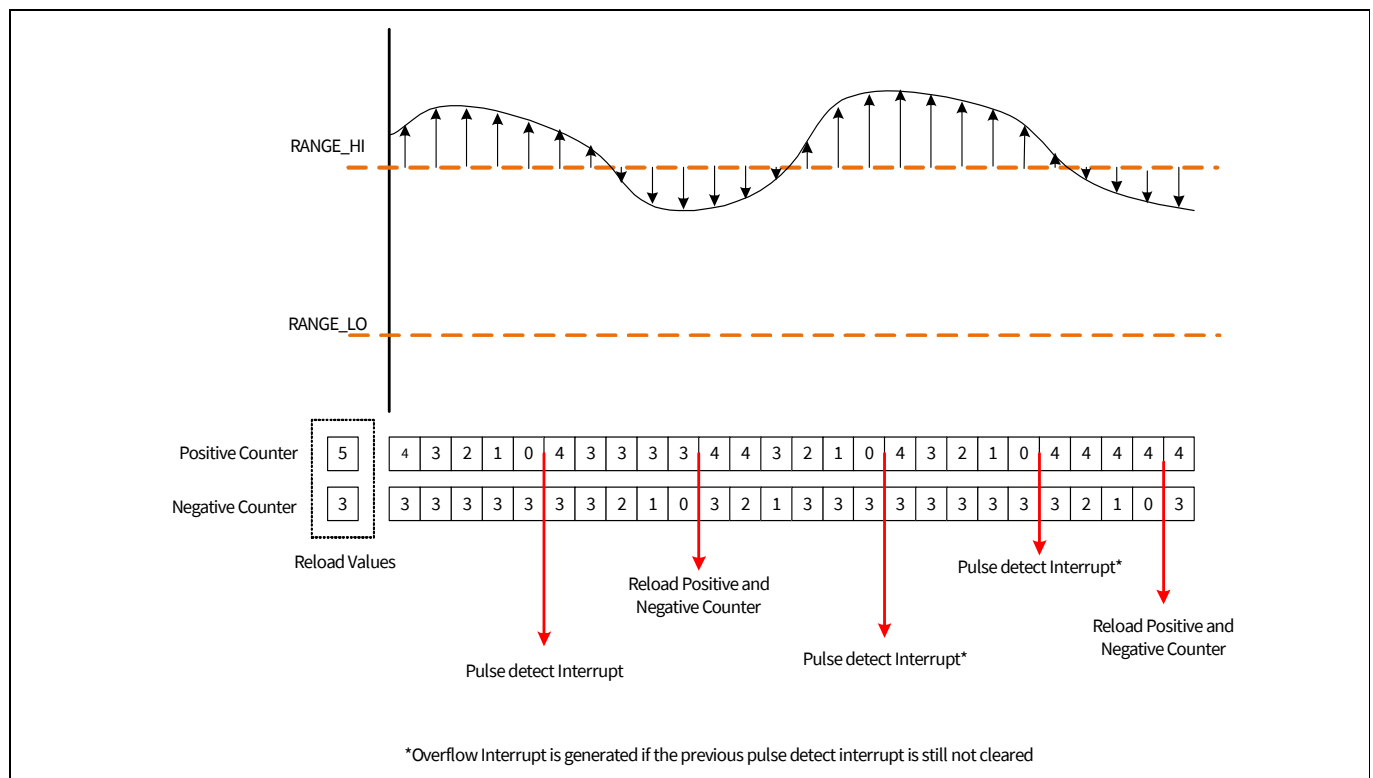
Figure 33-7. Pulse detection
