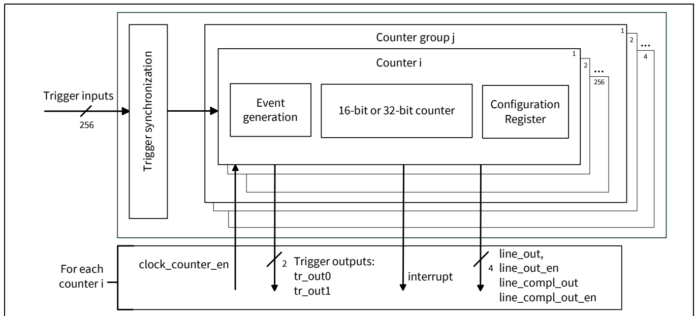
Figure 25-1. TCPWM block diagram
