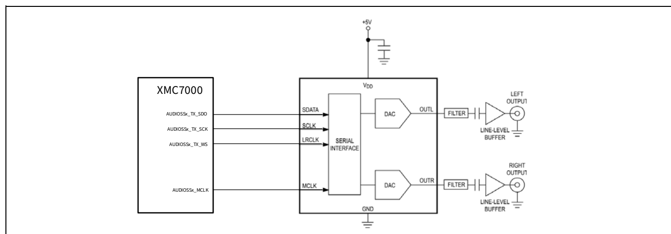
Figure 32-11. MCLK output signal for external audio codec
