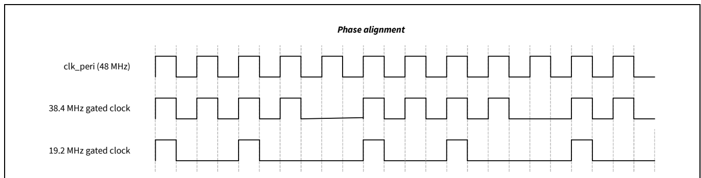
Figure 18-11. Phase-aligned fractional dividers
