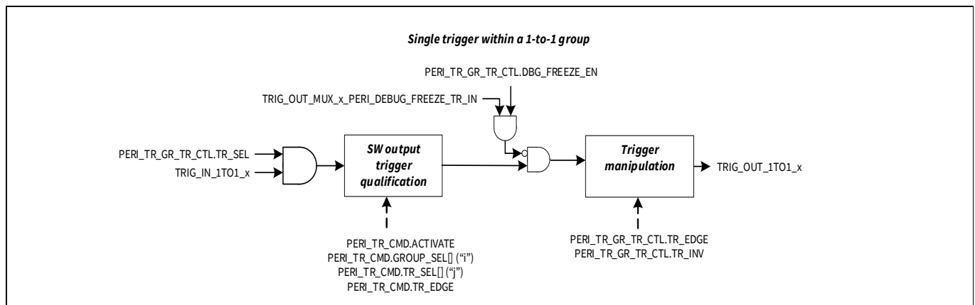
Figure 28-7. One-to-one trigger group
