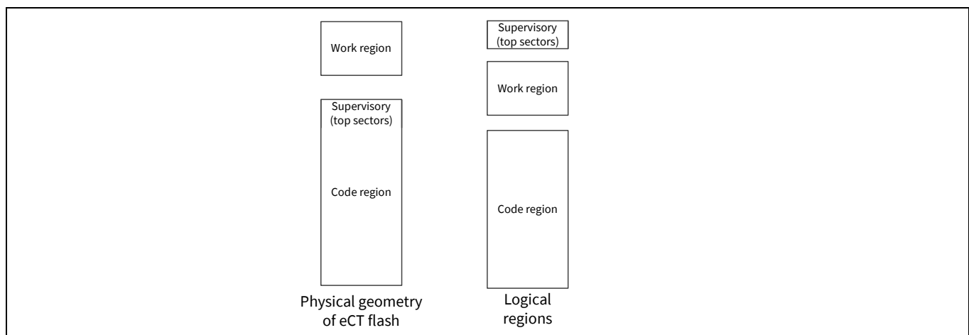
Figure 8-5. Regions of eCT flash
