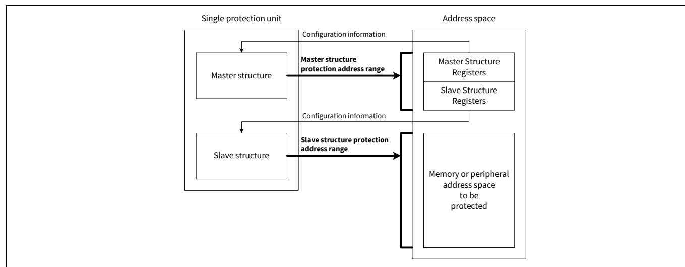
Figure 6-2. Concept of master and slave structure
