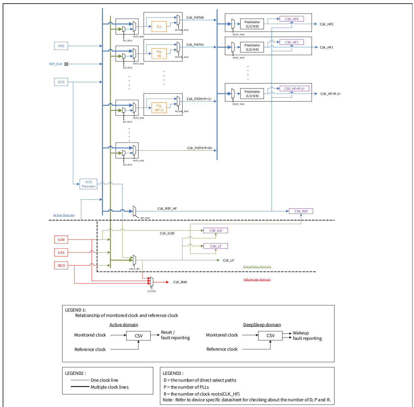
Figure 18-12. CSV diagram
