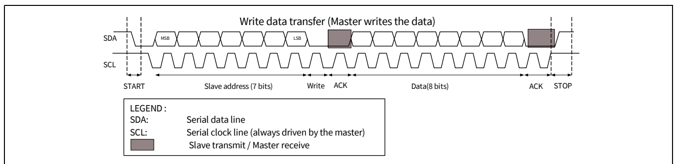
Figure 23-37. Master write data transfer
