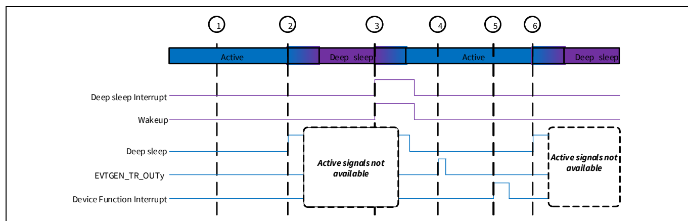
Figure 27-6. Use case waveform
