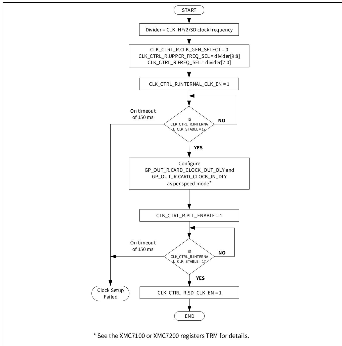
Figure 31-10. Clock setup
