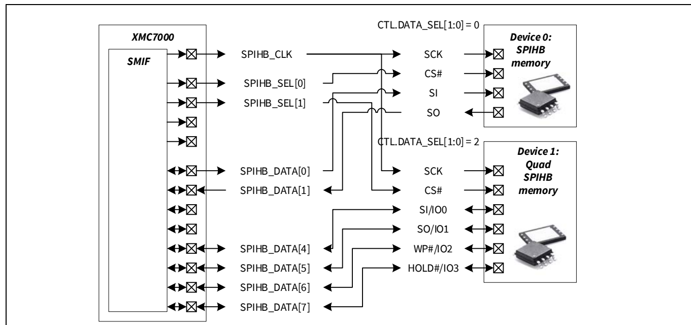
Figure 30-14. Single SPI device 0 to SPIHB_DATA[1:0], Quad SPI device 1 connected to SPIHB_DATA[7:4]
