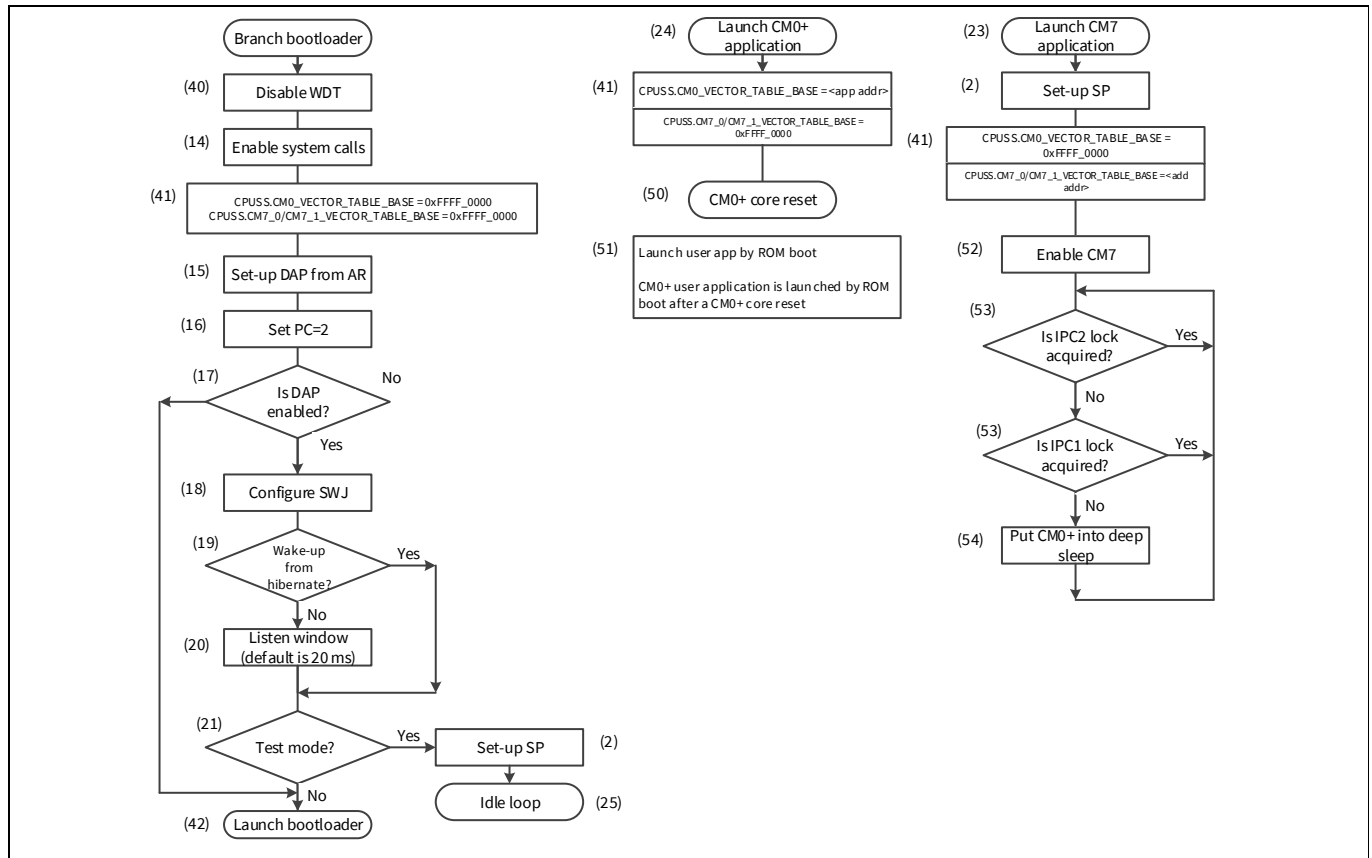
Figure 36-7. Flash boot flow
