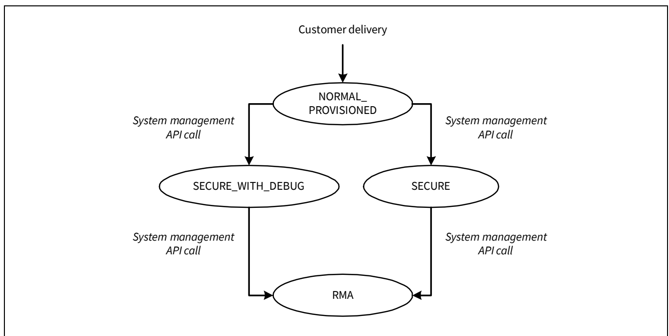
Figure 13-1. XMC7000 life cycle stage transitions
