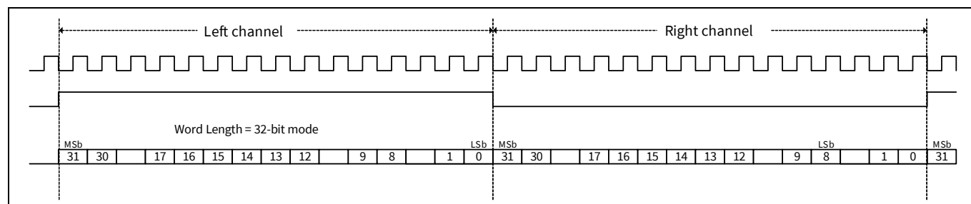
Figure 32-3. Left justified digital audio format
