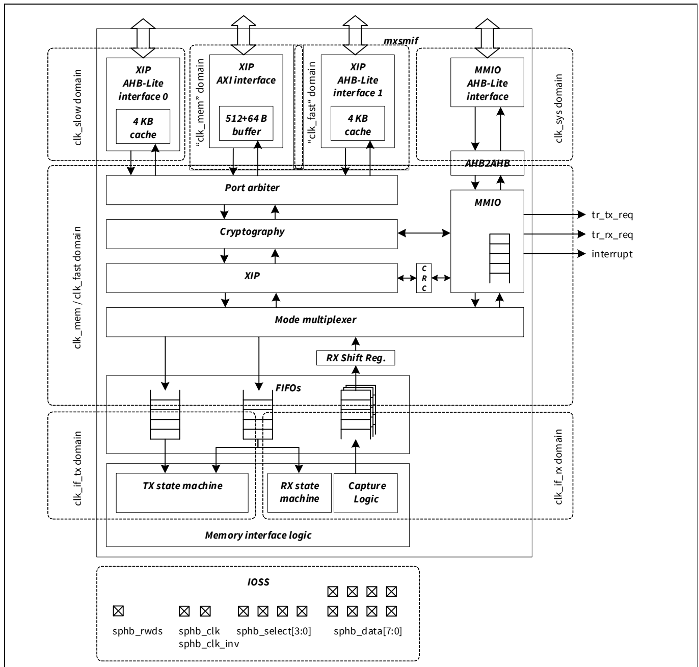
Figure 30-2. High-level block diagram of mxsmif (SMIF)
