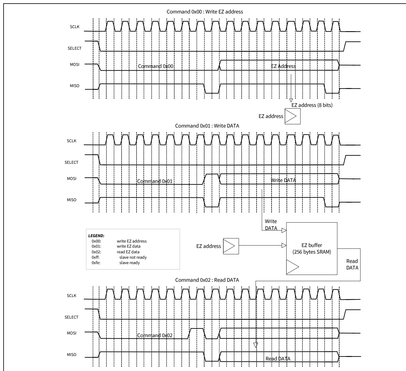
Figure 23-12. EZSPI example
