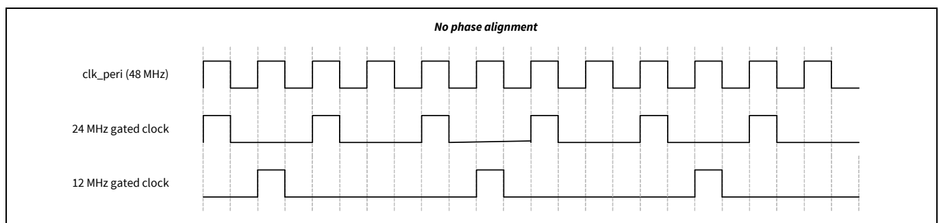
Figure 18-9. Non phase-aligned clock dividers
