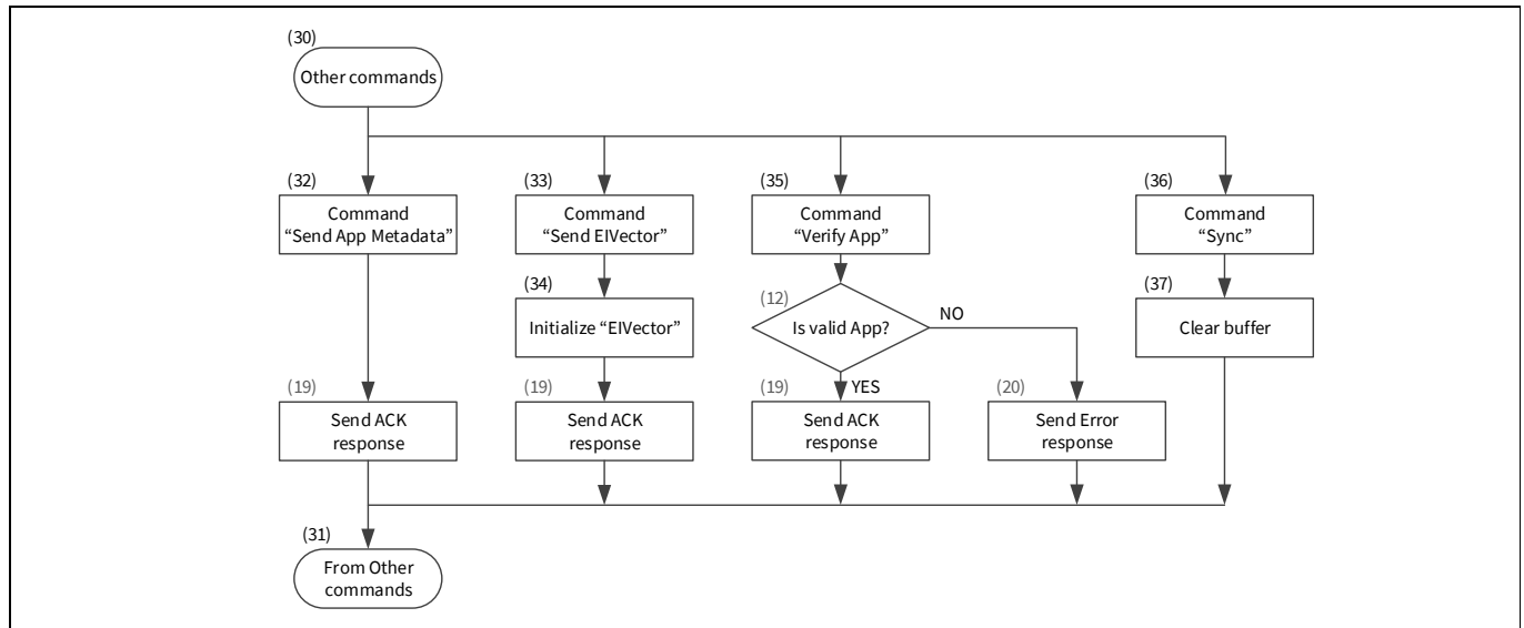
Figure 36-13. Internal bootloader flow
