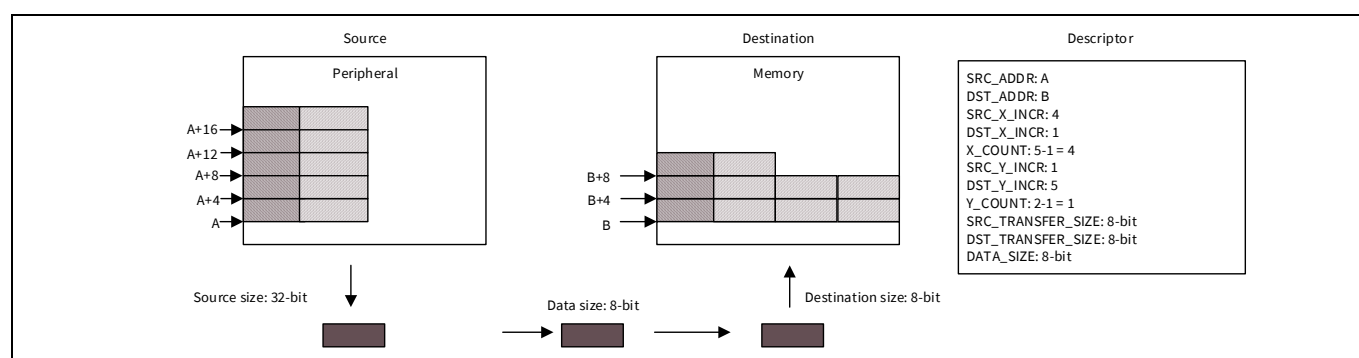
Figure 7-16. M-DMA 2D transfer
