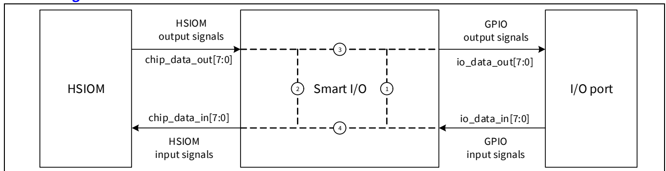
Figure 22-8. Smart I/O interface
