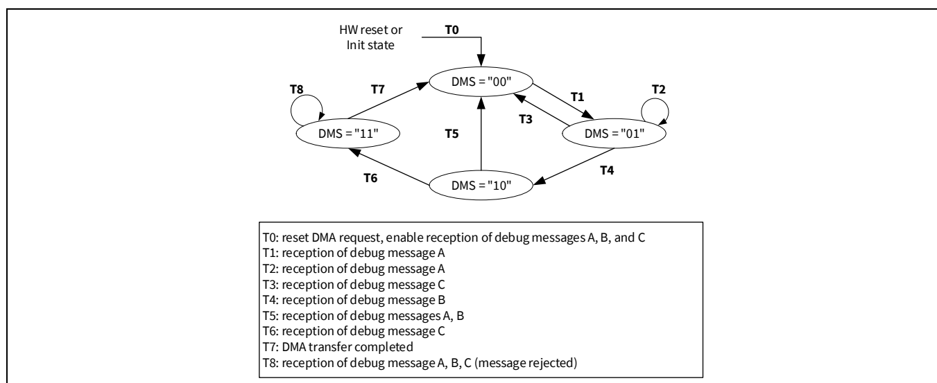
Figure 24-11. Debug message handling state machine
