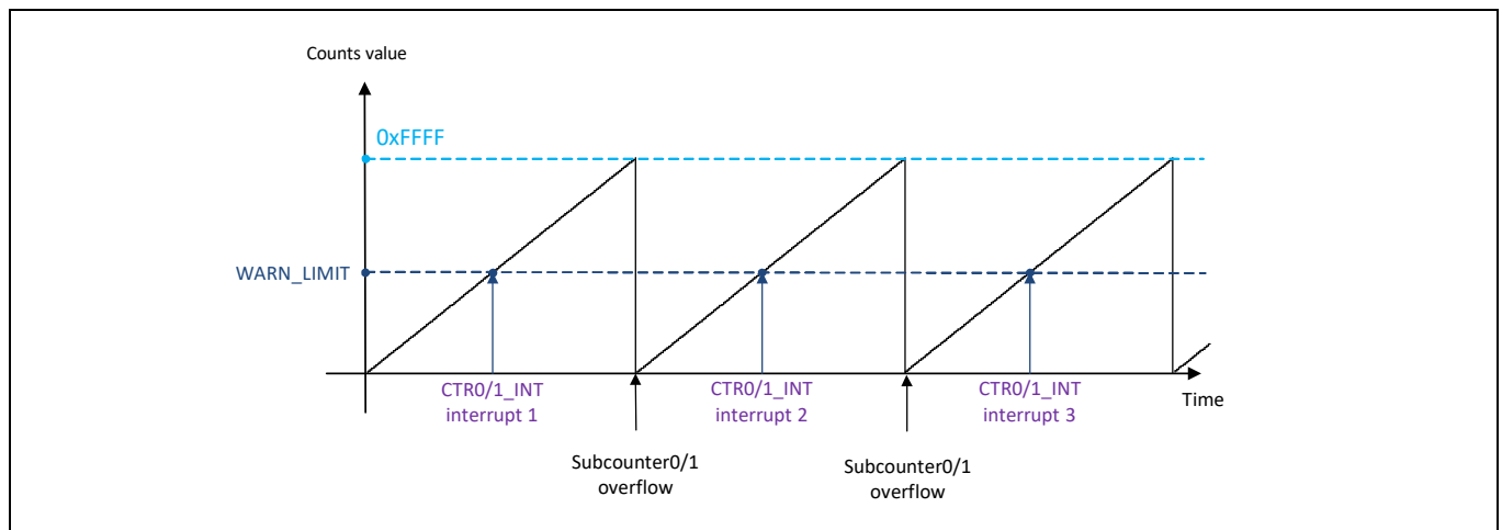
Figure 20-6. Subcounter 0/1 operation with WARN interrupt only ( MCWDTx_CTRy_CONFIG.AUTO_SERVICE = 0 )
