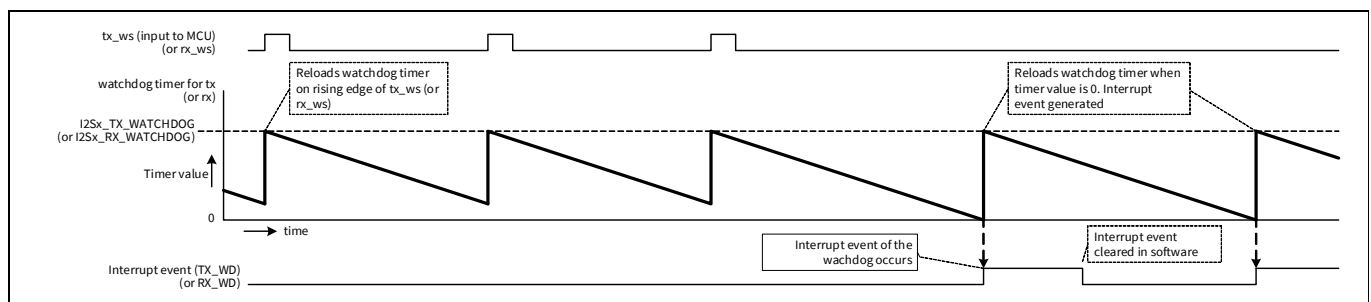
Figure 32-10. Watchdog timer working
