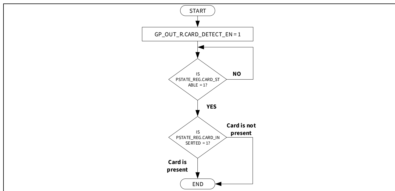
Figure 31-7. Card status check sequence
