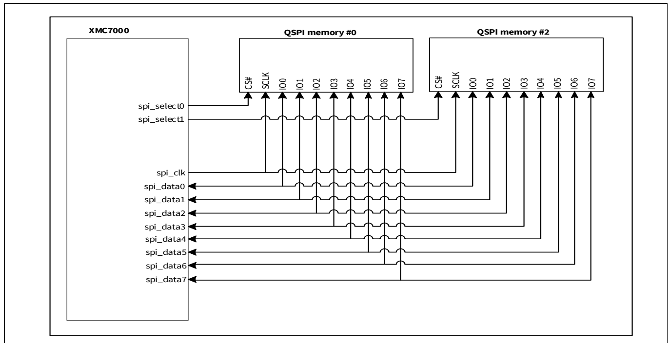
Figure 30-1. QSPI device example system diagram
