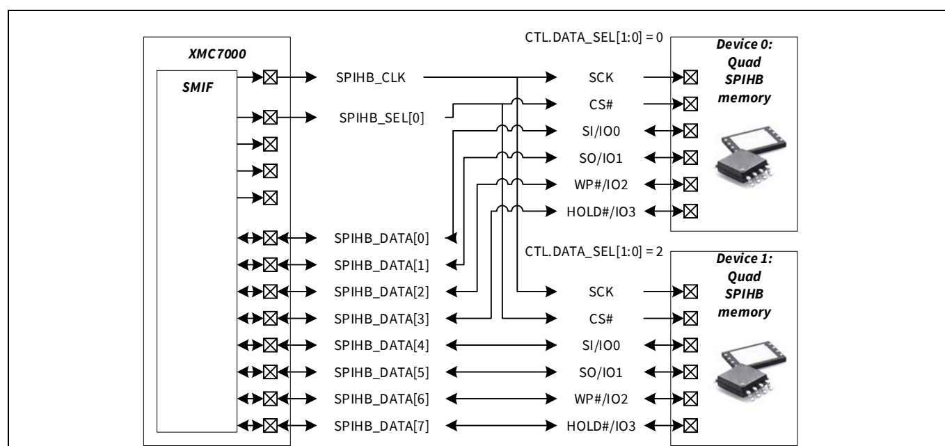
Figure 30-19. Dual-Quad SPI mode by connecting quad SPI device 0 to SPIHB_DATA[3:0], Quad SPI device 1 connected to SPIHB_DATA[7:4]
