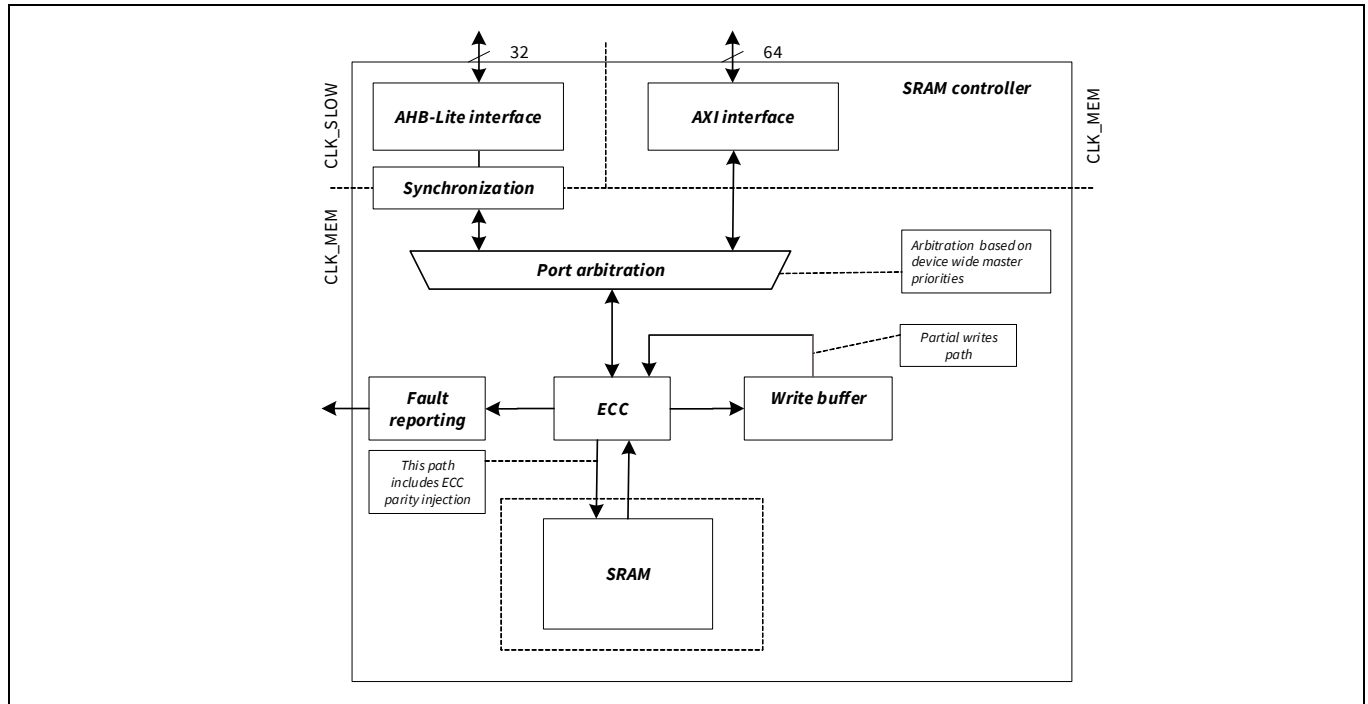
Figure 10-1. SRAM controller
