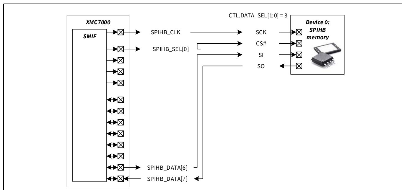
Figure 30-9. Single SPI device 0 connected to SPIHB_DATA[7:6]
