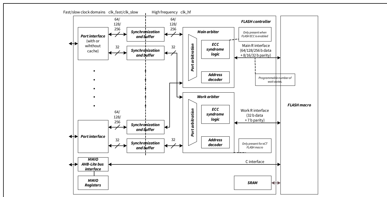
Figure 8-2. Flash controller
