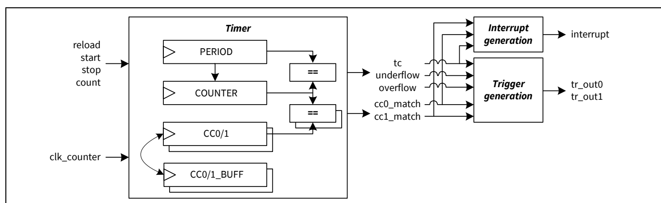
Figure 25-8. Timer functionality
