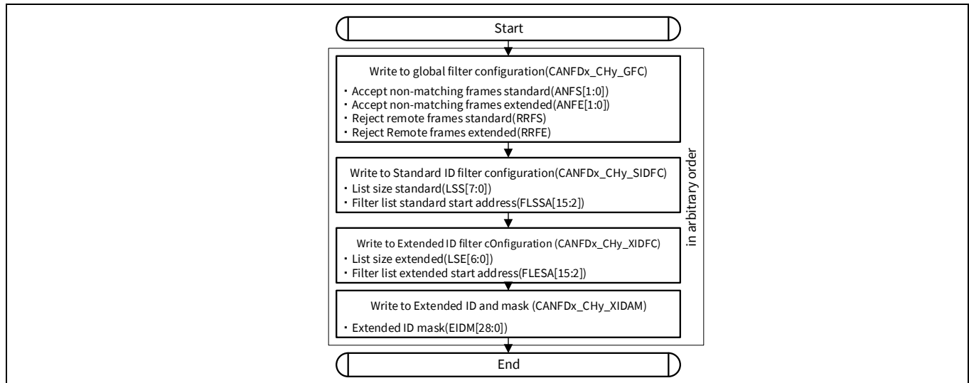
Figure 24-36. ID filter list configuration
