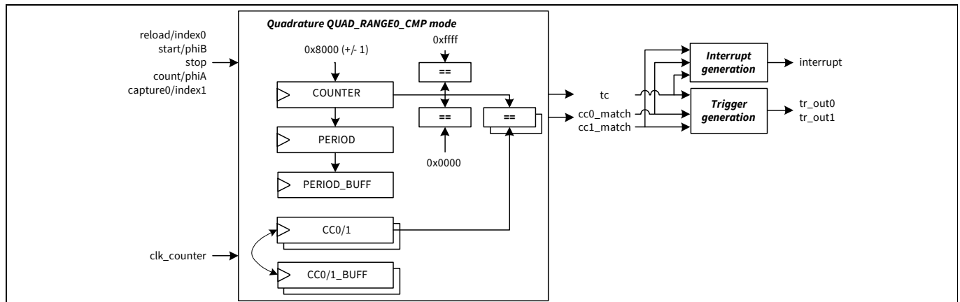
Figure 25-29. Quadrature (QUAD_RANGE0_CMP mode) function diagram
