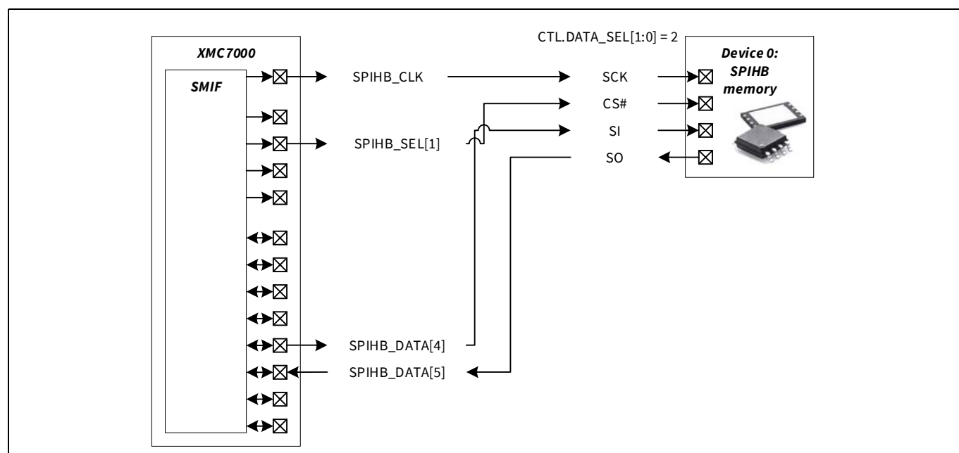
Figure 30-10. Single SPI device 0 connected to SPIHB_DATA[5:4]
