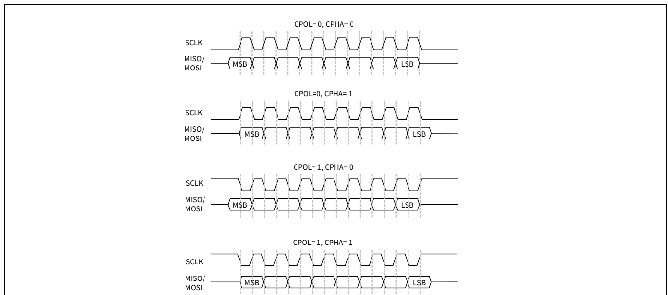
Figure 23-7. SPI Motorola, 4 modes
