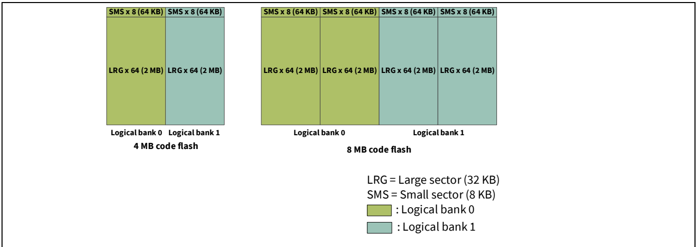
Figure 8-7. Code flash array organization
