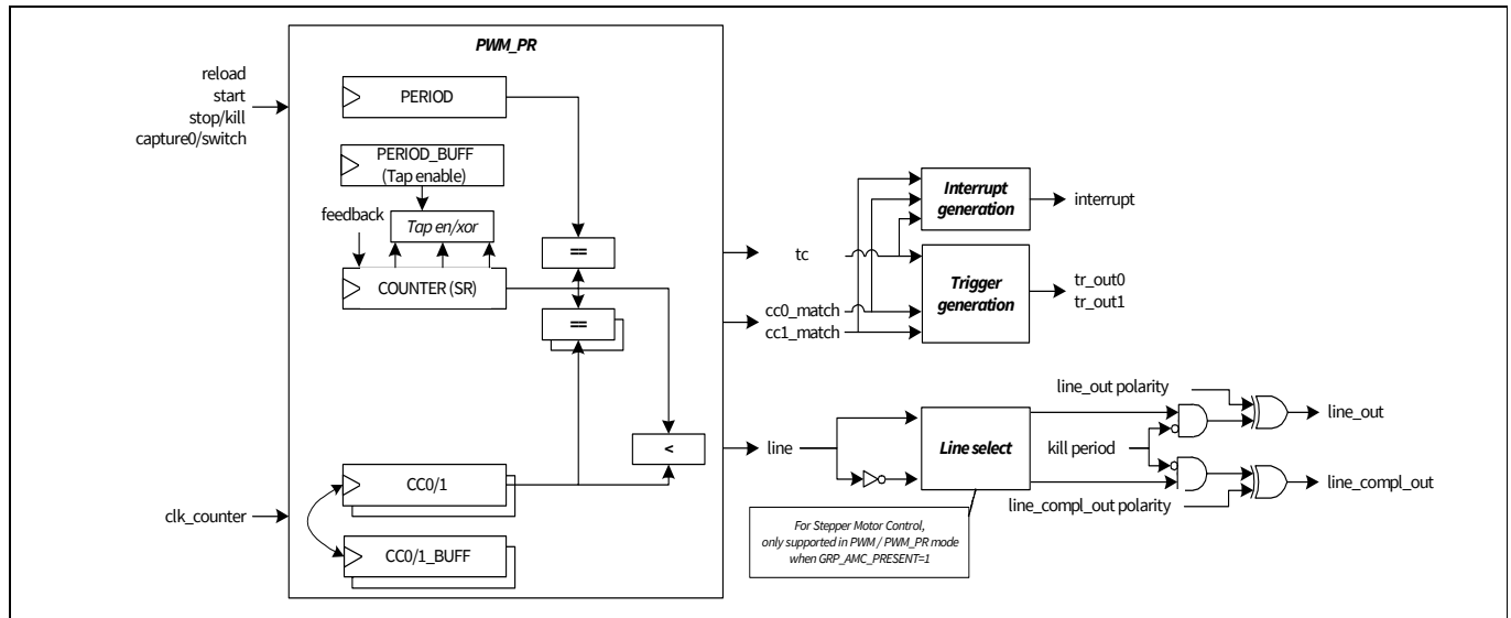
Figure 25-62. PWM_PR functionality
