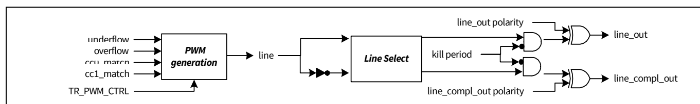
Figure 25-43. Line generation logic
