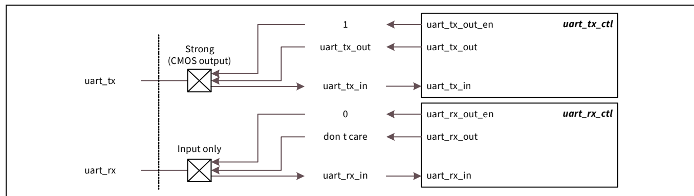
Figure 23-31. Standard UART mode, I/O pad connections
