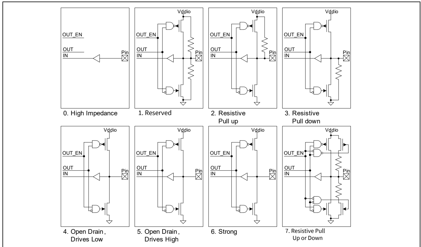
Figure 22-5. Fixed-function peripheral I/O drive mode block diagrams
