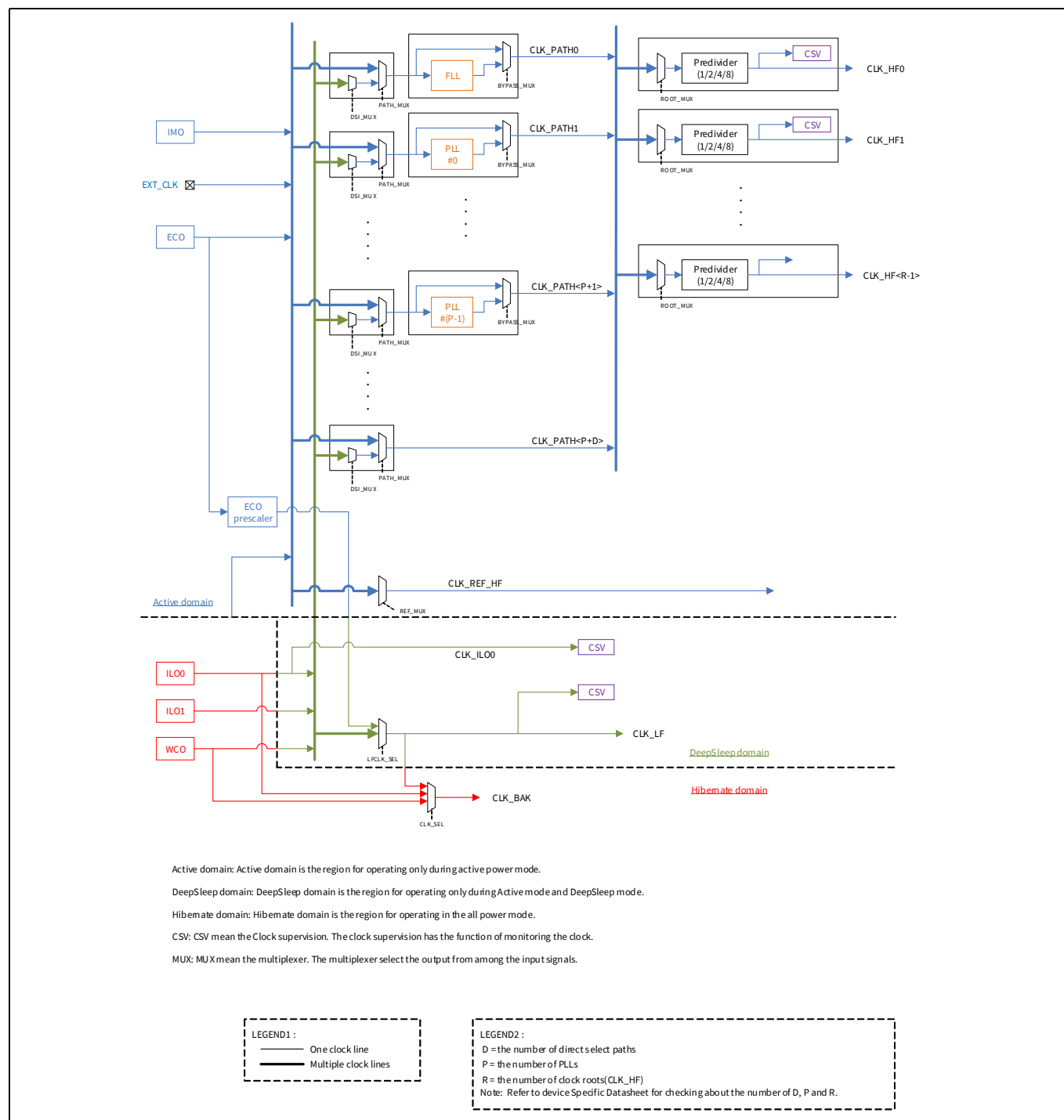
Figure 18-2. Clocking system block diagram
