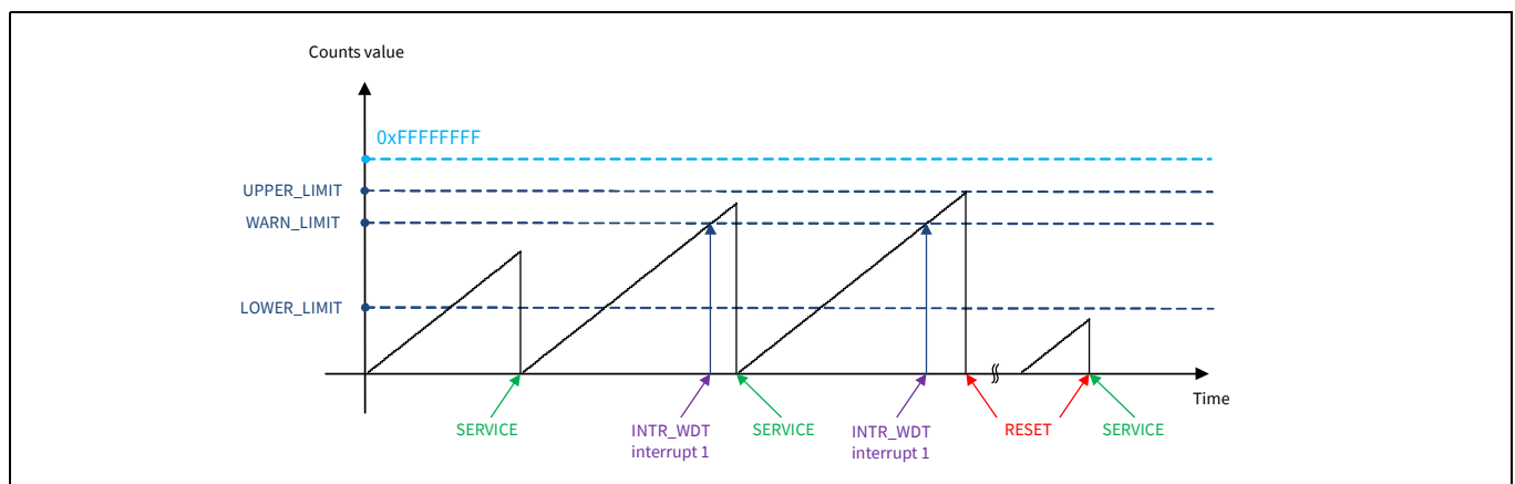
Figure 20-3. WDT counter operation in window mode
