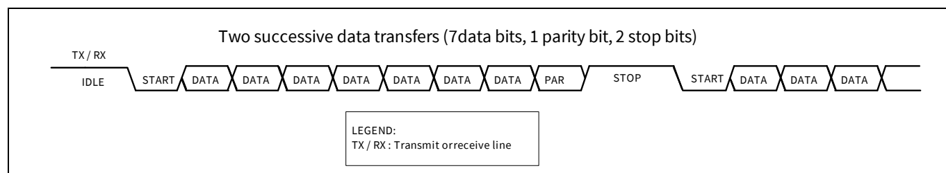
Figure 23-20. UART, standard protocol example
