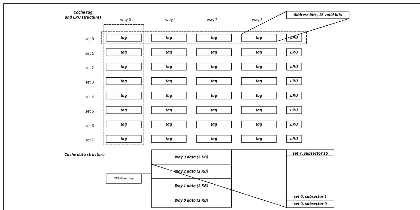
Figure 8-3. Cache
