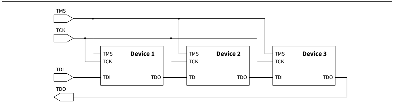
Figure 34-2. JTAG interface to multiple devices on a circuit board
