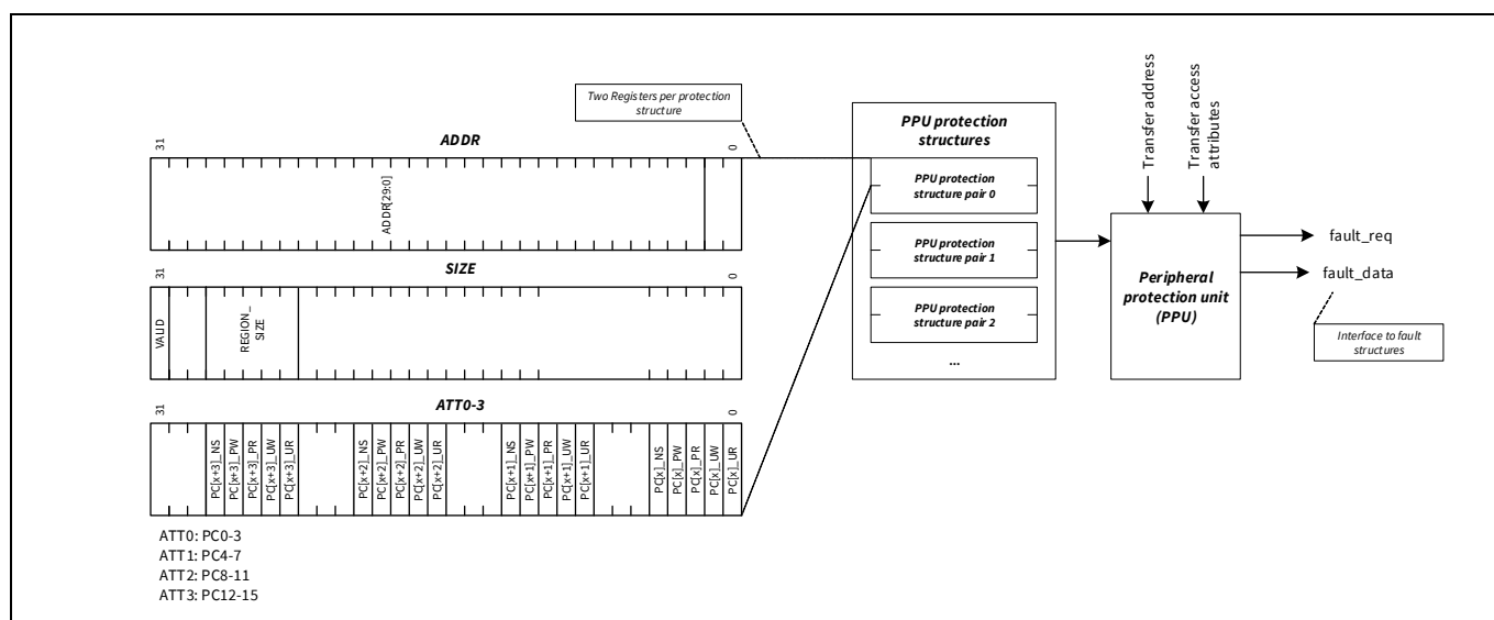
Figure 6-5. PPU functionality
