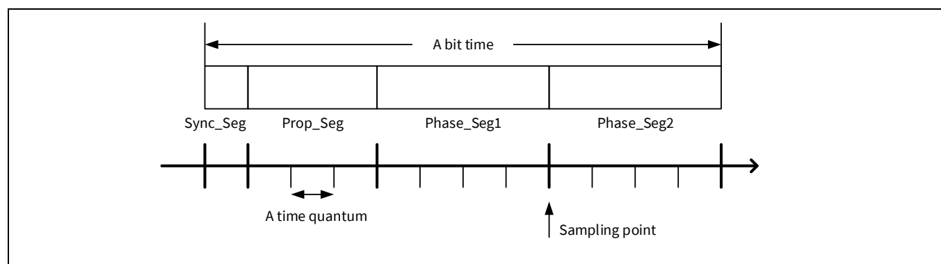
Figure 24-14. Bit time construction
