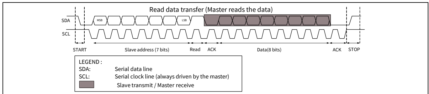
Figure 23-38. Master read data transfer
