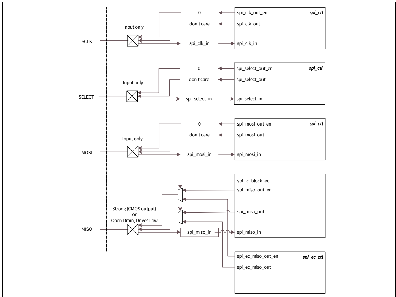
Figure 23-18. SPI slave I/O pad connections
