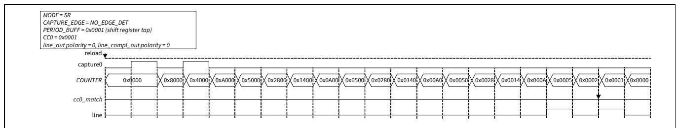
Figure 25-65. SR shift with PERIOD_BUFF = 0x0001
