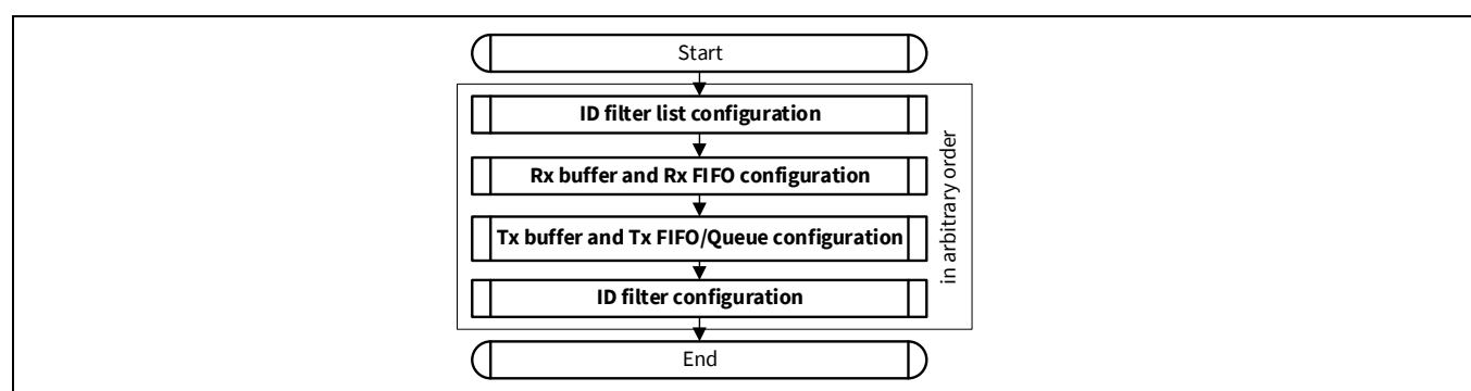
Figure 24-35. Message RAM configuration overview
