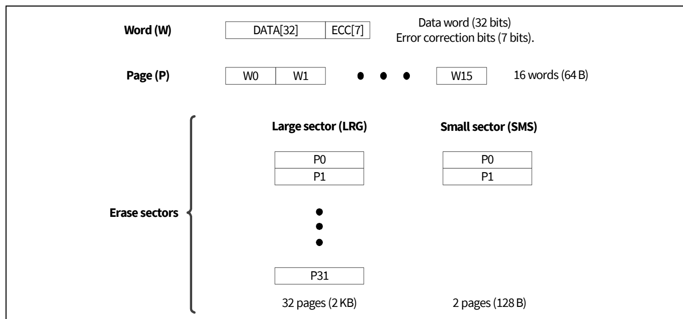
Figure 9-3. Work flash sector organization
