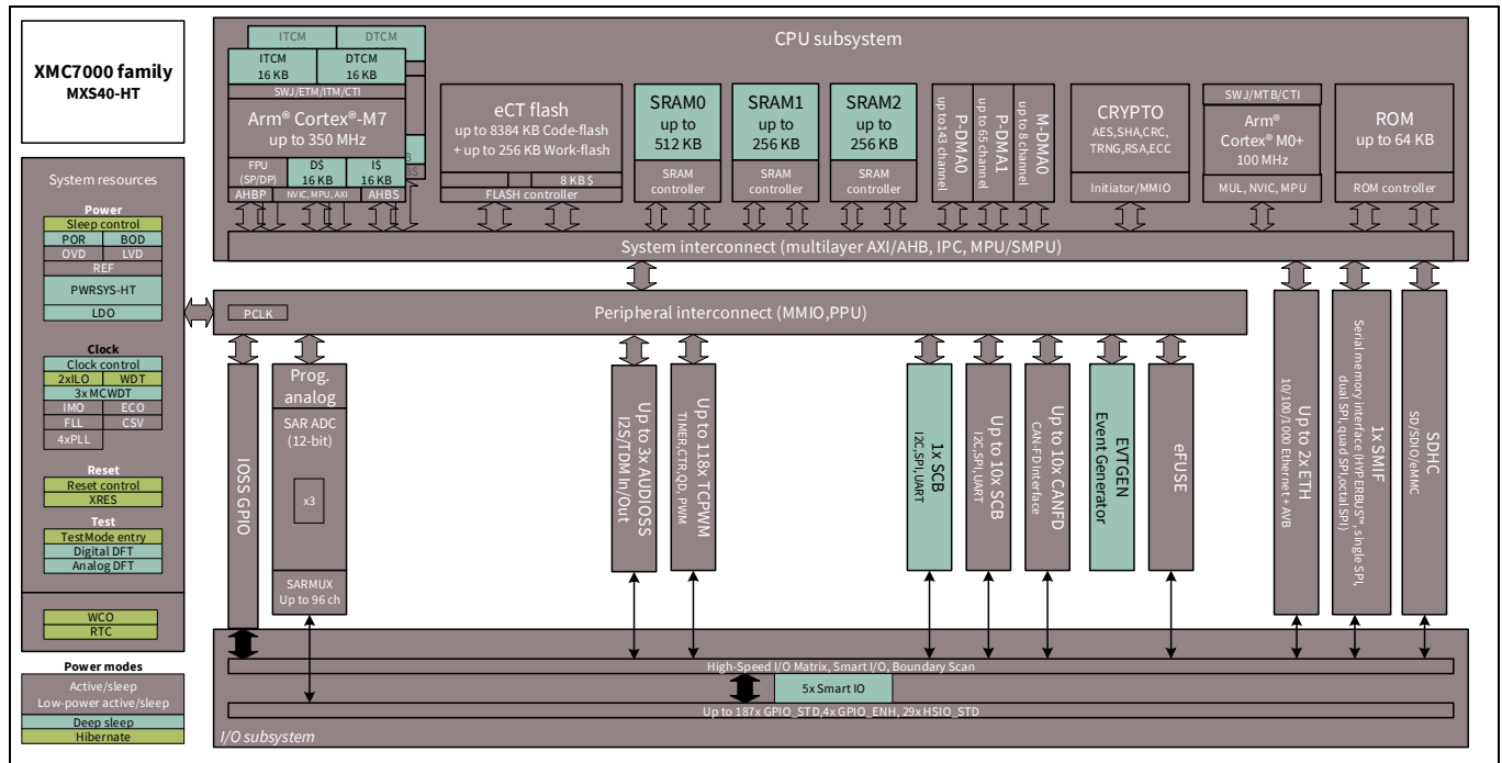
Figure 1-1. XMC7000 architecture diagram
