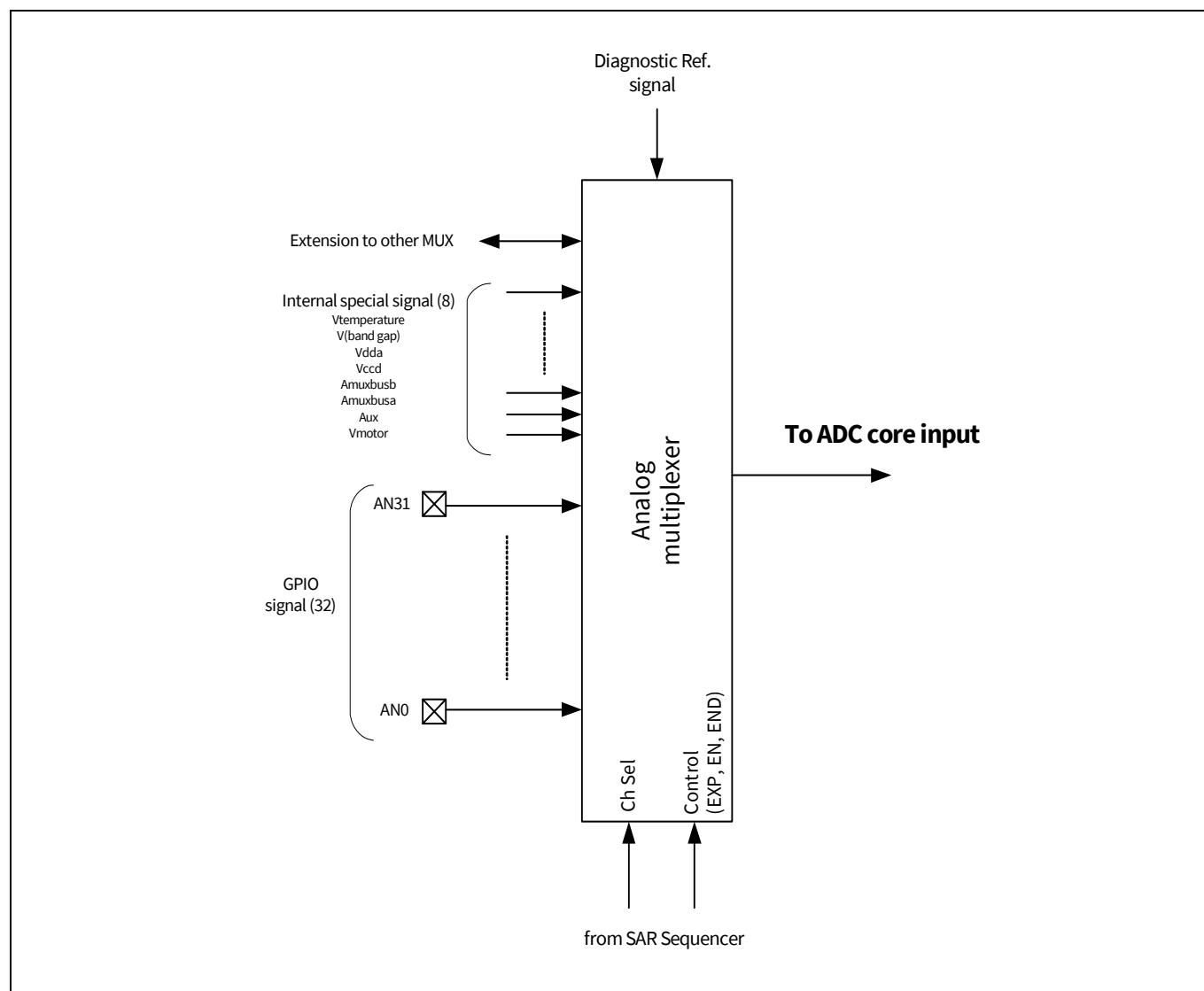
Figure 33-4. SARMUX block diagram
