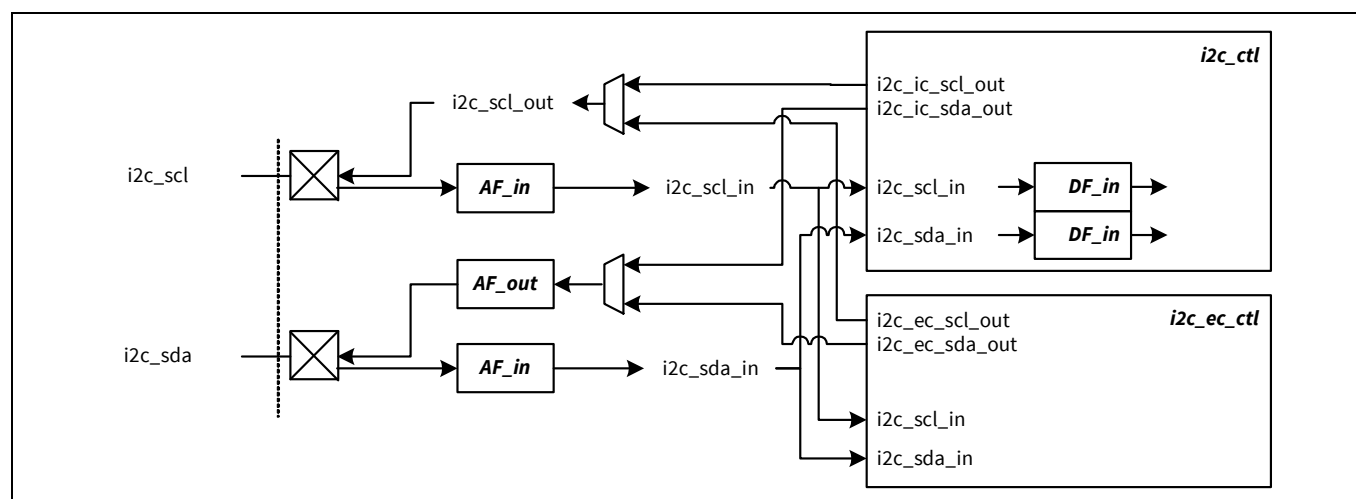
Figure 23-41. I 2 C glitch filtering connection
