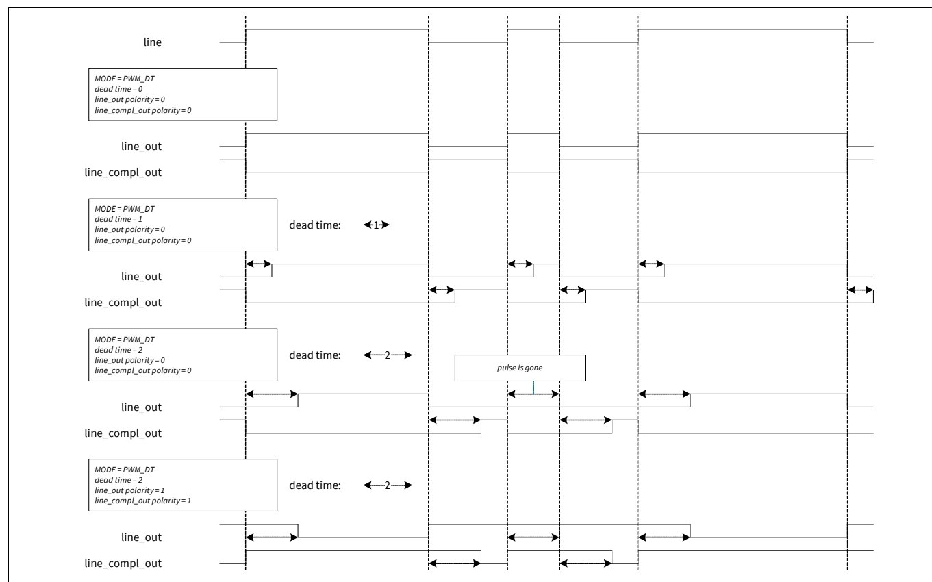
Figure 25-60. Dead-time timing
