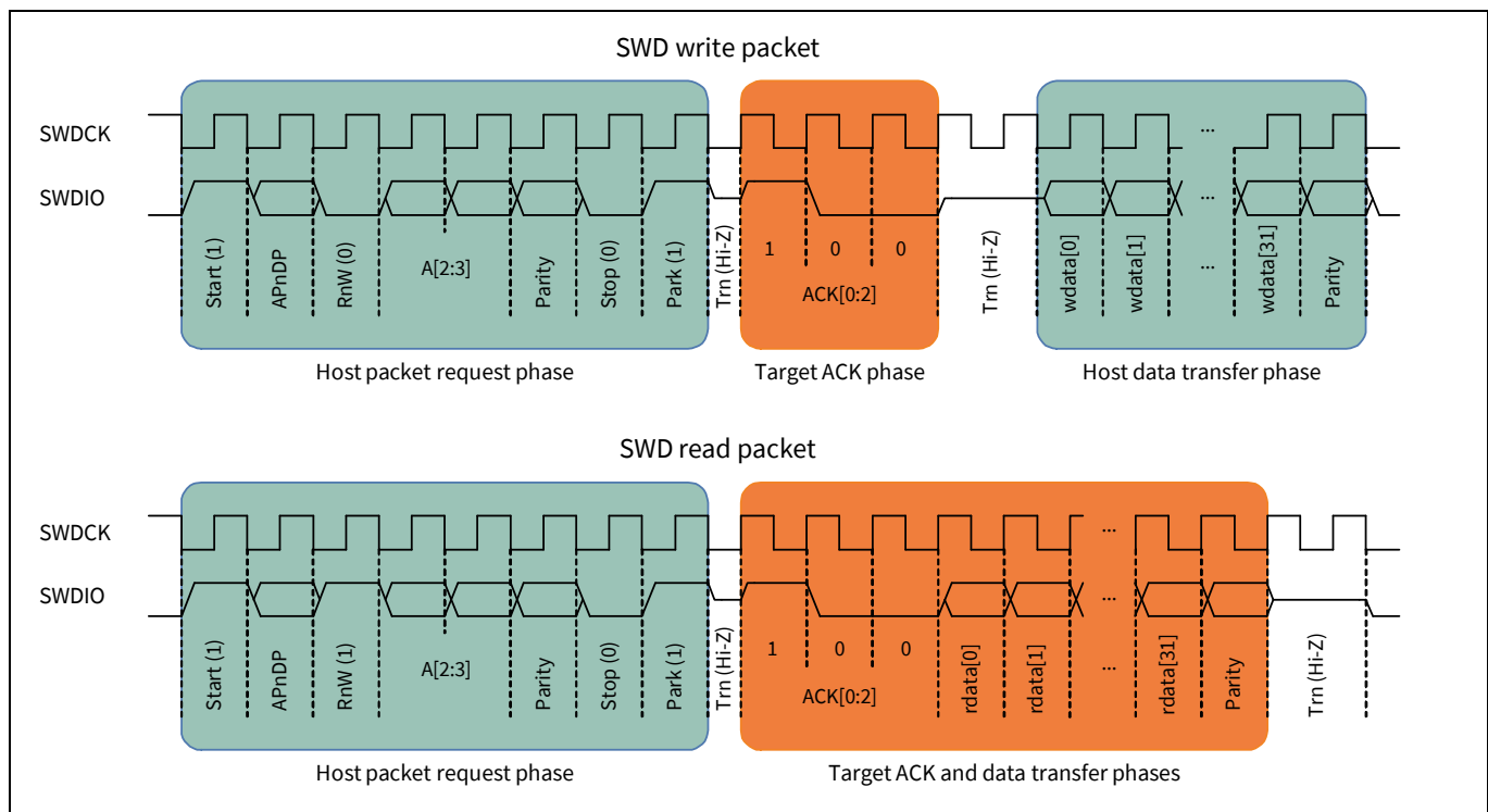
Figure 34-1. SWD write and read packet timing diagrams
