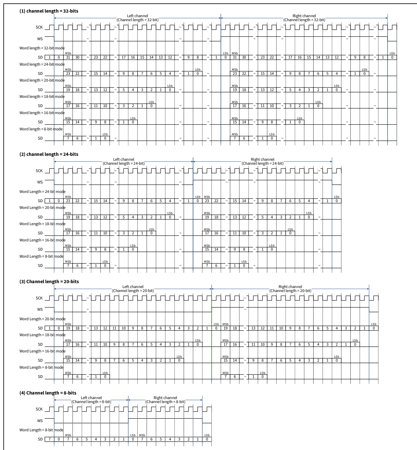
Figure 32-2. Standard I 2 S format (word length and channel length combination timing diagrams)
