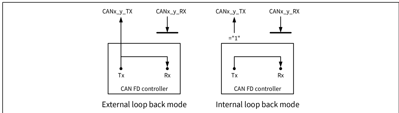
Figure 24-5. Pin control in loop back modes
