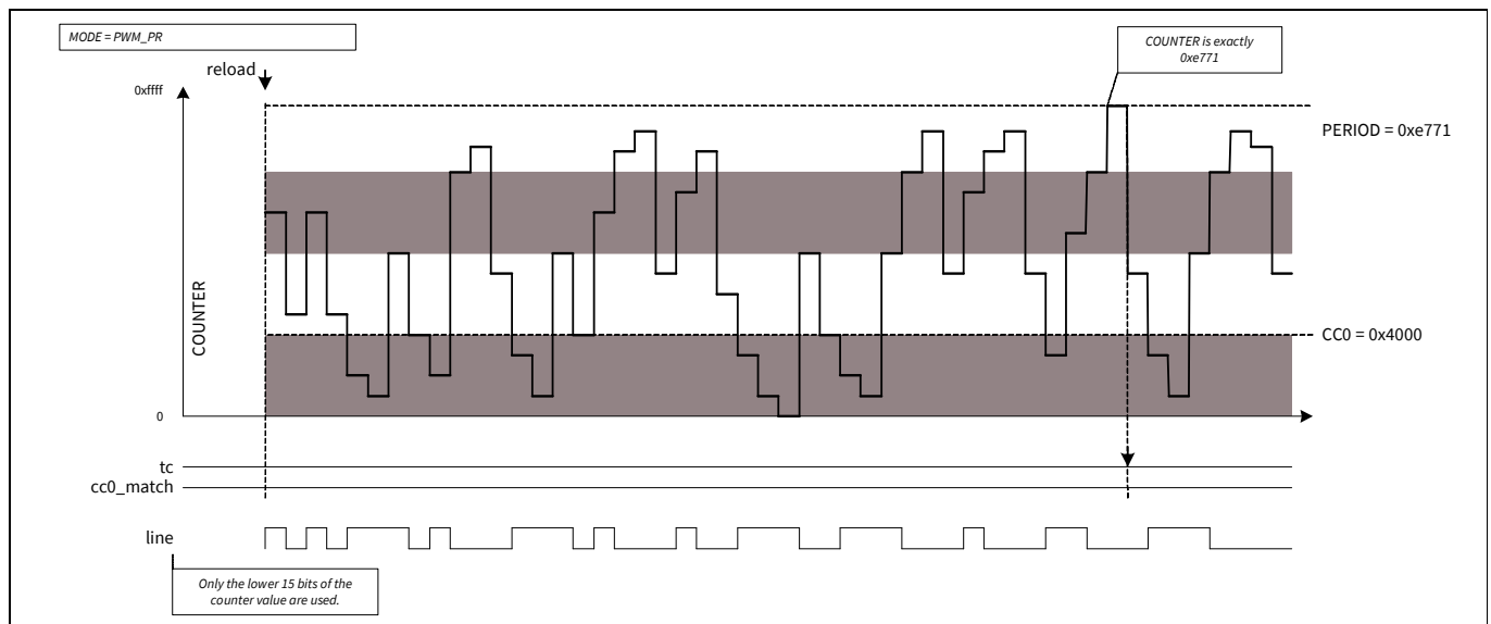
Figure 25-63. PWM_PR output
