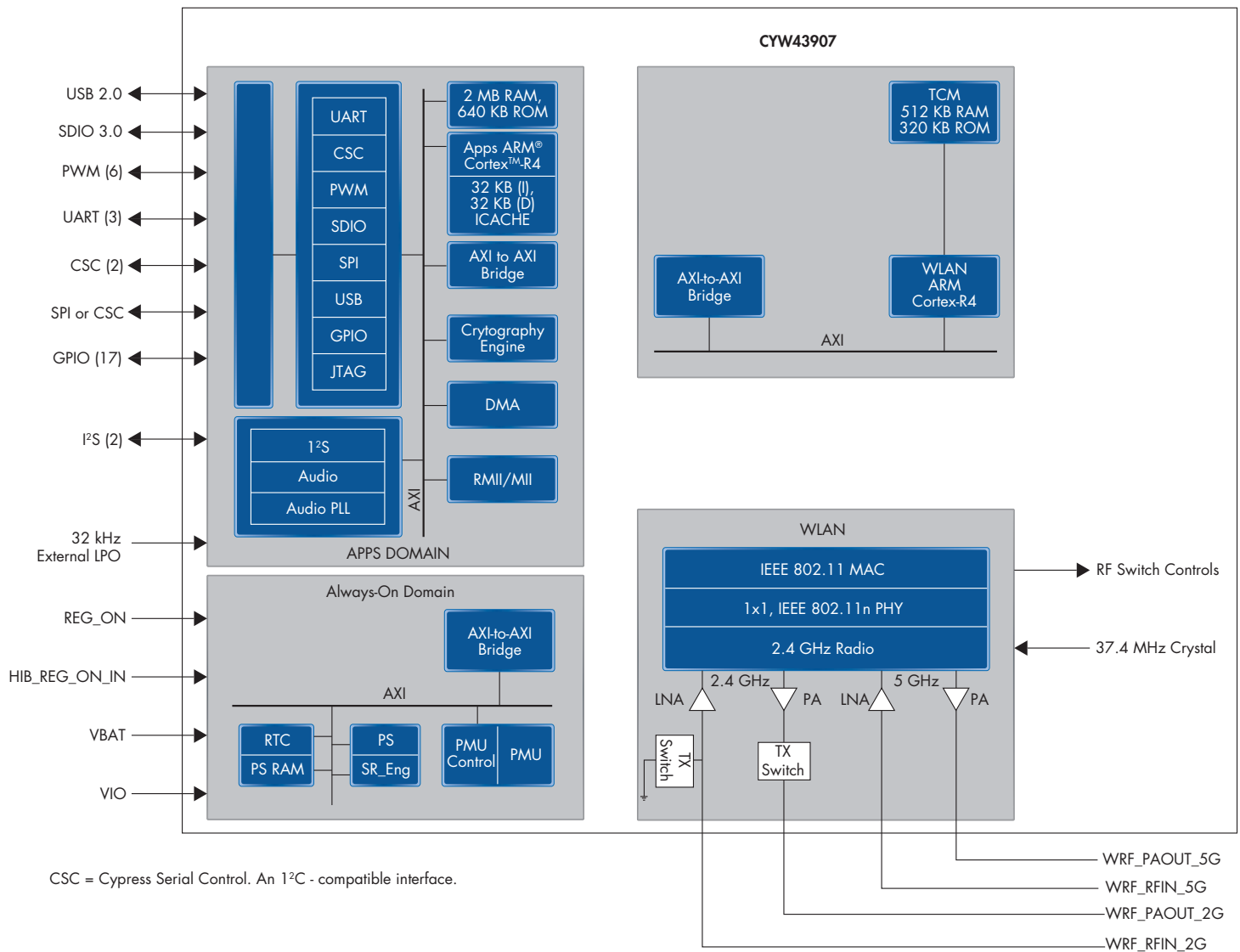
CYW43907 Block Diagram
