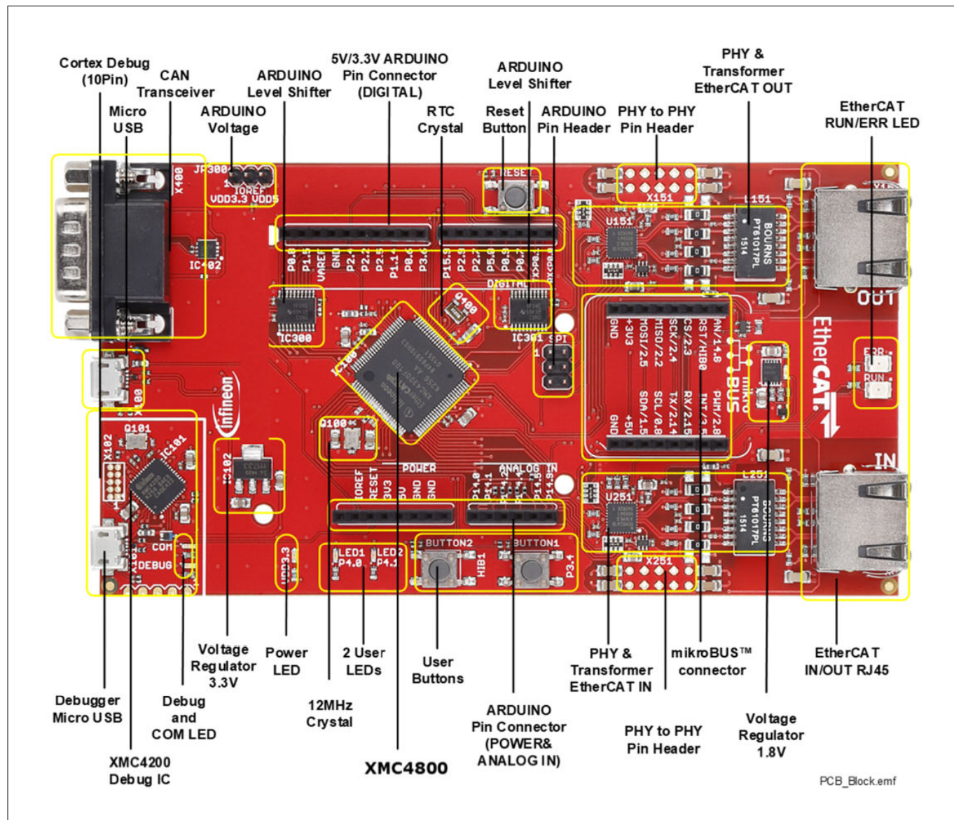
Figure 2 PCB of the XMC4800 IoT Amazon FreeRTOS Connectivity kit with EtherCAT®
