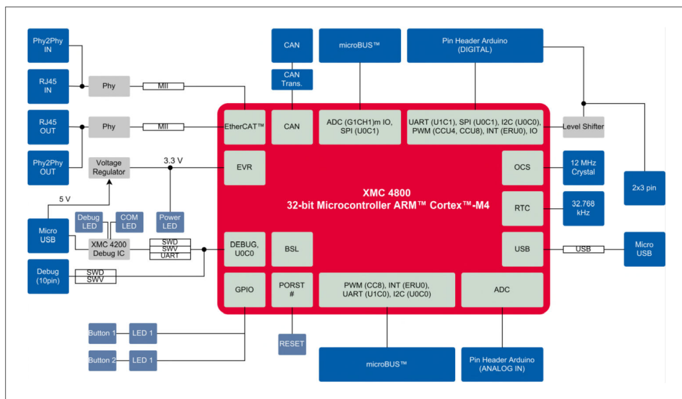
Figure 1 Block diagram of the XMC4800 IoT Amazon FreeRTOS Connectivity kit with EtherCAT®
