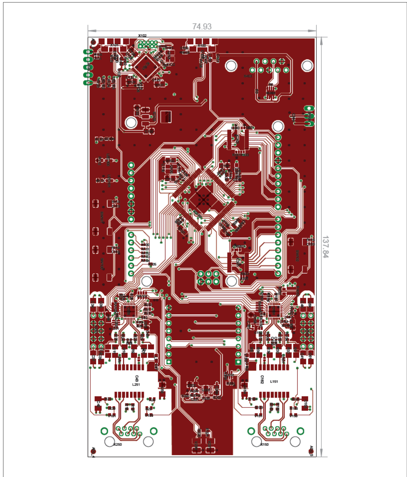
Figure 11 Components placement and geometry
