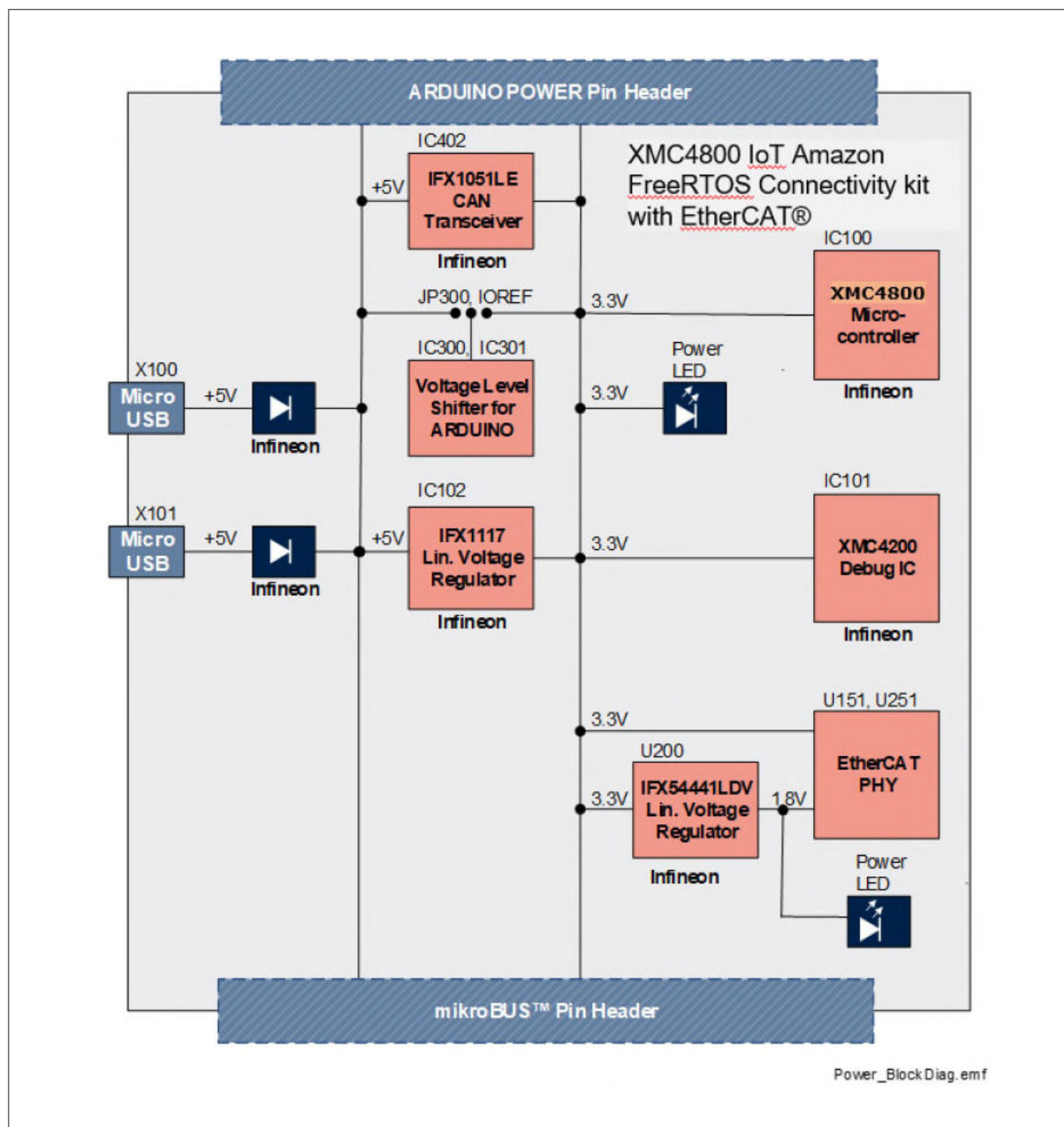
Figure 3 Power supply concept
