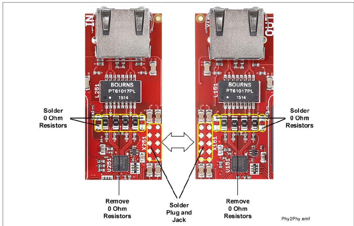
Figure 6 Phy-2-Phy EtherCAT® connection between two XMC4800 IoT Amazon FreeRTOS Connectivity kit with EtherCAT®
