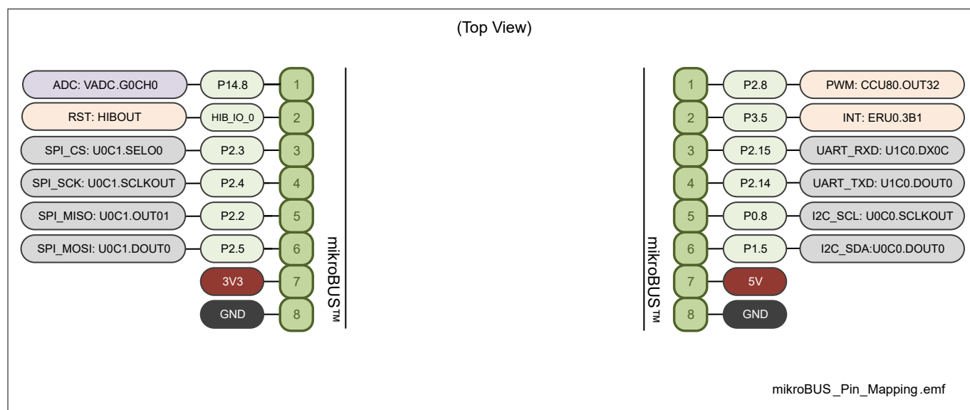
Figure 5 Mapping of Arduino™ functions to XMC™ pin functions
