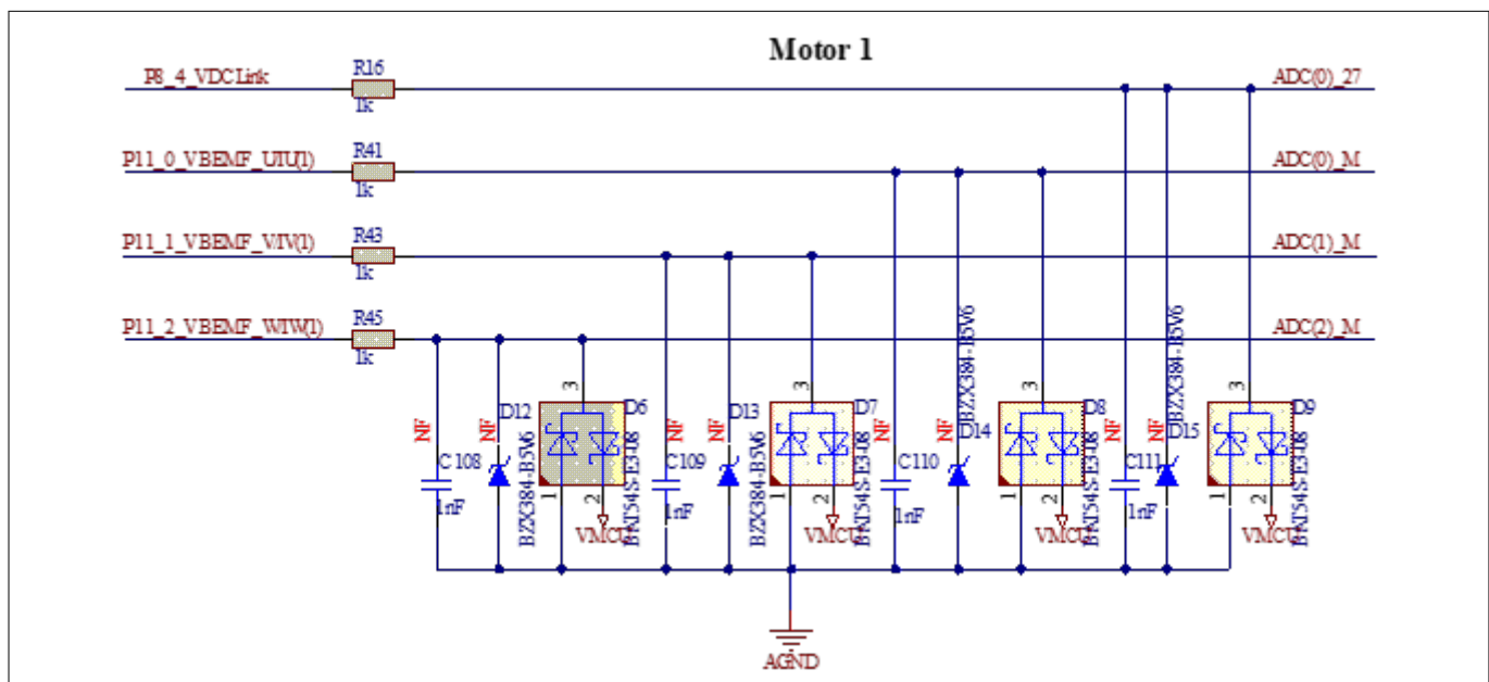
Figure 38 Analog to digital converter
