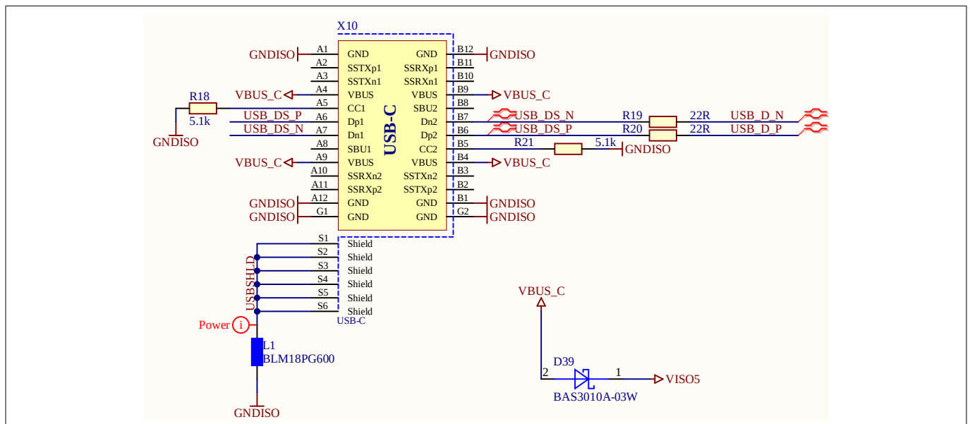
Figure 22 USB-C connector
