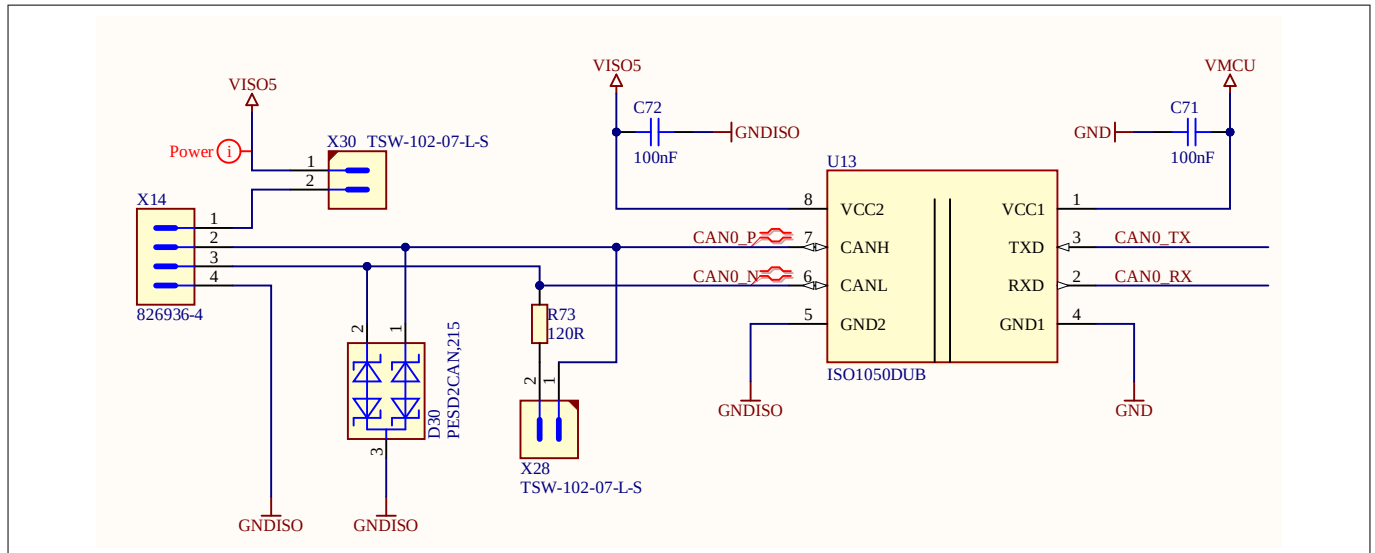
Figure 21 CAN interface and isolation
