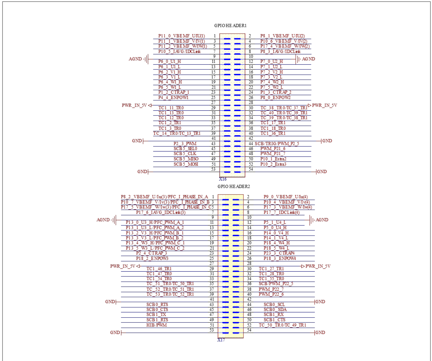
Figure 27 XMC7200D I/O headers
