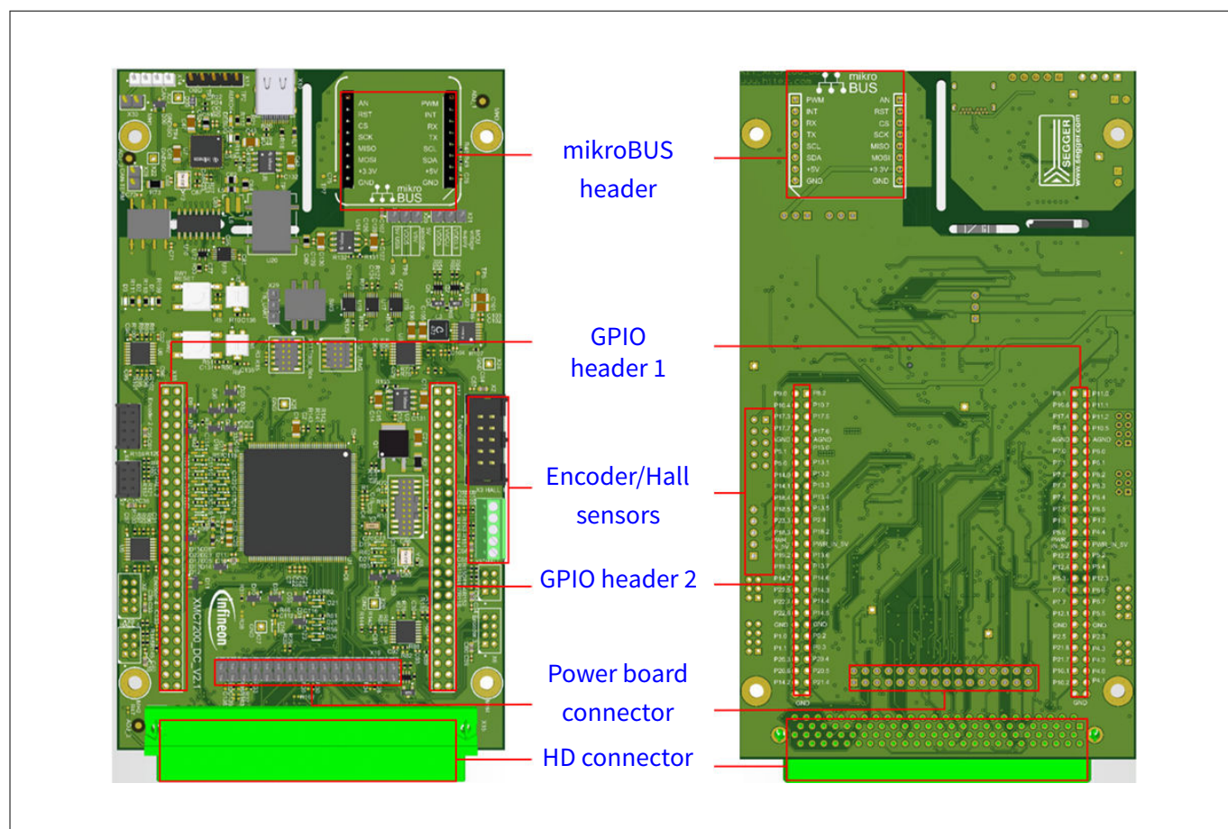
Figure 3 XMC7200 motor drive card headers
