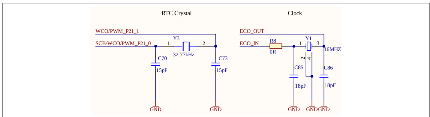
Figure 32 Crystal and oscillators
