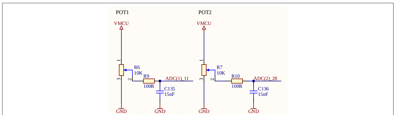
Figure 33 Potentiometers
