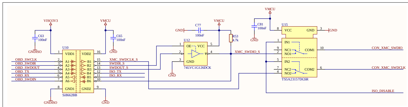
Figure 17 Interconnection between power plane and debugger plane
