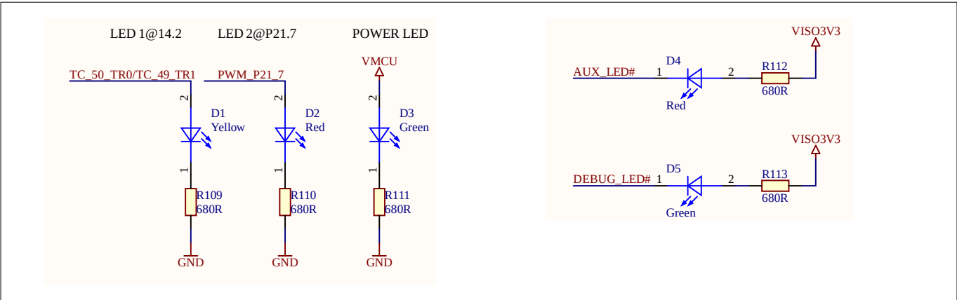
Figure 30 User LEDs
