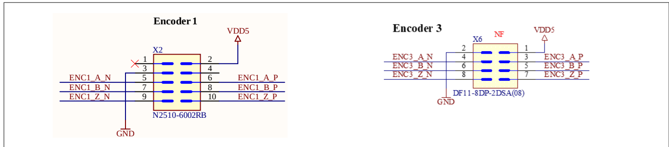
Figure 36 Encoder headers
