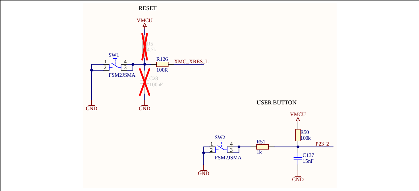
Figure 31 User buttons
