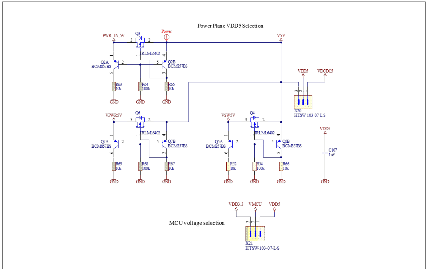
Figure 25 Voltage selection headers
