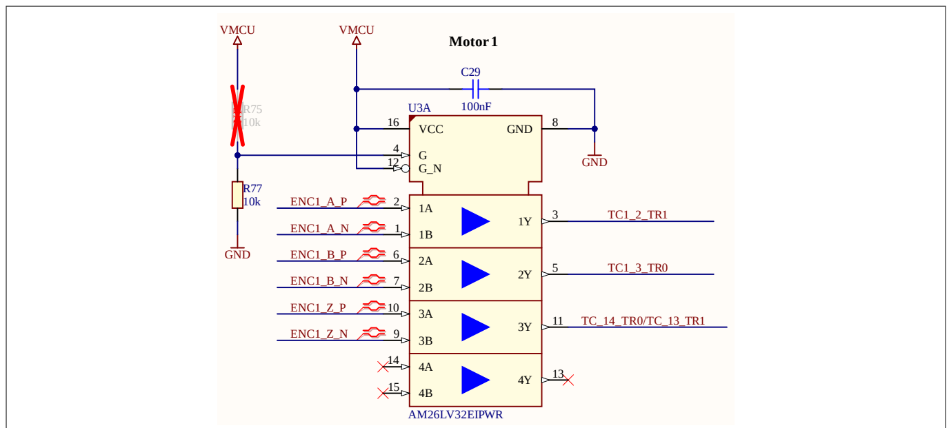
Figure 34 Motor encoder driver
