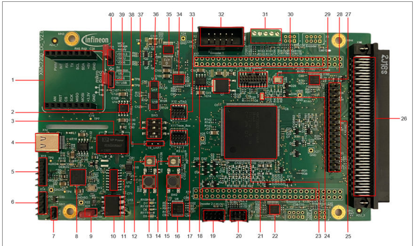
Figure 2 XMC7200 motor drive card – top view
