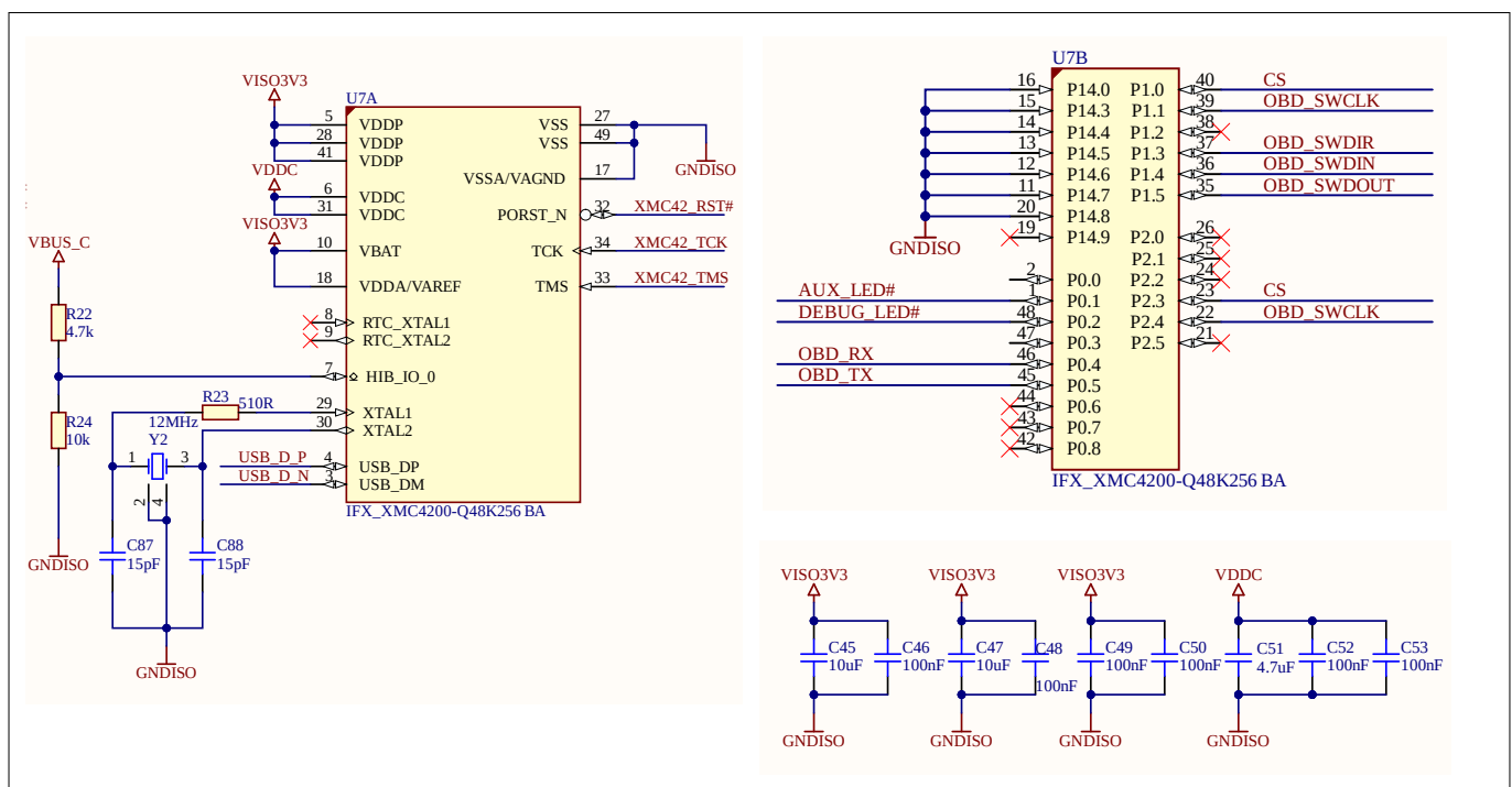
Figure 15 Onboard debugger
