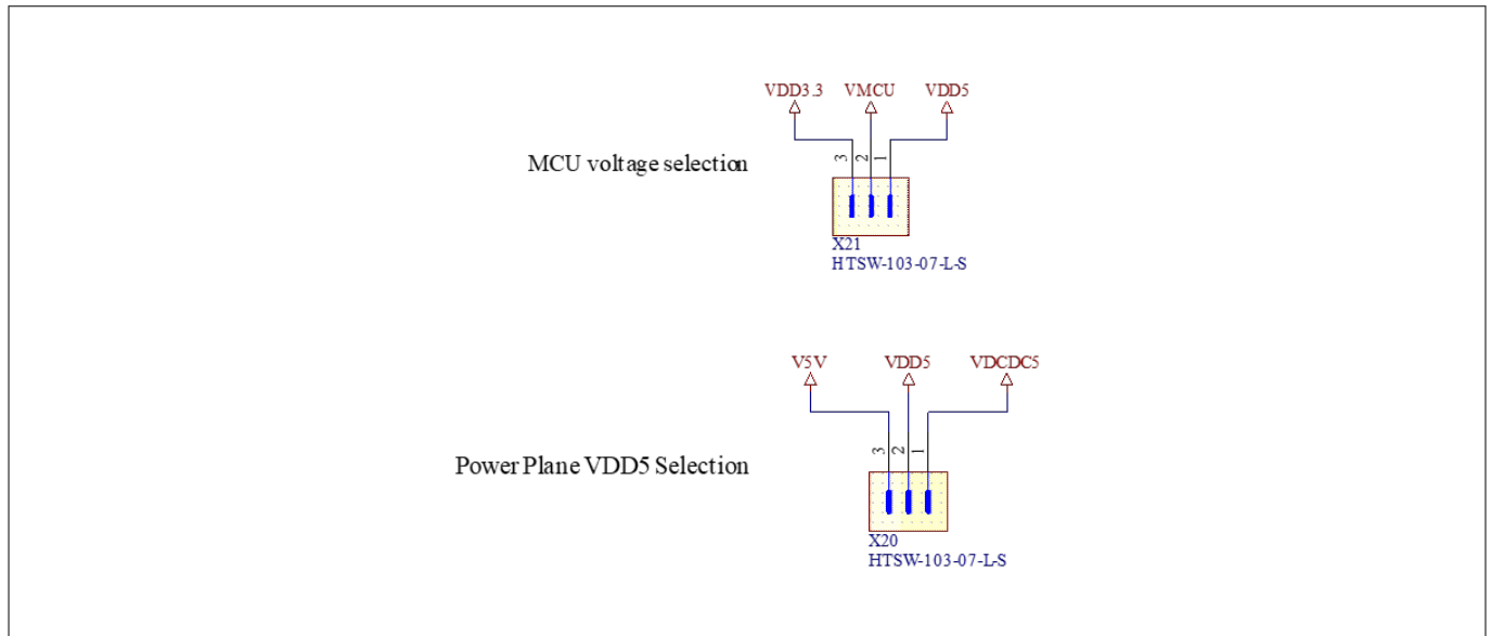
Figure 39 XMC7200 VDDIO2 voltage selection
