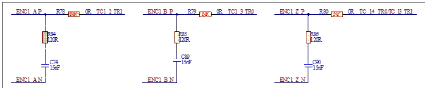
Figure 37 Encoder interconnection
