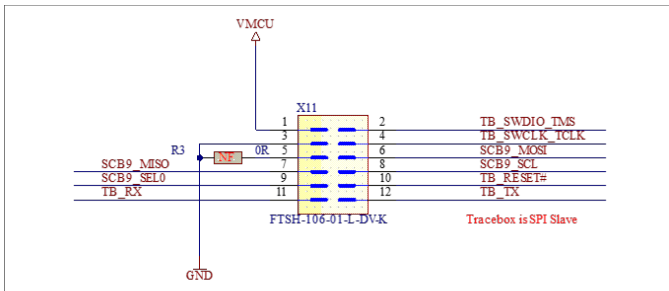
Figure 20 Tracebox header
