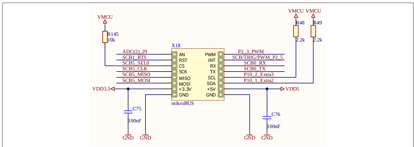
Figure 26 mikroBUS connector
