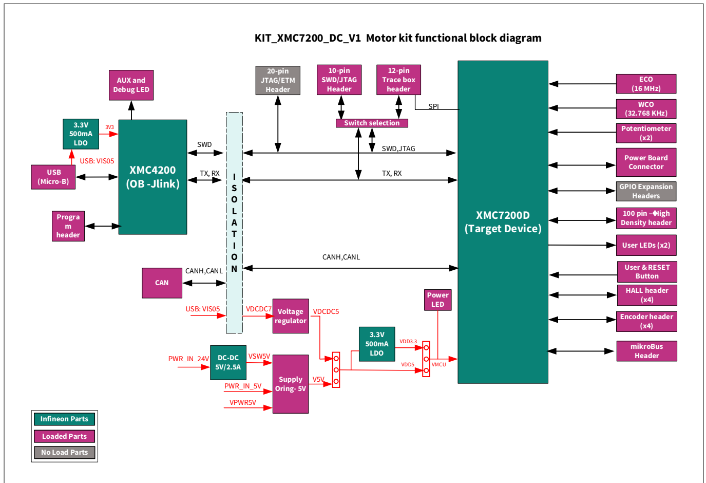
Figure 5 Block diagram of XMC7200 motor drive card
