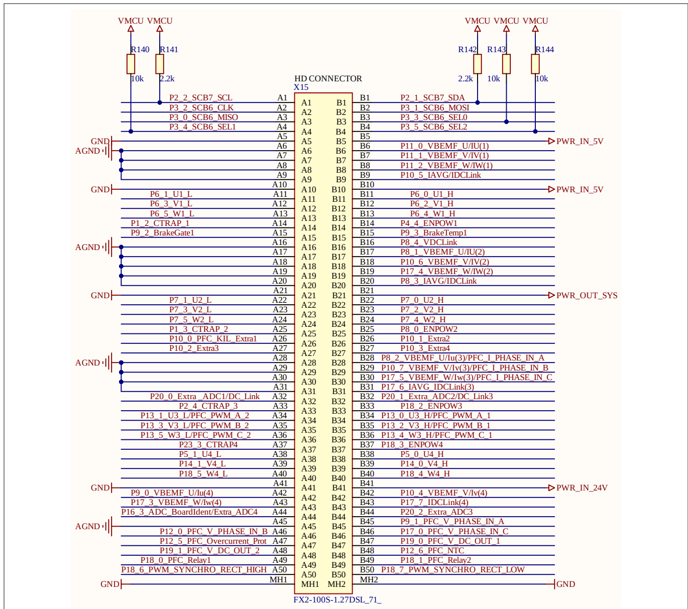
Figure 29 High-density connector
