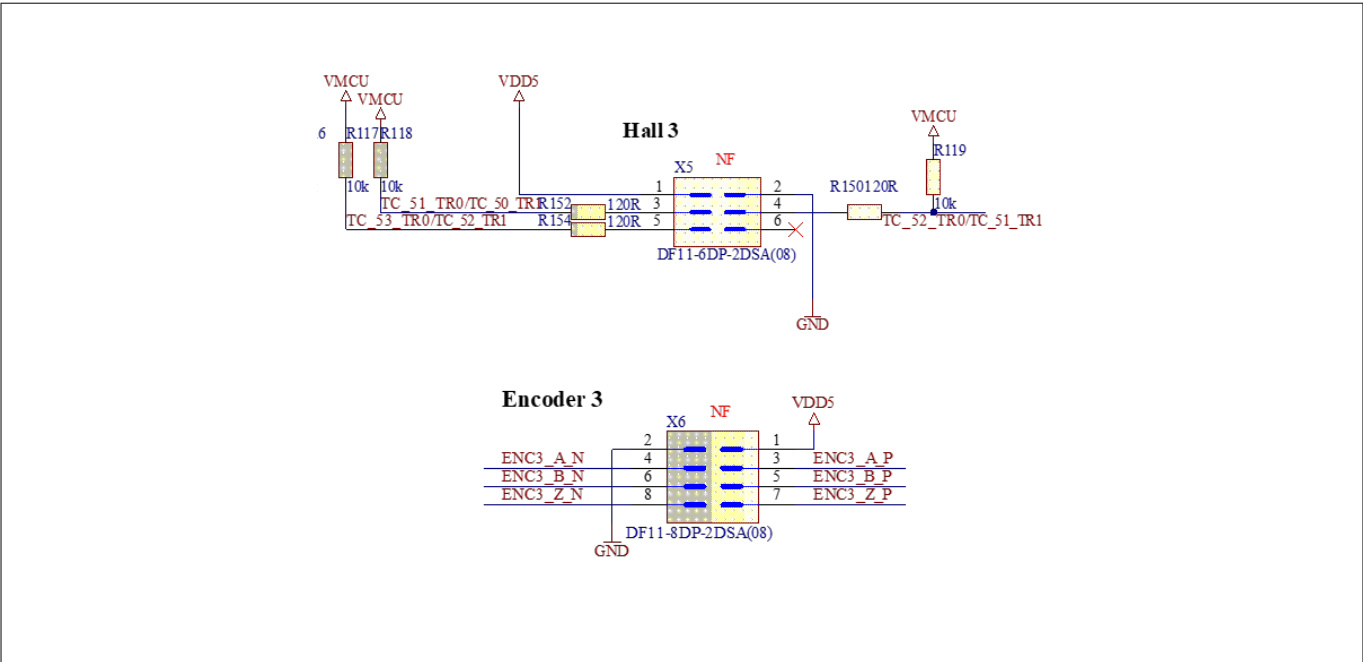
Figure 40 N.C. hall and encoder headers
