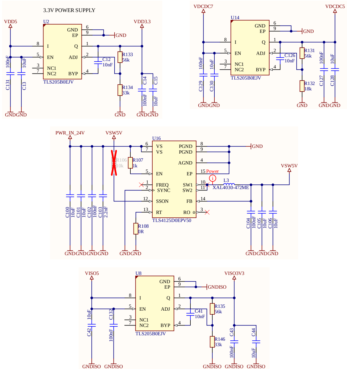
Figure 24 Voltage regulators
