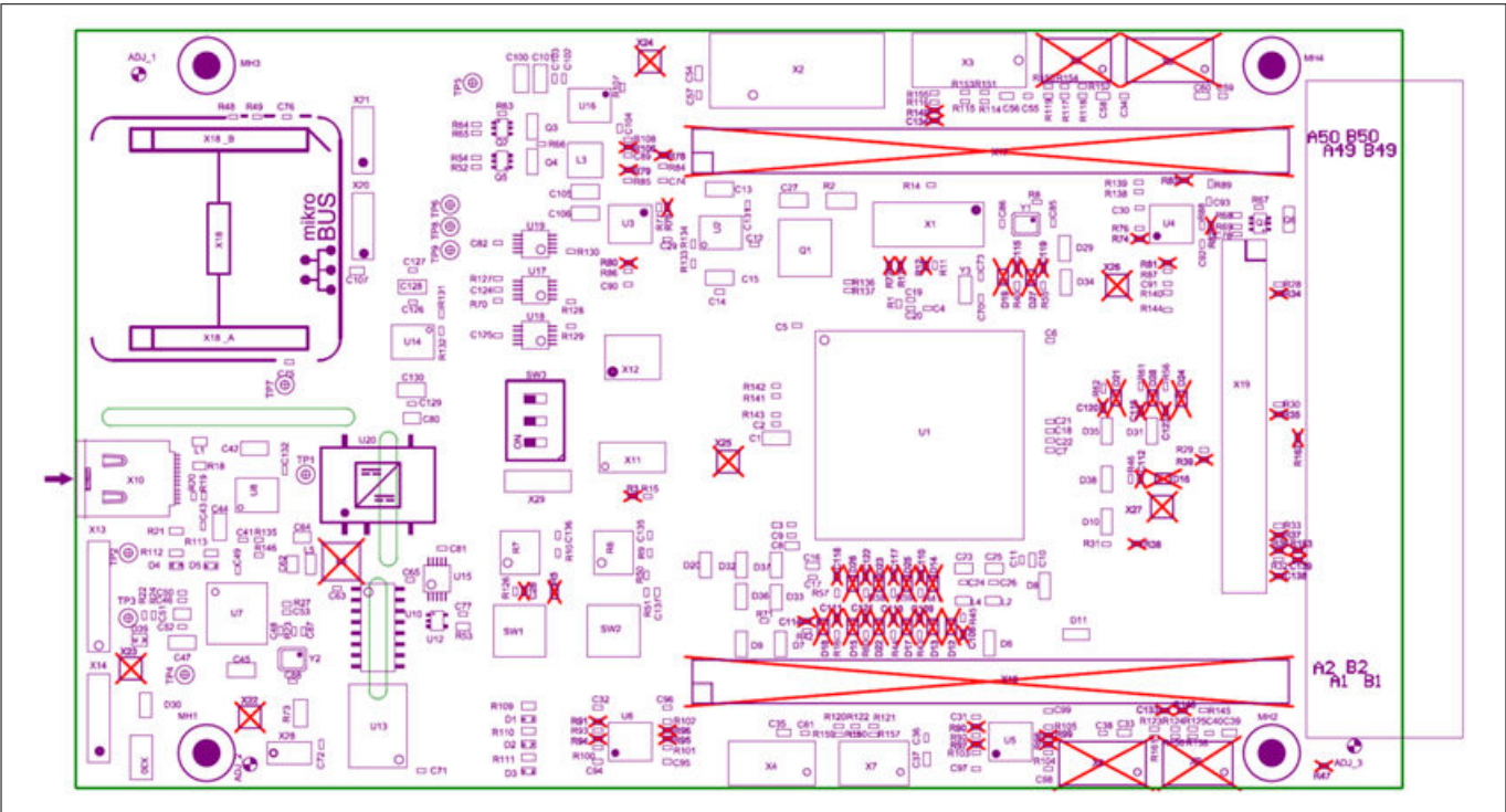
Figure 41 Component placement diagram
