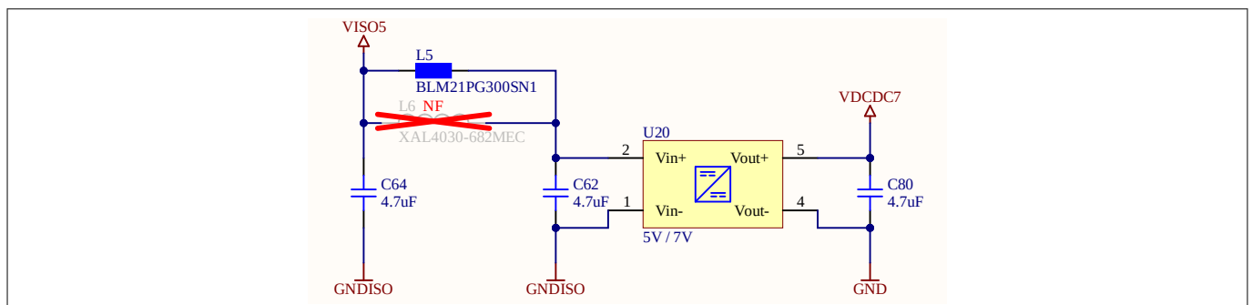
Figure 23 Power interconnection
