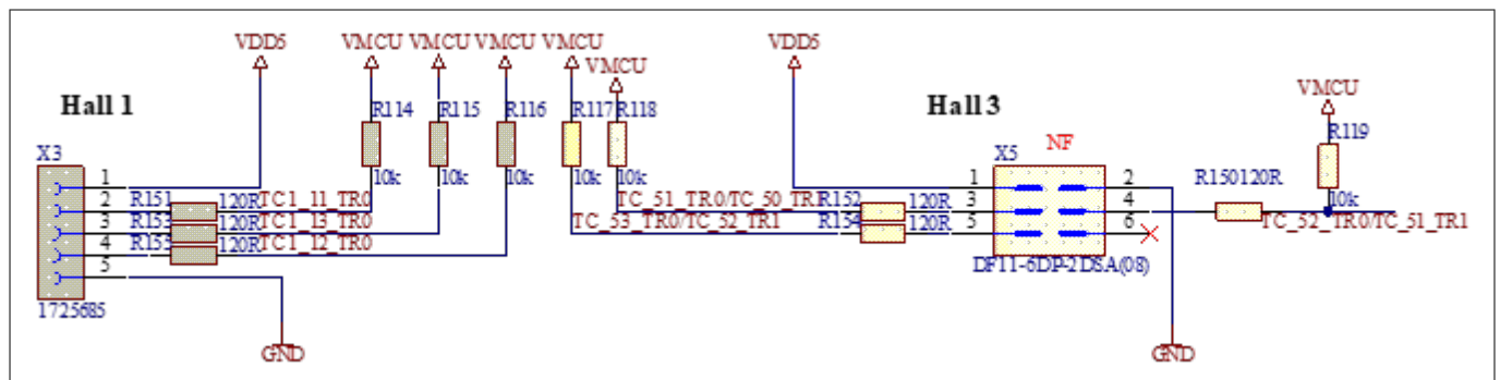
Figure 35 Hall headers
