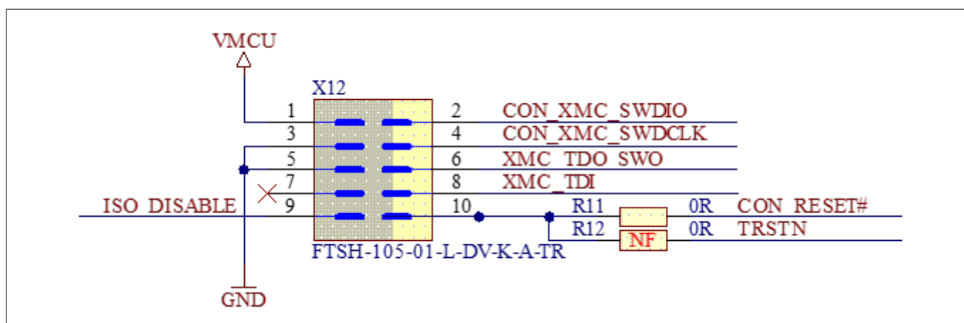
Figure 16 10-pin SWD/JTAG header
