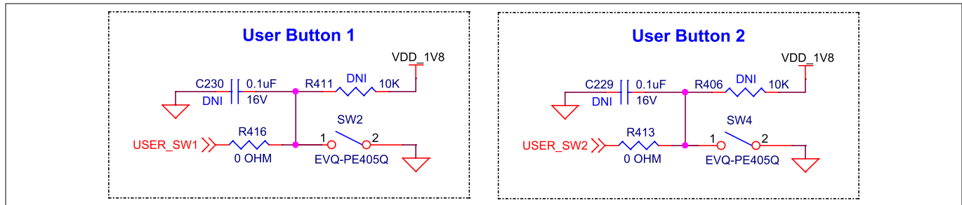
Figure 80 Schematic of user buttons
