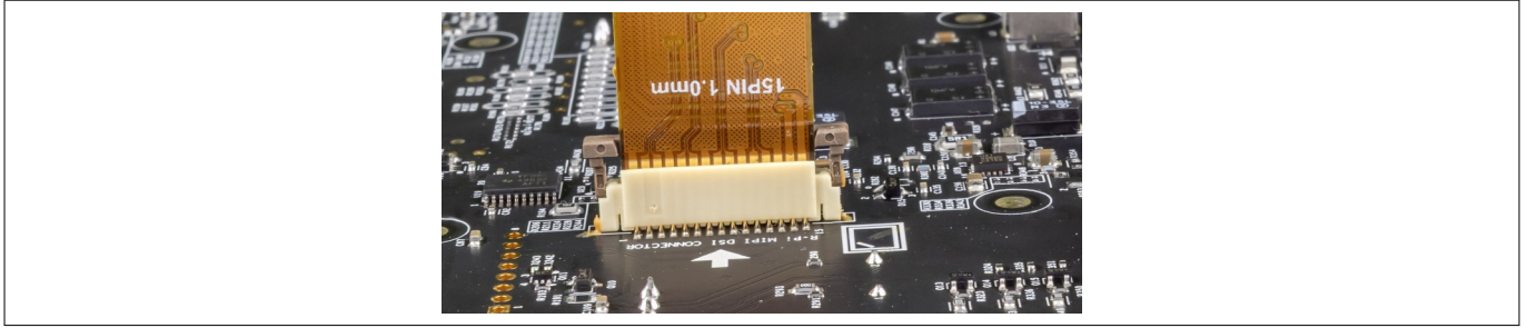
Figure 67 Connecting the MIPI DSI interface flex cable to 15pin FPC connector
