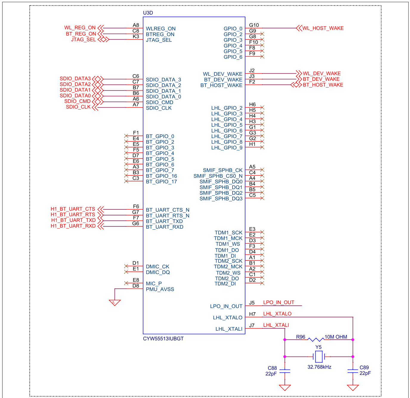
Figure 31 Radio subsystem
