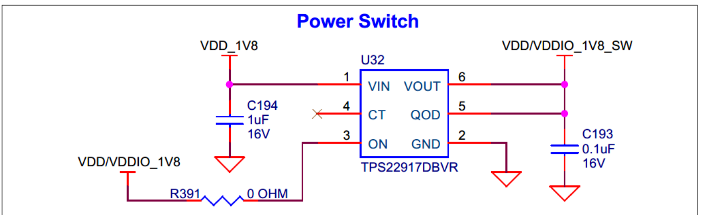
Figure 49 Schematic of power switch
