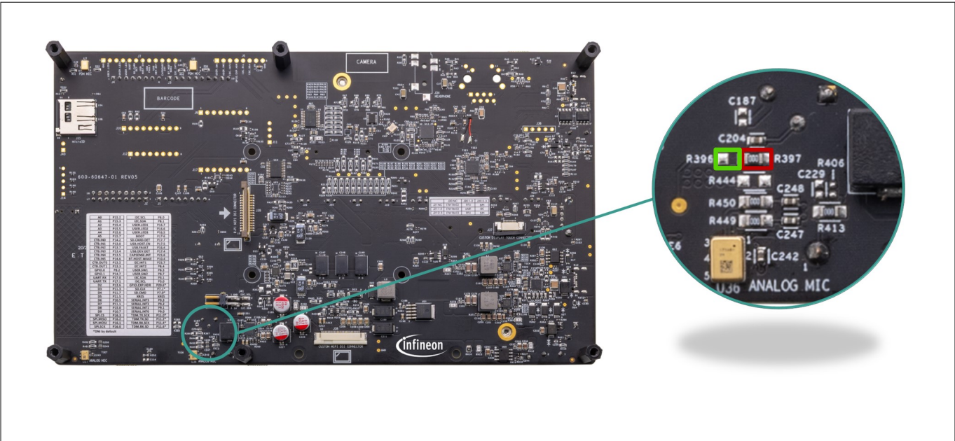
Figure 94 Rework region on baseboard for enabling Thermistor interface
