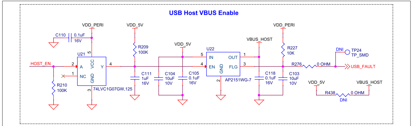
Figure 72 Schematic of USB Host VBUS enable circuit
