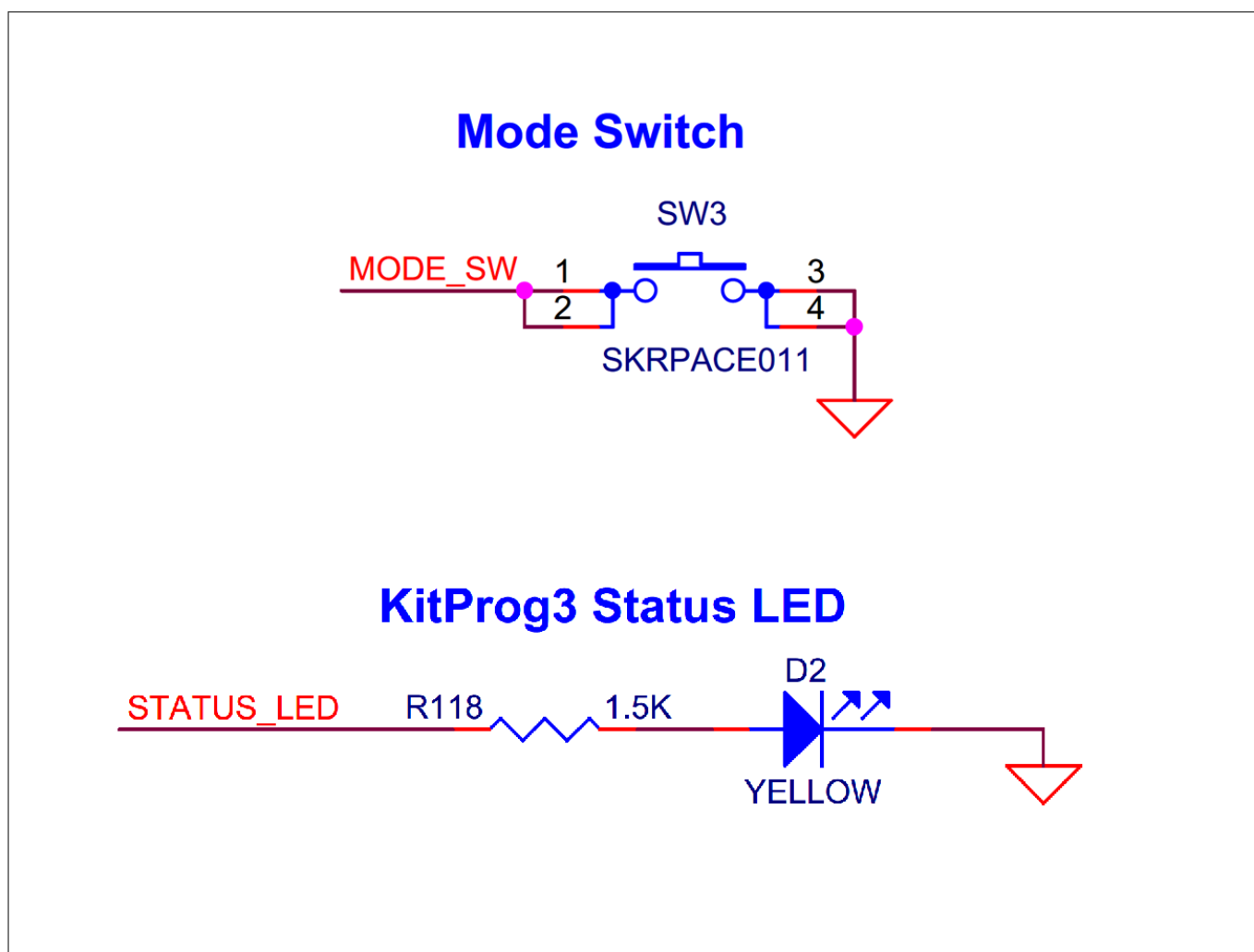
Figure 38 Schematic of KitProg3 mode switch and status LED
