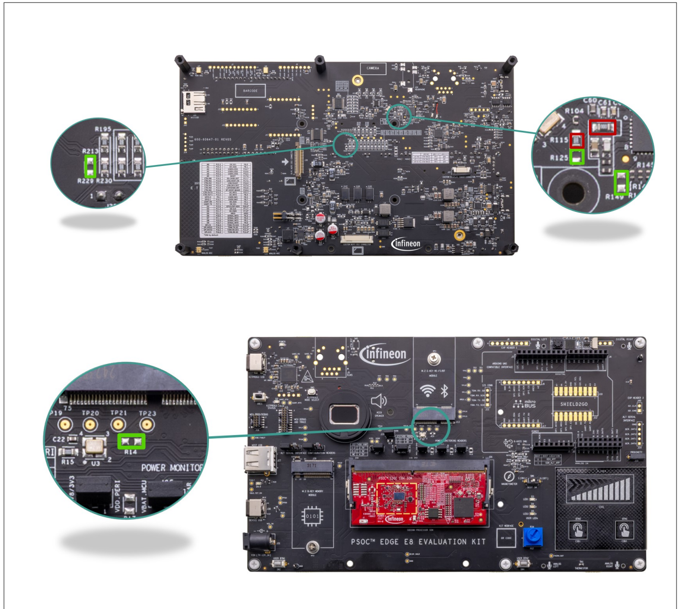
Figure 92 Rework region on baseboard for enabling Ethernet RMII mode
