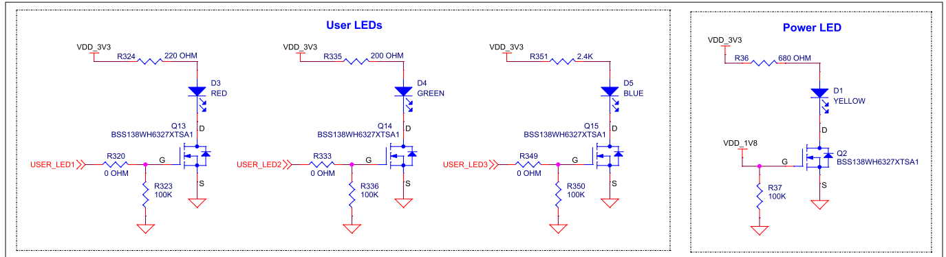
Figure 78 Schematic of User LEDs and Power LED
