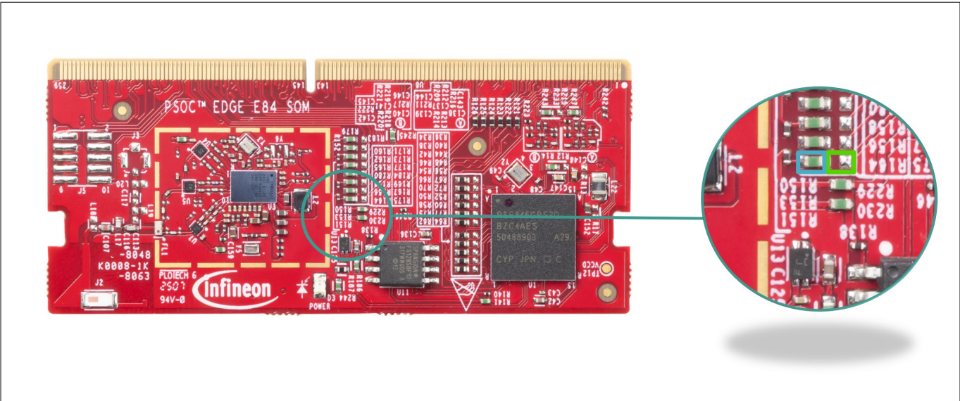
Figure 98 Rework region on SOM for enabling interface with expansion header 2
