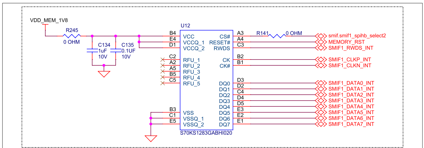
Figure 27 HYPERRAM™
