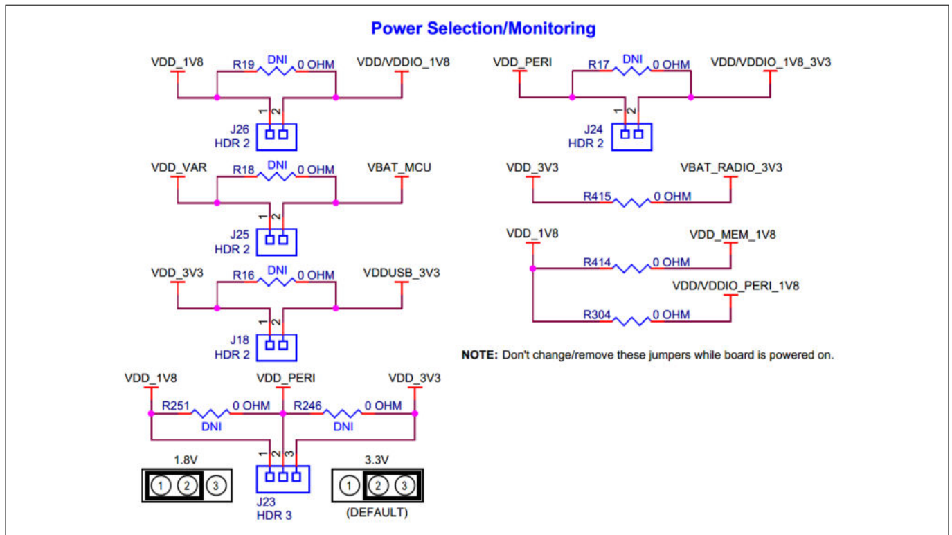
Figure 47 Schematic of PSOC™ Edge E84 power selection and current monitoring headers
