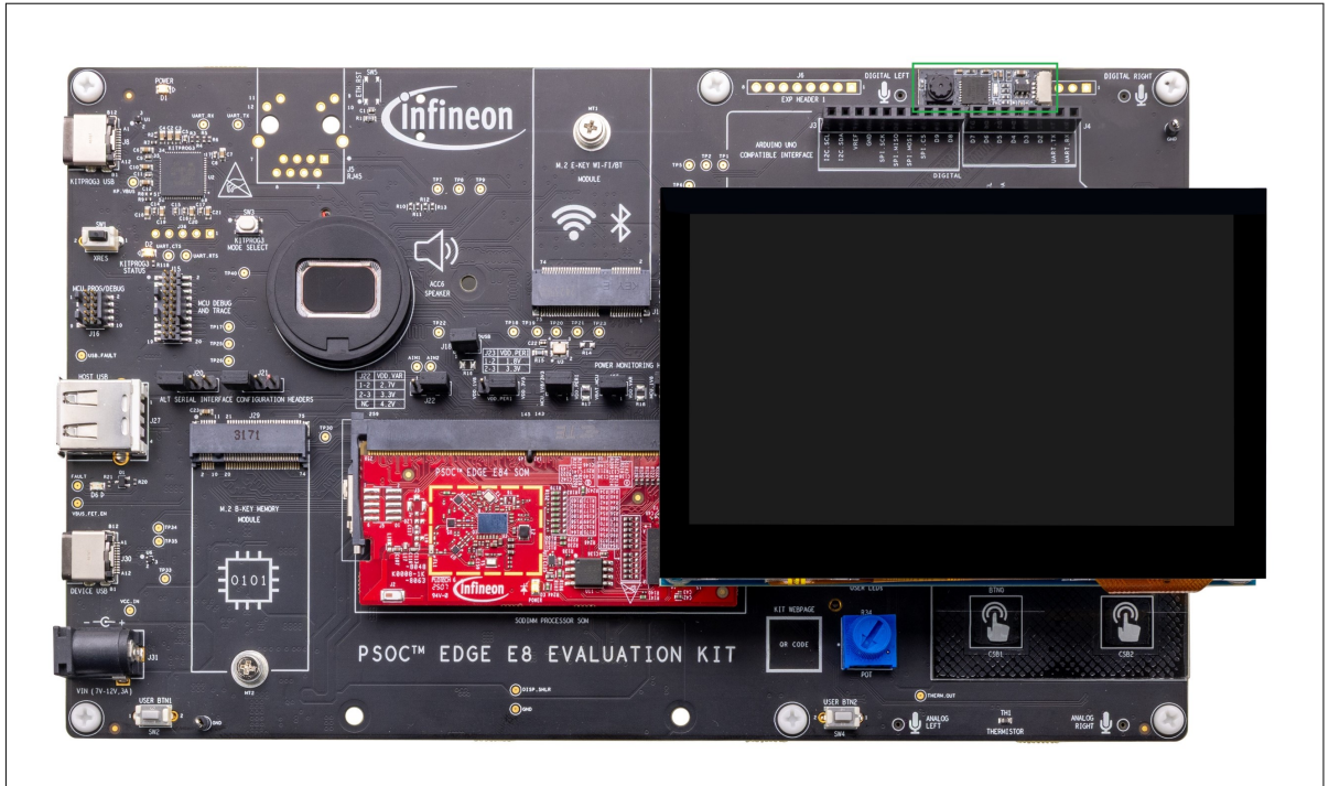
Figure 10 Camera Module placement
