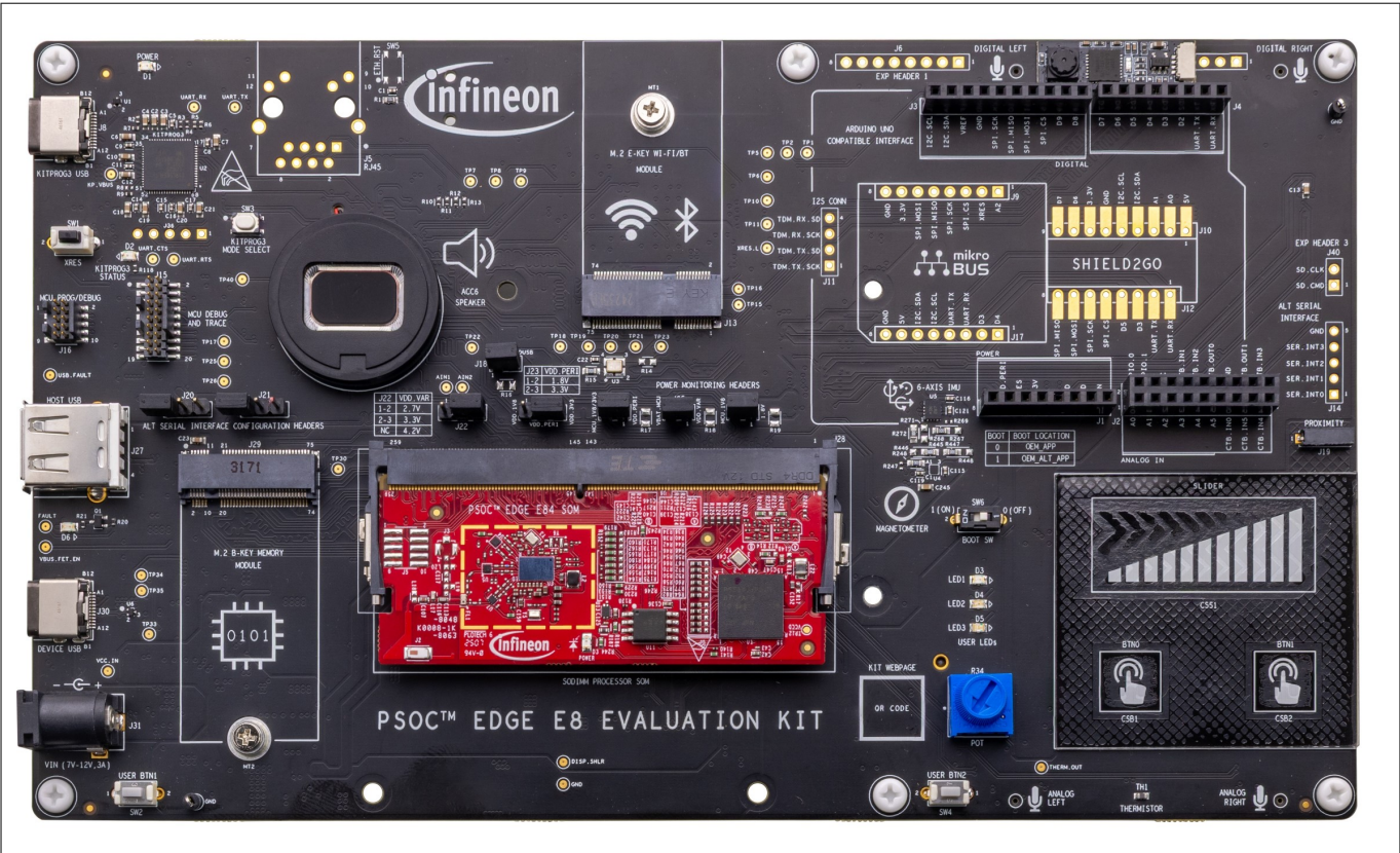
Figure 6 Baseboard top view with SOM connected
