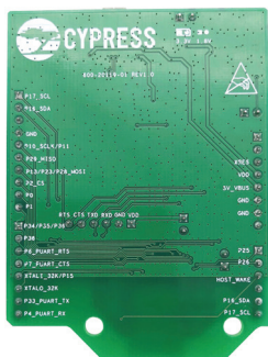
Figure 2: CYBT-413055-EVAL Bottom View
