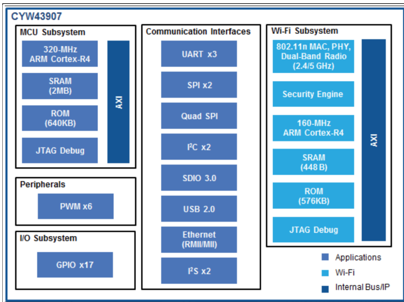
Figure 3 Block diagram
